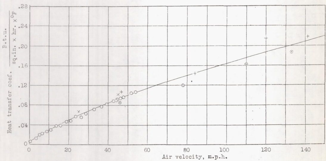
Fig. 25 Heat transfer coefficient vs. air velocity.
