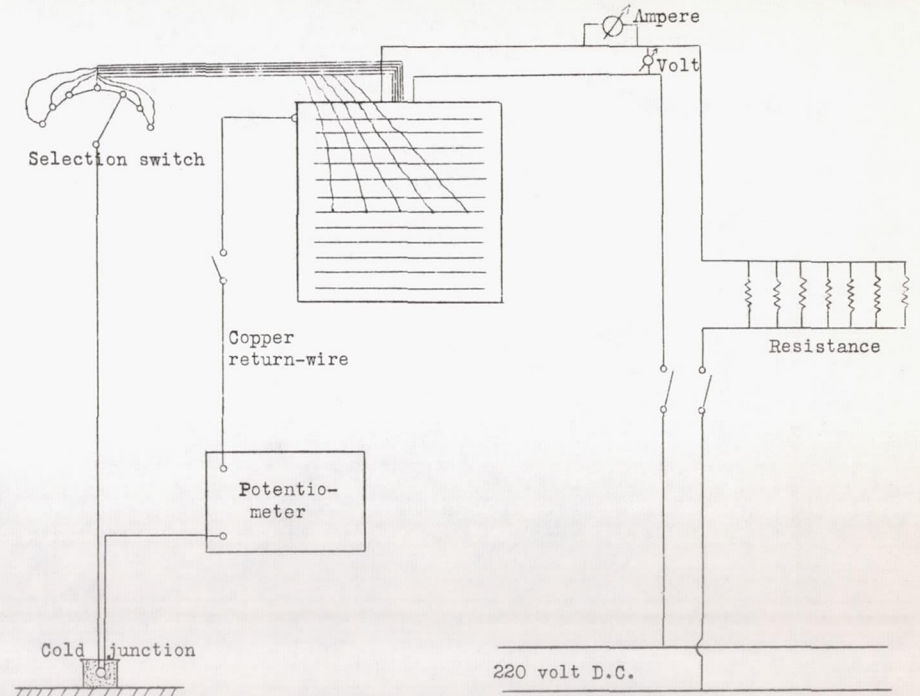
Fig. 5 Electrical connections used for heater and thermocouples.
