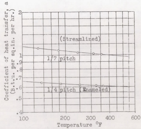
Fig.22 Relation of heat transfer to temperature.
