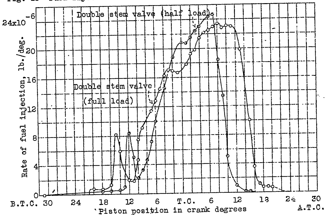
Fig. 16 Fuel injection rate curves for cards of Fig. 15
