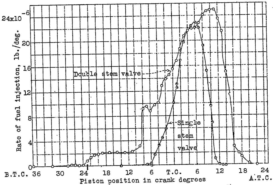
Fig. 13 Fuel injection rate curves for cards of Fig. 12
