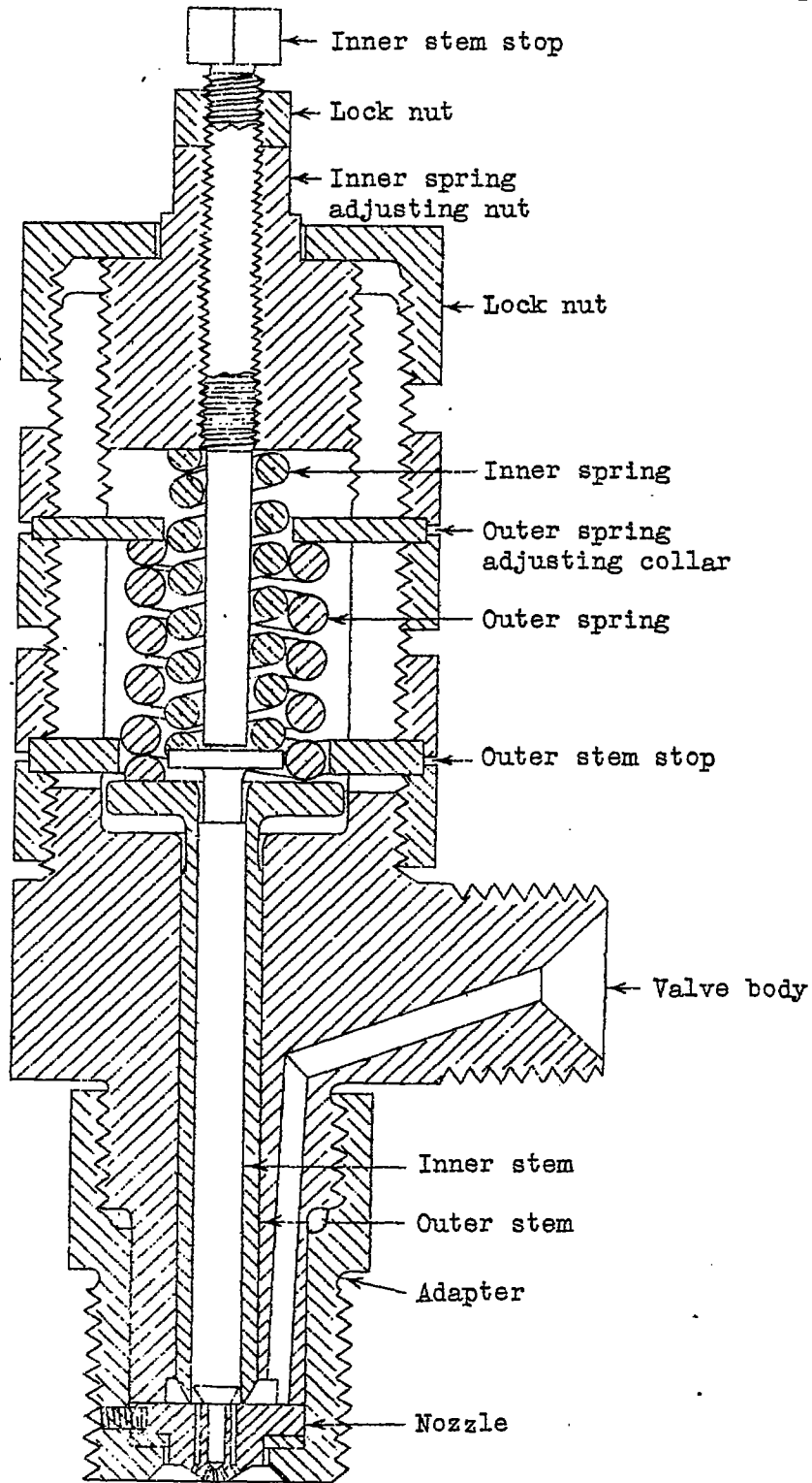
Fig. 2 Double-stem valve
