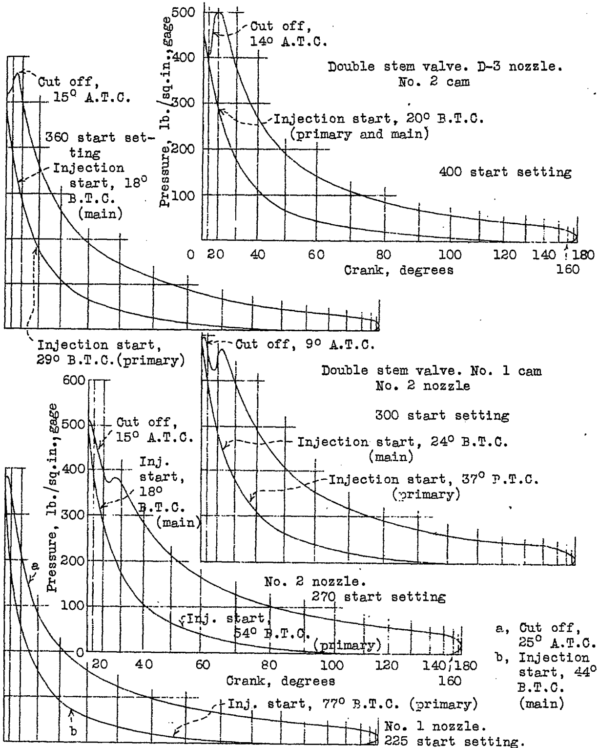
Fig. 19 Effect of rate of pump displacement on P-V cards with double injection
