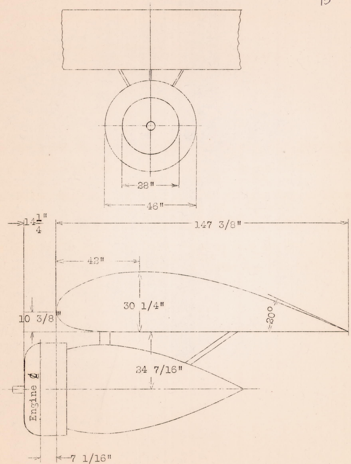
Fig.1 Nacelle and wing profile showing original nacelle location.
