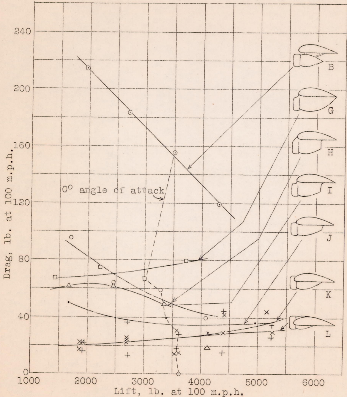
Fig.3 Effect of fairing nacelle into wing.
