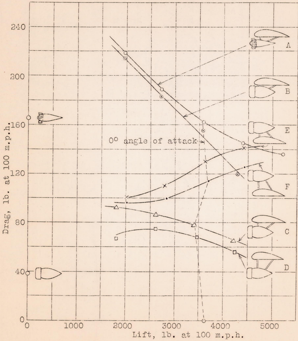
Fig.2 Effect of nacelle position.
