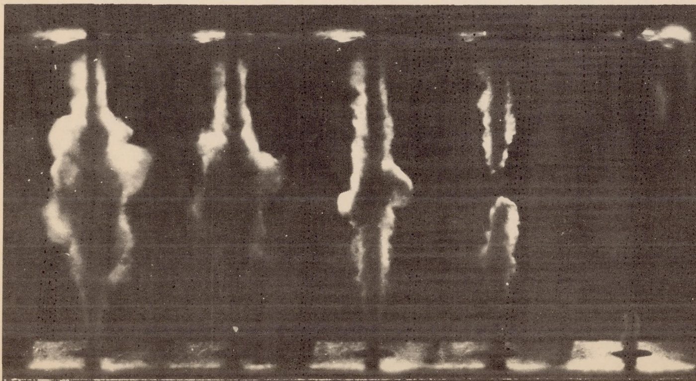
Fig.11 Opposed fuel sprays injected into air having a density corresponding to that in an engine at a compression ratio of 14.5:1. Fuel-injection pressure, 4,000 pounds per square inch. Chamber-air density, 1.1 pounds per cubic foot.
