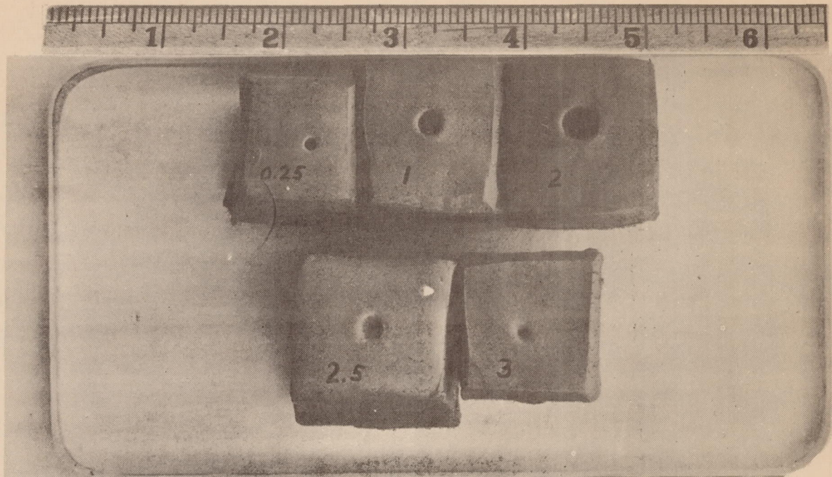
Fig.2 Impressions made in Plasticine by fuel sprays injected through air having a density of 1.1 pounds per cubic foot. Fuel-injection pressure - 4,000 pounds per square inch. Valve-opening pressure - 3,500 pounds per square inch. Figures beside each impression indicate the distance between the nozzle and the Plasticine, in inches.
