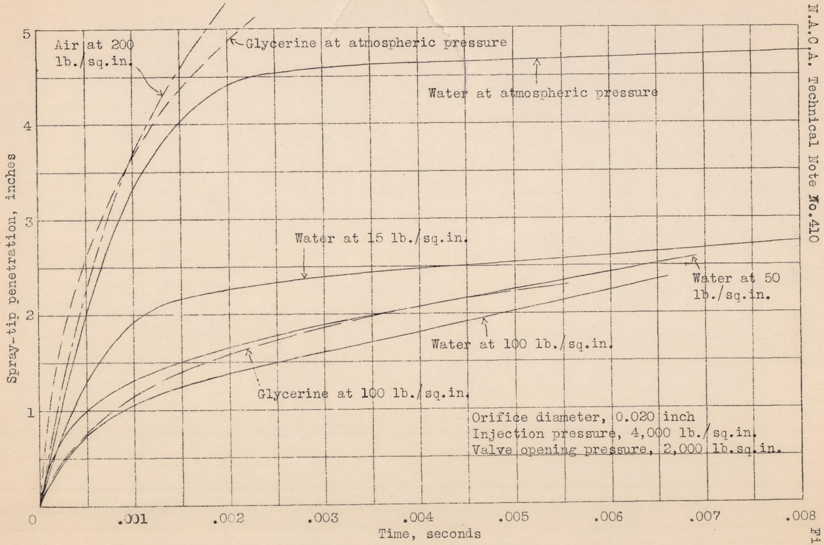
Fig. 7 Effect of the liquid pressure on the spray-tip penetration of fuel sprays injected into water and glycerine.
