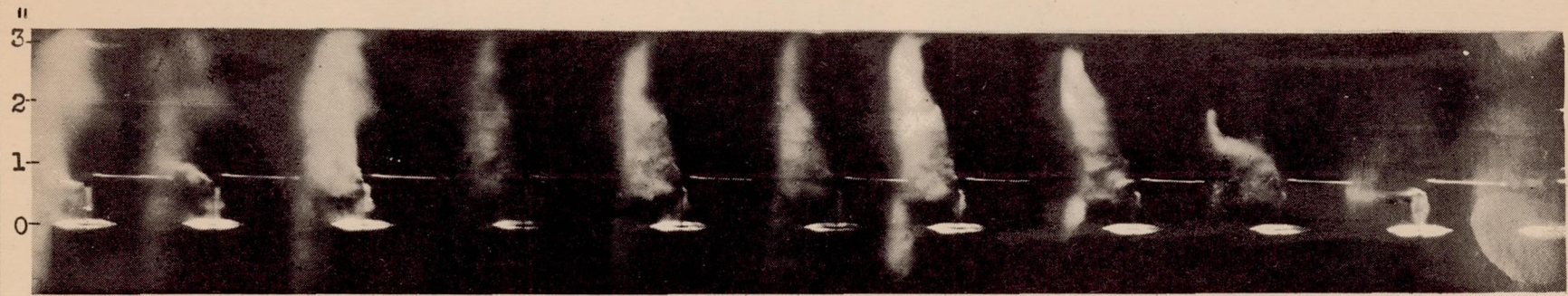
Fig.17 Fuel spray with an air jet impinging at right angles from the right. Fuel-injection pressure,500 pounds per square inch. Air-jet injection pressure,500 pounds per square inch. Chamber-air density,0.076 pounds per cubic foot.
