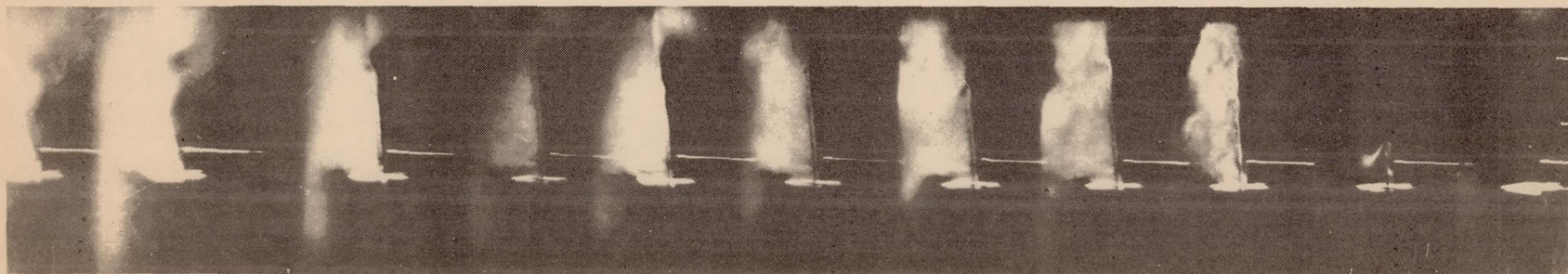
Fig. 16 Fuel spray with an air jet impinging at right angles from the right. Fuel-injection pressure, 1,000 pounds per square inch. Air-jet injection pressure, 200 pounds per square inch. Chamber-air density, 0.076 pounds per cubic foot.
