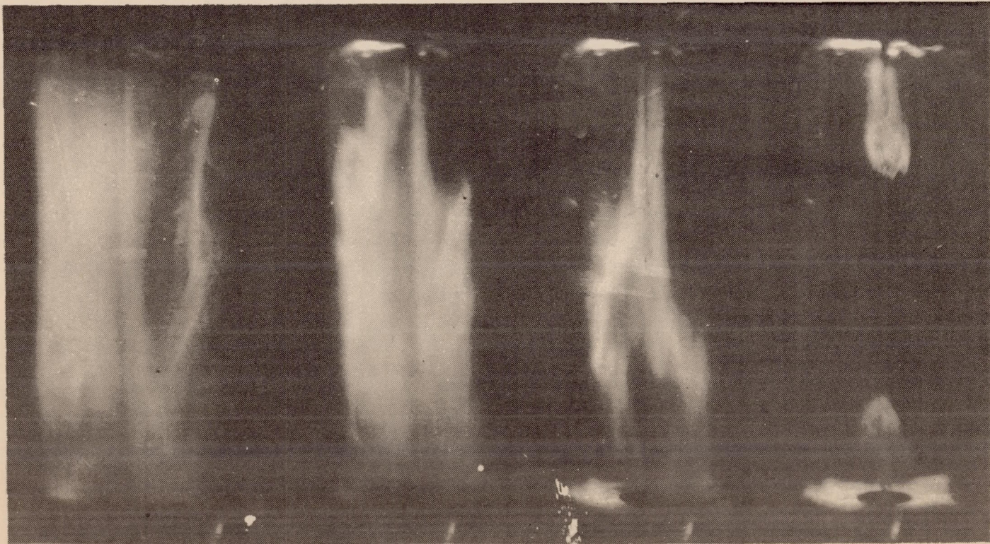
Fig. 8 Opposed fuel sprays injected into an evacuated chamber. Fuel-injection pressure, 4,000 pounds per square inch. Chamber-air density, 0.0025 pounds per cubic foot.
