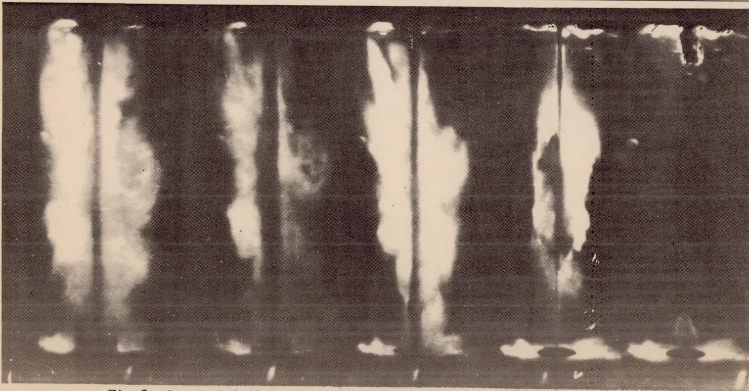
Fig.9 Opposed fuel sprays injected into air at atmospheric density. Fuel-injection pressure, 4,000 pounds per square inch. Chamber-air density, 0.076 pounds per cubic foot.
