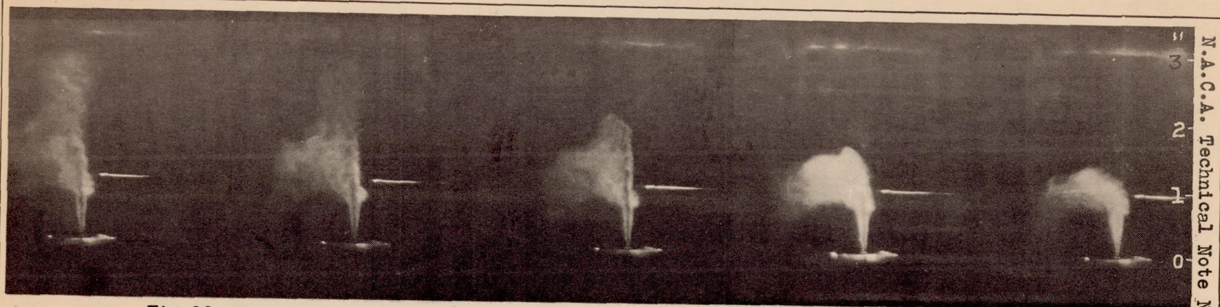
Fig.19 Fuel and air jets intersecting at right angles. Air jet from the right. Fuel-injection pressure, 1,000 pounds per square inch. Air-jet injection pressure, 500 pounds per square inch. Chamber-air density, 1.1 pounds per cubic foot.
