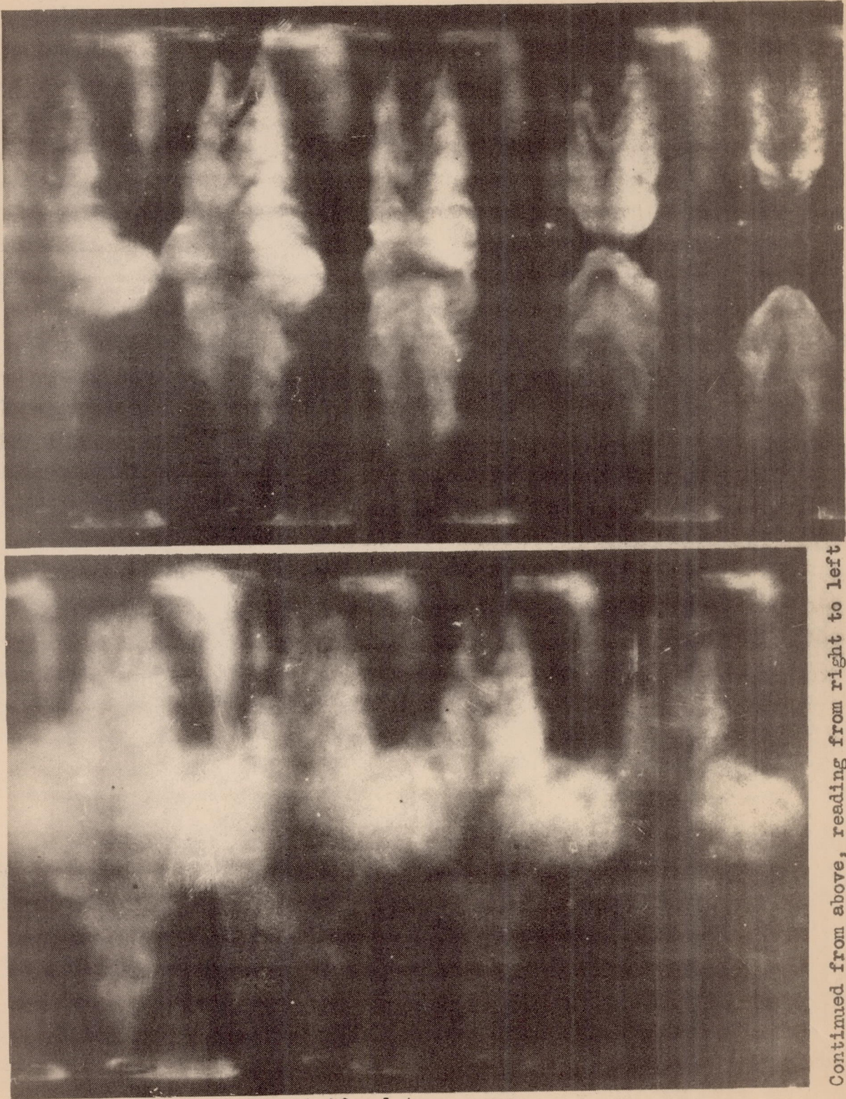
Fig.12 Opposed centrifugal-type sprays. Fuel-injection pressure, 8,000 pounds per square inch. Diameter of orifices, 0.022 inch. Groove helix angles, 40°. Chamber-air density, 1.1 pounds per cubic foot.
