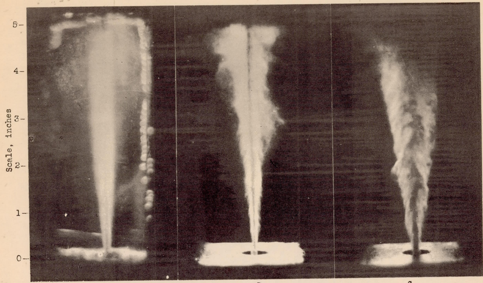
Fig. 4 High-speed spark photographs of fuel sprays injected into air having different densities.
