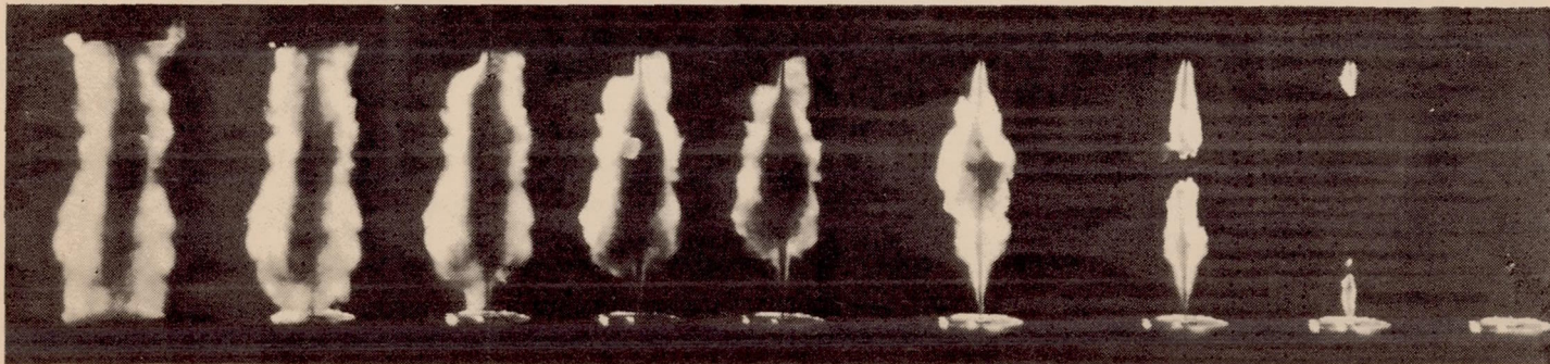
Fig. 14 Opposed sprays using a high injection pressure. Fuel-injection pressure, 4,000 pounds per square inch. Chamber-air density, 1.1 pounds per cubic foot. Distance between open nozzles, 3 inches.
