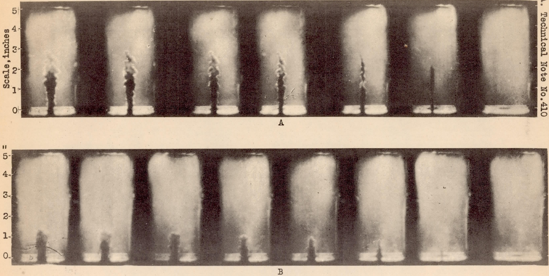
Fig. 6 Diesel oil injected into water. Fuel-injection pressure, 2000 pounds per square inch. Chamber water pressure, (A) Atmospheric. " " " (B) 25 pounds per square inch.
