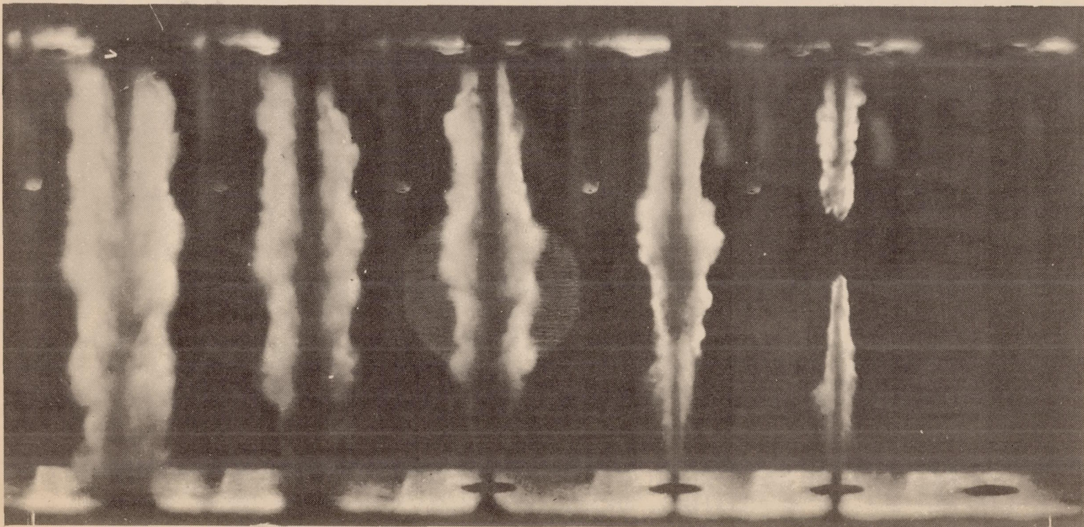
Fig.10 Opposed fuel sprays injected into air having a density corresponding to that in an engine at a compression ratio of 7.9:1. Fuel-injection pressure, 4,000 pounds per square inch. Chamber-air density, 0.60 pounds per cubic foot.
