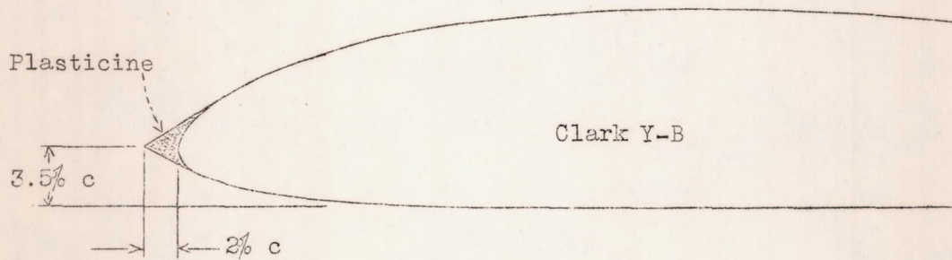
Figure 1.-Sketch showing method of forming sharp leading edges.
