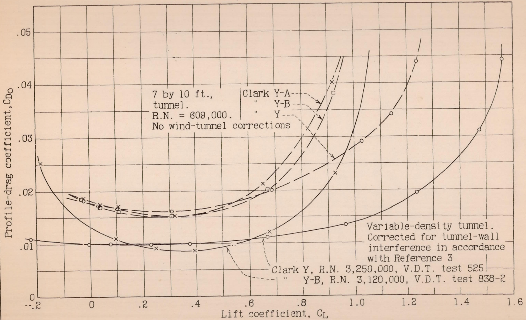
Figure 5 -Profile drag
