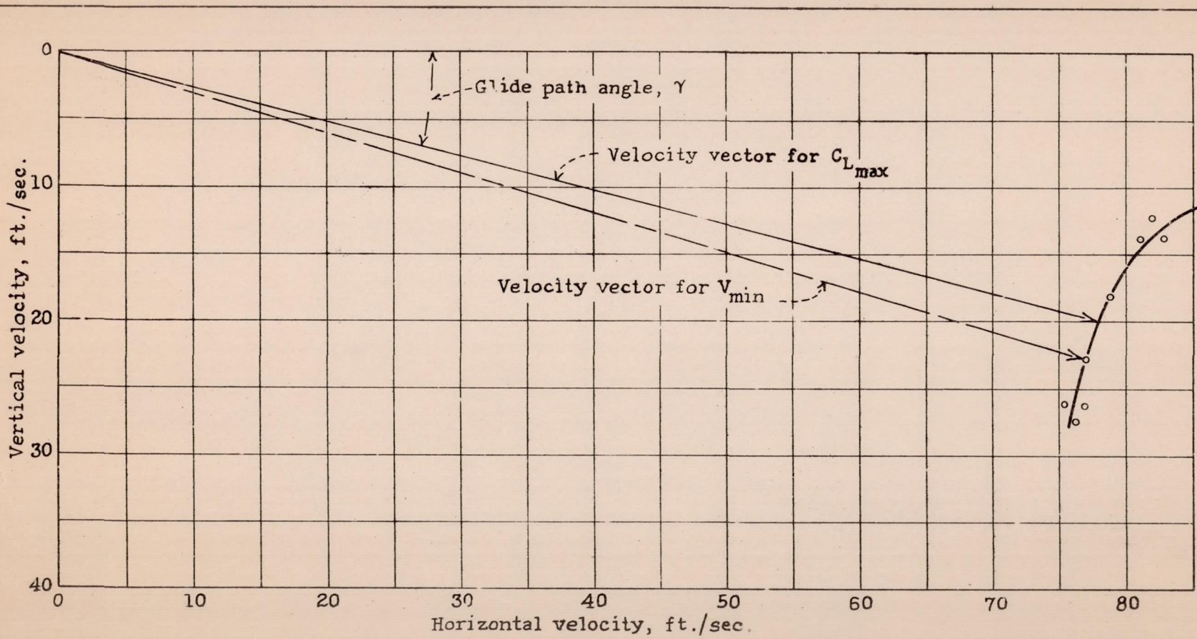
Figure 11 - Typical velocity diagram for XN2Y-1 airplane.
