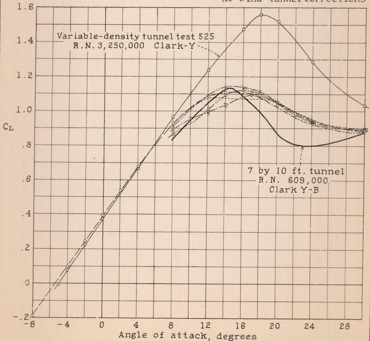
Figure 4.-Comparison of lift curves for the airfoils tested under different conditions
