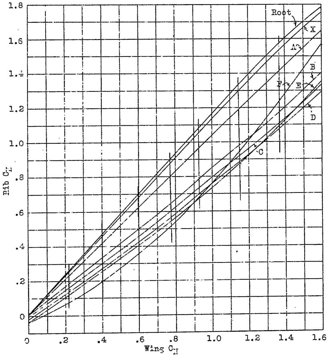
Rib C_{L_i} vs. wing C_{L_i}
