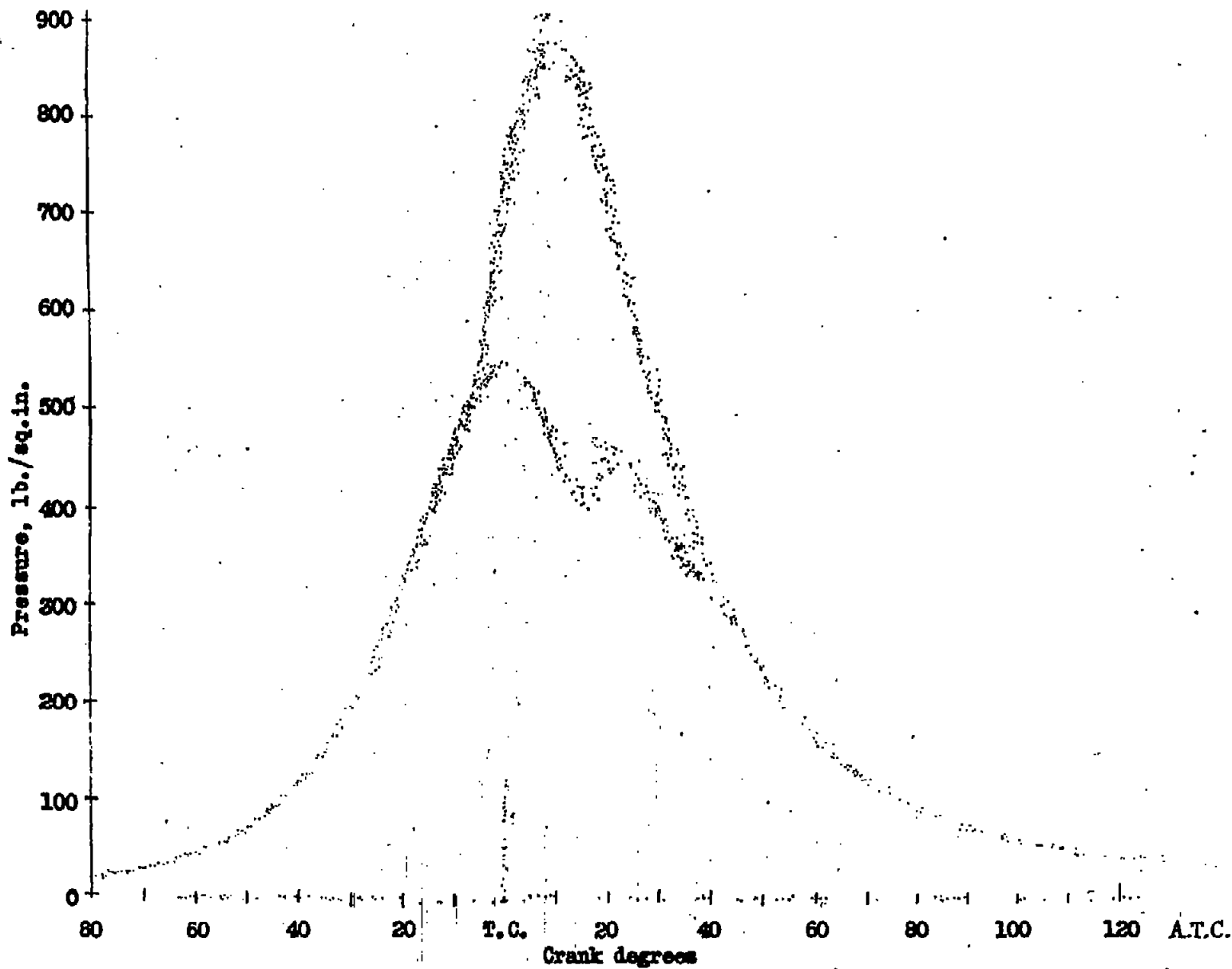
Figure 14.- Typical quiescent combustion chamber indicator card. (Optimum and retarded i.a.a.).
