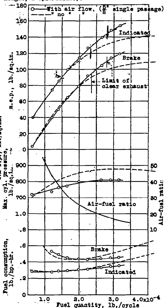
Figure 5.- Comparison of engine performance with and without air flow. (Single-passage displacer, 1,500 r.p.m.).
