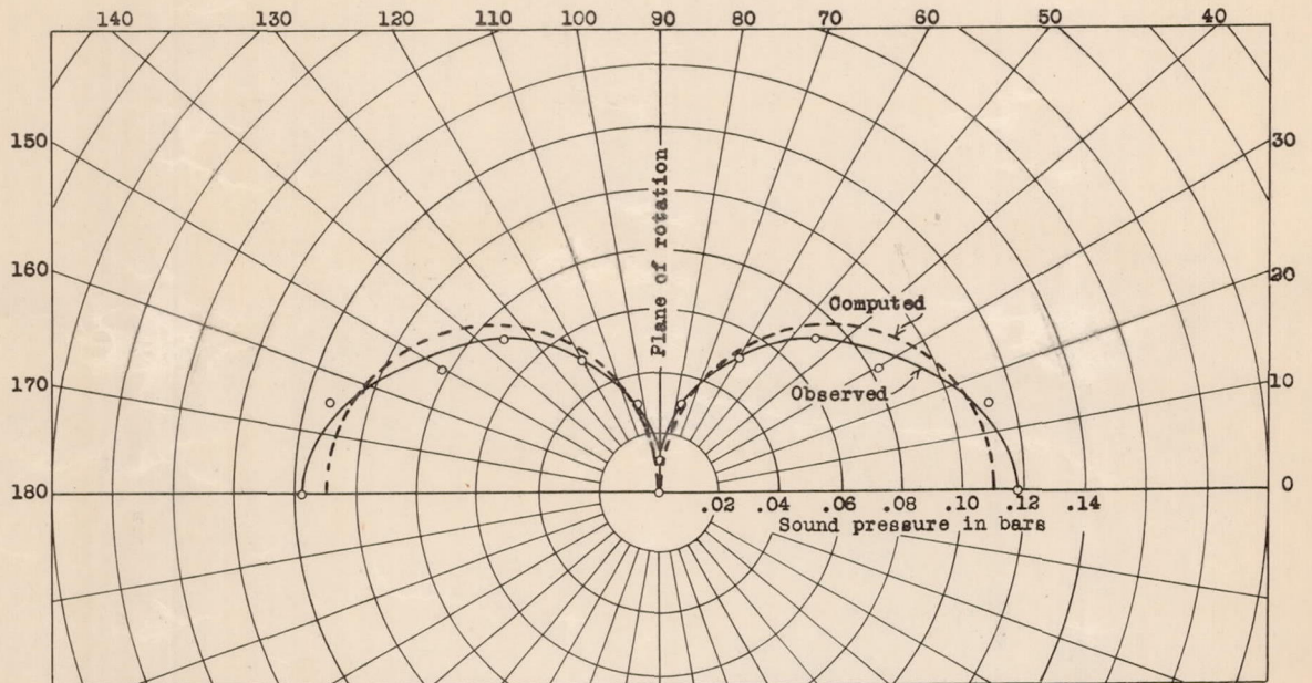
Figure 1.-Distribution of sound pressure about 18-inch rod rotating 2,800 times a minute.
