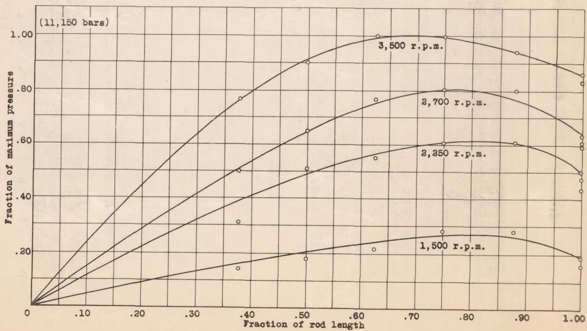
Figure 6.- Pressure distribution along 12-inch rod at four rotational speeds.
