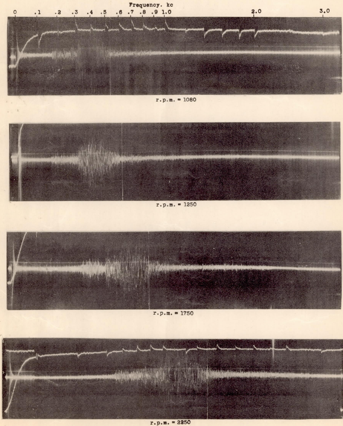
Figure 3.- Sound spectra from 24-inch rod at four rotational speeds. Vertical line indicates computed frequency for tip.
