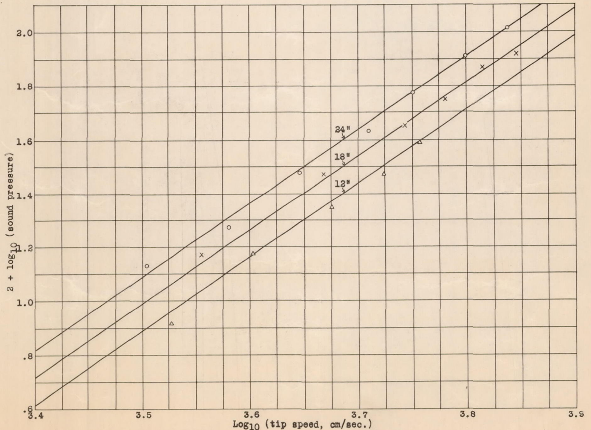
Figure 2.-Variation of sound pressure with tip speed for three rods.
