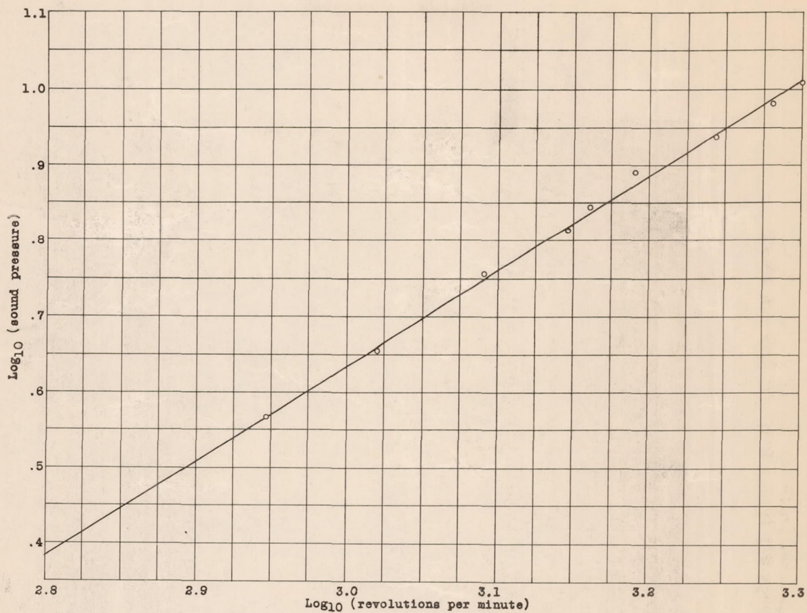
Figure 5.- Variation of pressure field with rotational speed.
