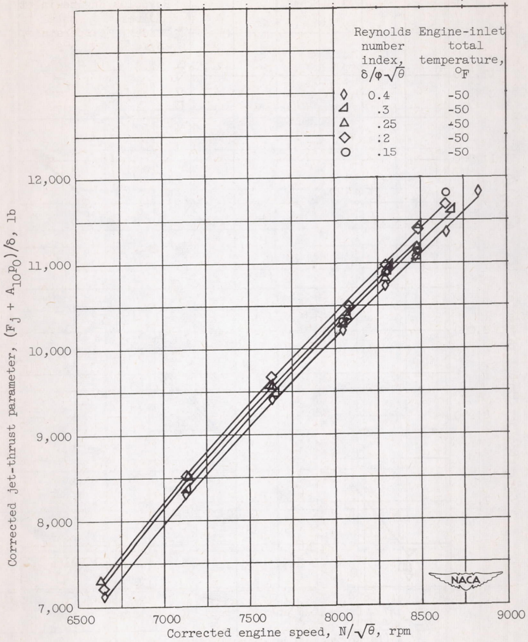
(g) Corrected jet-thrust parameter at inlet temperature of -50° F.
