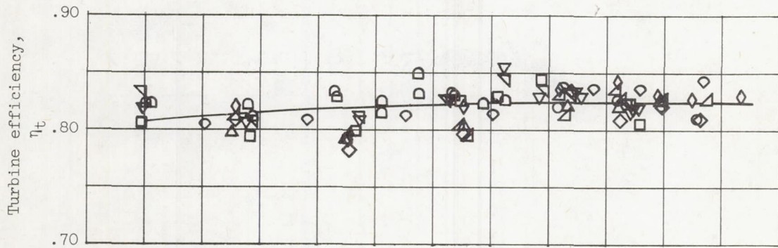
(b) Turbine efficiency.
