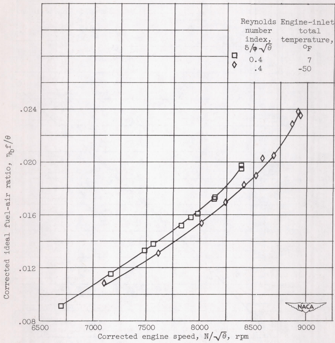
(c) Corrected ideal fuel-air ratio.
