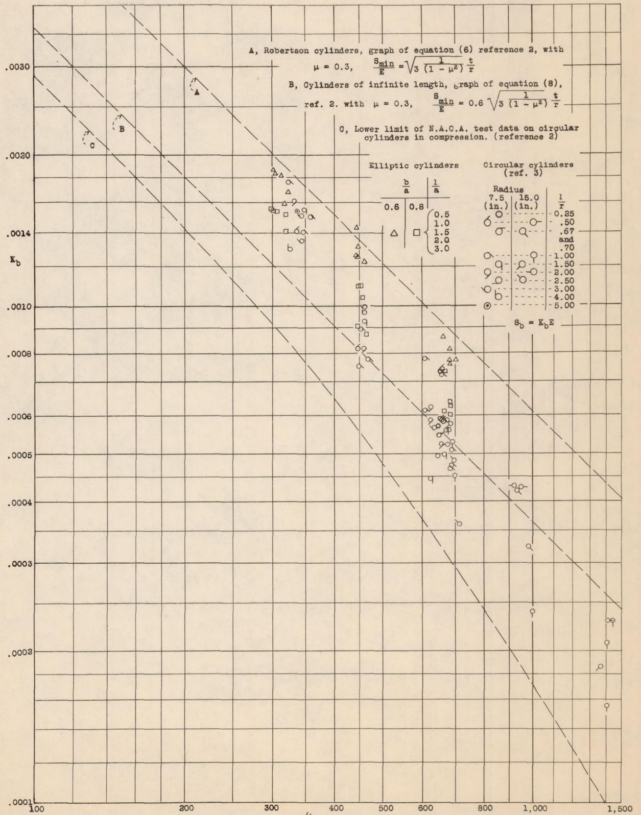
Figure 8. - Logarithmic plot of K_b against radius/thickness ratio (pure bending tests).
