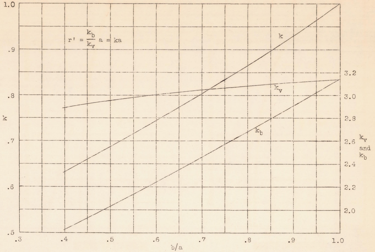
Figure 7.- Stress coefficients.
