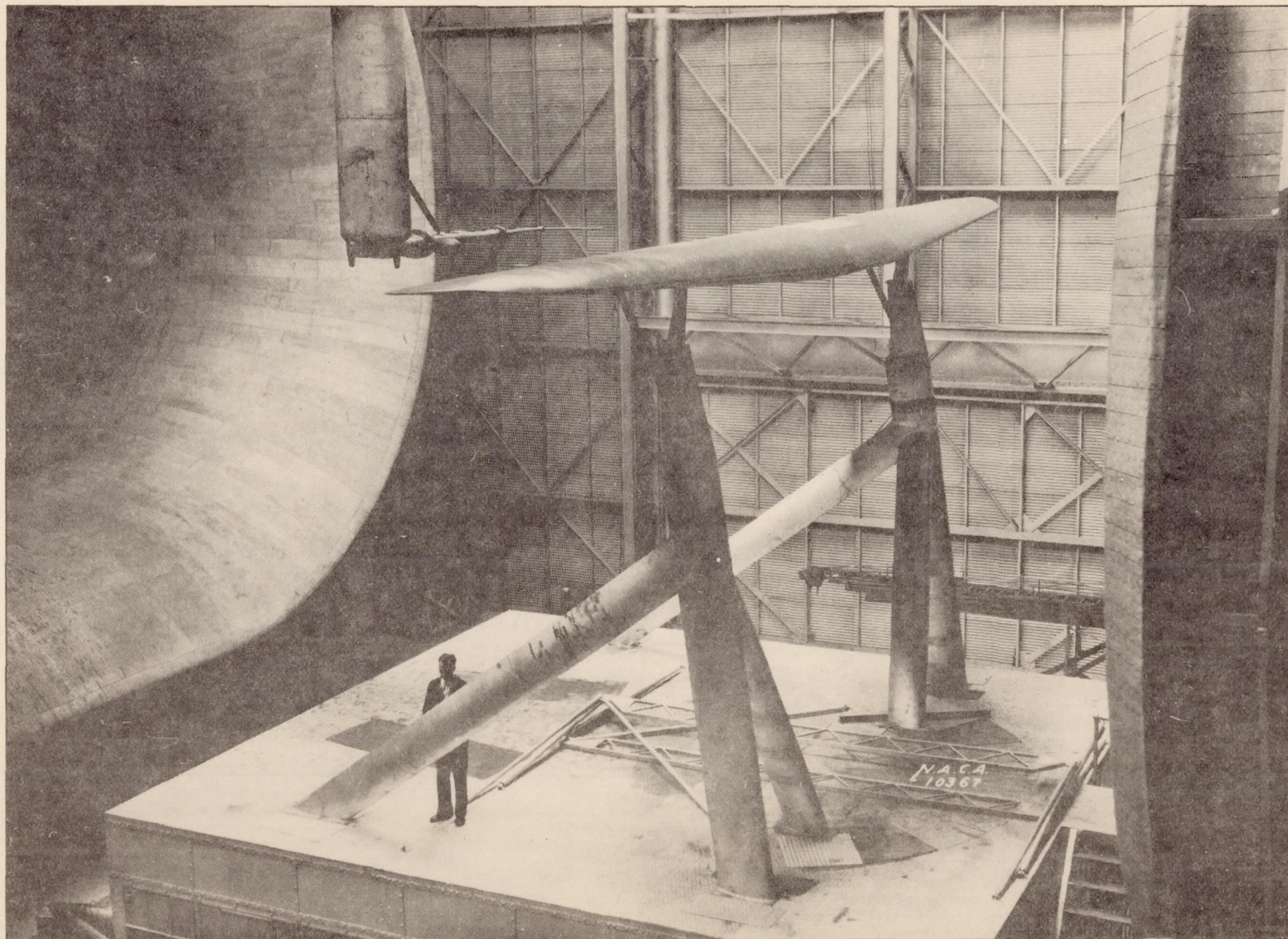
Figure 5.- Typical test set-up. The 3:1 tapered U.S.A. 45 airfoil.
