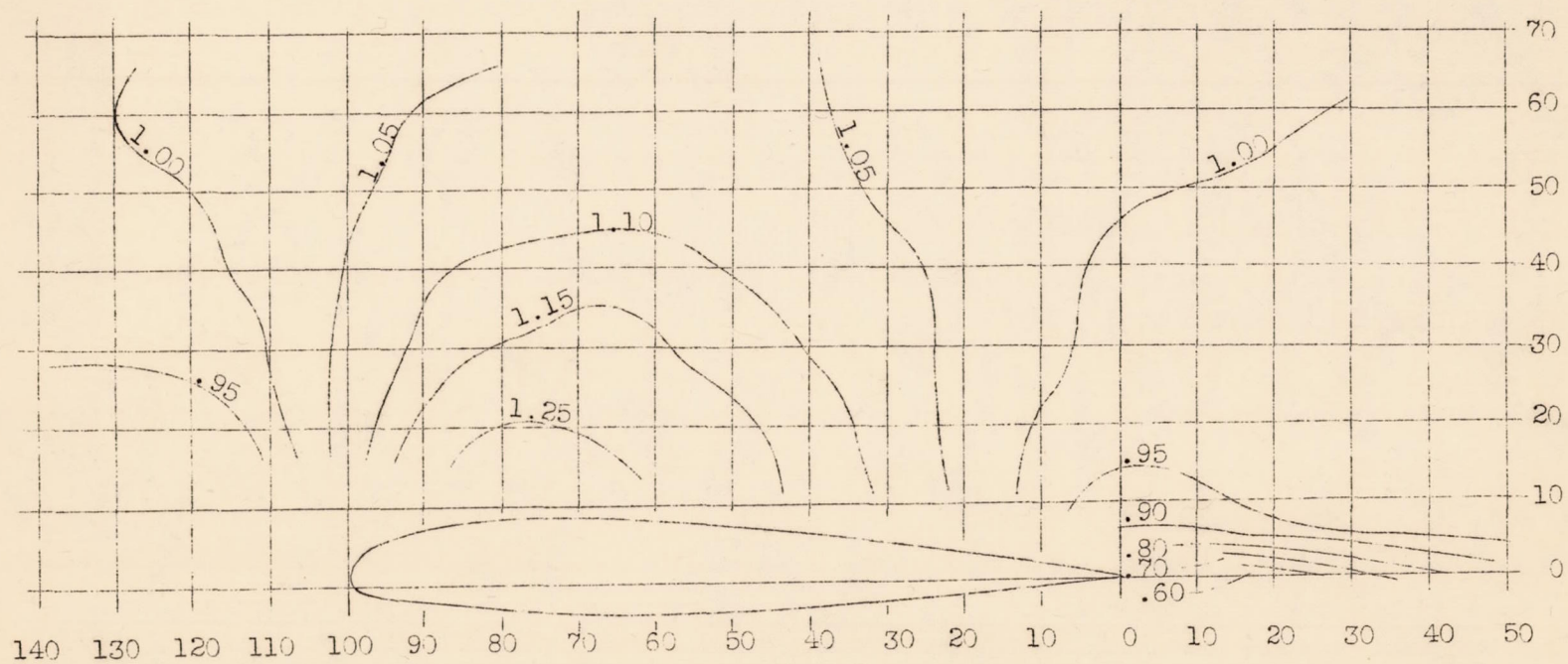
Figure 14.- Rectangular N.A.C.A. 23012 airfoil, 6 by 36 ft. Survey station: 0.389 semispan inboard of wing tip. Pitot axis parallel to airfoil chord. Coordinates in percentage of chord. Contours of q/q_{true} , \alpha = -0.2^\circ , C_L = 0.070
