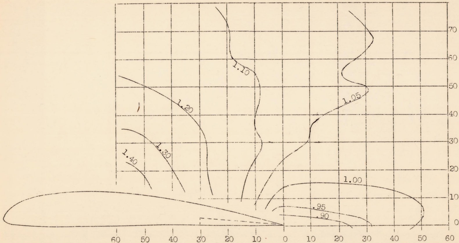
Figure 16.- Fairchild 22 with Zap flap. Wing: 5.21 (mean chord) by 32.83 ft., N-22 section profile, rectangular (rounded tip) form. Zap flap: chord, 1.65 ft., total flap area, 44.0 sq. ft., flap closed, \delta_f = 0^\circ , hinge axis at 70 percent chord. Survey station: 0.431 semispan inboard of wing tip. Chord at survey station: 5 ft. 6 in. Pitot axis parallel to wing chord. Coordinates in percentage of chord. Contours of q/q_{true} , \alpha = -0.8^\circ , C_L = 0.376
