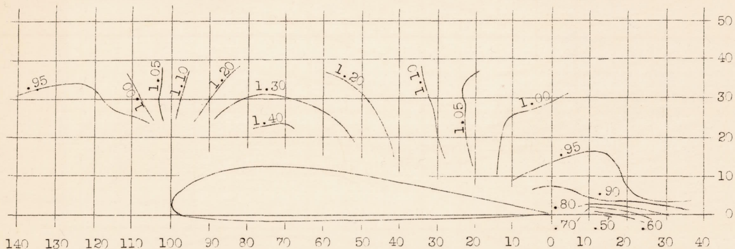
Figure 10.- Y0-31A mock-up. Wing: 7.38 (mean chord) by 45.75 ft., U.S.A. 45 section profile, elliptical plan form. Survey station: 0.429 semispan inboard of wing tip. Chord at survey station: 8 ft. 3 13/32 in. Pitot axis parallel to wing chord. Coordinates in percentage of chord. Contours of q/q_{\text{true}} , \alpha = -0.4^\circ , C_L = 0.153
