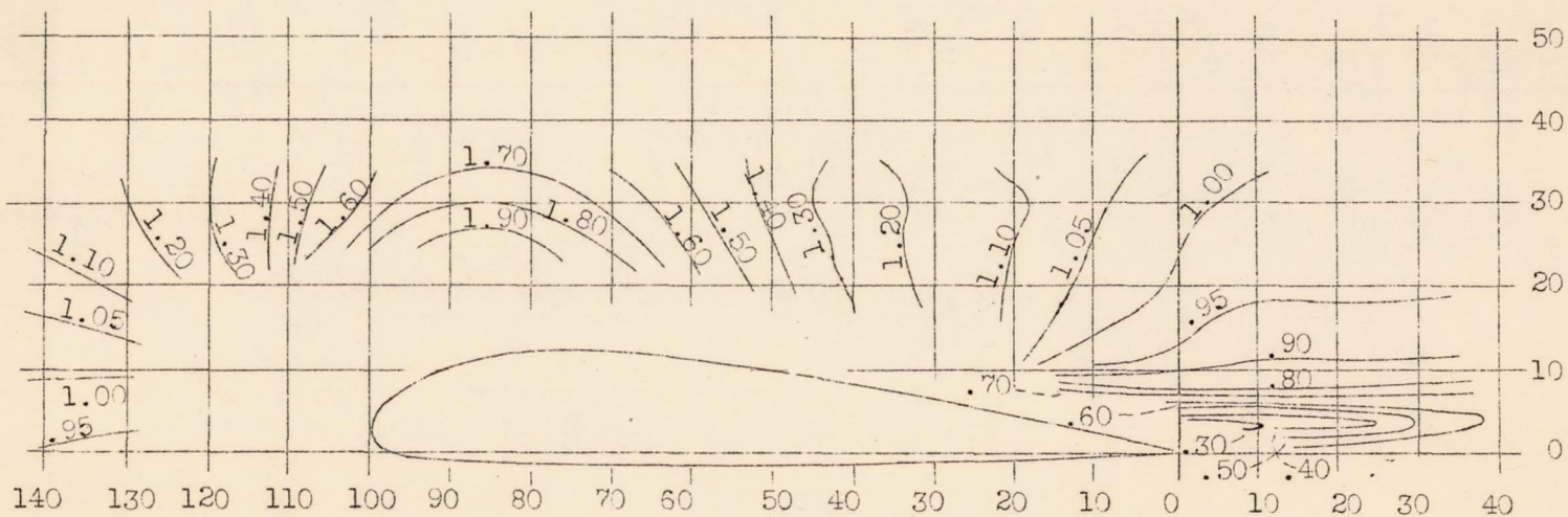
Figure 11.- YO-31A mock-up. Wing: 7.38 (mean chord) by 45.75 ft., U.S.A. 45 section profile, elliptical plan form. Survey station: 0.429 semispan inboard of wing tip. Chord at survey station: 8 ft. 3 \frac{13}{32} in. Pitot axis parallel to wing chord. Coordinates in percentage of chord. Contours of q/q_{\text{true}} , \alpha = 15.9^\circ , C_L = 1.345
