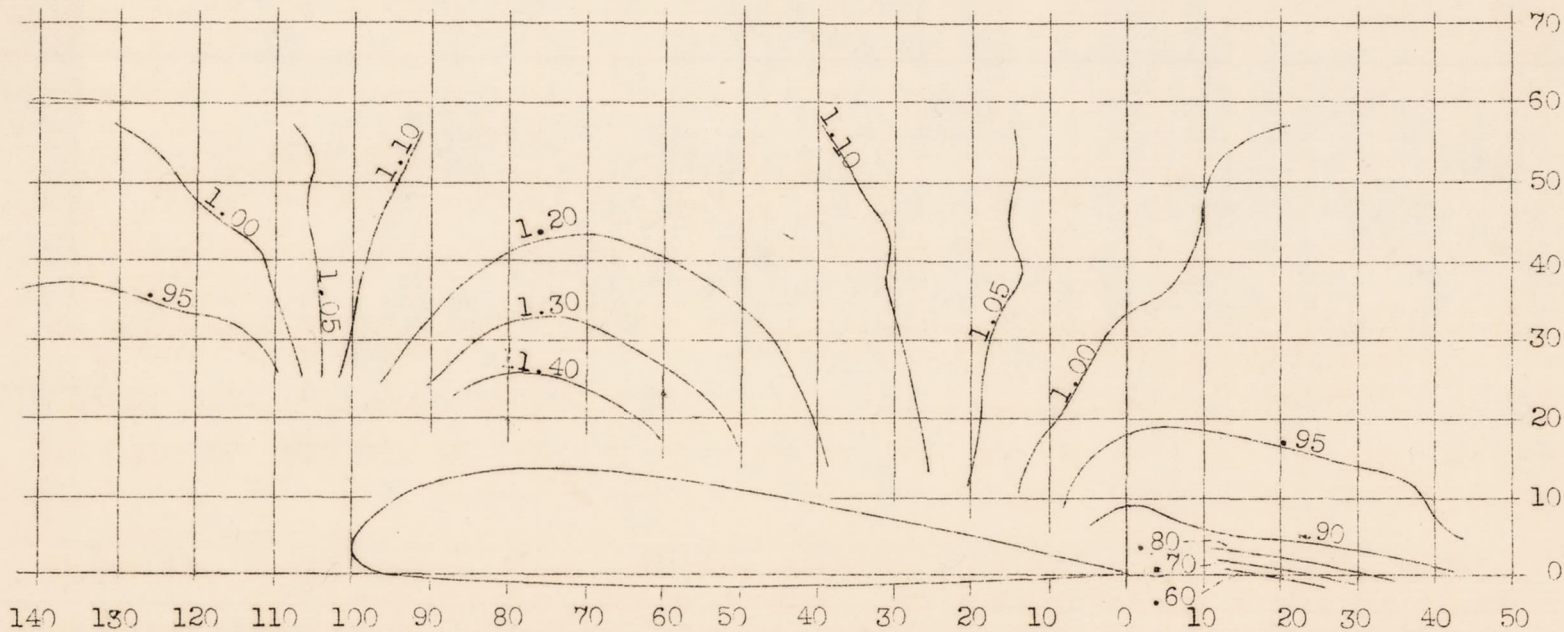
Figure 12.- 2:1 tapered U.S.A. 45 airfoil, 7.38 (mean chord) by 45.75 ft. Survey station: 0.432 semispan inboard of wing tip. Chord at survey station: 7 ft. 2 in. Pitot axis parallel to airfoil chord. Coordinates in percentage of chord. Contours of q/q_{true} , \alpha = -0.5^\circ , C_L = 0.240
