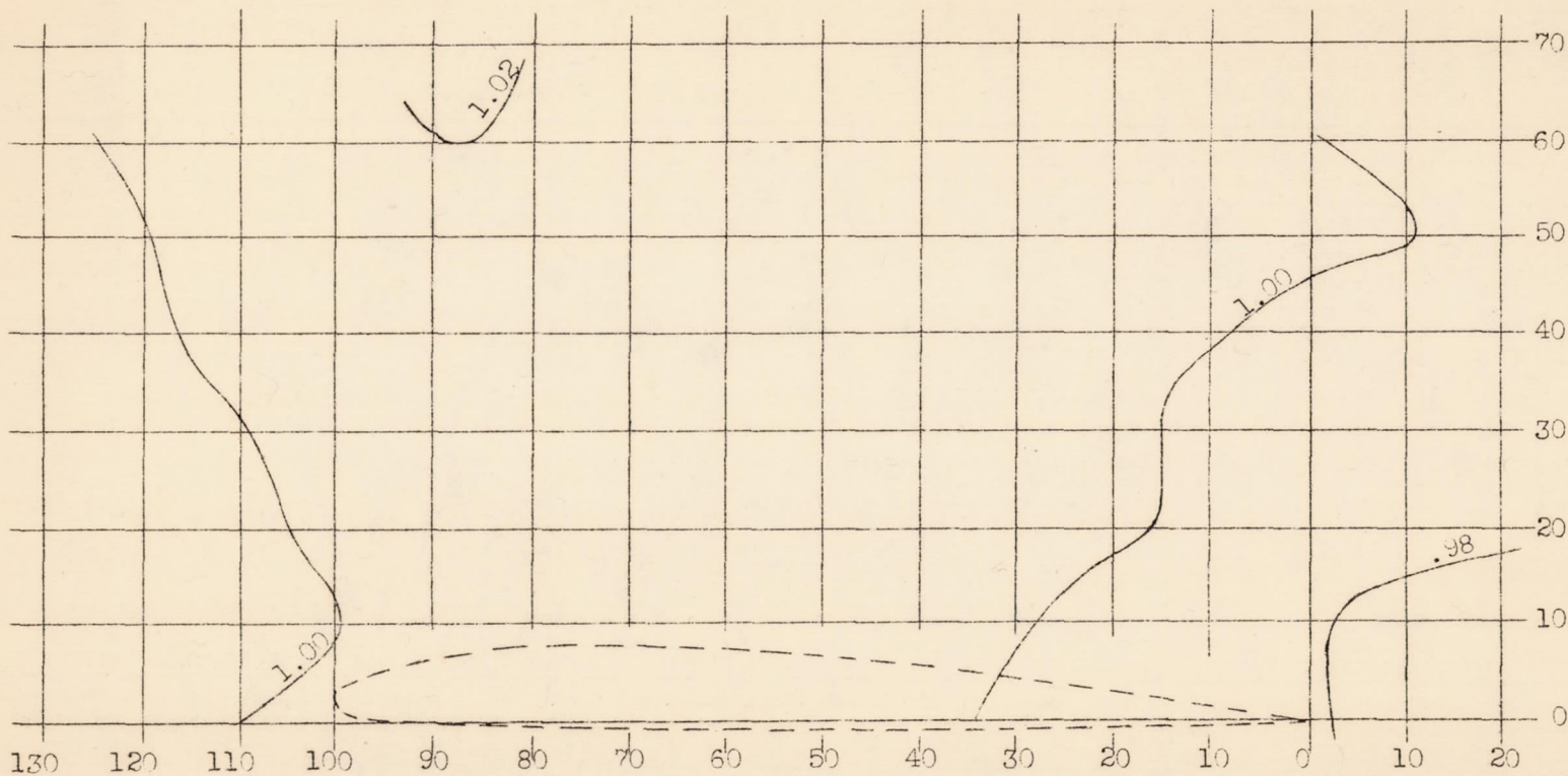
Figure 6.- YO-31A mock-up. Wing: 7.38 (mean chord) by 45.75 ft., U.S.A. 45 section profile, elliptical plan form. Survey station: 0.043 semispan outboard of wing tip. Coordinates in percentage of chord at station 0.036 semispan inboard of wing tip, chord 3 ft. 5 \frac{15}{32} in. Pitot axis parallel to wing chord. Contours of q/q_{true} , \alpha = -0.4^\circ , C_L = 0.153
