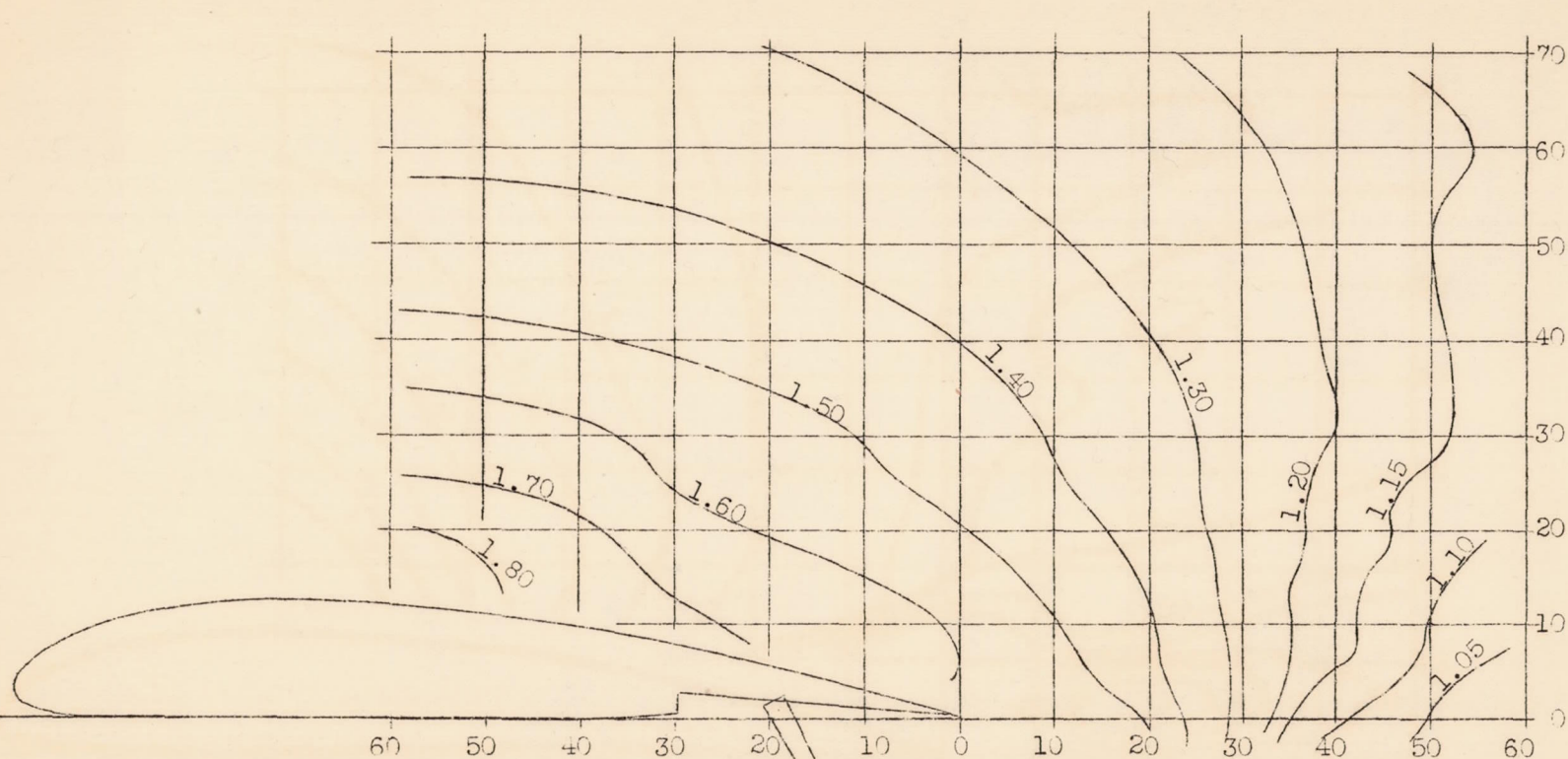
Figure 18.- Fairchild 22 with Zap flap. Wing: 5.21 (mean chord) by 32.83 ft., N-22 section profile, rectangular (rounded tip) plan form. Zap flap: chord, 1.65 ft., total flap area, 44.0 sq. ft., flap open, \delta_f = 59^\circ , hinge axis at 80 percent chord. Survey station: 0.431 semispan inboard of wing tip. Chord at survey station: 5 ft. 6 in. Pitot axis parallel to wing chord. Coordinates in percentage of chord. Contours of q/q_{true} , \alpha = -1.9^\circ , C_L = 1.286
