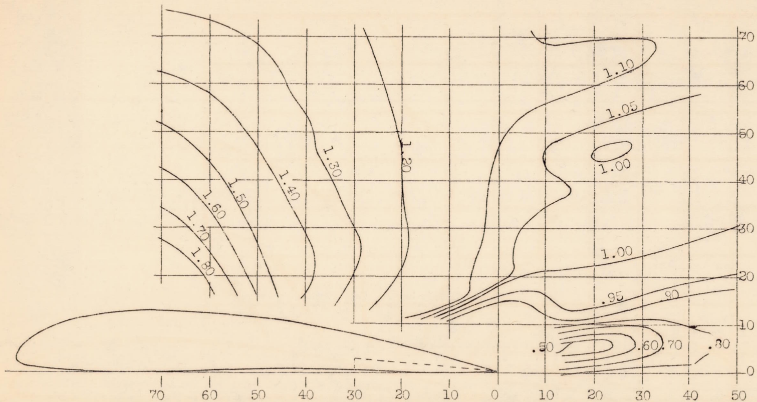
Figure 17.- Fairchild 22 with Zap flap. Wing: 5.21 (mean chord) by 32.83 ft., N-22 section profile, rectangular (rounded tip) plan form. Zap flap: chord, 1.65 ft., total flap area, 44.0 sq. ft., flap closed, \delta_f = 0^\circ , hinge axis at 70 percent chord. Survey station: 5 ft. 6 in. Pitot axis parallel to wing chord. Coordinates in percentage of chord. Contours of C_p/q_{true} , \alpha = 17.0^\circ , C_L = 1.420 .
