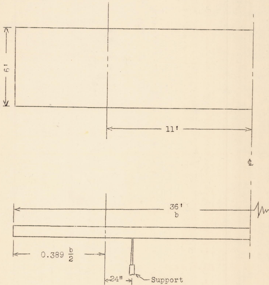
Figure 3.- The survey station for the N.A.C.A. 23012 airfoil.
