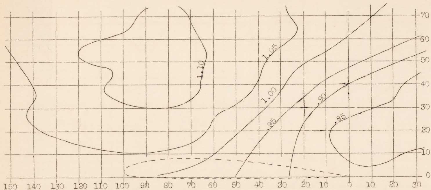
Figure 7.- YO-31A mock-up. Wing: 7.38 (mean chord) by 45.75 ft., U.S.A. 45 section profile, elliptical plan form. Survey station: 0.043 semispan outboard of wing tip. Coordinates in percentage of chord at station 0.036 semispan inboard of wing tip, chord, 3 ft. 5 15/32 in. Pitot axis parallel to wing chord. Contours of q/q_{\text{true}} , \alpha = 15.9^\circ , C_L = 1.345
