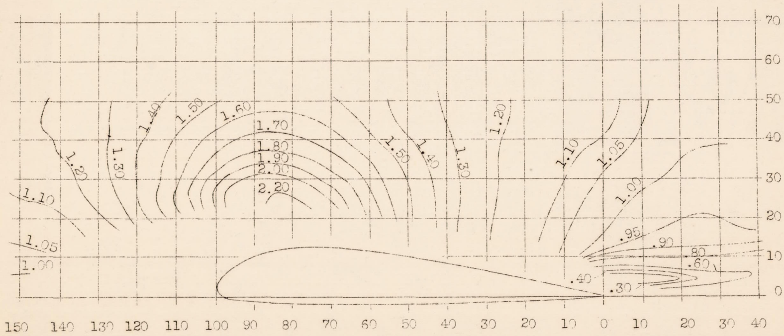
Figure 13.- 2:1 tapered U.S.A. 45 airfoil, 7.38 (mean chord) by 45.75 ft. Survey station: 0.432 semispan inboard of wing tip. Chord at survey station: 7 ft. 2 in. Pitot axis parallel to airfoil chord. Coordinates in percentage of chord. Contours of 1/q_{true} , \alpha = 16.3^\circ , C_L = 1.300
