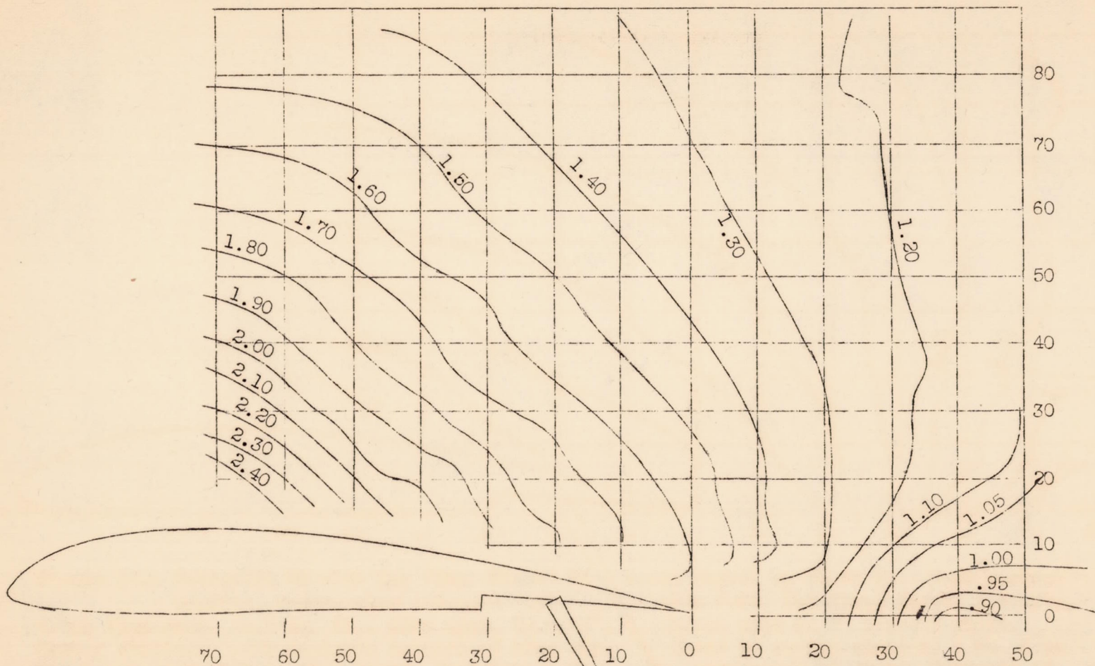
Figure 19.—Fairchild 22 with Zap flap. Wing, 5.21 (mean chord) by 32.83 ft., N-22 section profile, rectangular (rounded tip) plan form. Zap flap, chord, 1.65 ft. total flap area, 44.0 sq.ft., flap open, \delta_f = 59^\circ , hinge axis at 80 percent chord. Survey station, 0.431 semispan inboard of wing tip. Chord at survey station, 5 ft. 6 in. Pitot axis parallel to wing chord. Coordinates in percentage of chord. Contours of q/q_{true} , \alpha = 15.9^\circ , C_L = 2.380
