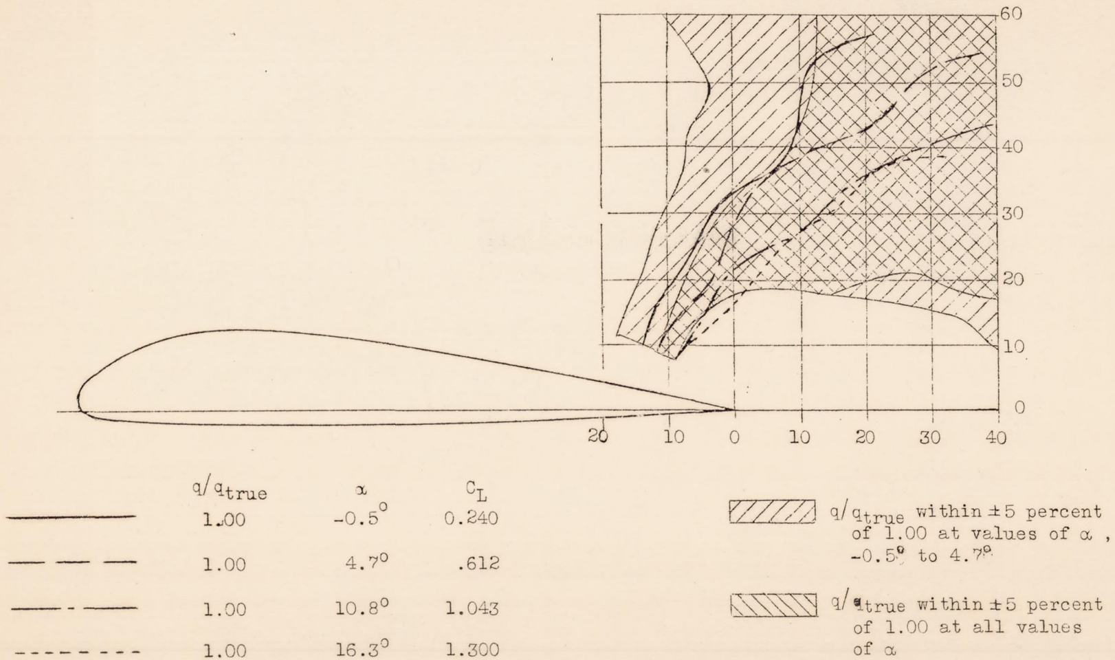
Figure 23.- 2:1 tapered U.S.A. 45 airfoil, 7.38 (mean chord) by 45.75 ft. Survey station: 0.432 semispan inboard of wing tip. Chord at survey station: 7 ft. 2 in. Coordinates in percentage of chord. Pitot axis parallel to airfoil chord.
