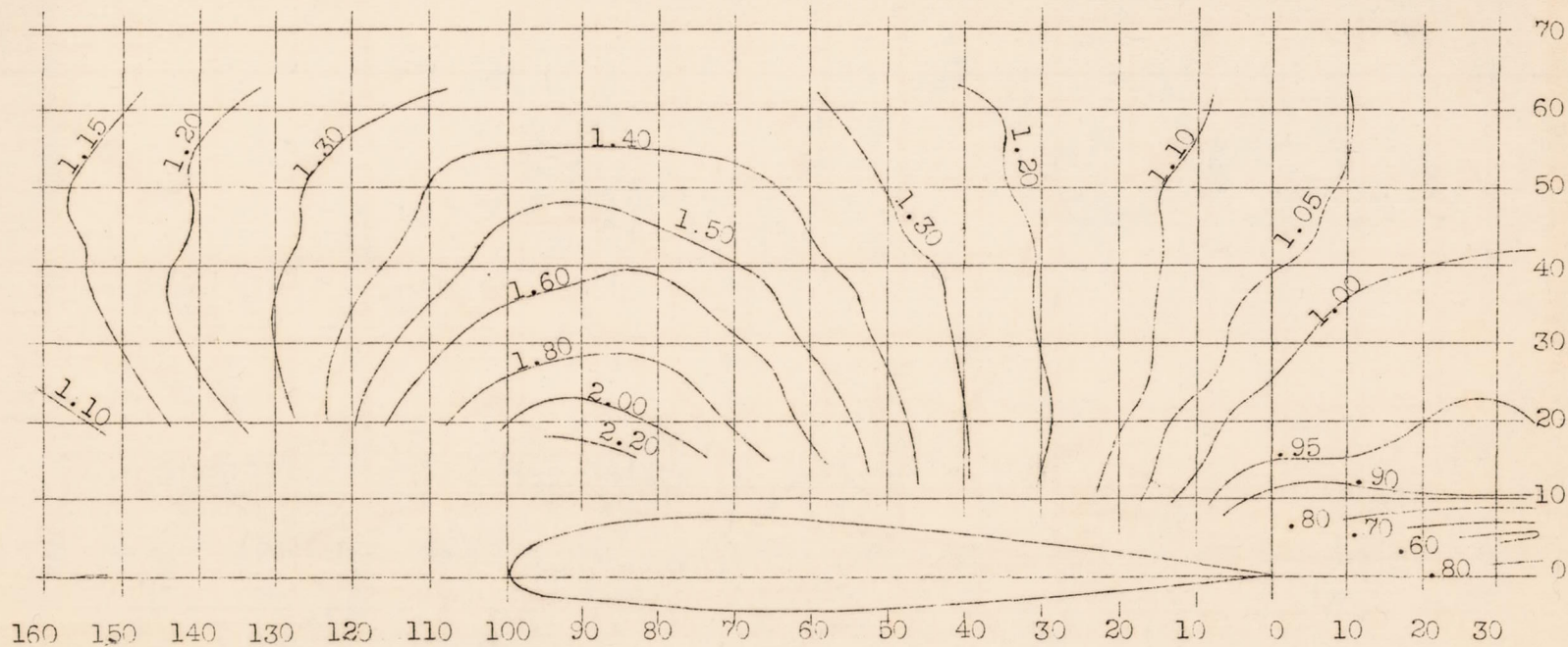
Figure 15.- Rectangular N.A.C.A. 23012 airfoil, 6 by 36 ft. Survey station: 0.389 semispan inboard of wing tip. Pitot axis parallel to airfoil chord. Coordinates in percentage of chord. Contours of q/q_{true} , \alpha = 17.1^\circ , C_L = 1.327
