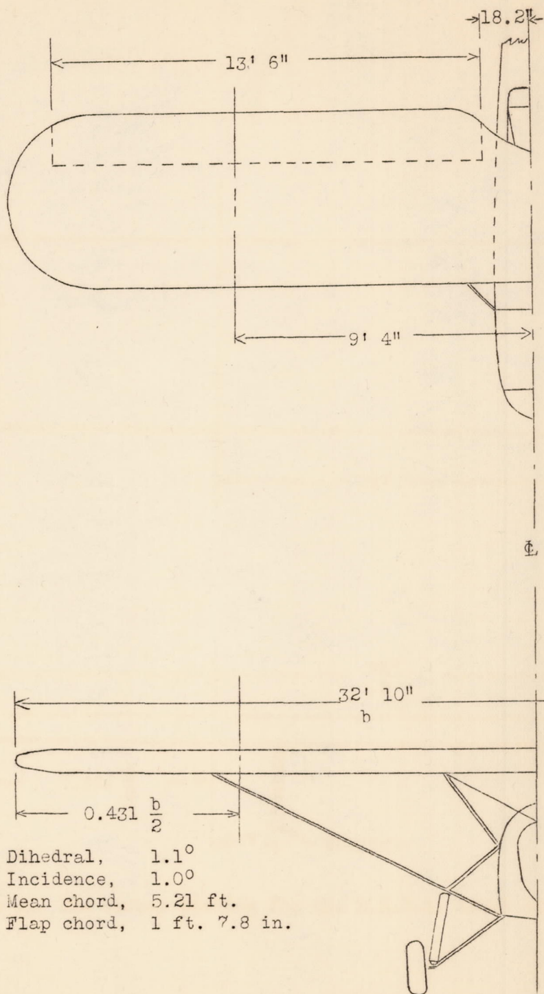
Figure 4.- The survey station for the Fairchild 22 with N-22 airfoil and Zap flap.
