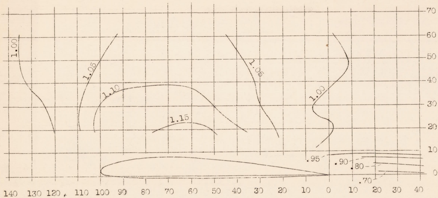
Figure 8.- YO-31A mock-up. Wing: 7.38 (mean chord) by 45.75 ft., U.S.A. 45 section profile, elliptical plan form. Survey station: 0.036 semispan inboard of wing tip. Chord at survey station: 3 ft. 5 \frac{15}{32} in. Pitot axis parallel to wing chord. Coordinates in percentage of chord. Contours of q/q_{true} , \alpha = -0.4^\circ , C_L = 0.153
