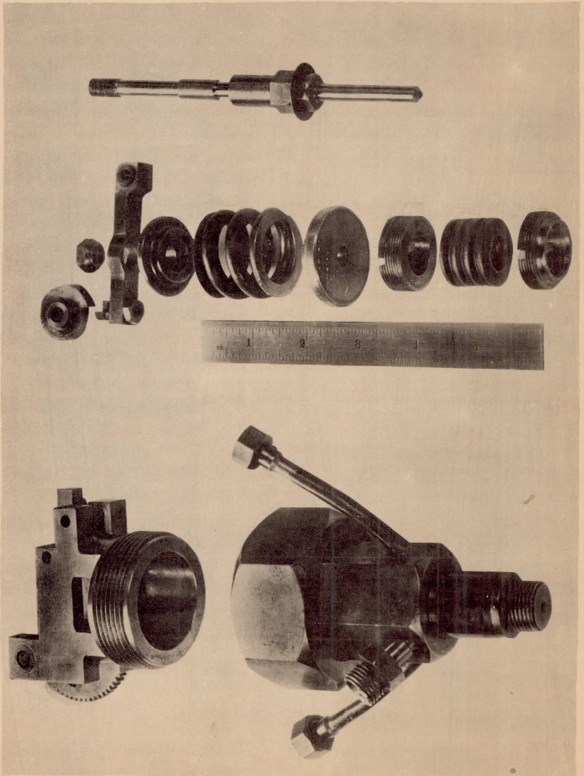
Figure 3.-N.A.C.A. gas-sampling valve (disassembled).
