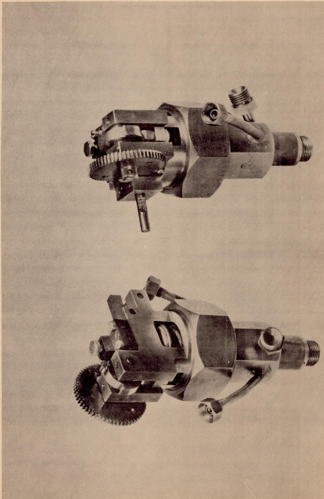
Figure 2.-N.A.C.A. gas-sampling valve (assembled).
