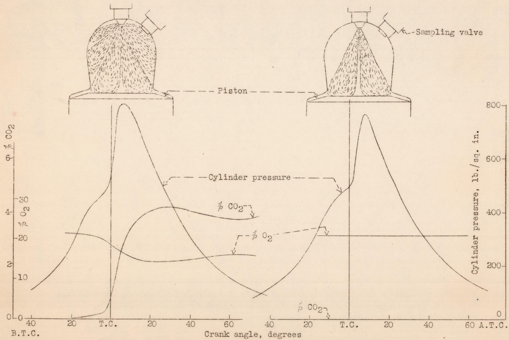
Figure 6.-Combustion process indicated by cylinder gas analysis.
