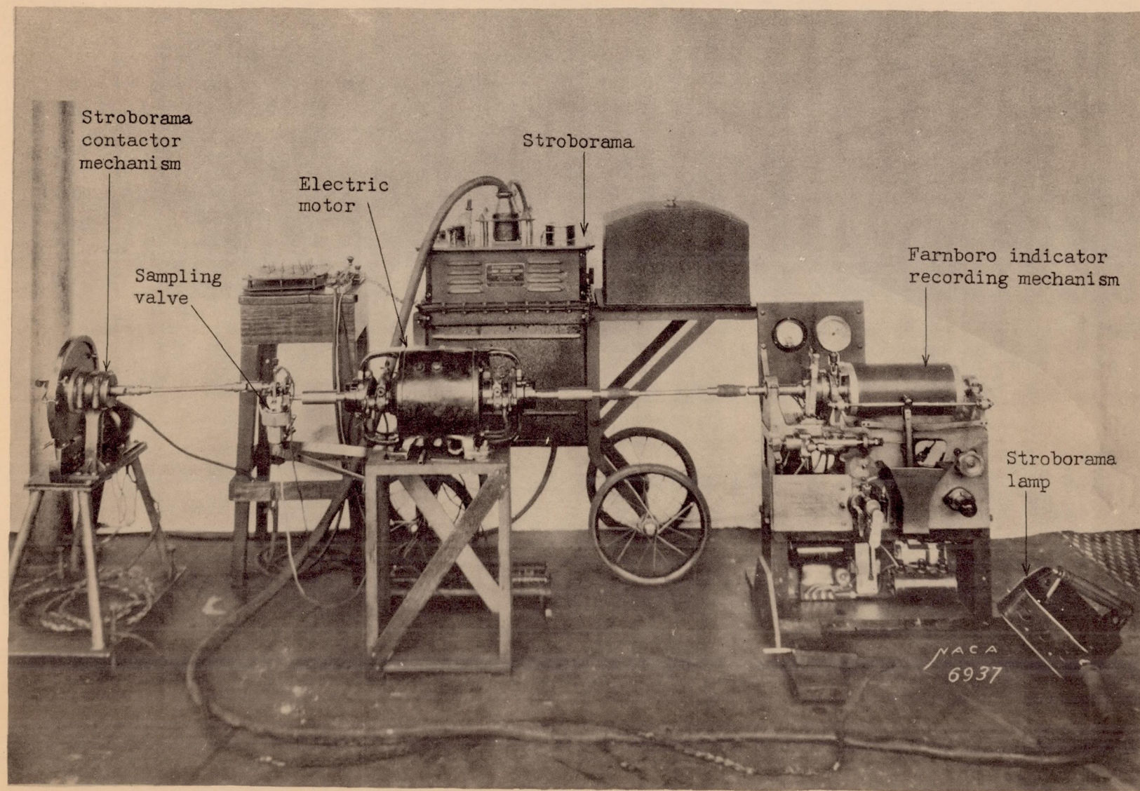
Figure 4.-Test apparatus
