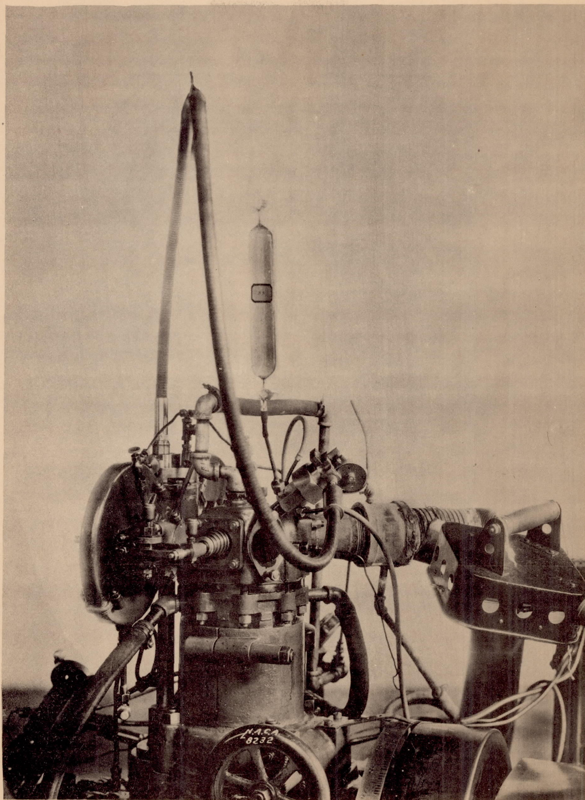
Figure 5.-Engine installation of N.A.C.A. gas-sampling valve.
