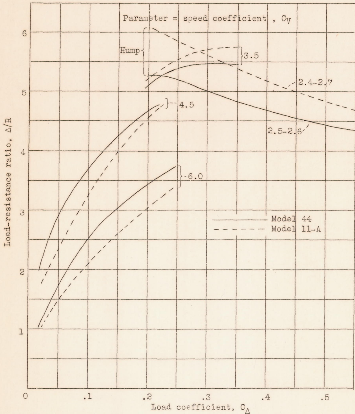
Figure 16.- Comparison of load-resistance ratios of Models 44 and 11-A at best trim angle.
