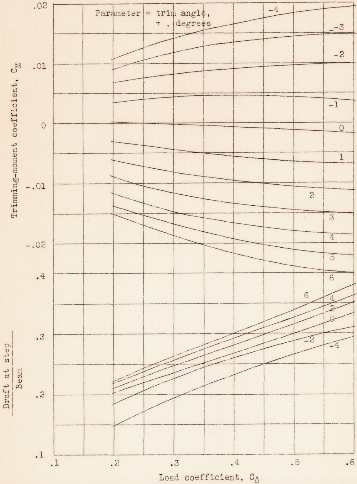
Figure 11.- Trimming-moment coefficient and draft-beam ratio at rest. Model 44.
