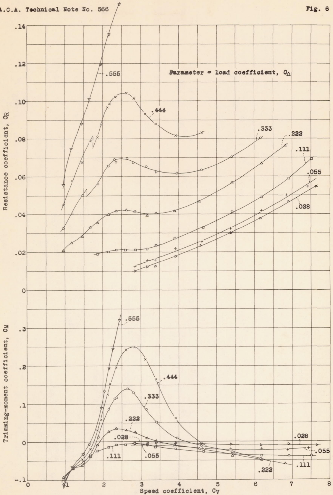
Figure 6.- Variation of C_R and C_M with C_v . \tau = 6^\circ . Model 44.
