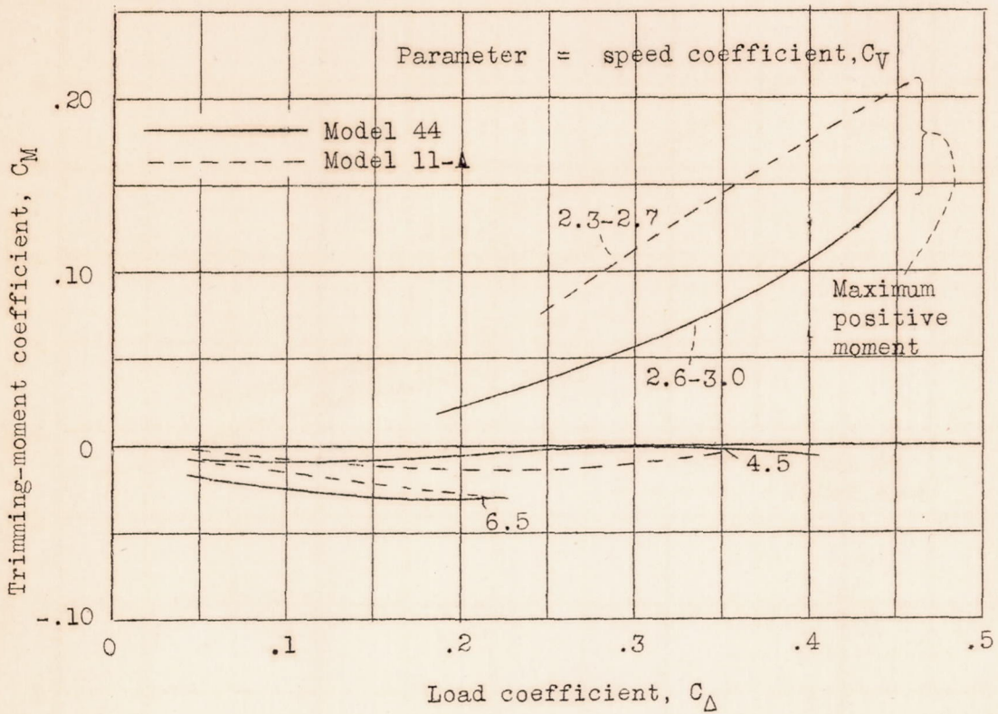
Figure 18.- Comparison of trimming-moment coefficients of Models 44 and 11-A at best trim angle.
