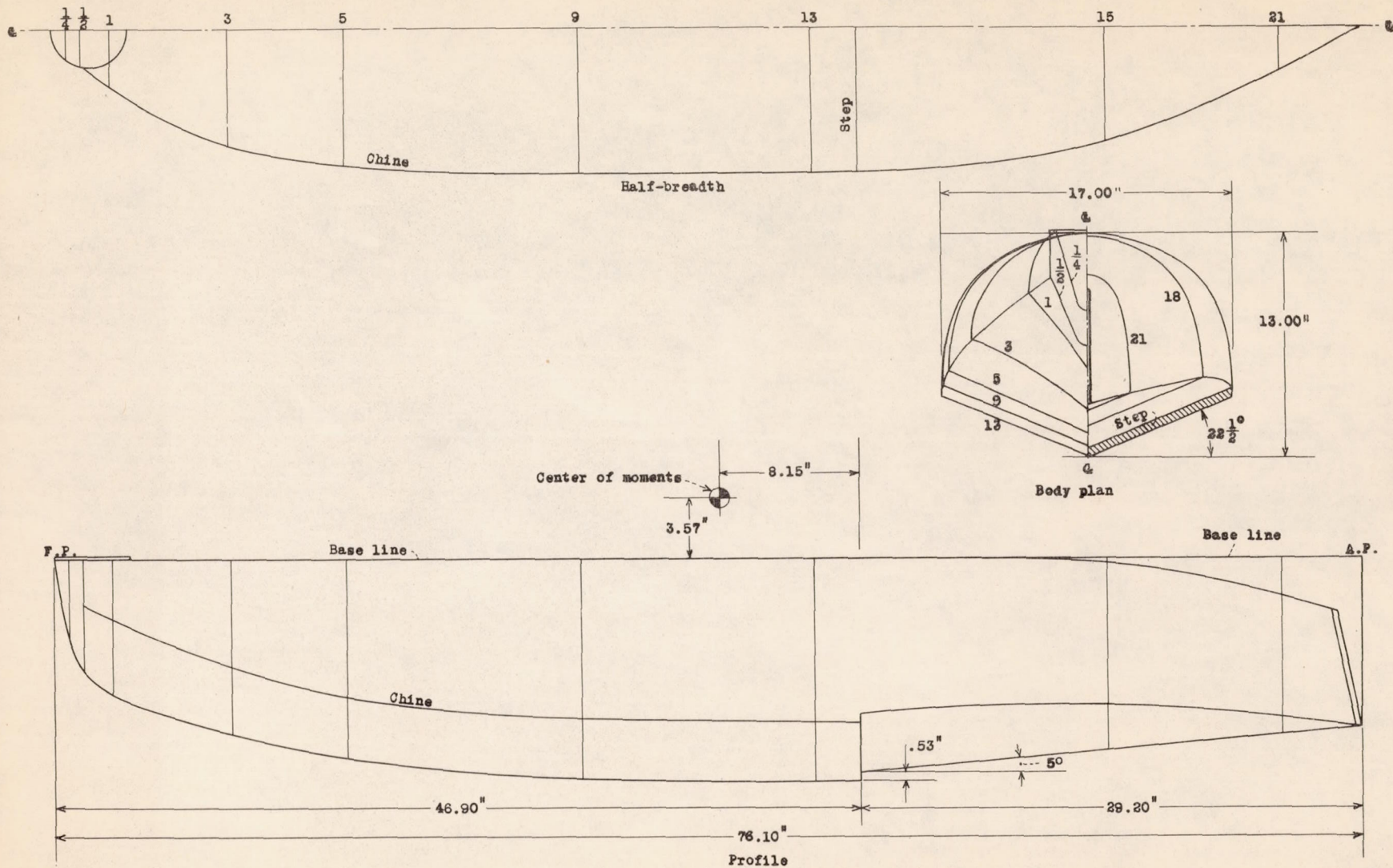
Figure 2.- Lines of N.A.C.A. Model 44 (NC hull).
