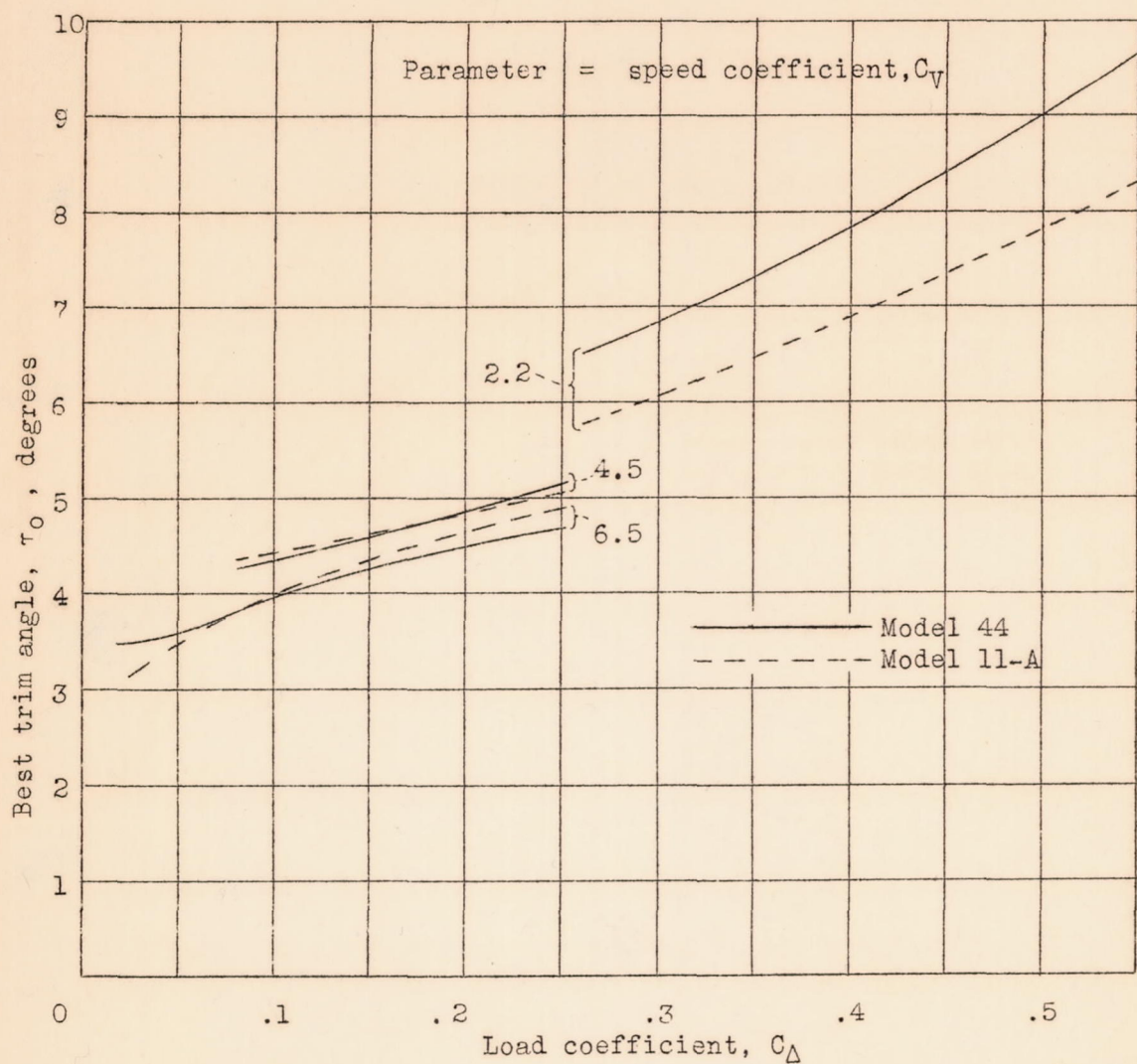
Figure 17.- Comparison of best trim angles of Models 44 and 11-A.
