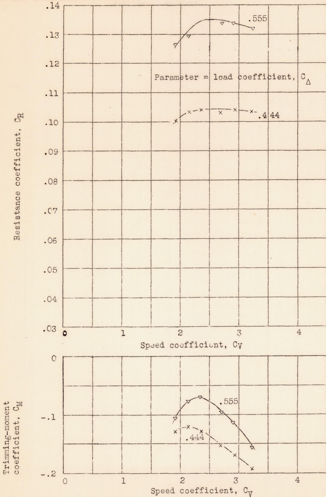
Figure 9.- Variation of C_R and C_M with C_V . \tau = 12^\circ . Model 44.
