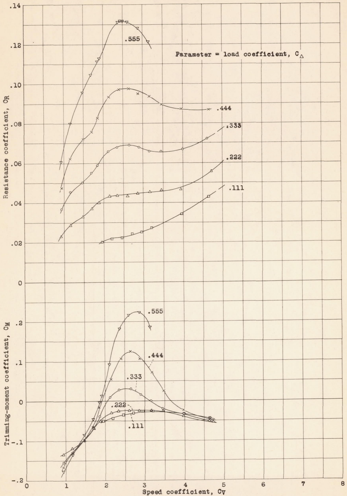
Figure 7.- Variation of C_R and C_M with C_v . \tau = 8^\circ . Model 44.
