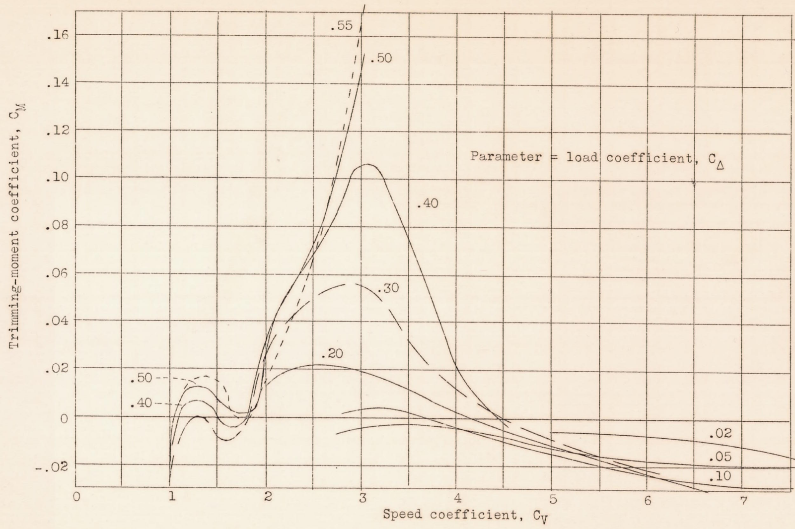
Figure 15.- Variation of C_M with C_V at best trim angle. Model 44.
