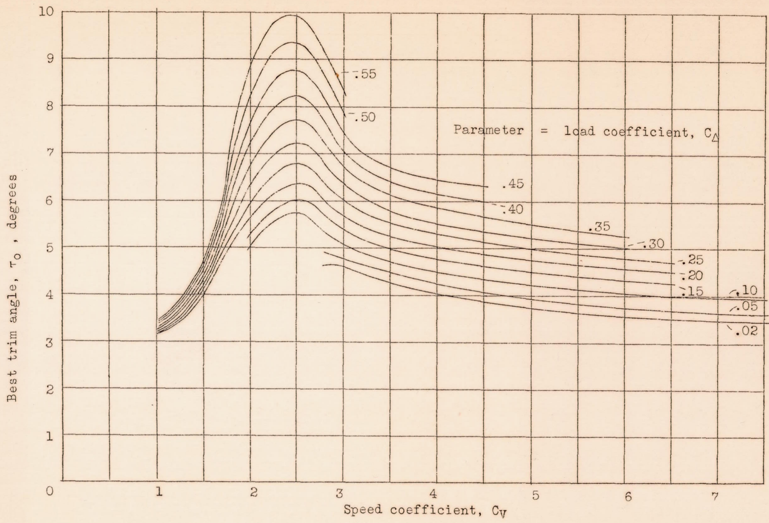
Figure 14.- Variation of \tau_0 with C_v . Model 44.
