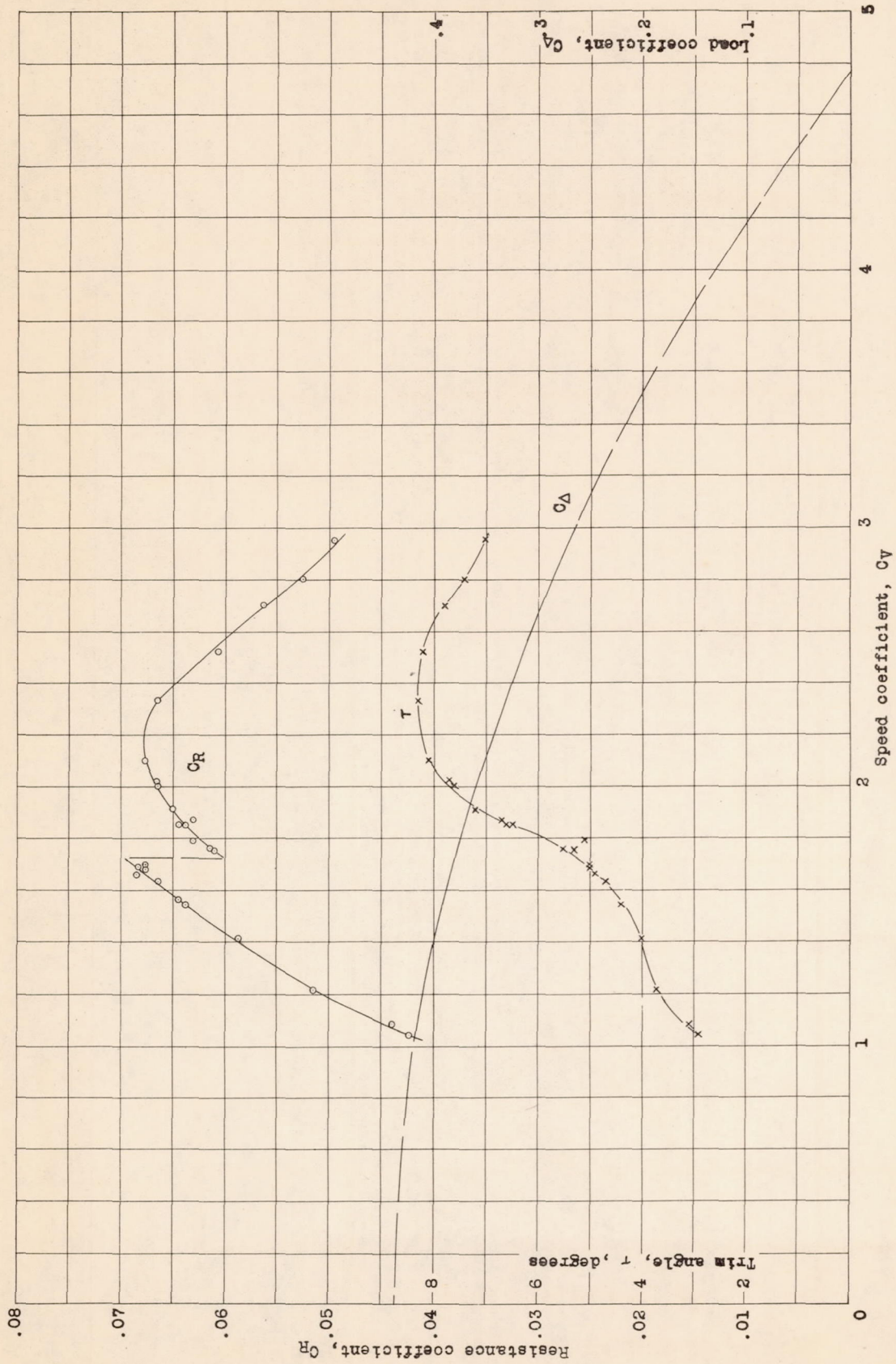
Figure 10.- Free-to-trim test results. Model 44
