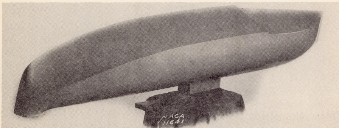
Figure 3.- N.A.C.A. model 44
