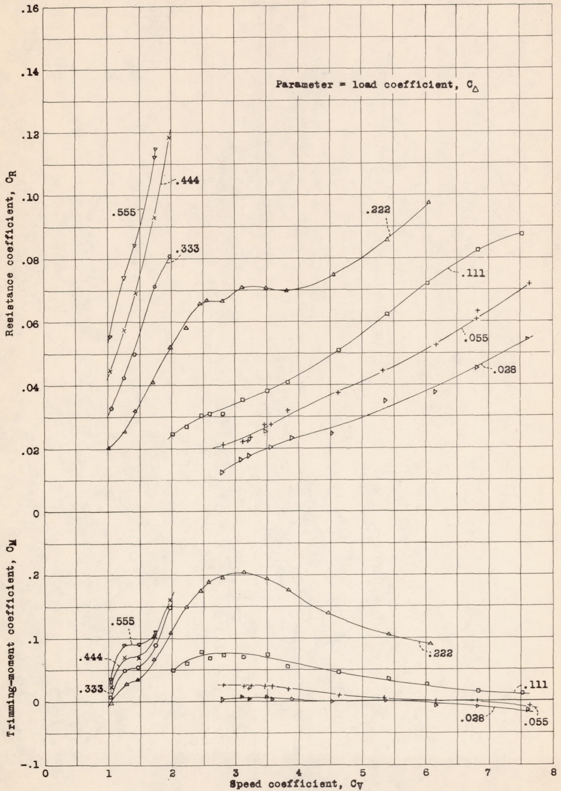
Figure 4.- Variation of C_R and C_M with C_v . \tau = 2^\circ . Model 44.
