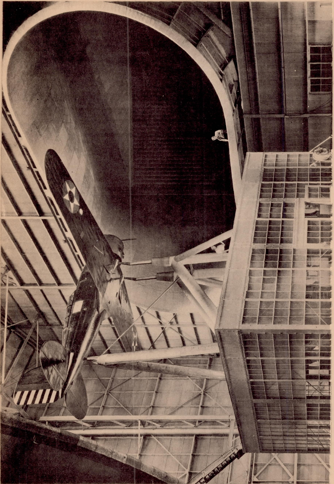
Figure 1.-Lockheed Altair ready for tests in the full-scale wind tunnel.
