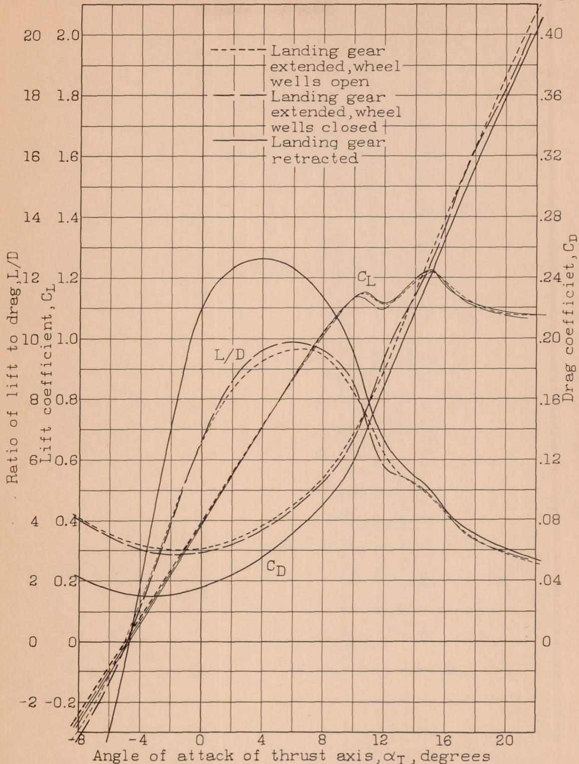
Figure 3.-Lift and drag characteristics of Lockheed Altair with landing gear both extended and retracted. Propeller off, stabilizer and elevator at 0° to thrust axis. Wing area = 294 sq.ft. Corrected for jet boundary.
