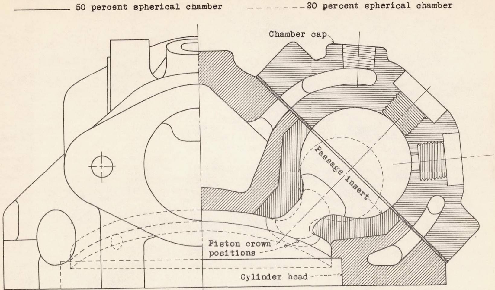
Figure 2.- Prechamber combustion chamber.
