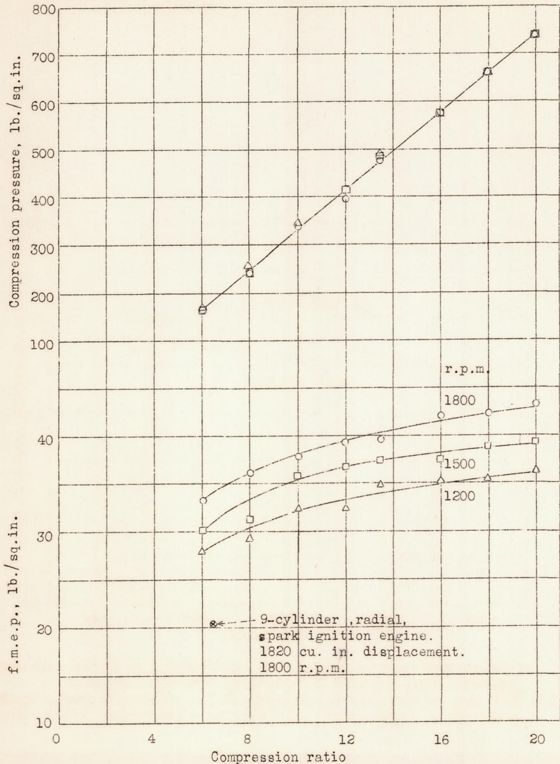
Figure 11.- Effect of compression ratio on f.m.e.p. and compression pressure. Test unit 1, prechamber cylinder head, integral chamber; oil temperature - out, 180° F.; water temperature - out, 180° F.
