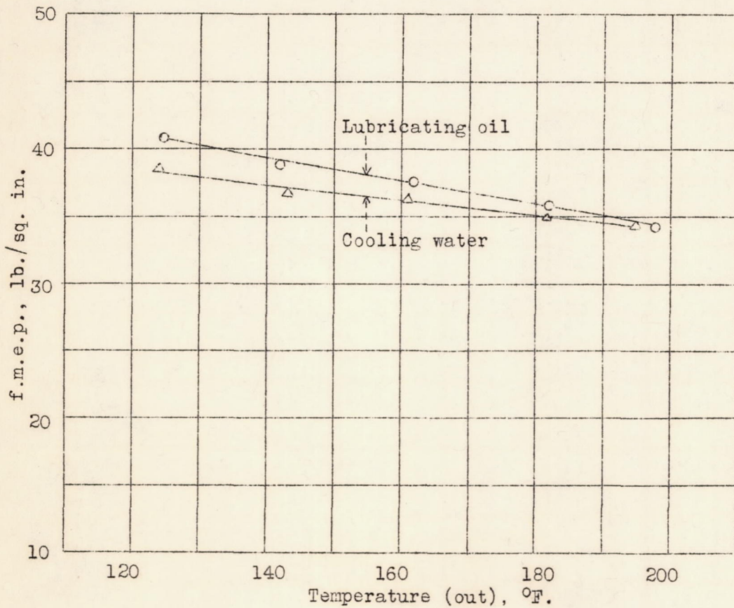
Figure 10.- Effect of lubricating oil and cooling-water temperature on f.m.e.p. Test unit 1; prechamber cylinder head, integral chamber; compression ratio, 13.5; standard oil temperature- out, 180° F.; standard water temperature - out, 170° F., engine speed, 1,500 r.p.m.
