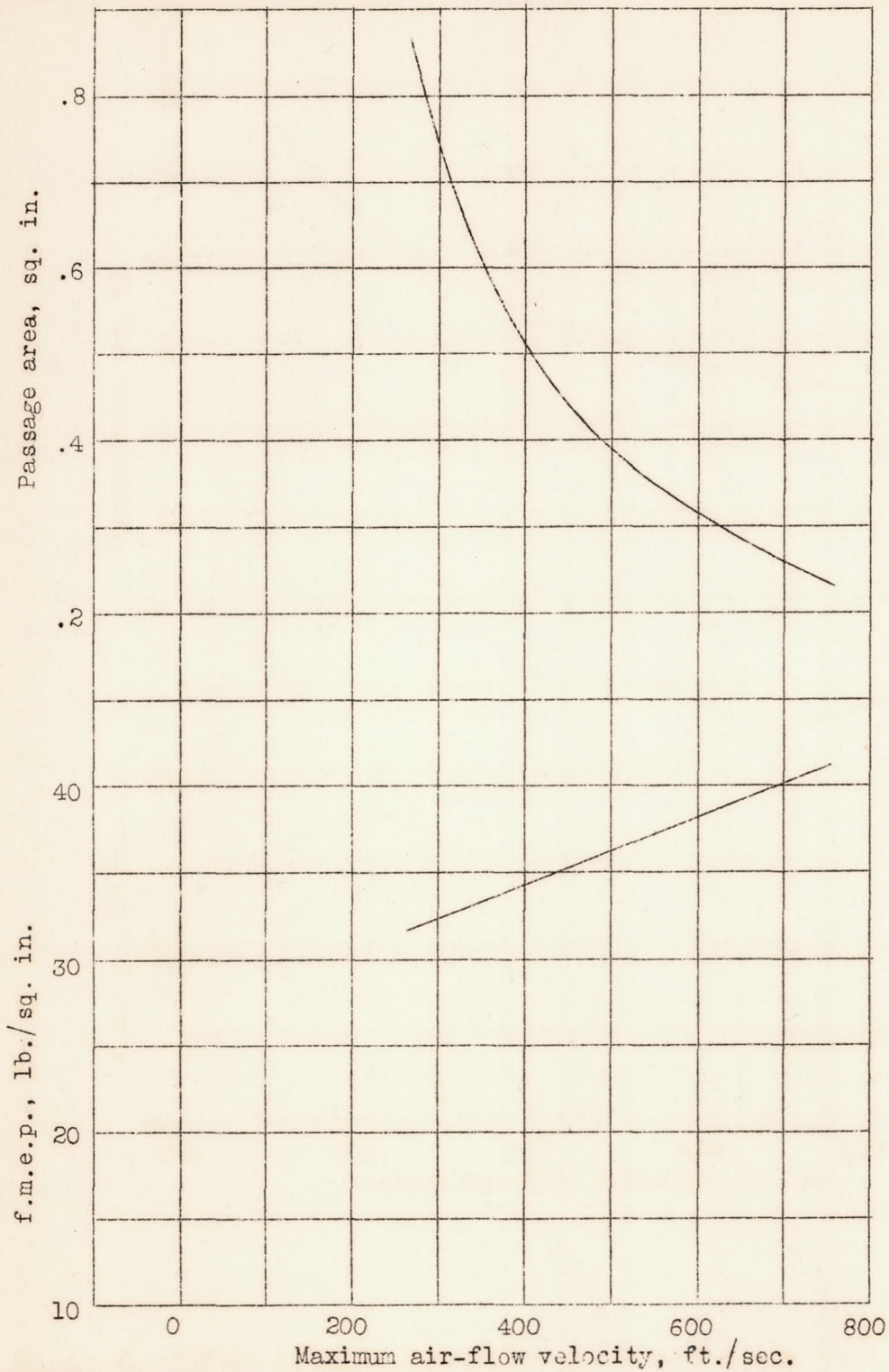
Figure 7.- Effect of maximum air-flow speed on f.m.e.p. Test unit 2; displacer combustion chamber; compression ratio, 15.3; oil temperature - out, 165° F.; water temperature - out, 170° F.; engine speed, 1,500 r.p.m.
