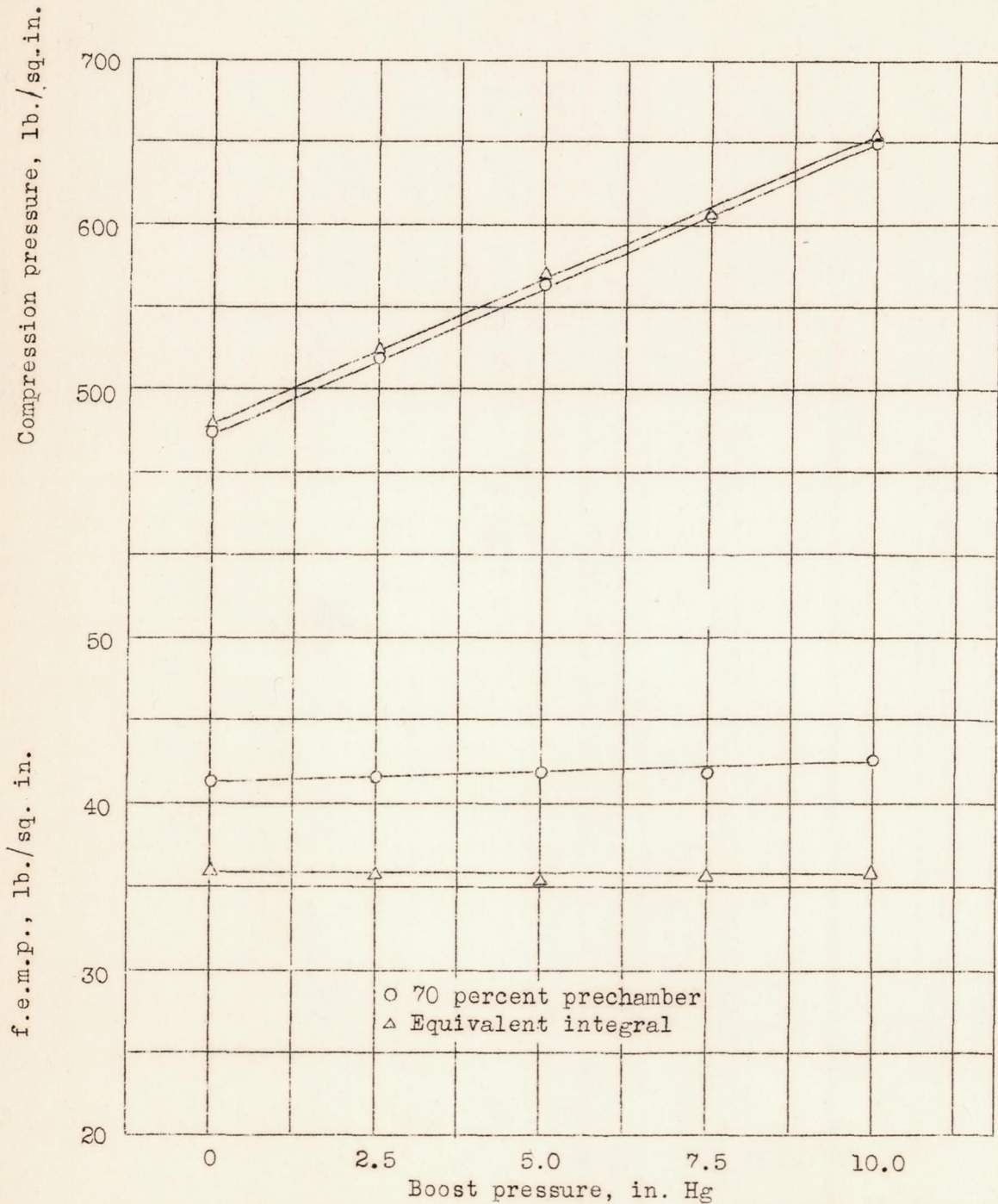
Figure 9.- Effect of boost pressure on f.m.e.p. using both integral and 70-percent chamber. Test unit 1, prechamber cylinder head; compression ratio, 13.5, oil temperature - out, 180° F., water temperature - out, 170° F., engine speed, 1,500 r.p.m.
