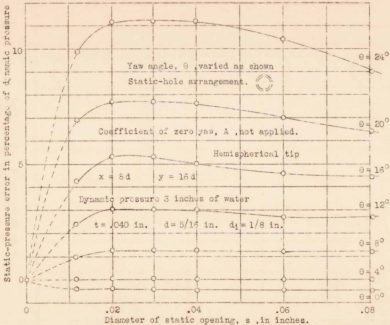
Figure 15.- Effect of size of static openings on static-pressure error.
