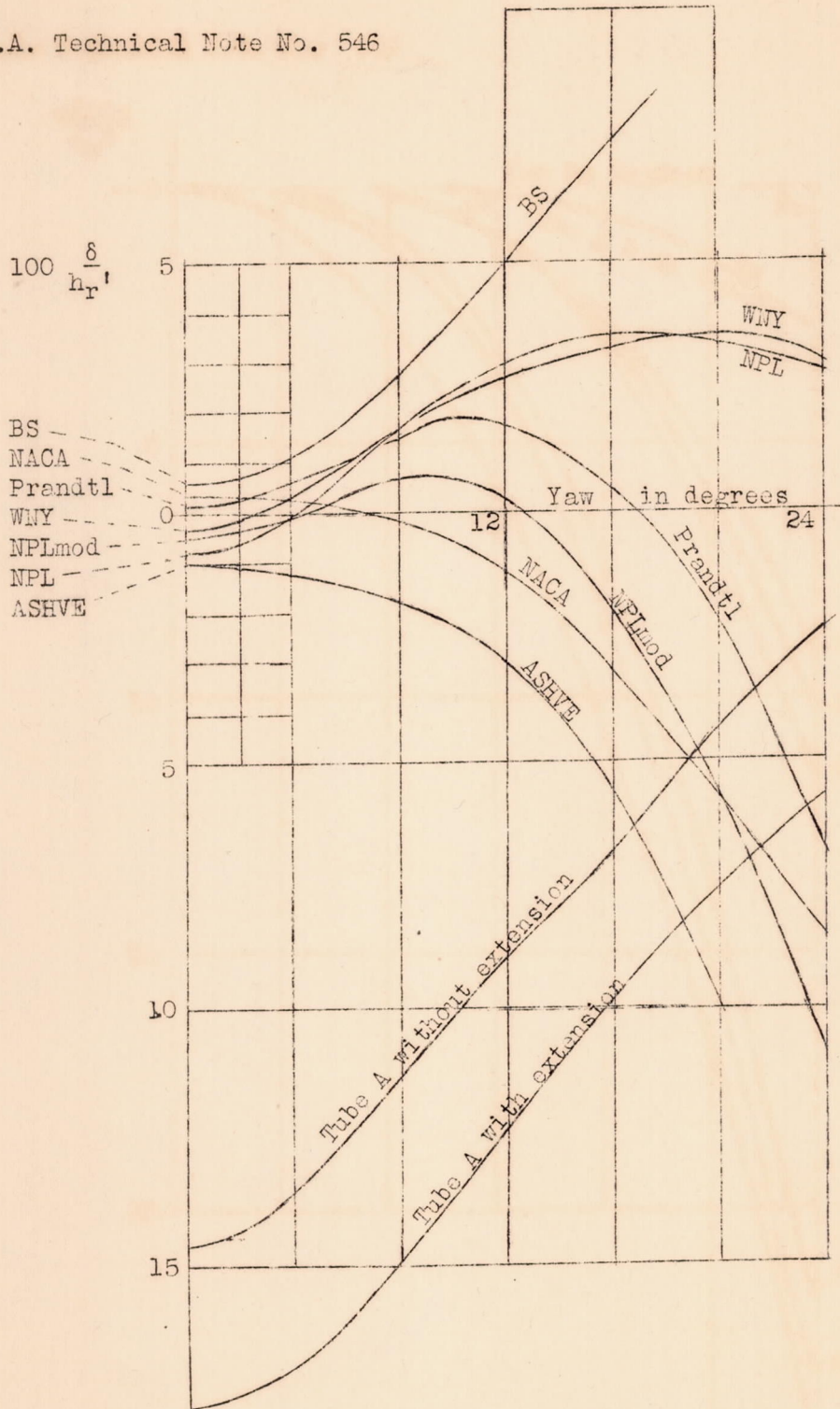
Figure 11.- Variation of resultant velocity pressure errors with yaw for eight types of pitot-static tube
