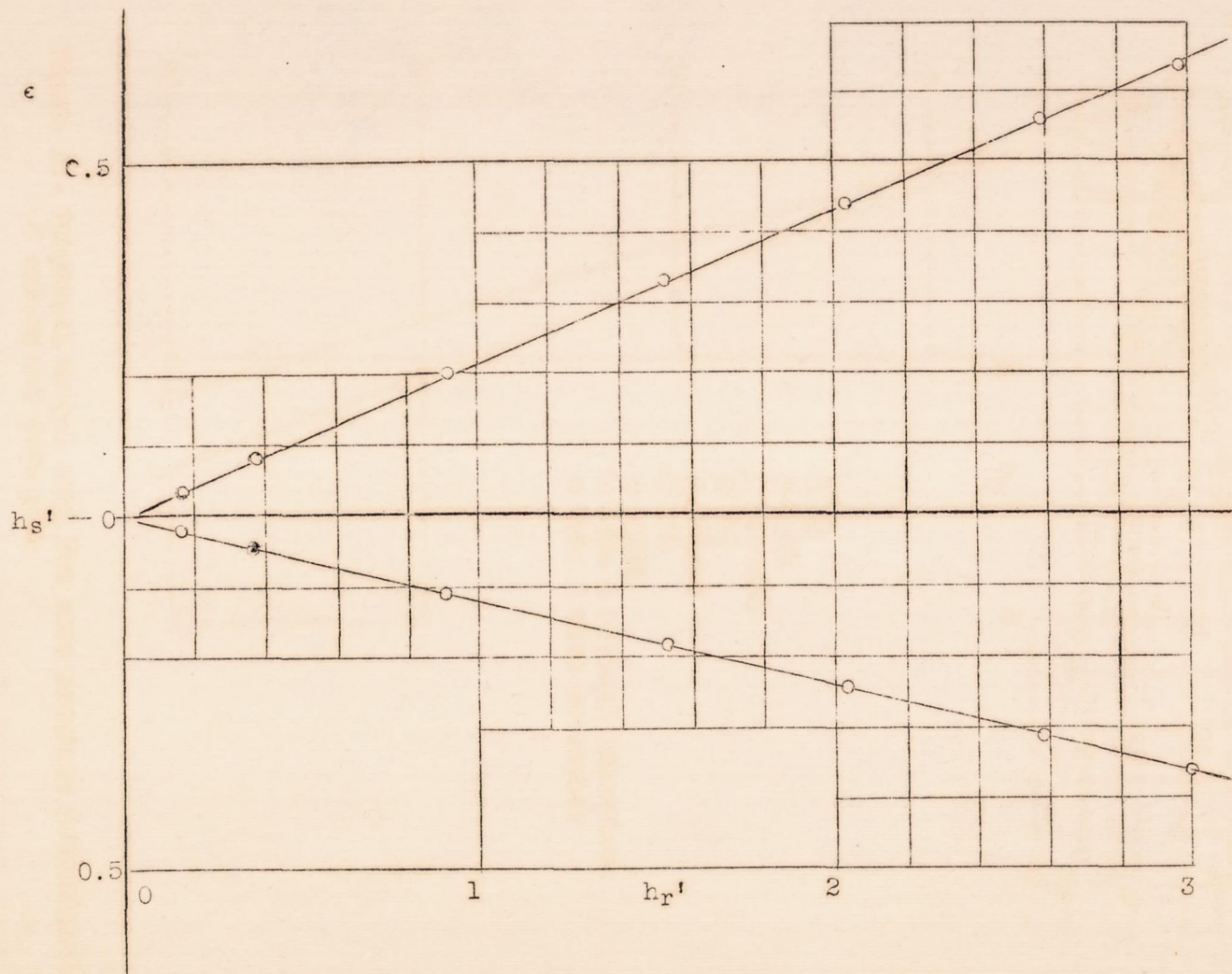
Figure 7.- Variation of \epsilon and h_s' with h_r' for NPLmod tube at about 24^\circ of yaw
