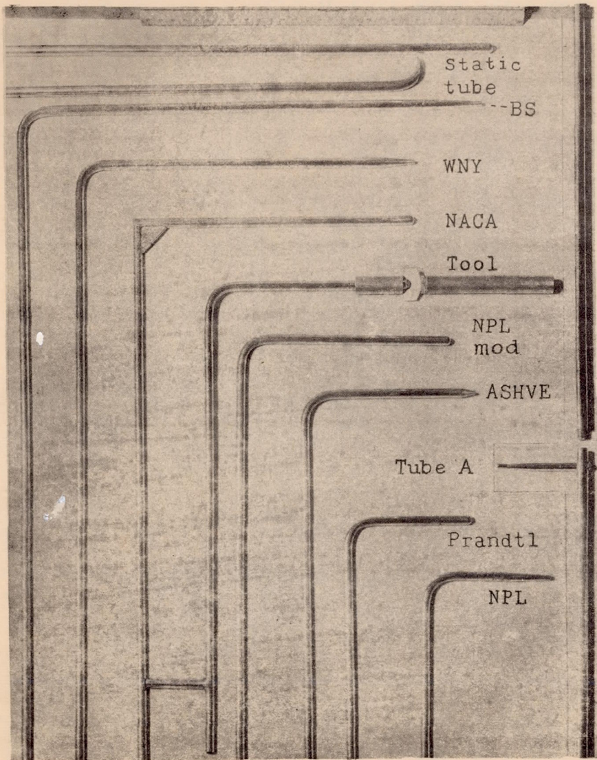
Figure 2.- Models used in investigation.
