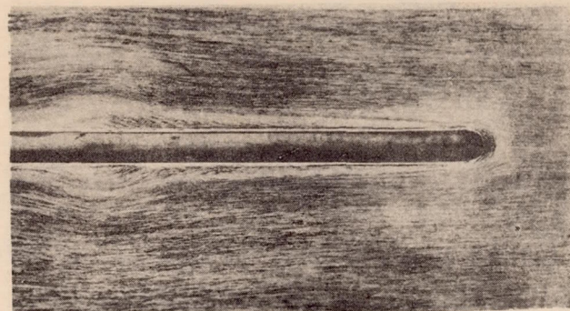
Figure 12.- Fales record for flow by a head with hemispherical tip and with a stem (in position shown) of same diameter as that of the head.
