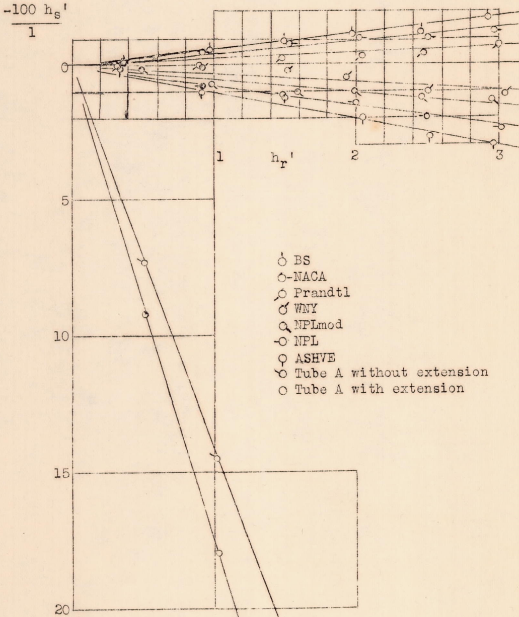
Figure 6.- Graphical method used for more accurate determination of errors for zero yaw.
