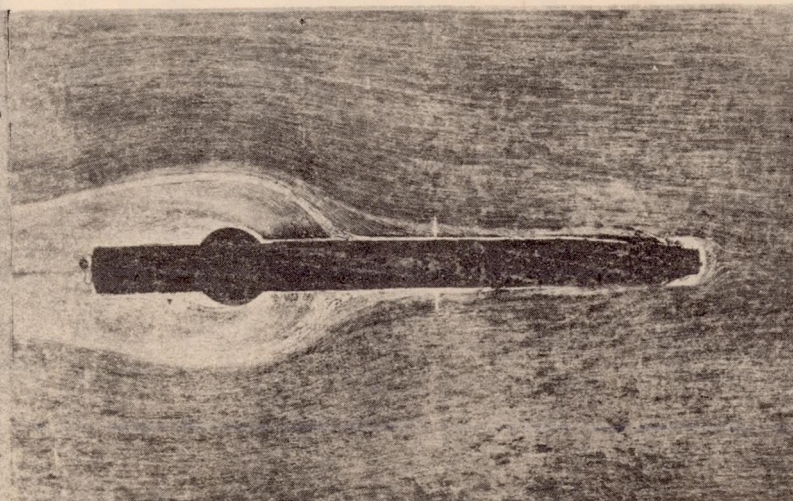
Figure 13.- Fales record for flow by a model simulating conditions in tube A.
