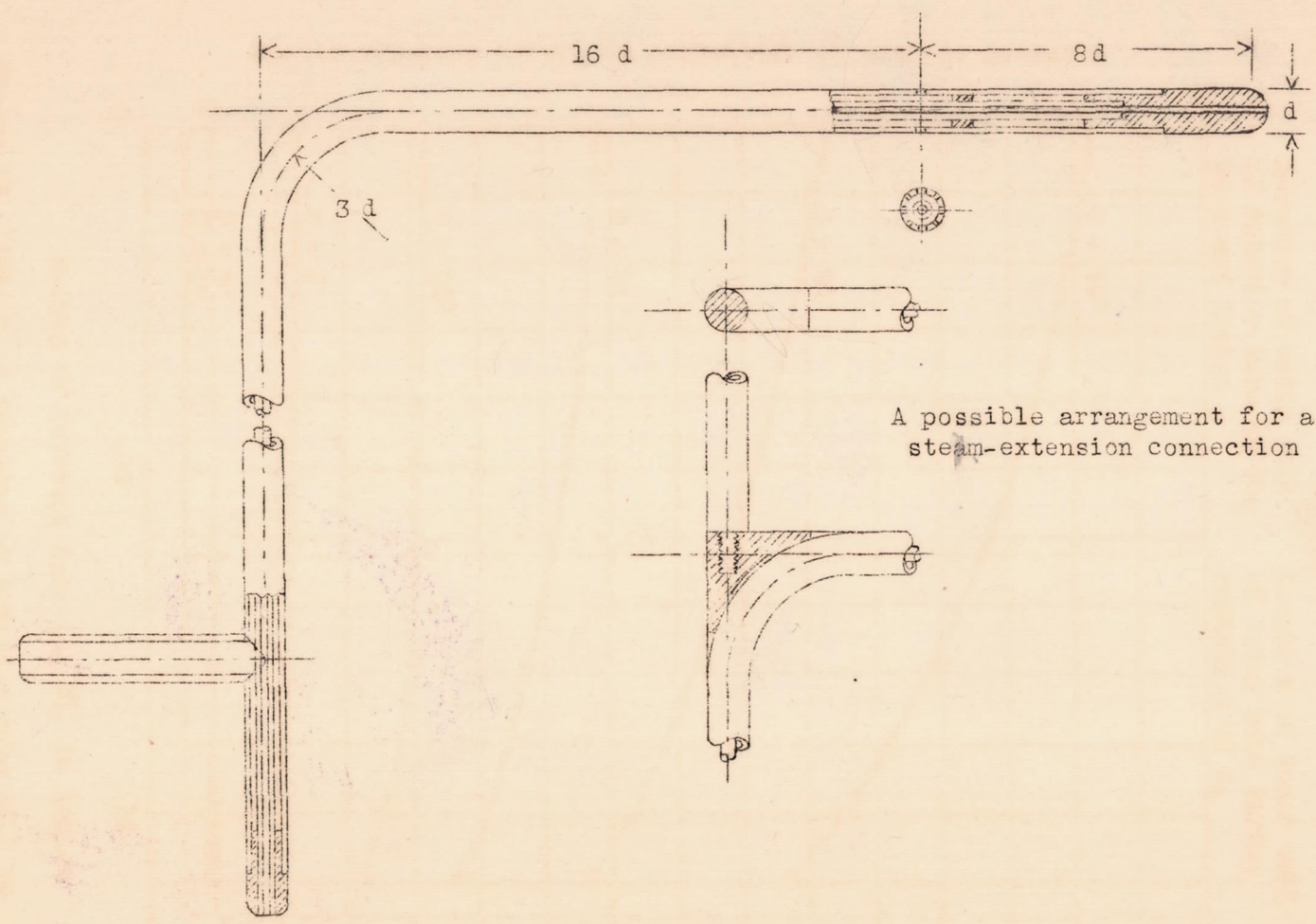
Figure 18.- Proposed tentative standard pitot-static tube.
