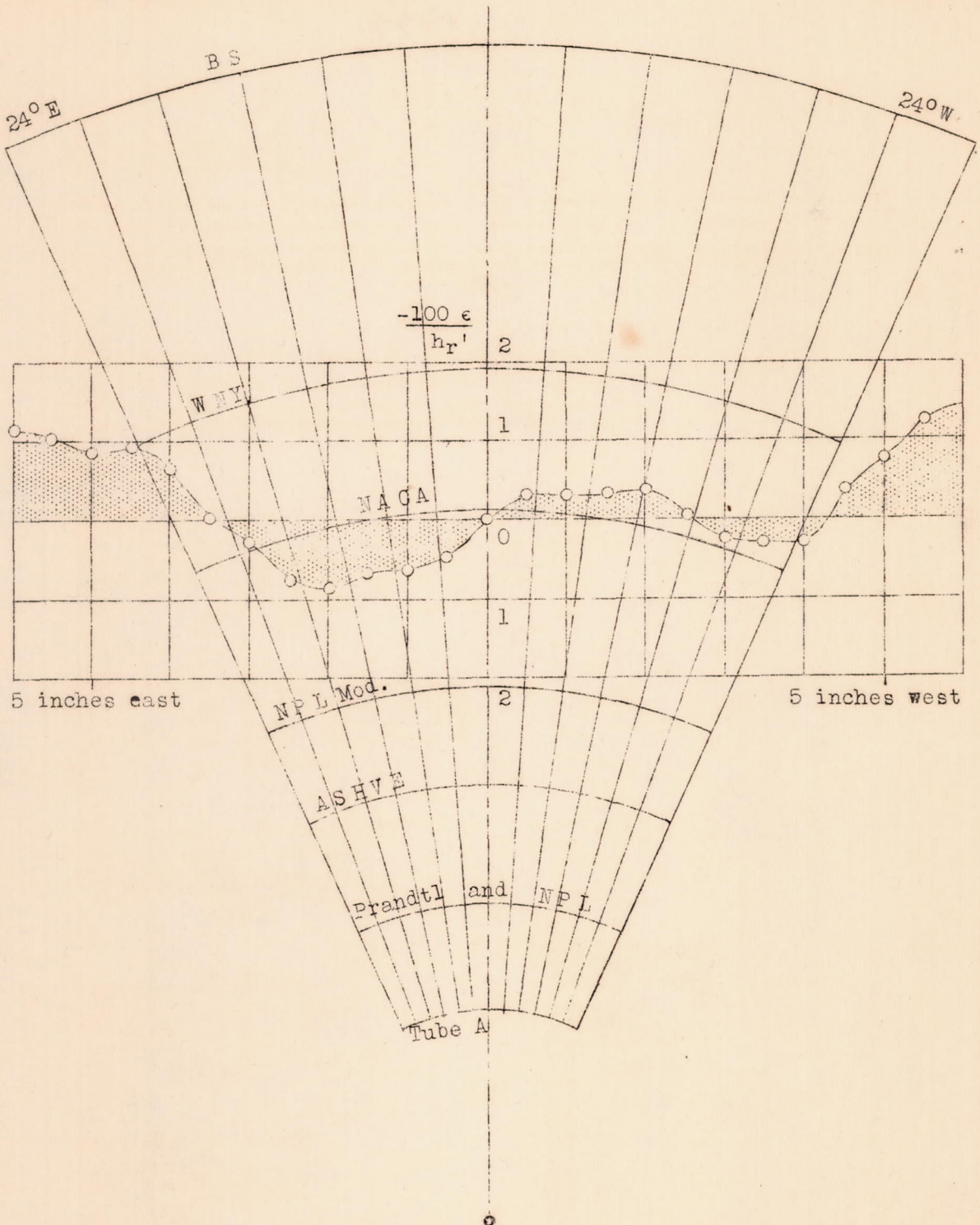
Figure 4.- Chart used in correcting for nonuniformity of air stream.
