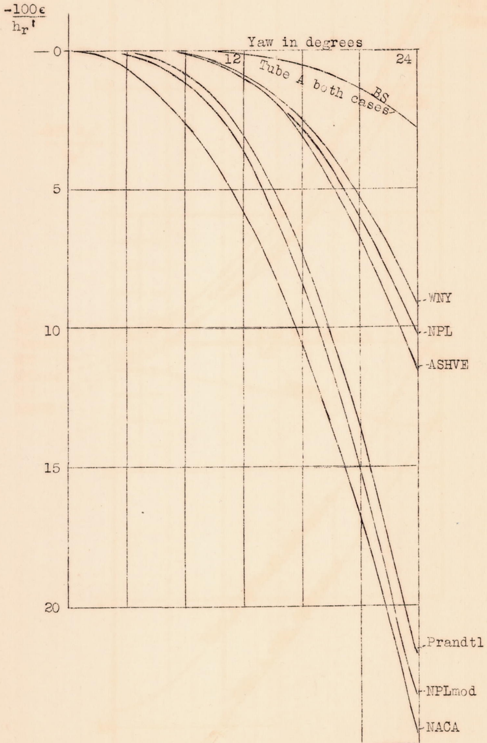
Figure 10.- Variation of impact-pressure errors with yaw for eight types of pitot-static tube.
