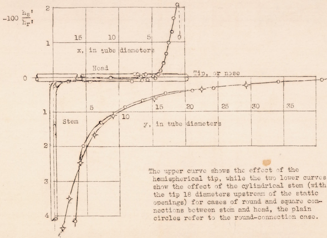
Figure 5.- Static pressure errors caused by presence of stem and tip.
