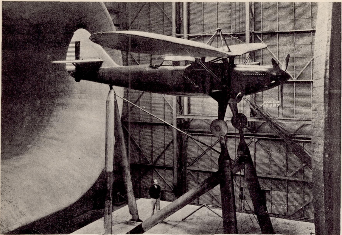
Figure 3.- YO-31A airplane with prestone radiator exposed.
