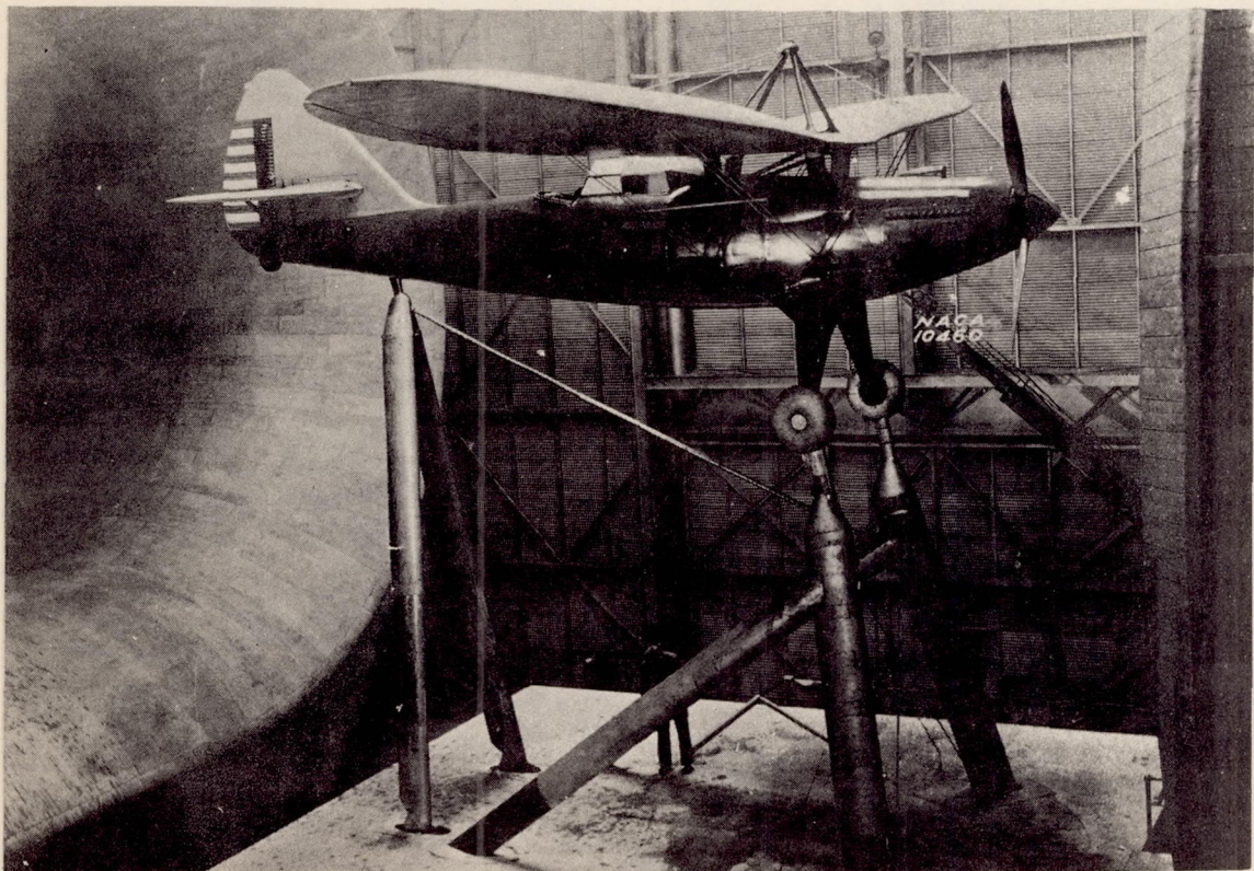
Figure 4.- YO-31A airplane with no radiators exposed.
