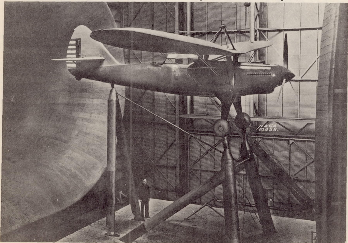
Figure 2.- YO-31A airplane with oil radiator exposed.
