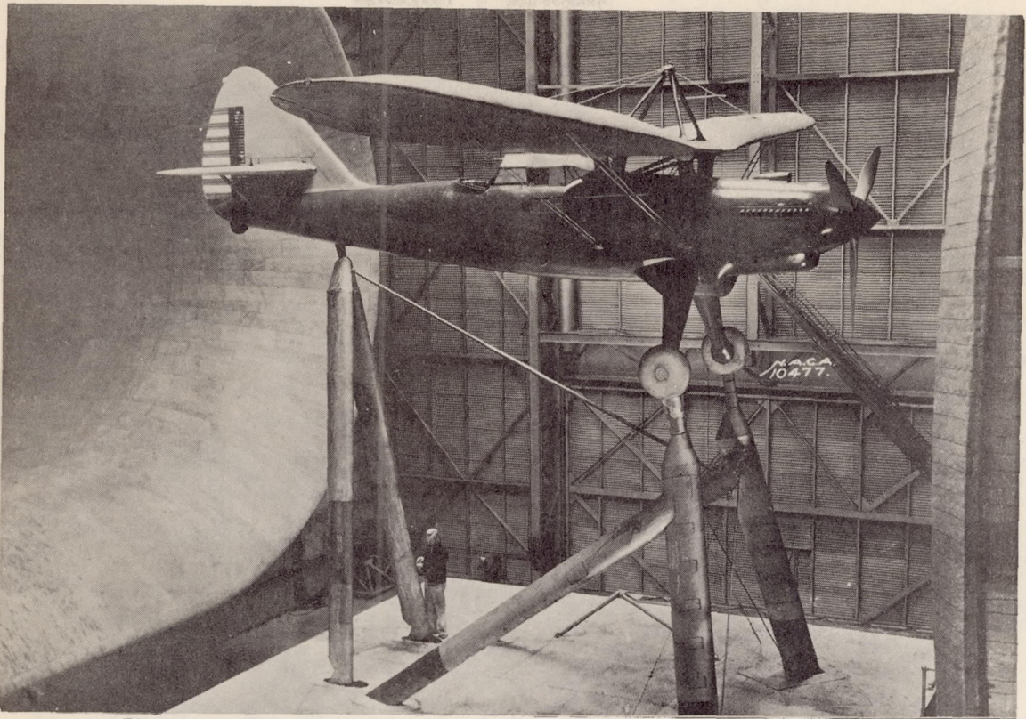
Figure 1.- YO-31A airplane with oil and prestone radiators exposed.
