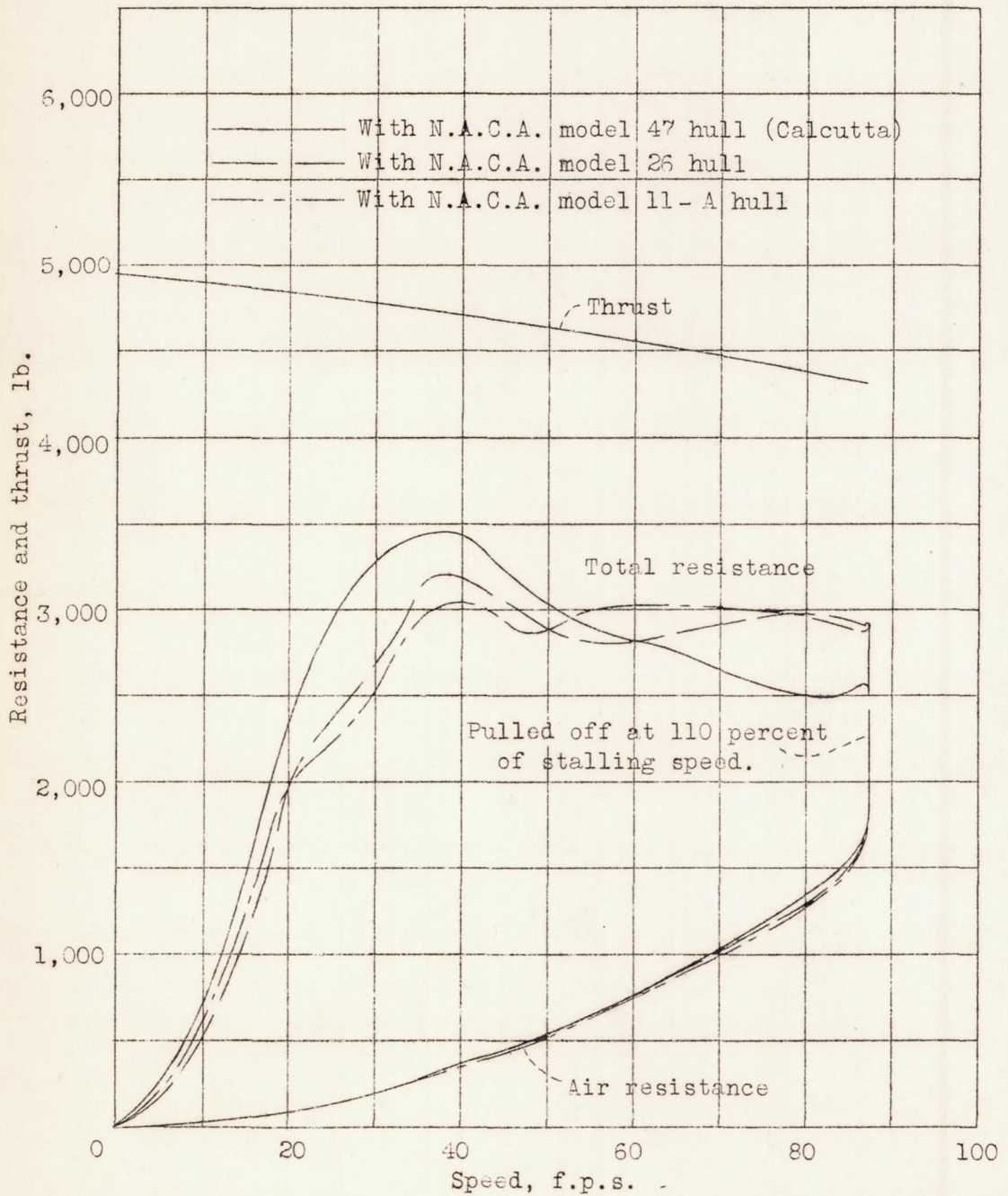
Figure 20.- Resistance and thrust for take-off with 20,000 lb. load.
