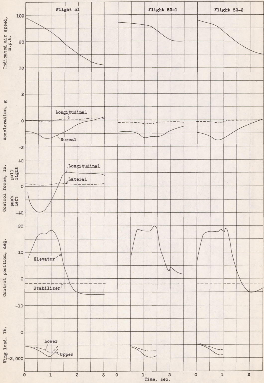
Figure 5.- Time histories of three inverted push-ups from level flight (original wings).
