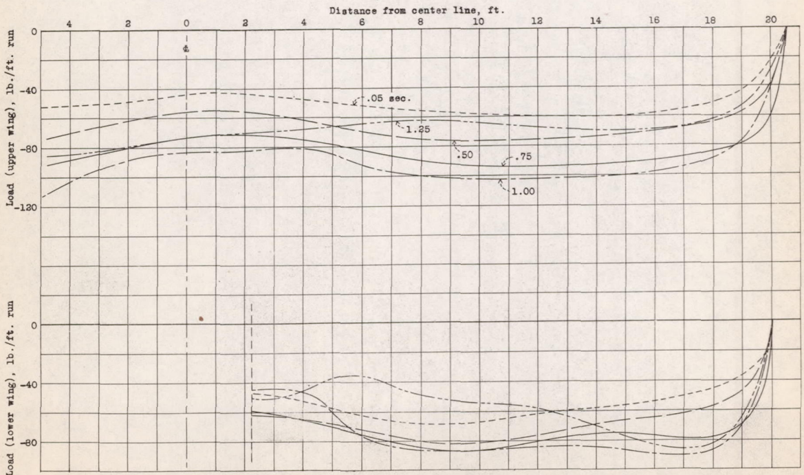
Figure 10.- Variation of load distribution during an inverted push-up (flight 51-1, original wings).
