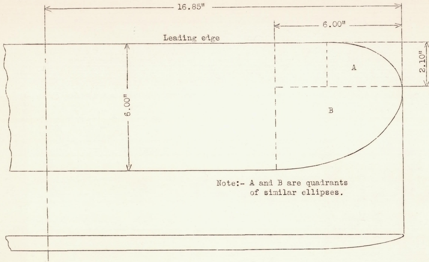
Figure 1.- The rectangular Clark Y wing with rounded tips.
