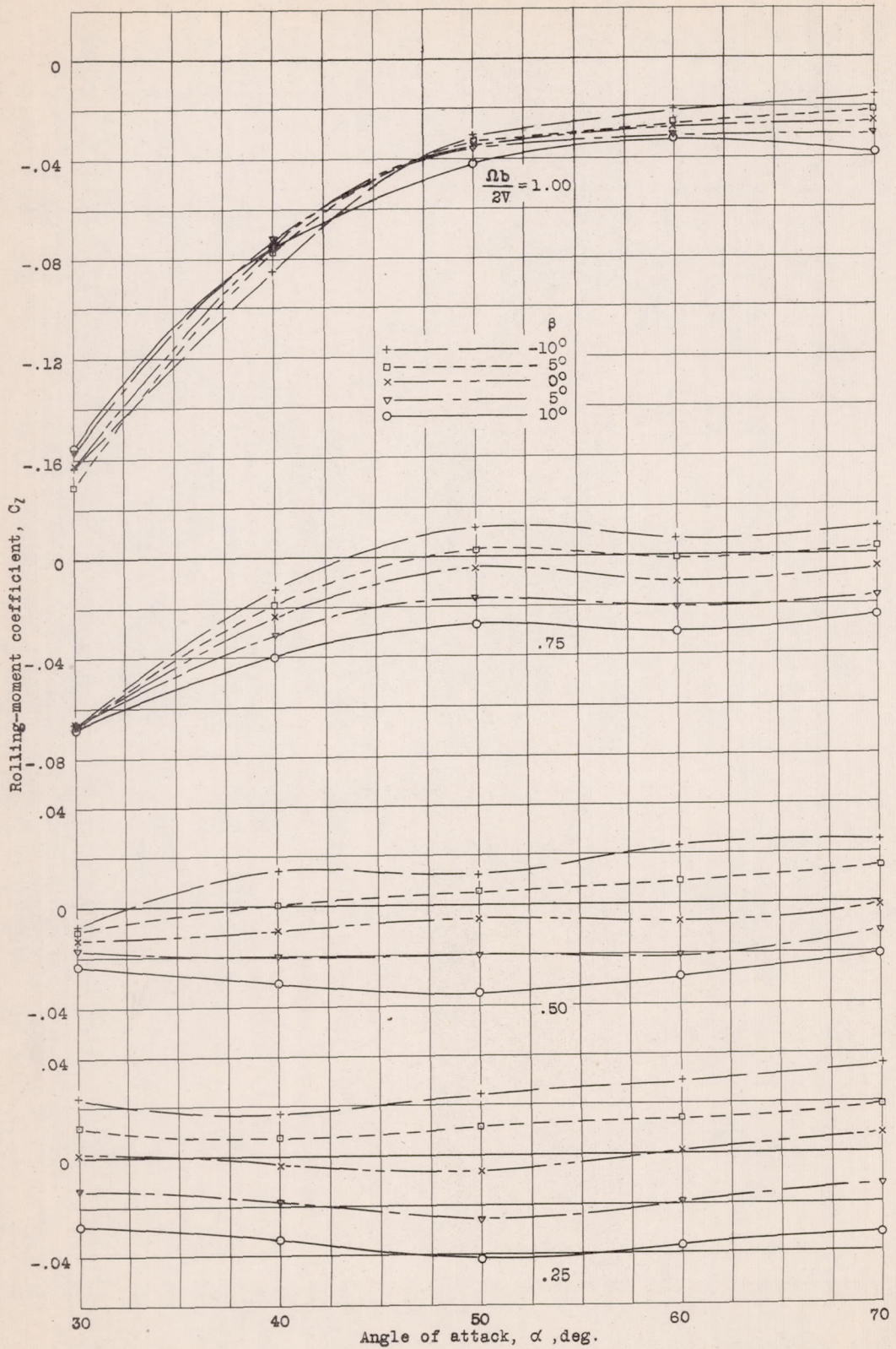
Figure 9b.- Variation of rolling-moment coefficient C_l (body axes) with angle of attack; 5:2 tapered wing, rounded tips.
