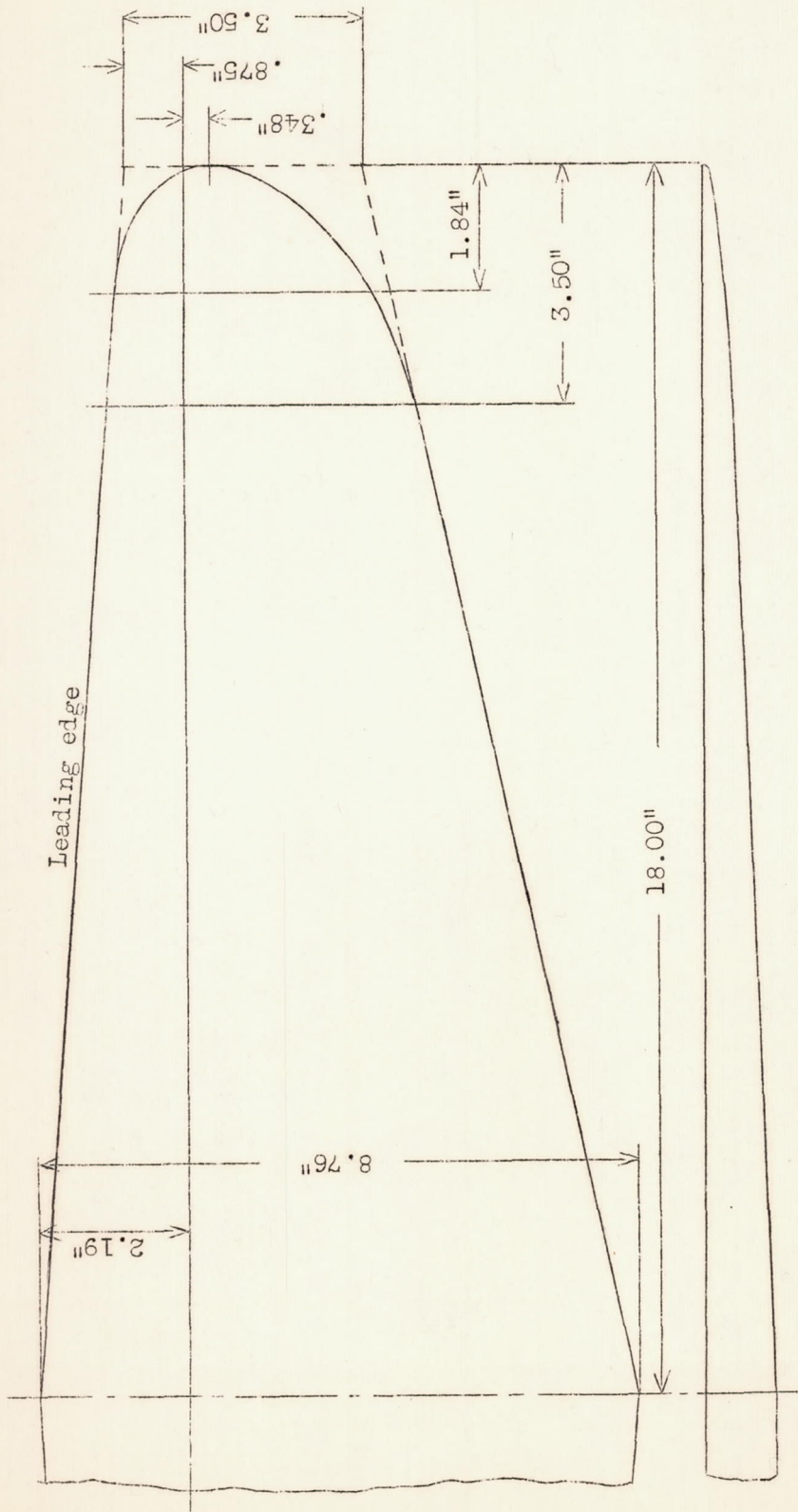
Figure 2.- The 5:2 tapered Clark Y wing with rounded tips.
