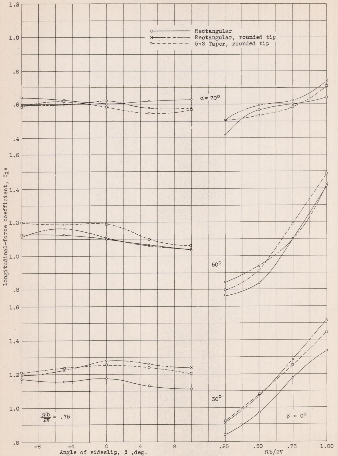
Figure 6.- Variation of longitudinal-force coefficient C_x'' (earth axes) with angle of sideslip and with \Omega b / 2V
