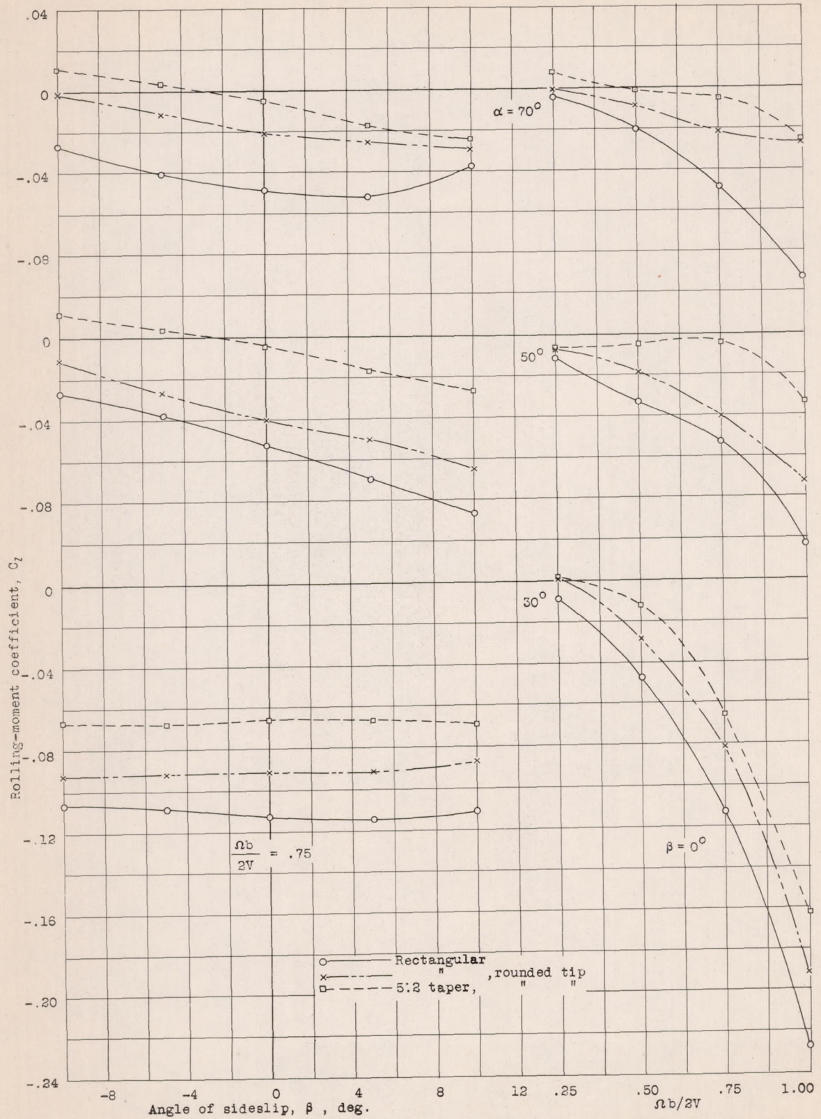
Figure 10.- Variation of rolling-moment coefficient C_z (body axes) with angle of sideslip and \Omega b / 2V .
