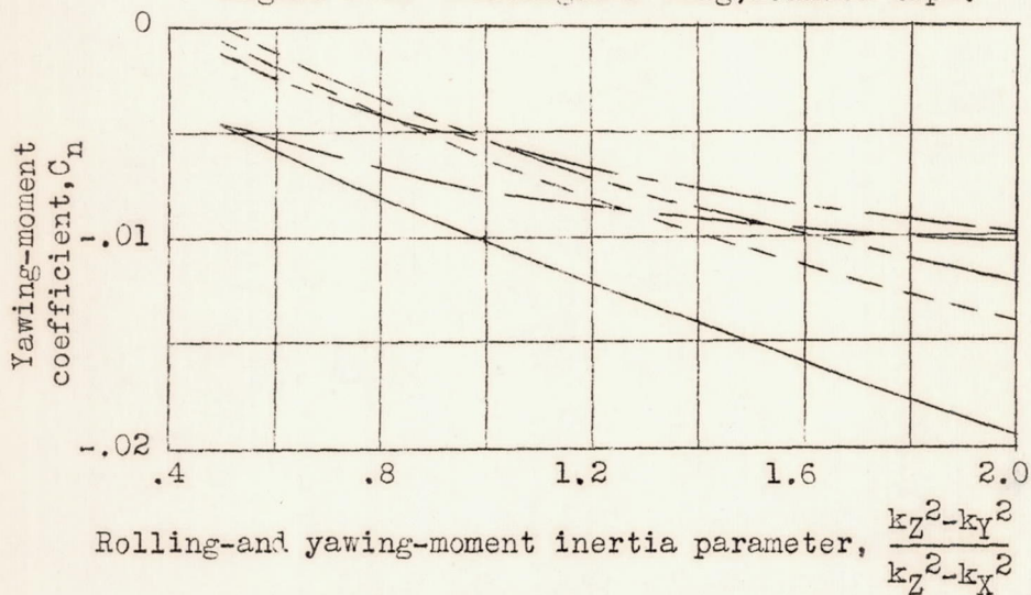
Figure 20b.- 5:2 tapered wing, rounded tips.
