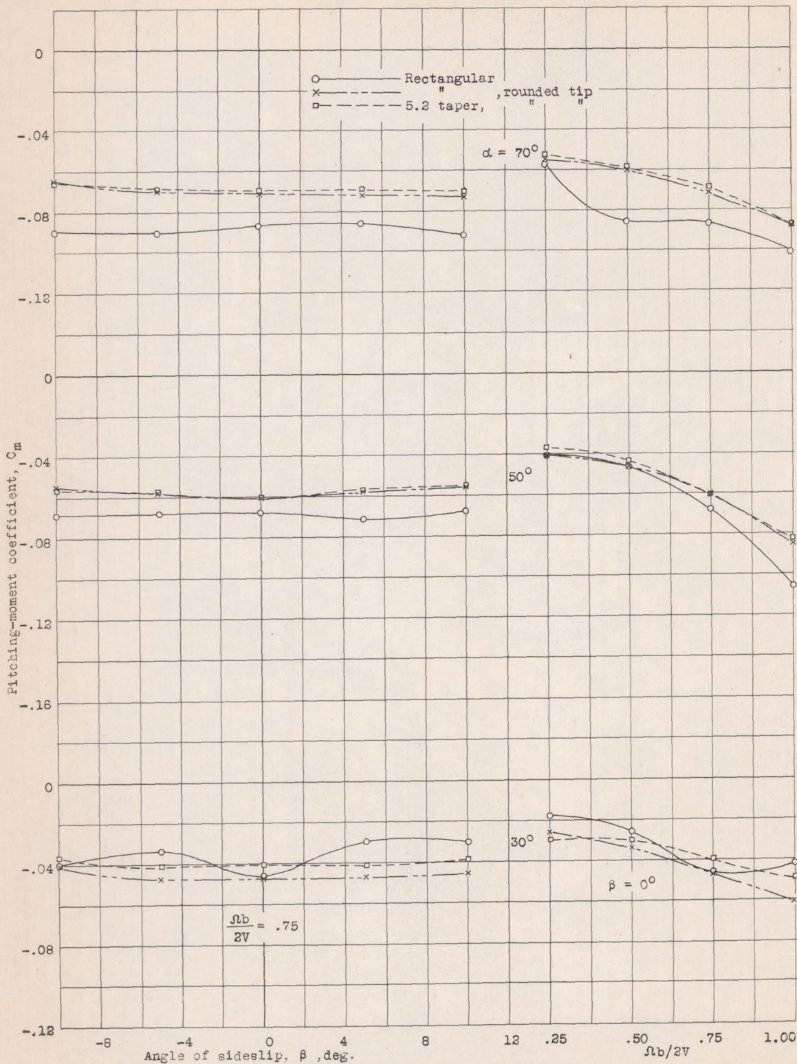
Figure 12.- Variation of pitching-moment coefficient C_m (body axes) with angle of sideslip and \Omega b/2V .
