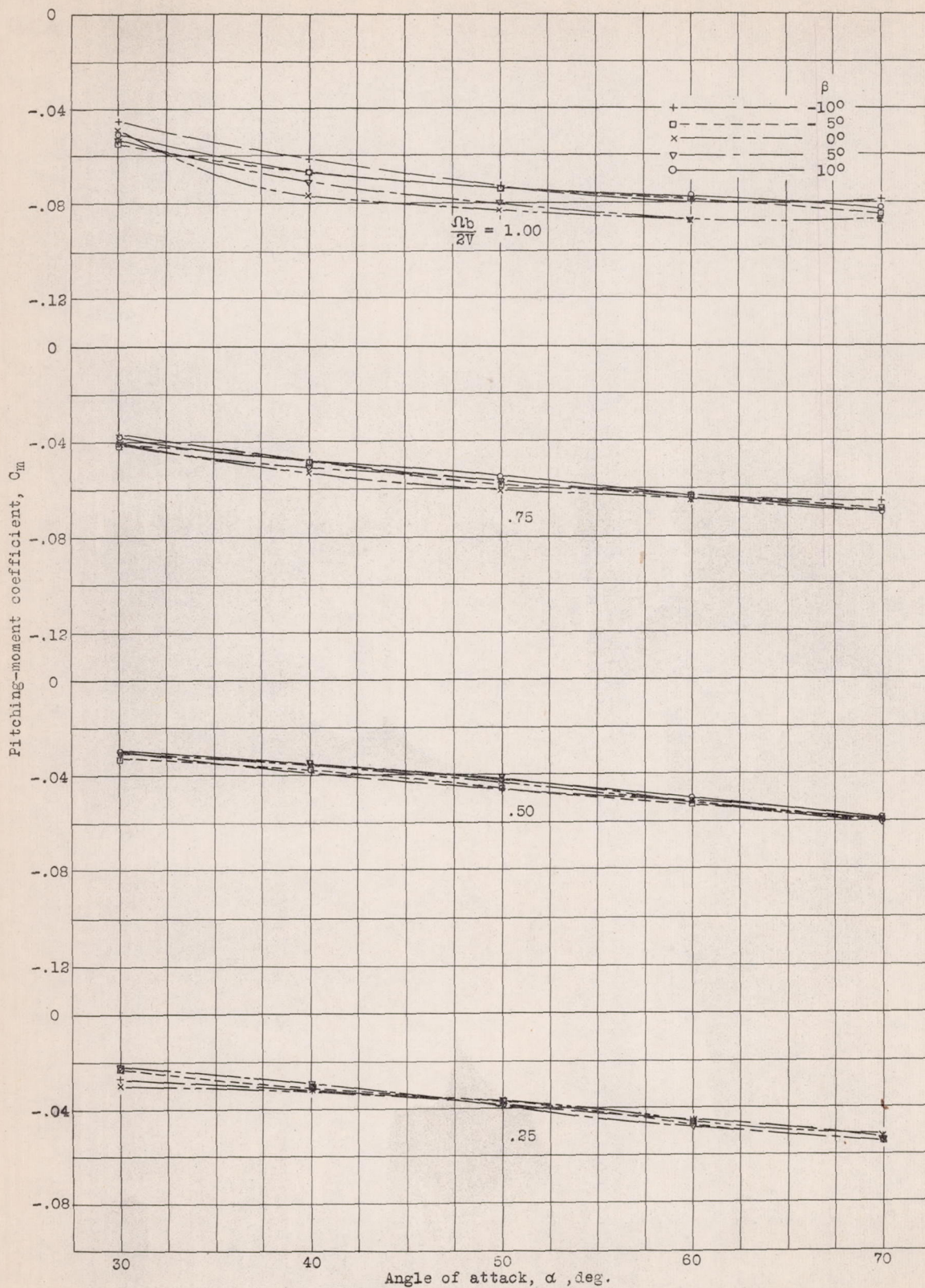
Figure 11b.- Variation of pitching-moment coefficient C_m (body axes) with angle of attack; 5:2 tapered wing; rounded tip.
