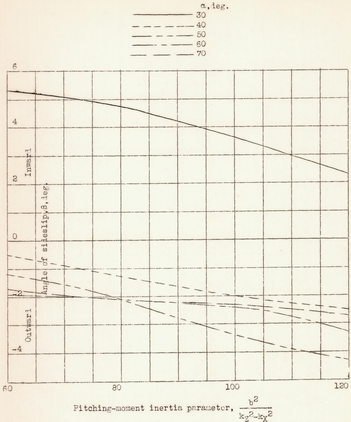
Figure 17a.- Effect of pitching-moment inertia parameter upon sideslip necessary for equilibrium in a spin; rectangular wing, rounded tips.
