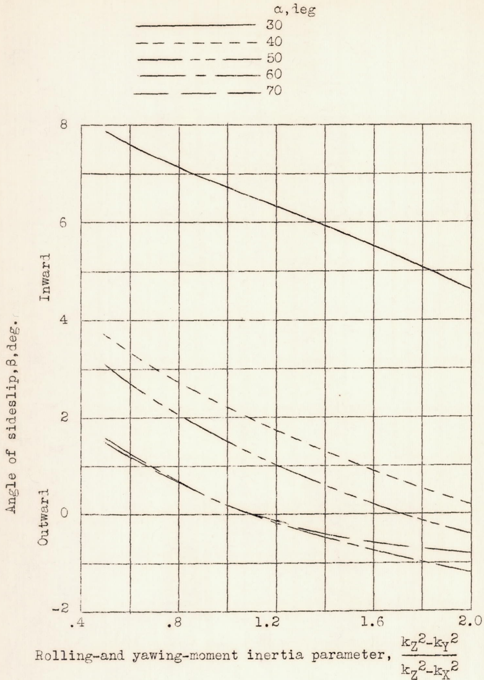
Figure 19b.- Effect of rolling and yawing moment inertia parameter upon sideslip necessary for equilibrium in a spin; 5:2 tapered wing, rounded tips.
