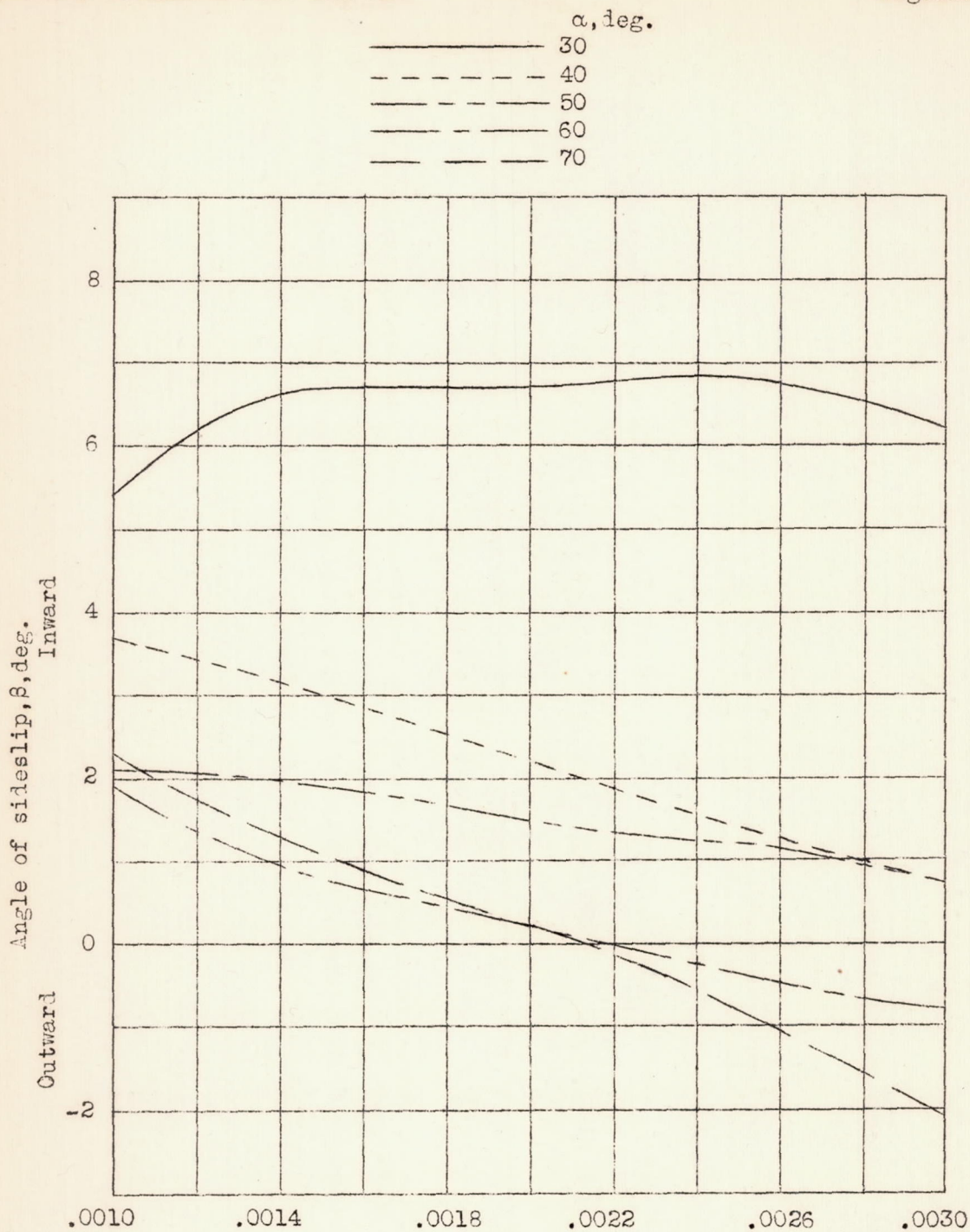
Figure 15b.- Effect of pitching-moment coefficient upon sideslip necessary for equilibrium in a spin; 5:2 tapered wing, rounded tips.
