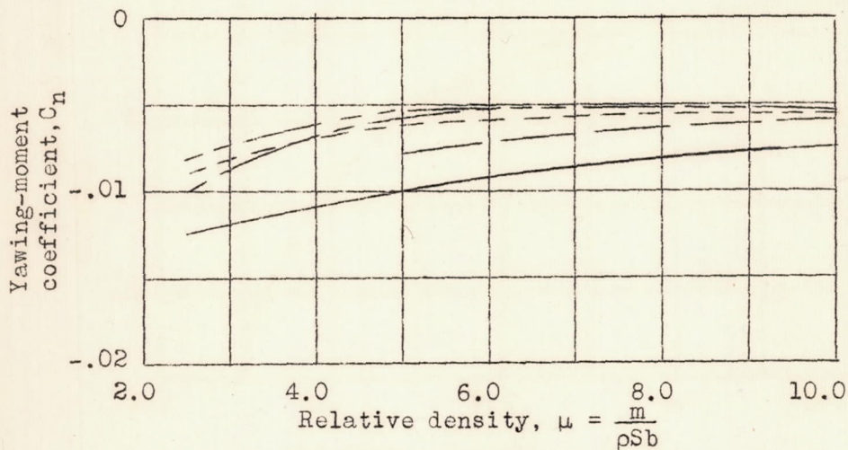
Figure 22b.- 5:2 tapered wing, rounded tips.
