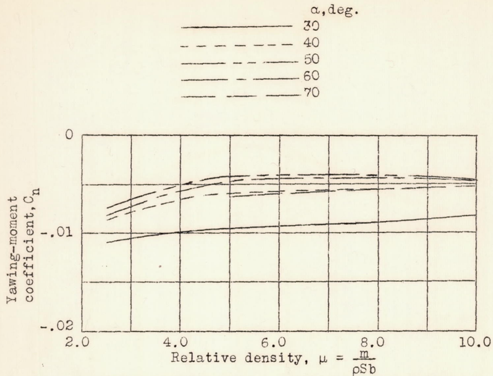
Figure 22a.- Rectangular wing, rounded tips.
