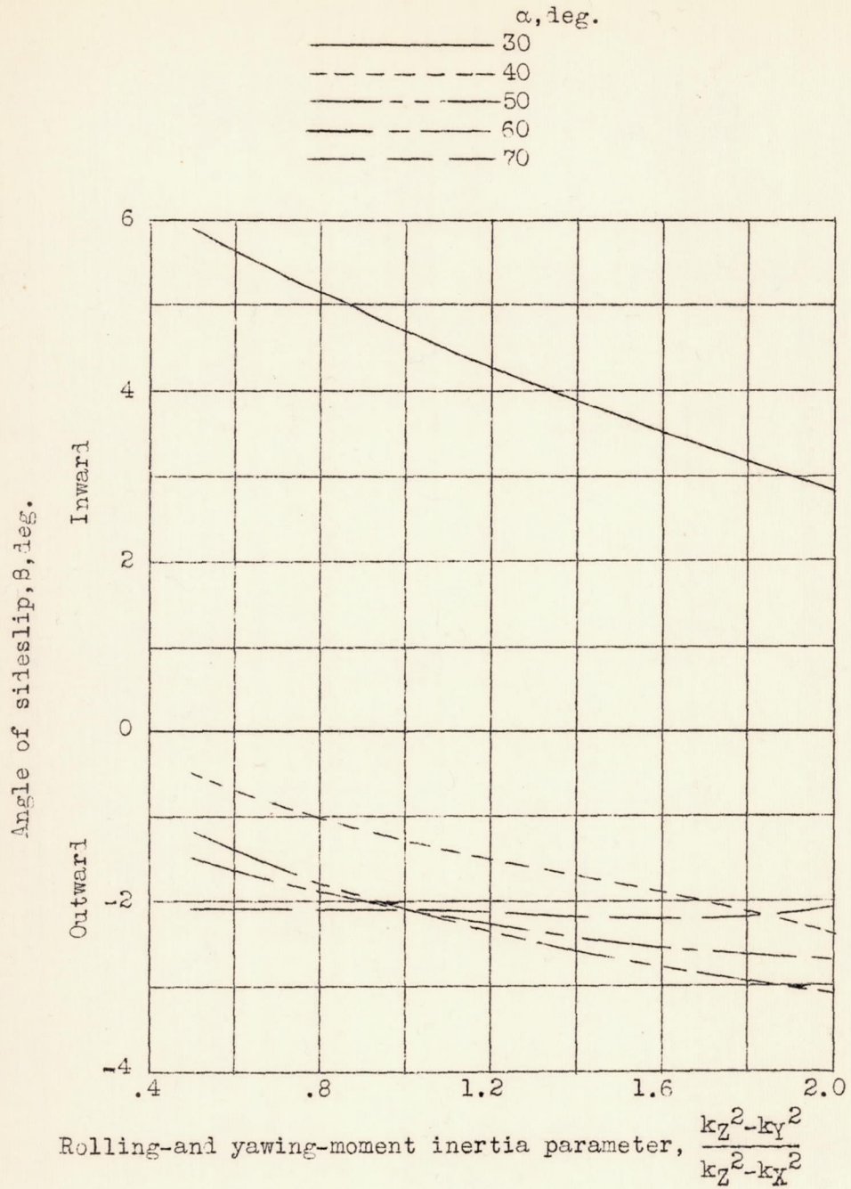
Figure 19a.- Effect of rolling-and yawing-moment inertia parameter upon sideslip necessary for equilibrium in a spin; rectangular wing, rounded tips.
