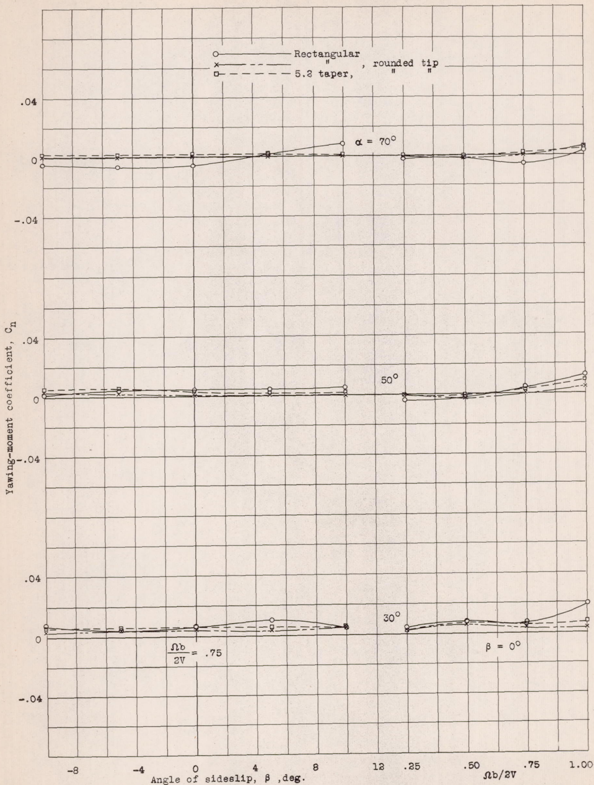
Figure 14.- Variation of yawing-moment coefficient C_n (body axes) with angle of sideslip and \Omega b/2V .
