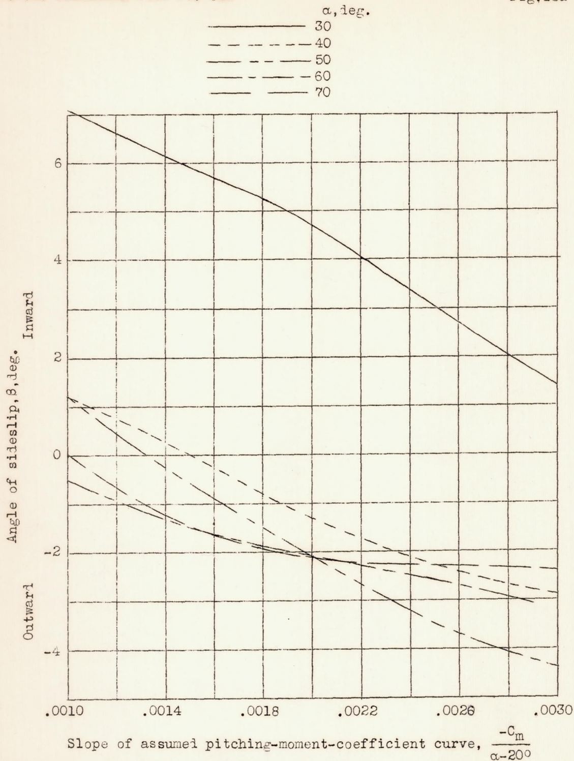
Figure 15a.- Effect of pitching-moment coefficient upon sideslip necessary for equilibrium in a spin; rectangular wing, rounded tips.
