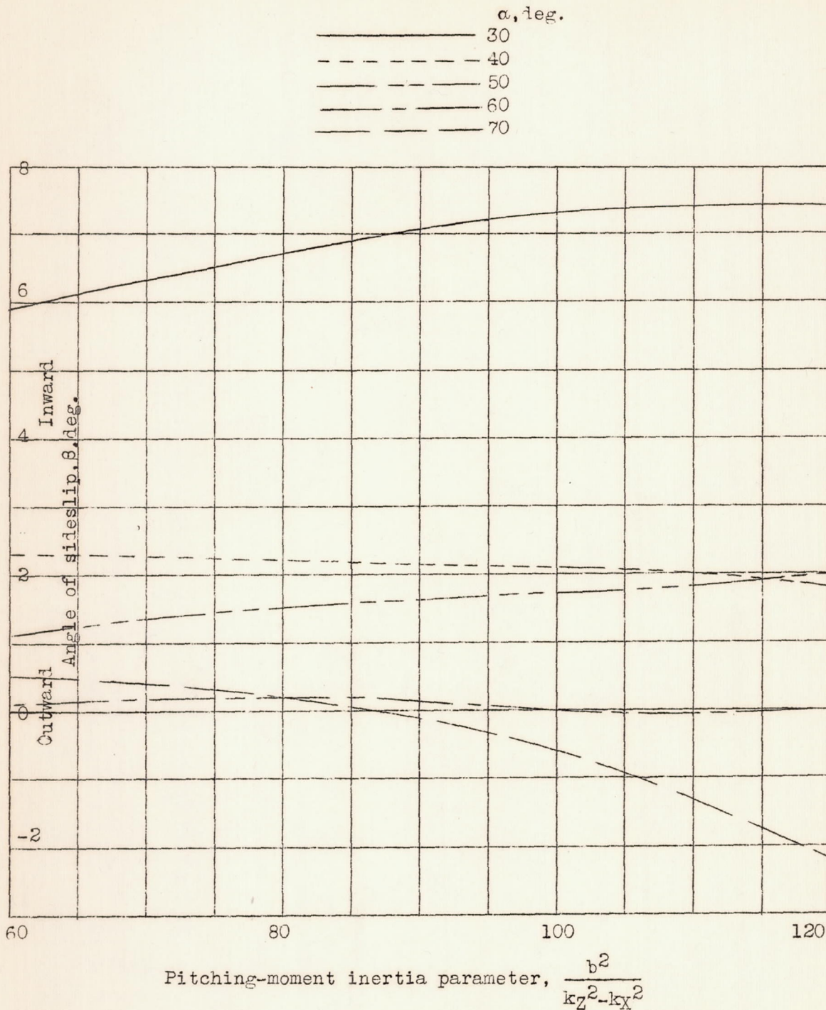
Figure 17b.- Effect of pitching-moment inertia parameter upon sideslip necessary for equilibrium in a spin; 5:2 tapered wing, rounded tips.
