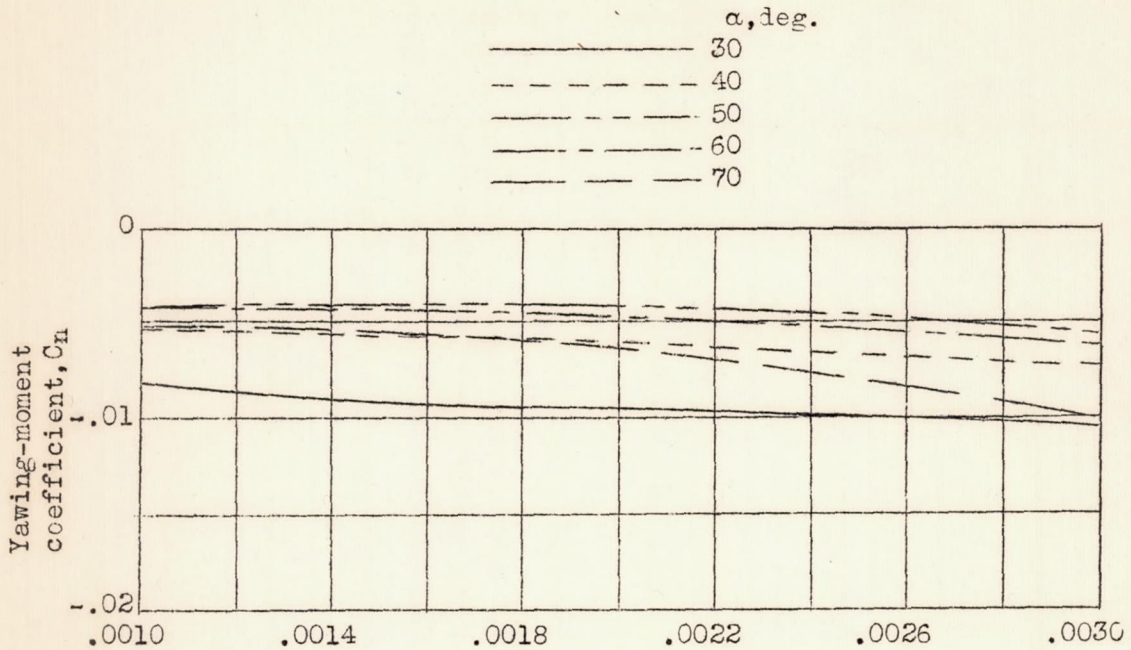
Slope of assumed pitching-moment-coefficient curve, \frac{-C_m}{\alpha-20^\circ} Figure 16a.- Rectangular wing, rounded tips.
