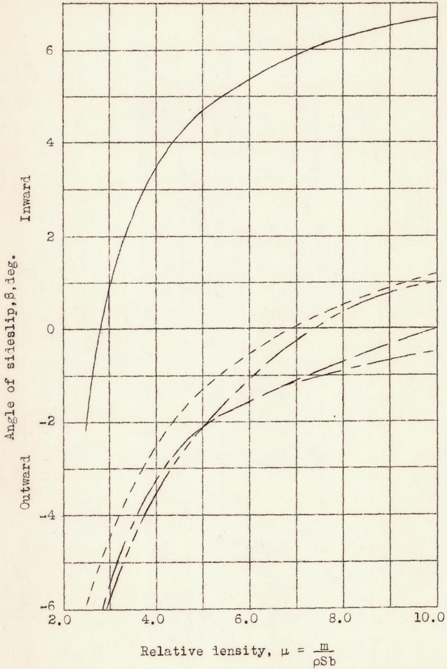
Figure 21a.- Effect of relative density of airplane upon sideslip necessary for equilibrium in a spin; rectangular wing, rounded tips.
