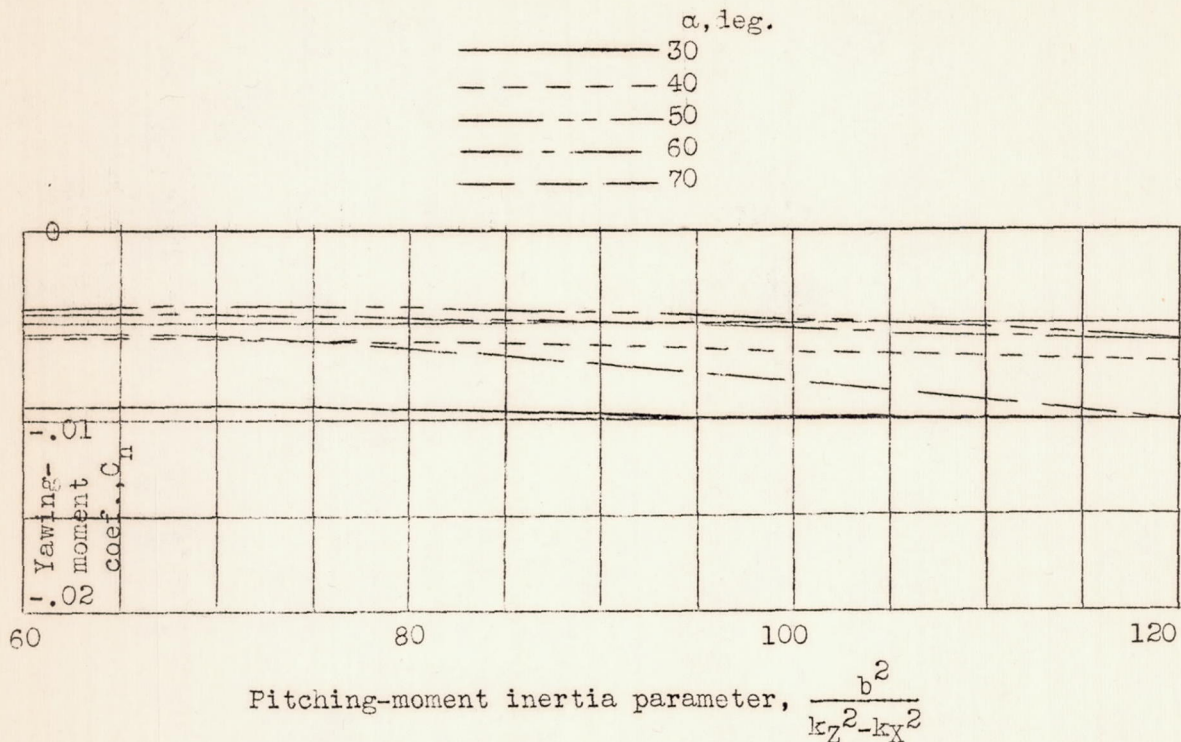
Figure 18a.- Rectangular wing, rounded tips.
