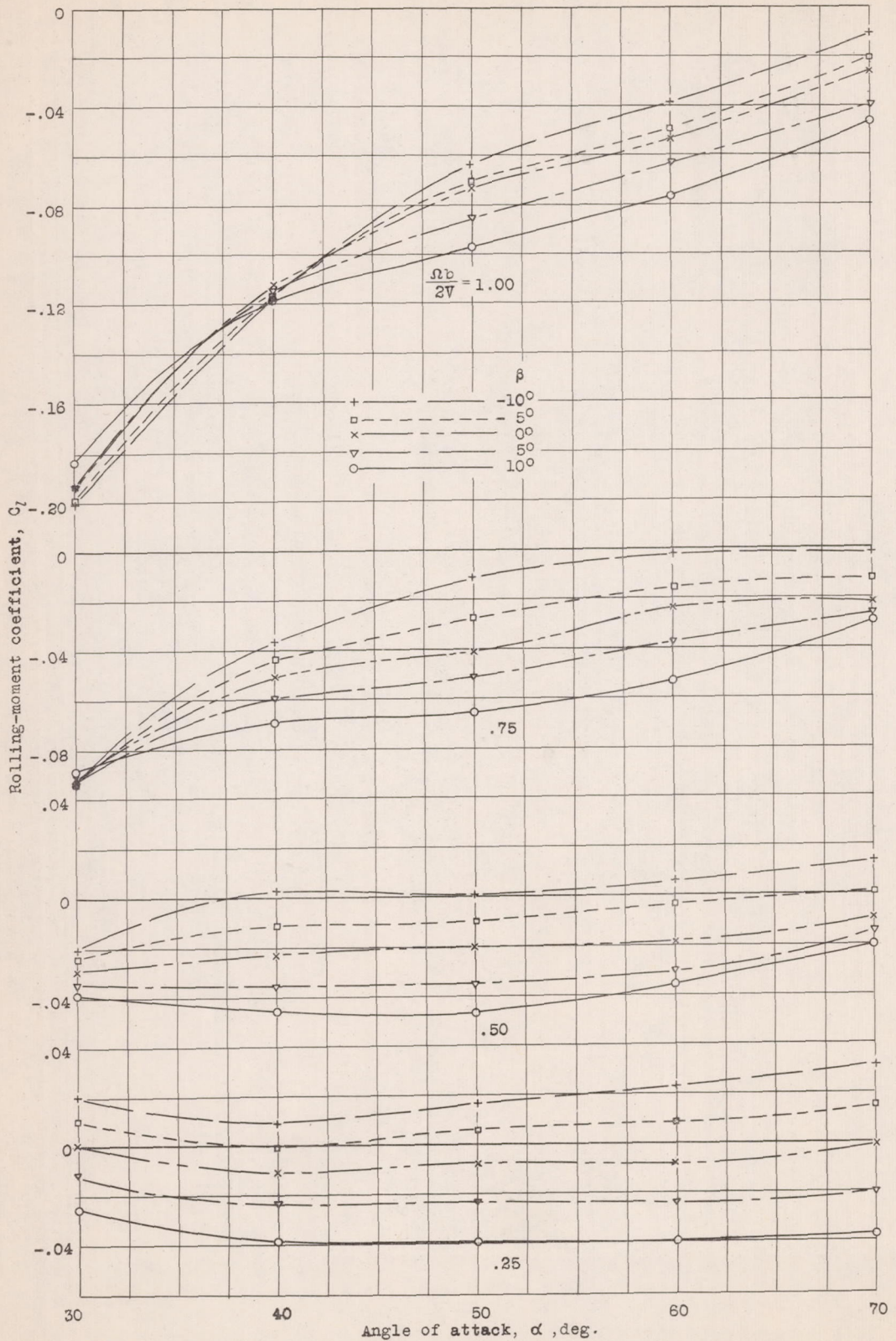
Figure 9a.- Variation of rolling-moment coefficient C_l (body axes) with angle of attack; rectangular wing, rounded tips.
