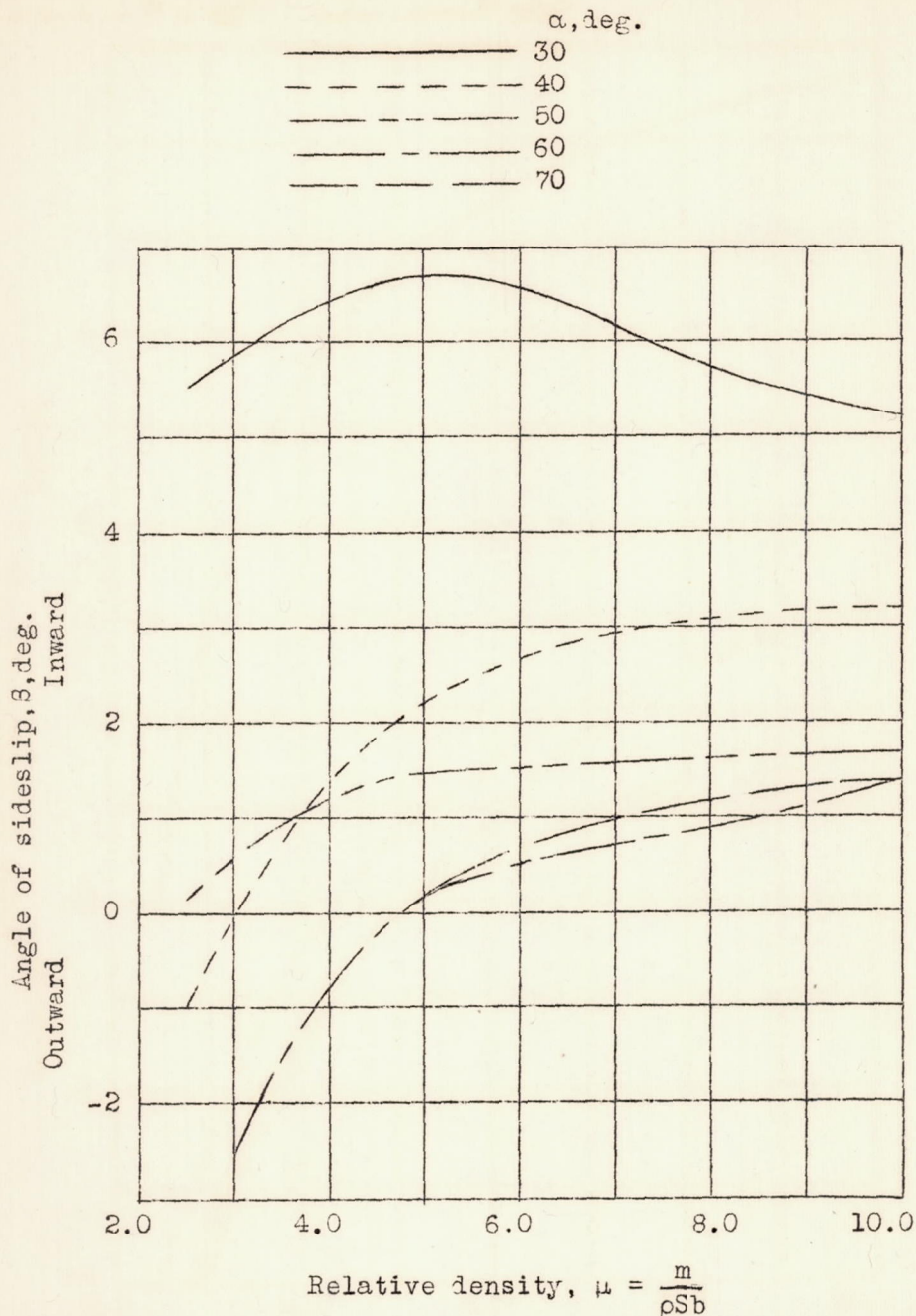
Figure 21b.- Effect of relative density of airplane upon sideslip necessary for equilibrium in a spin; 5:2 tapered wing, rounded tips.
