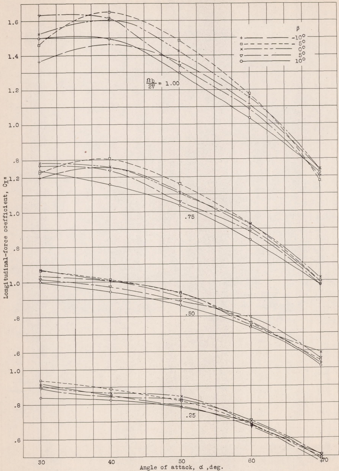
Figure 5a.- Variation of longitudinal-force coefficient C_{x''} (earth axes) with angle of attack; rectangular wing, rounded tips.
