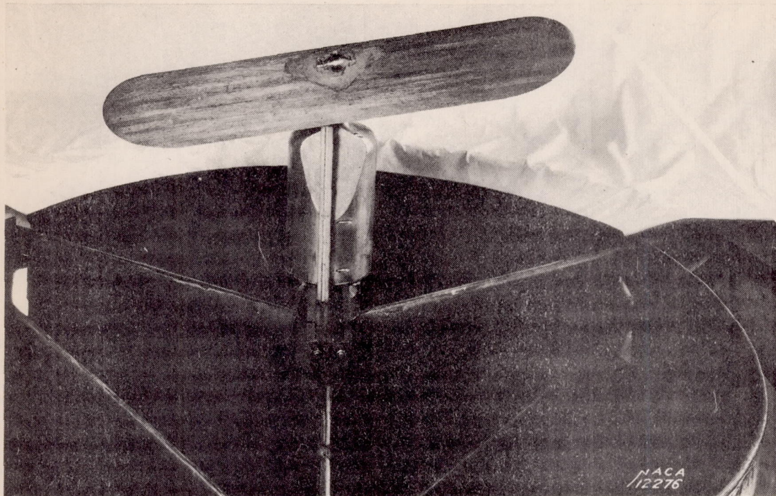
Figure 3.- The rectangular Clark Y wing with rounded tips mounted on the spinning balance.
