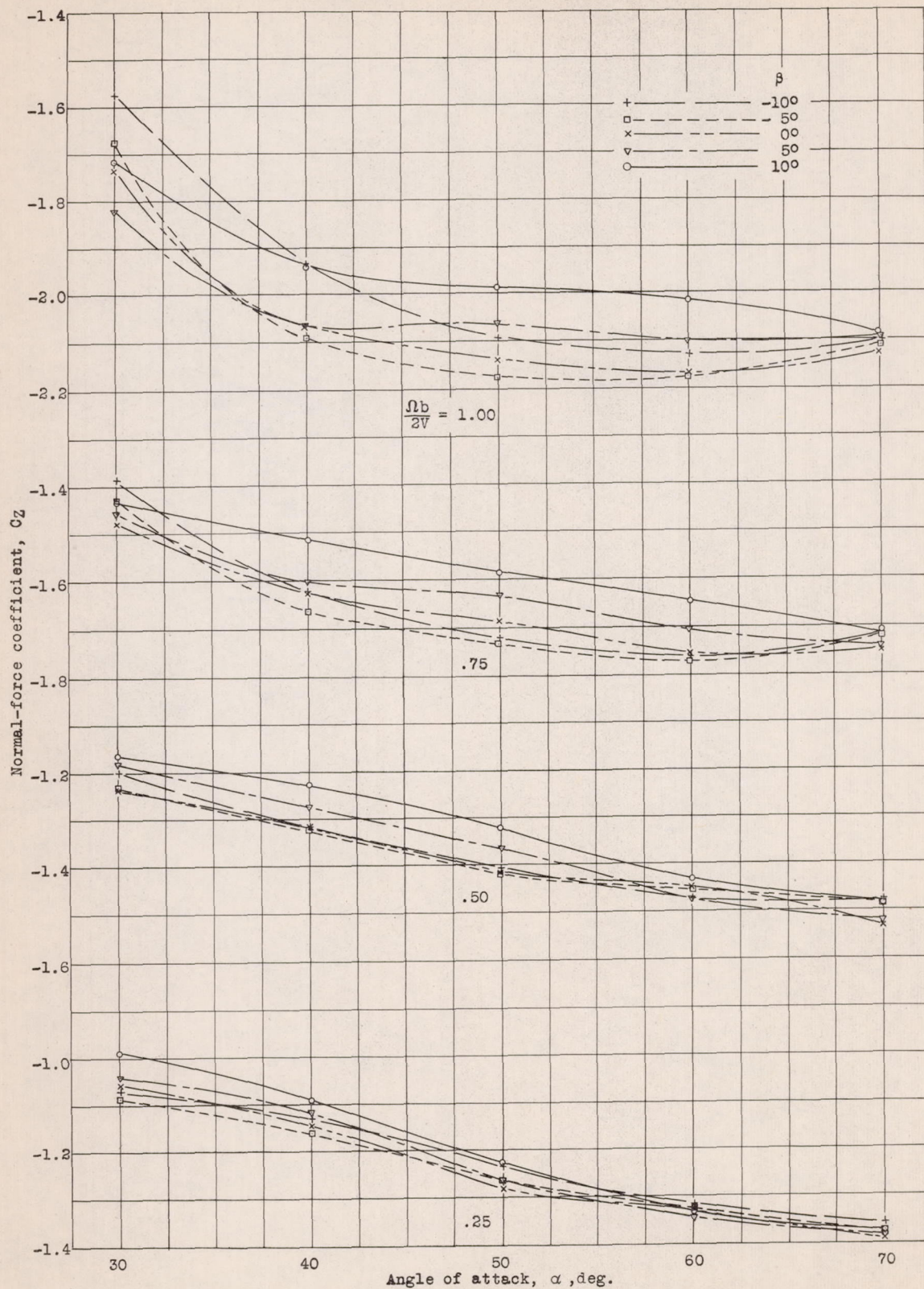
Figure 7a.- Variation of normal-force coefficient C_z (body axes) with angle of attack; rectangular wing, rounded tips.
