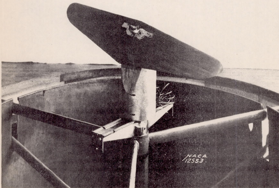
Figure 4.- The 5:2 tapered Clark Y wing with rounded tips mounted on the spinning balance.
