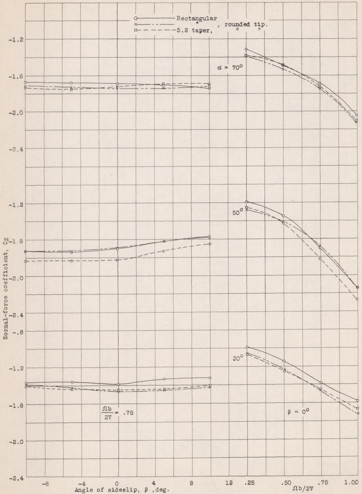
Figure 8.- Variation of normal-force coefficient C_z (body axes) with angle of sideslip and \Omega b / 2V .
