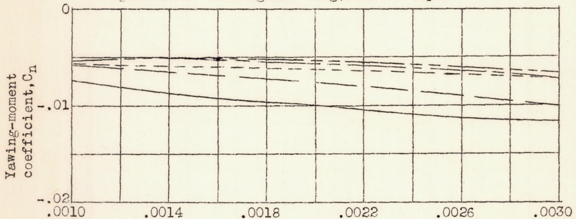
Slope of assumed pitching-moment-coefficient curve, \frac{-C_m}{\alpha-20^\circ} Figure 16b.- 5:2 tapered wing, rounded tips.
