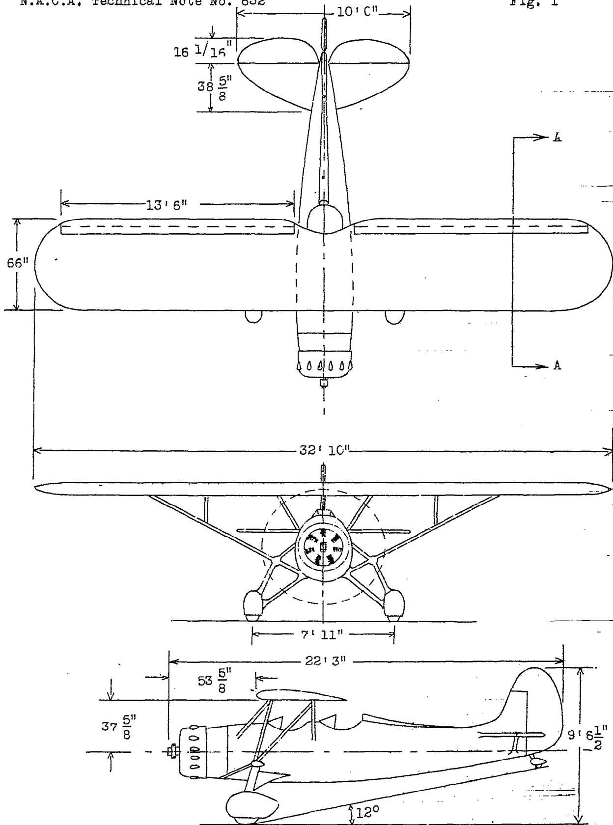
Figure 1.- Three-view drawing of the Fairchild 22 airplane.
