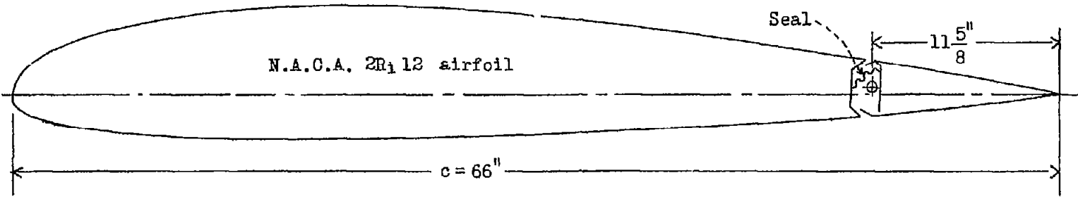
Section A-A, (Figure 1)
