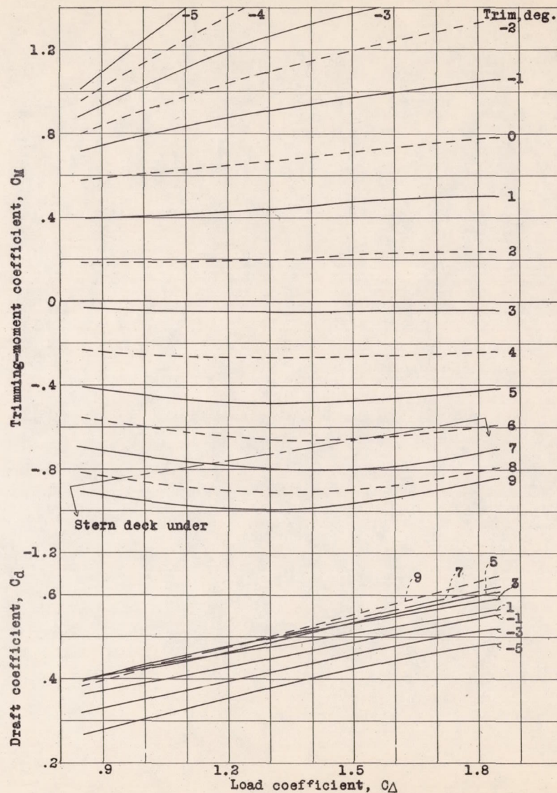
Figure 17.- Model 57-B-5. Static properties.
