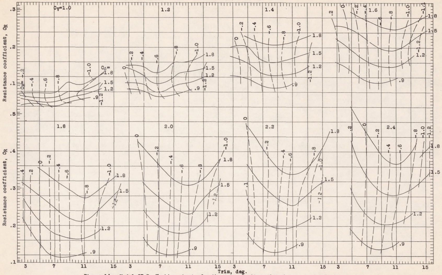
Figure 14a.-Model 57-B. Working charts for the determination of resistance and trimming moment.
