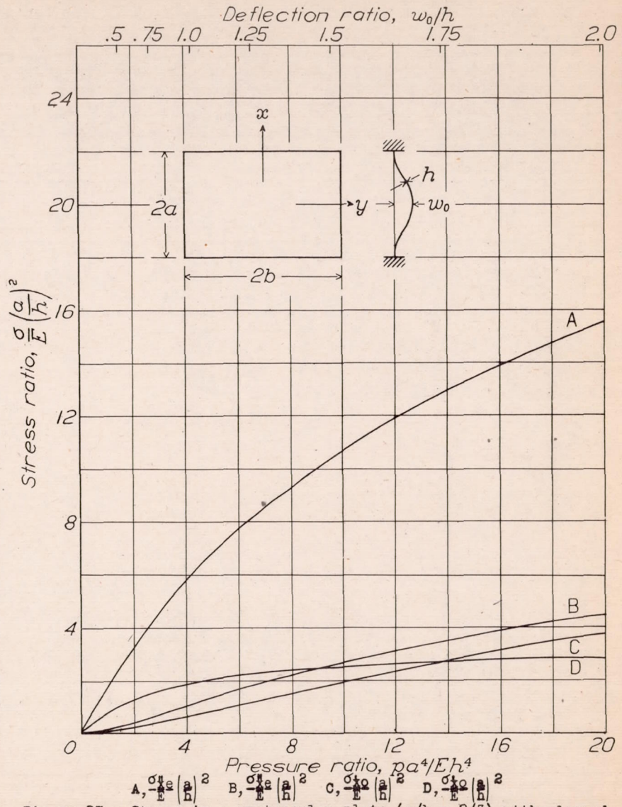
Figure 27.- Stress in a rectangular plate ( a/b = 2/3 ) with clamped edges according to reference 11. Poisson's ratio, 0.3.
