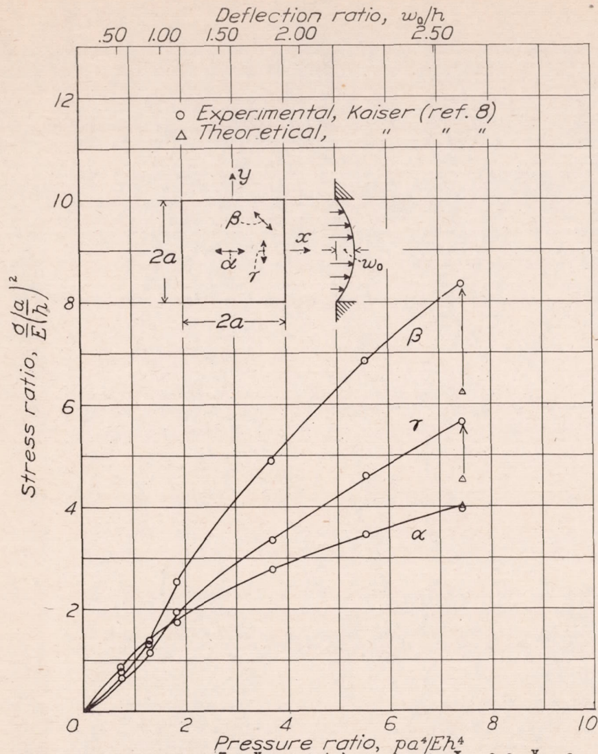
(β) Across diagonal at \frac{x}{a} = \frac{y}{a} = 0.6 (γ) Along axis \frac{x}{a} = 0.6, \frac{y}{a} = 0 (α) Along axis \frac{x}{a} = \frac{y}{a} = 0 Figure 32.- Maximum extreme-fiber stresses in a square plate with freely supported edges according to reference 8. Poisson's ratio, 0.3.
