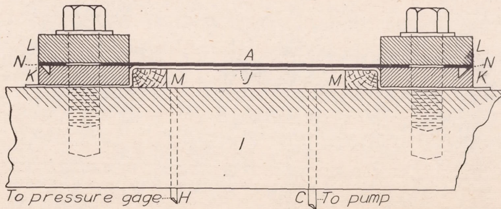
Figure 6. Section through plate mounted for normal pressure test with clamped edges.
