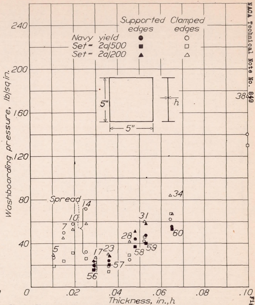
Figure 39.- Comparison of washboarding pressures for 5-by-5-inch 17S-T aluminum-alloy plates.
