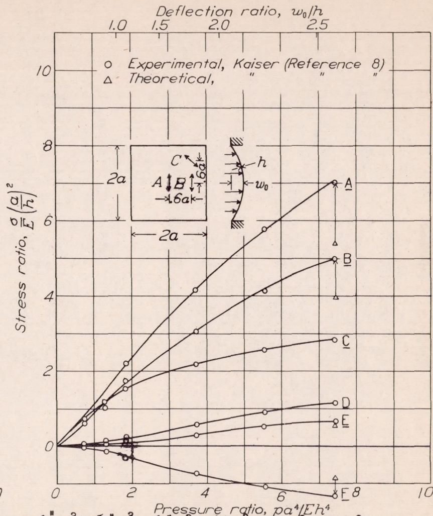
Figure 31.- Stresses in a square plate with freely supported edges according to reference 8. Poisson's ratio, 0.3.
