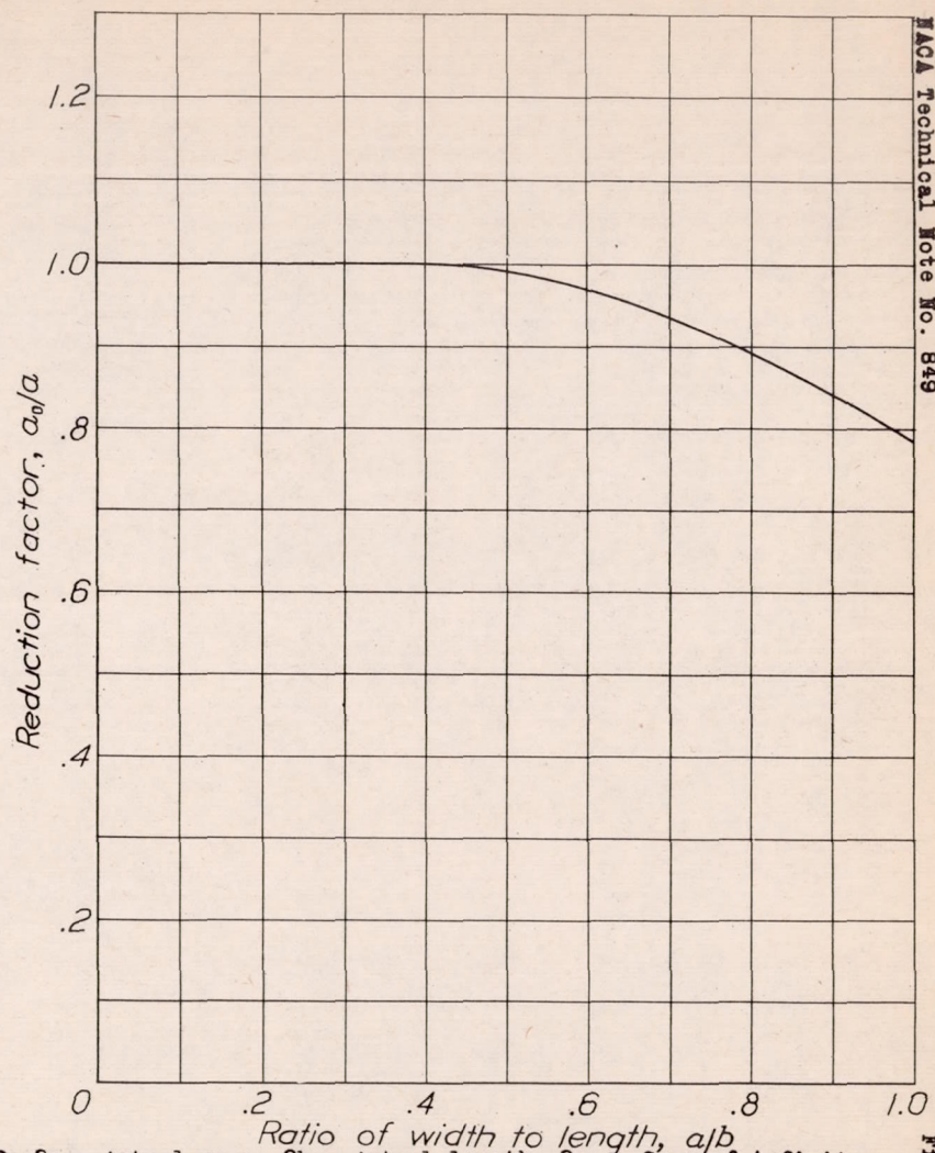
Figure 35.- Reduction factor for maximum stress at center of longest side of clamped rectangular plates.
