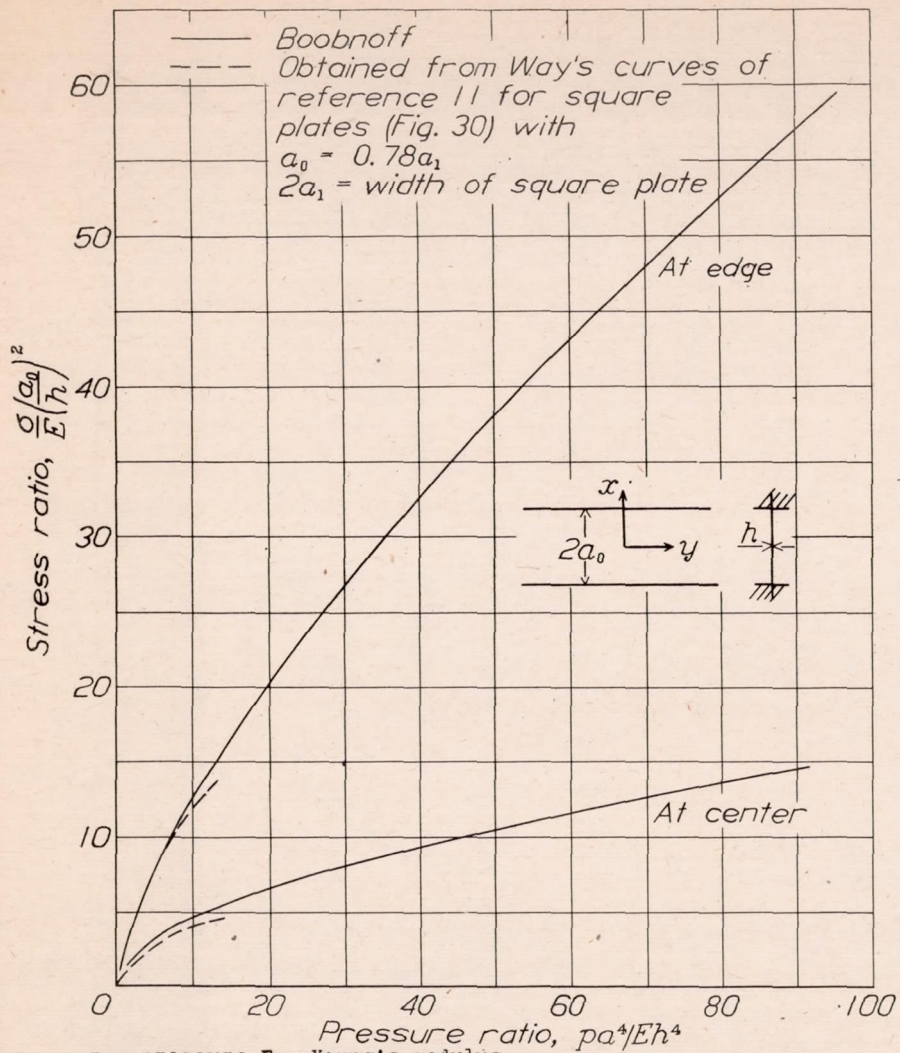
Figure 36.- Extreme-fiber stress in infinite plate strip ( a/b = 0 ), clamped edges, according to reference 12. Poisson's ratio, 0.3.
