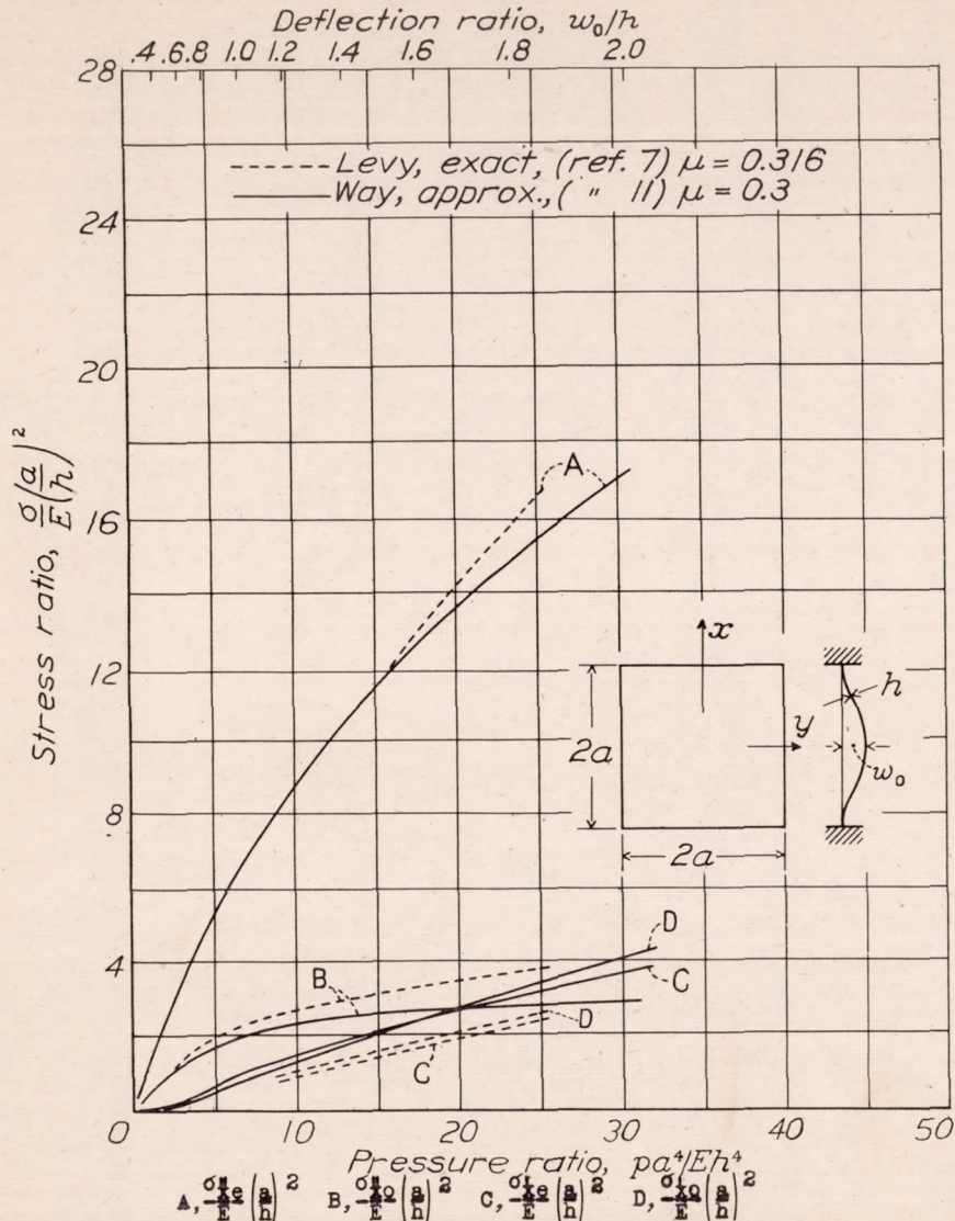
Figure 26.- Stress in a square plate with clamped edges.
