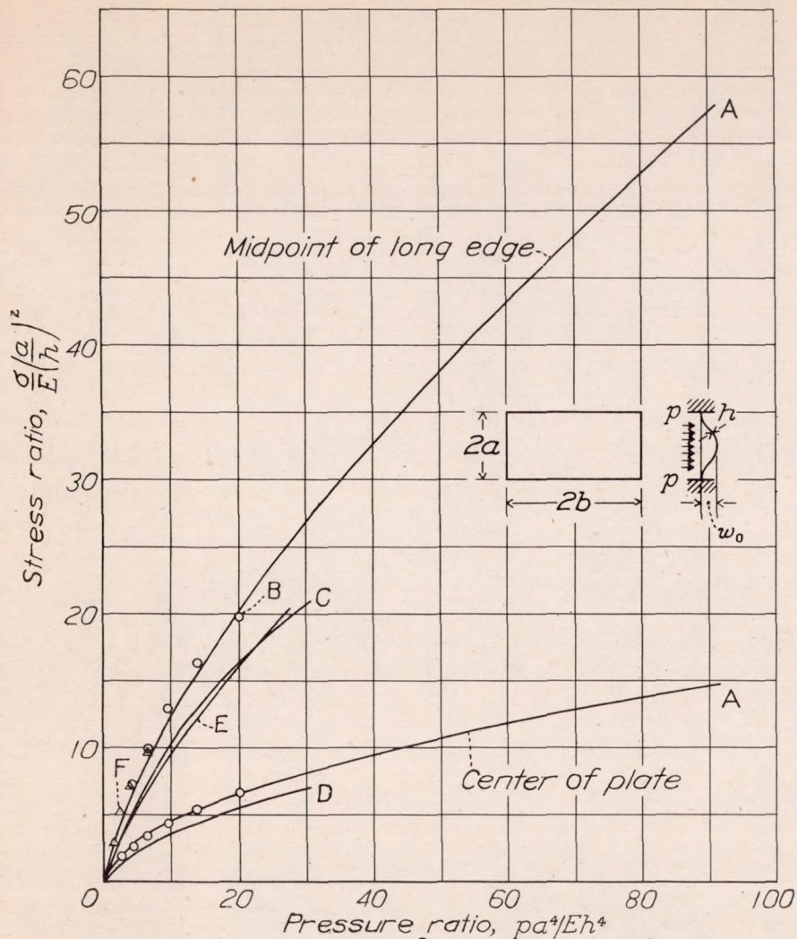
Figure 30.- Extreme-fiber stresses for rectangular plates with clamped edges. Data from references 7, 11 and 12.
