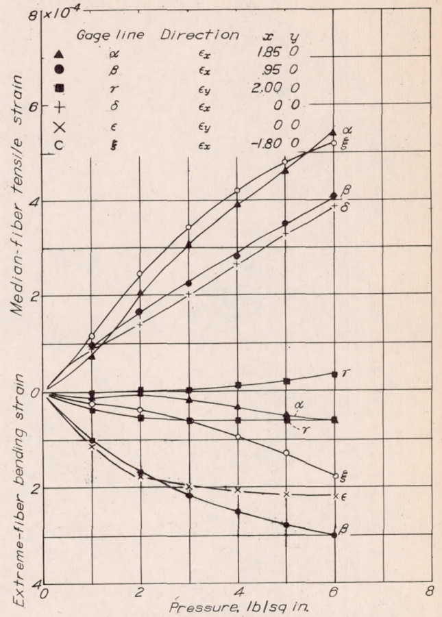
Figure 17.- Medium-fiber tensile strain and extreme-fiber bending strain (average over 1-in. gage length) for square 178-T aluminum-alloy plate 10a with clamped edges.
