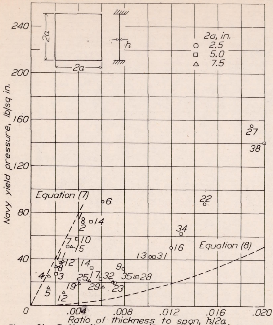
Figure 34.- Washboarding pressures (Navy yield pressure) for square 178-T aluminum-alloy plates with clamped edges. Plates 12 and 14 had two distinct yield pressures.
