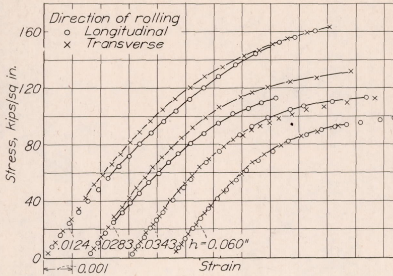
Figure 2.— Tensile stress strain curves for 18:8 stainless steel.
