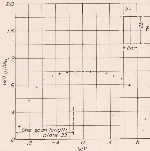
Figure 10.— Deflection curve along longitudinal center line of rectangular plates 33(17S-T) with clamped edges.
