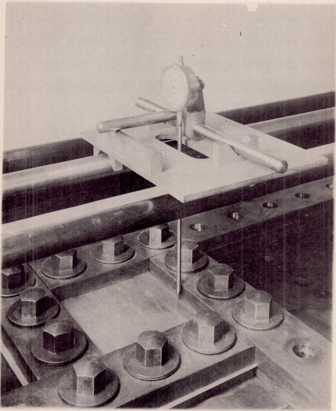
Figure 7.- Auxiliary platform for measuring deflections at points 1/20 inch apart.
