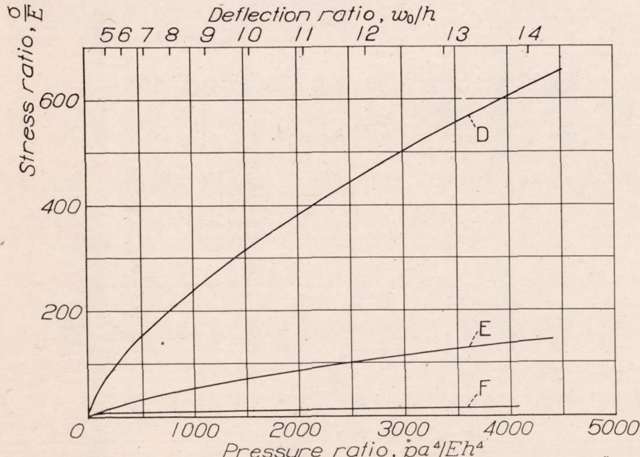
Figure 28.- Stress in infinite plate strip ( a/b = 0 ) with clamped edges according to reference 11. Poisson's ratio, 0.3.
