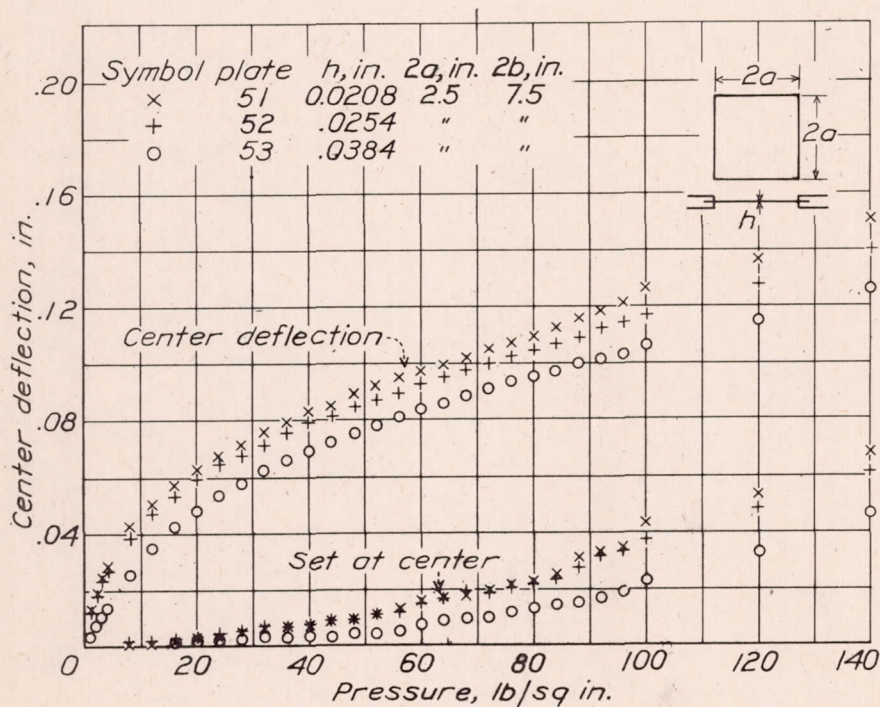
Figure 13.— Deflection and set at center of rectangular 17S-RT aluminum alloy plates with clamped edges.
