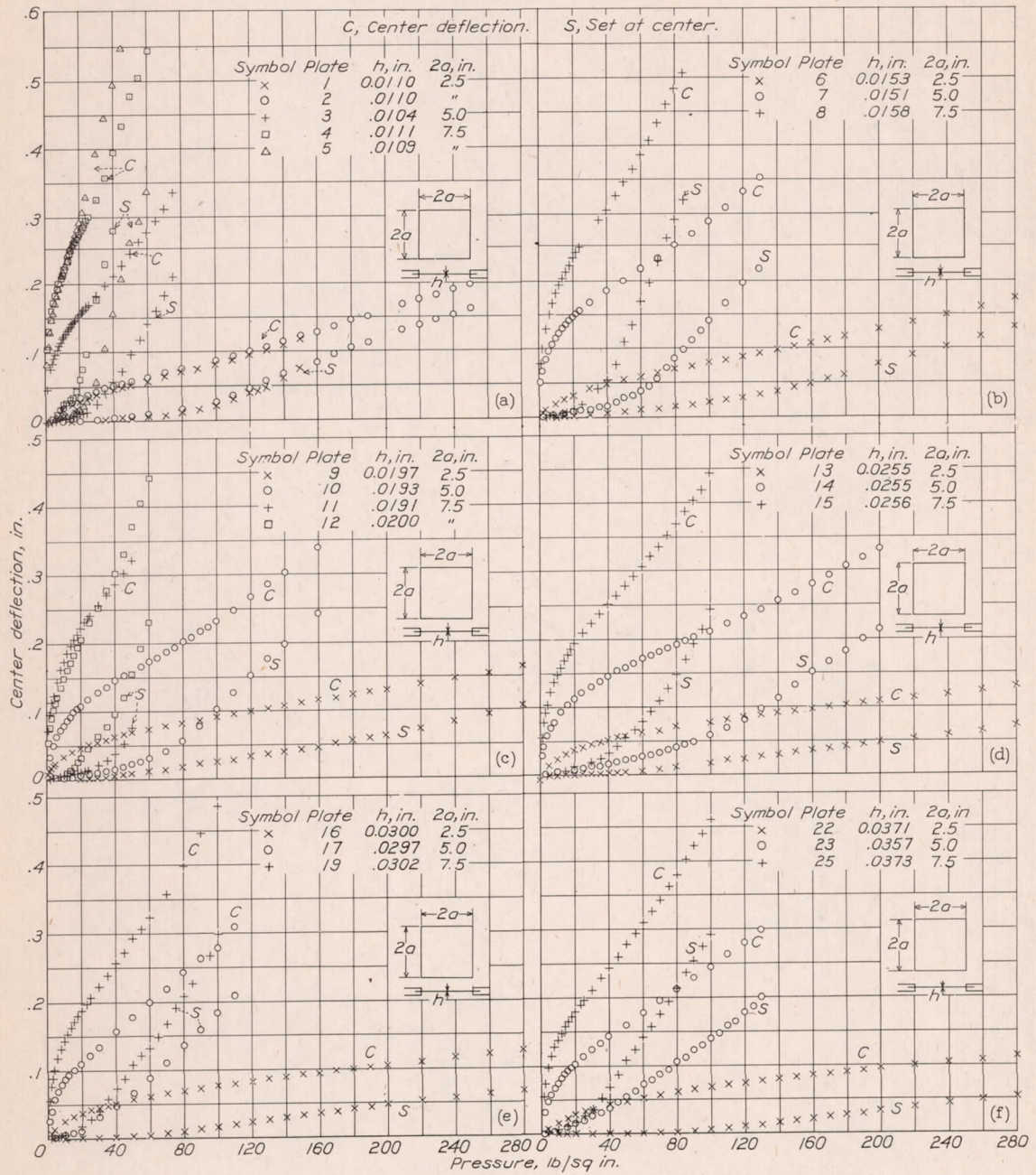
Figure 11 (a to j).— Deflection and set at center of square 17S-T aluminum-alloy plates with clamped edges.
