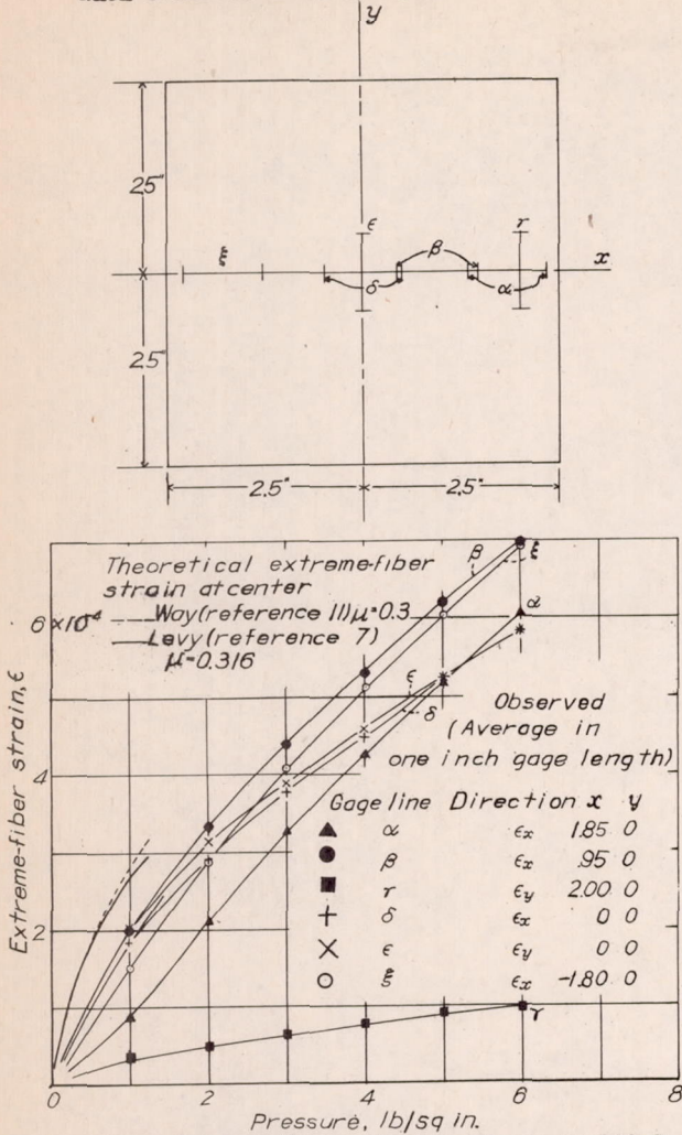
Figure 16.- Extreme-fiber strains on square 178-T aluminum-alloy plate 10a with clamped edges.
