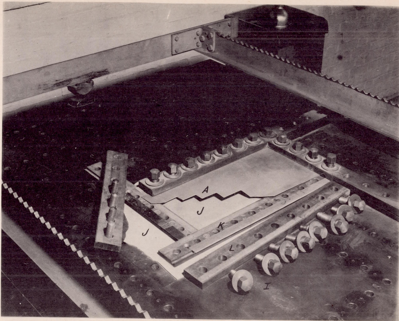
Figure 5.- Cut-away plate showing method of clamping plate in testing apparatus.
