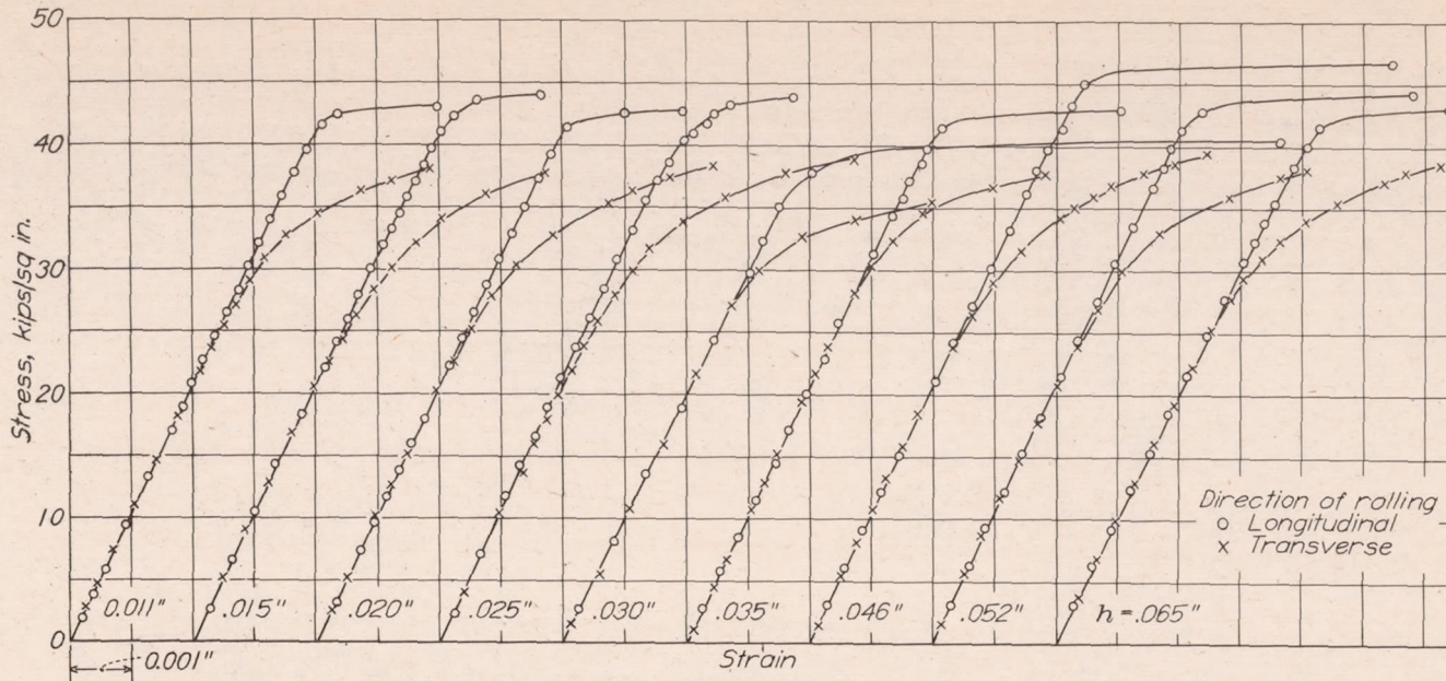
Figure 1. Tensile stress strain curves for 17S T aluminum alloy.
