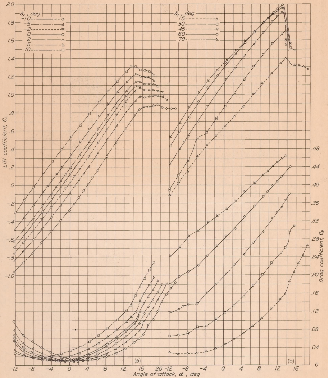
(a) Small flap deflections.
