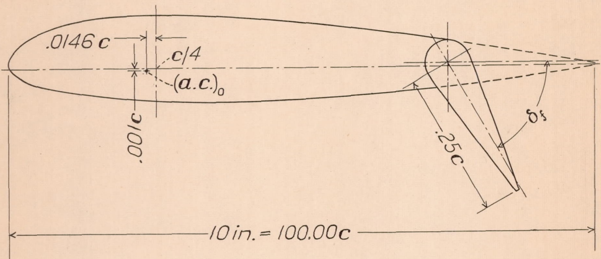
Figure 2.- Plain flap on the rectangular N.A.C.A. 23015 airfoil.
