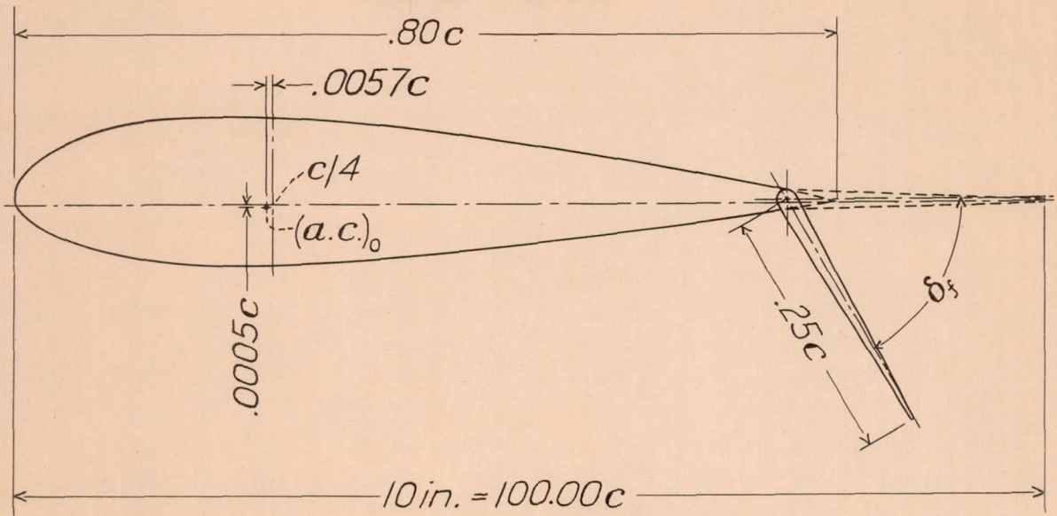
Figure 1.- Gwinn flap on the rectangular N.A.C.A. 23018 airfoil.
