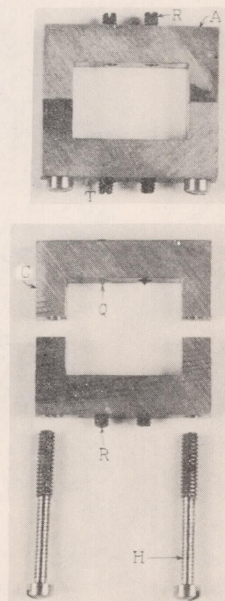
Figure 4.- Auxiliary clamps.
