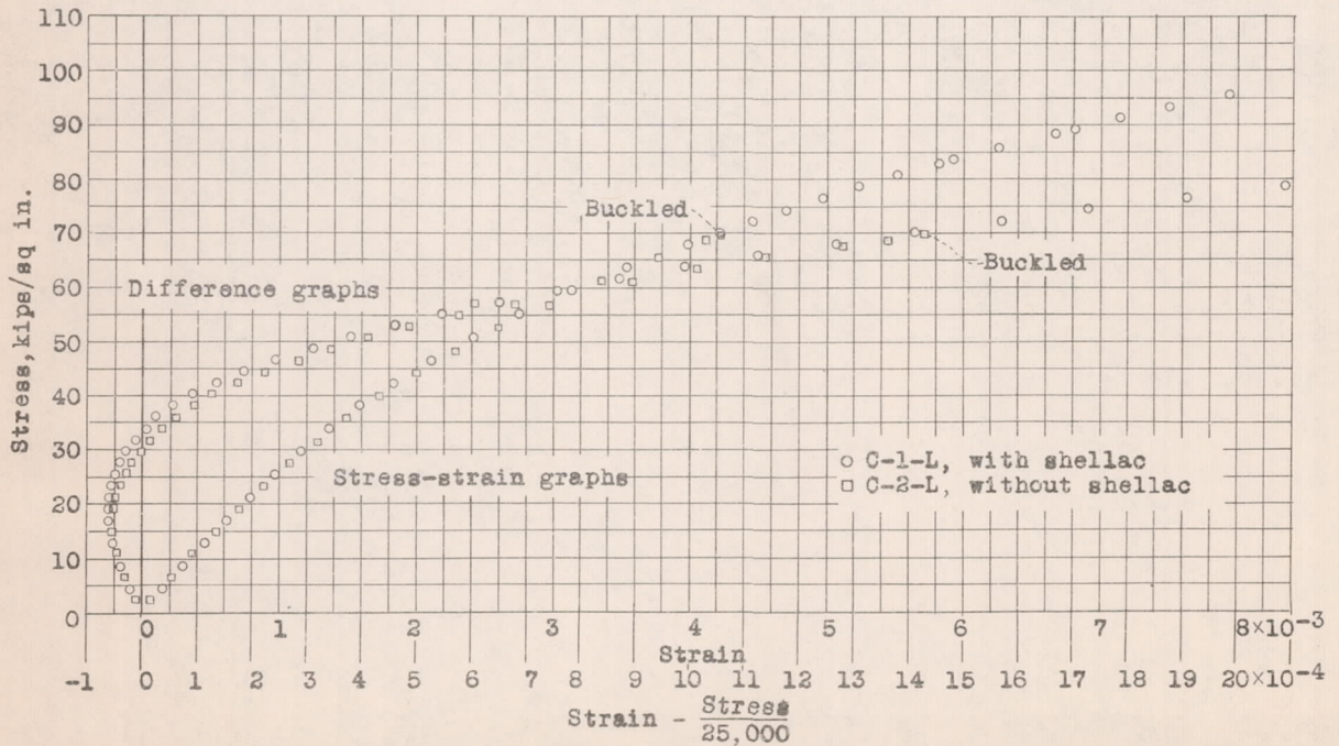
Figure 6.- Stress-strain and difference graphs for packs C1L and C2L from pack compressive tests.
