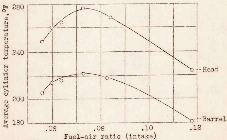
Figure 7.- Effect of mixture strength on cylinder temperatures. Spark timing, 16 crank degrees B.T.C.
