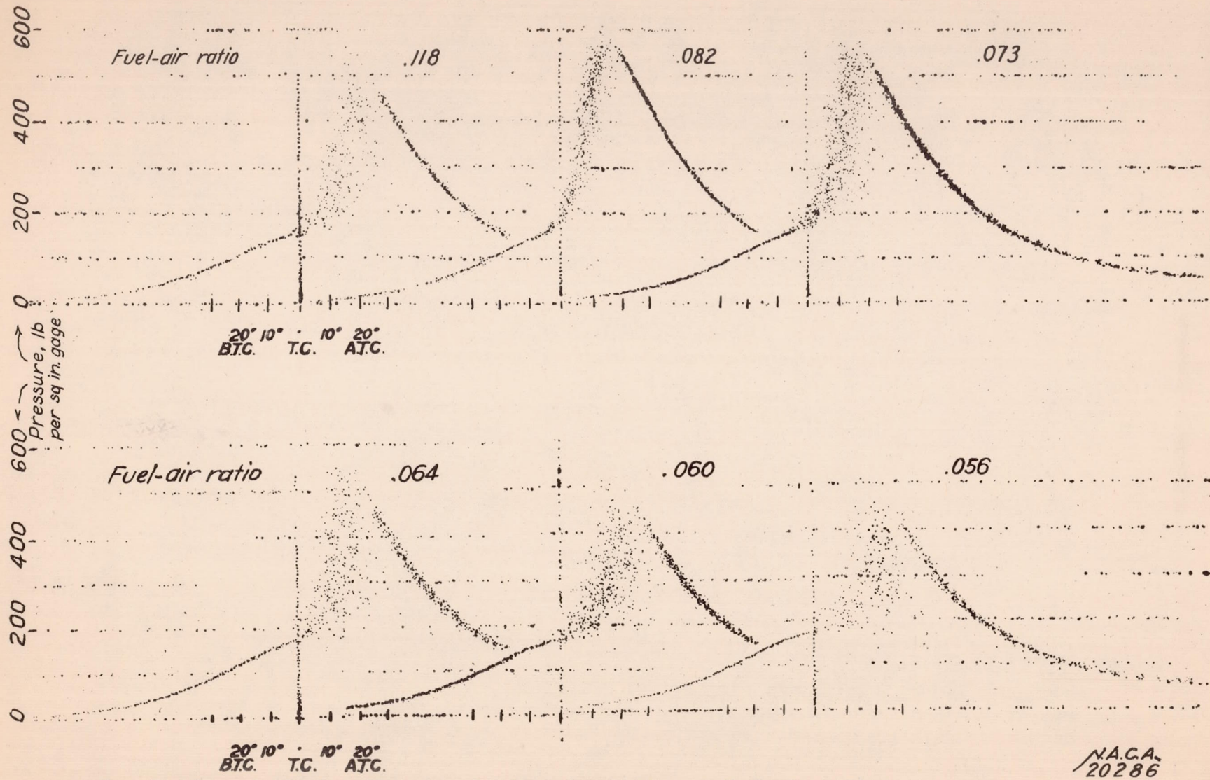
Figure 2.- Farnboro indicator diagrams obtained for different fuel-air ratios. Engine speed, 1500 rpm, compression ratio, 7.4, spark timing, 16 crank degrees B.T.C.
