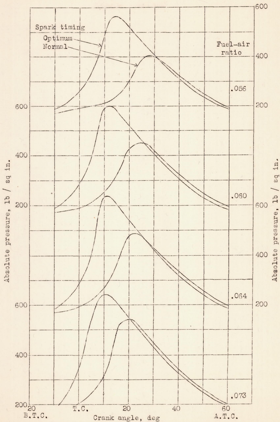
Figure 4.- Effect of mixture strength and spark timing on indicator-card shape.
