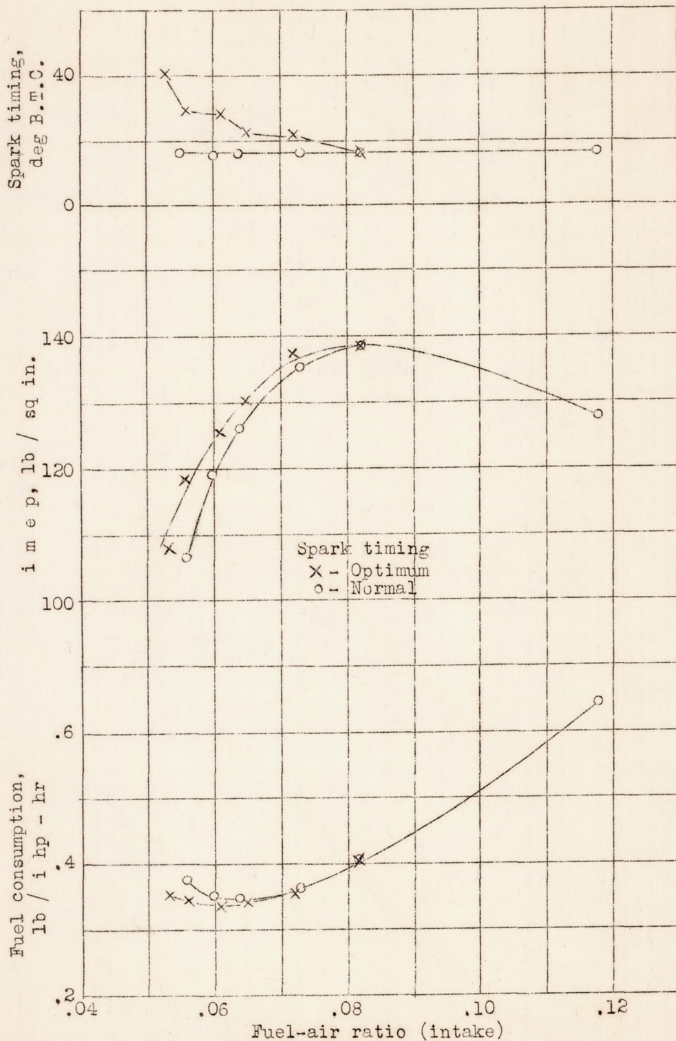
Figure 5.- Effect of mixture strength and spark timing on engine performance.
