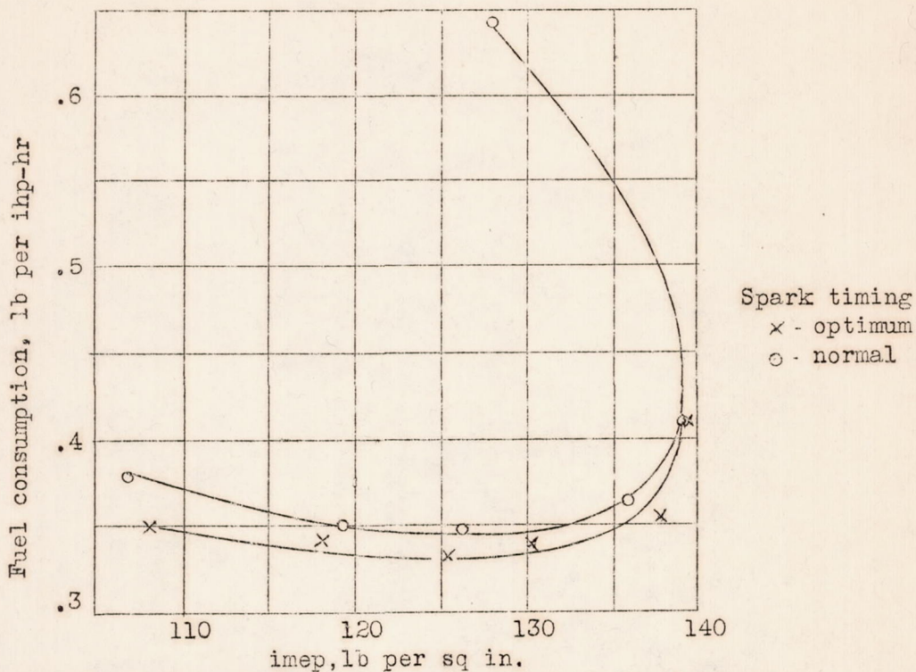
Figure 6.- Variation of fuel consumption with indicated mean effective pressure (mixture control run).
