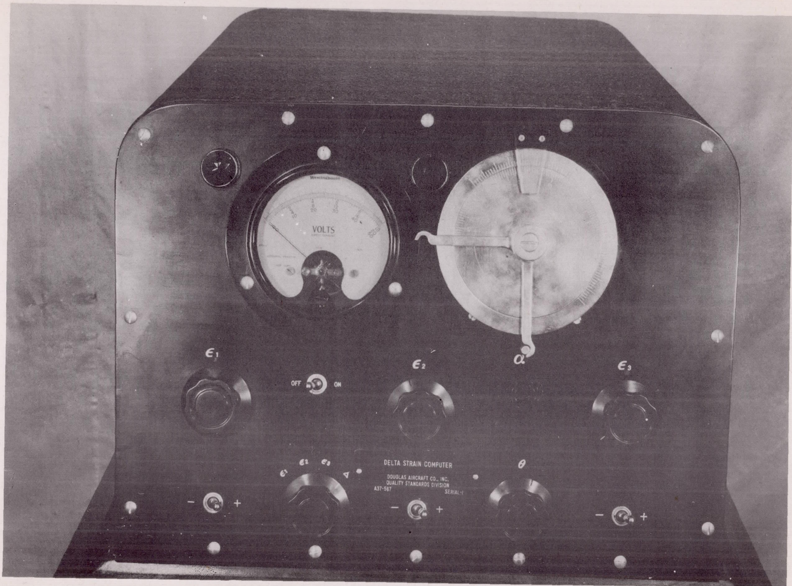
Figure 3. - Delta strain computer containing shaft-coupled Selsyn devices.
