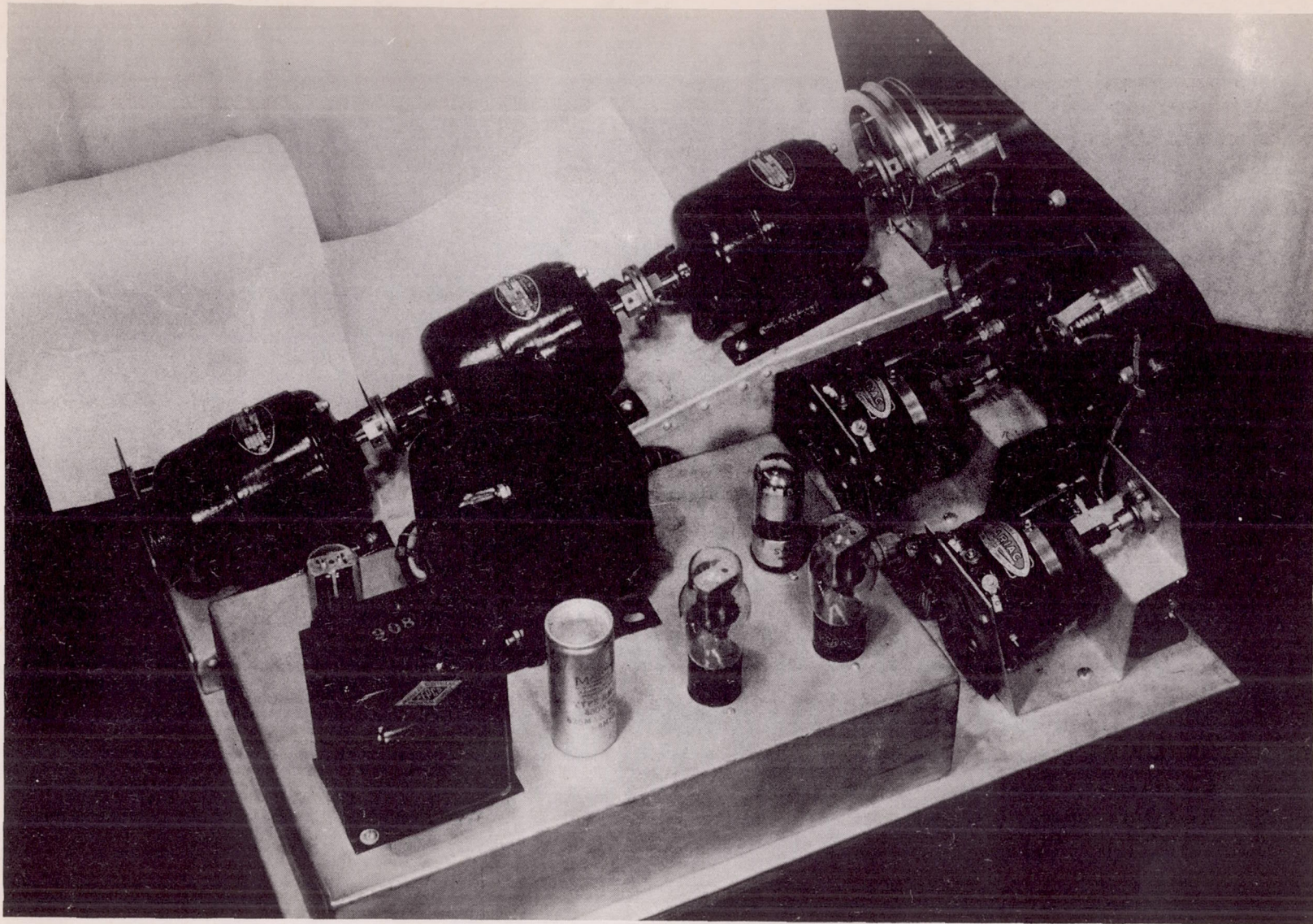
Figure 4. - View of delta strain computer showing shaft-coupled Selsyn devices.
