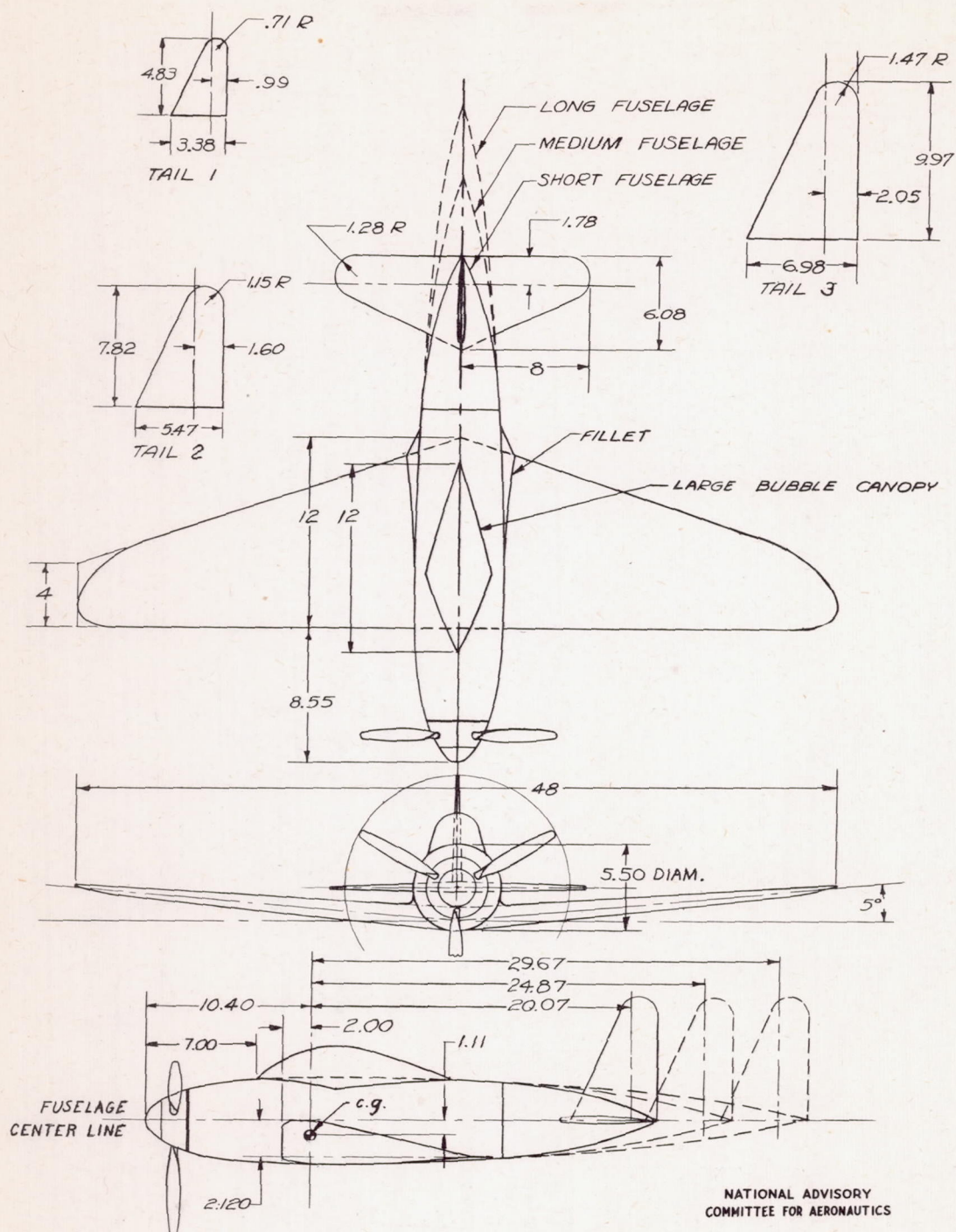
Figure 2.- Three-view drawing of model. Wing, NACA 23012 airfoil section; all rudder hinge lines located 29.3 percent of root chord from trailing edge of vertical tail; diameter of propeller, 14.25 inches; blade angle at 0.75 radius, 30°. (All dimensions in in.)
