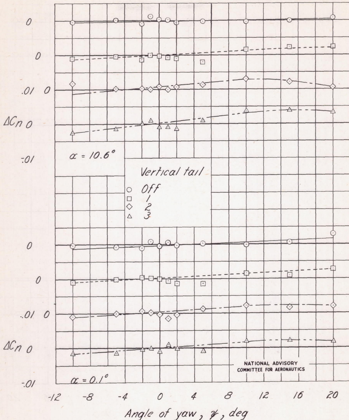
(b) Large bubble canopy; medium-length fuselage.
