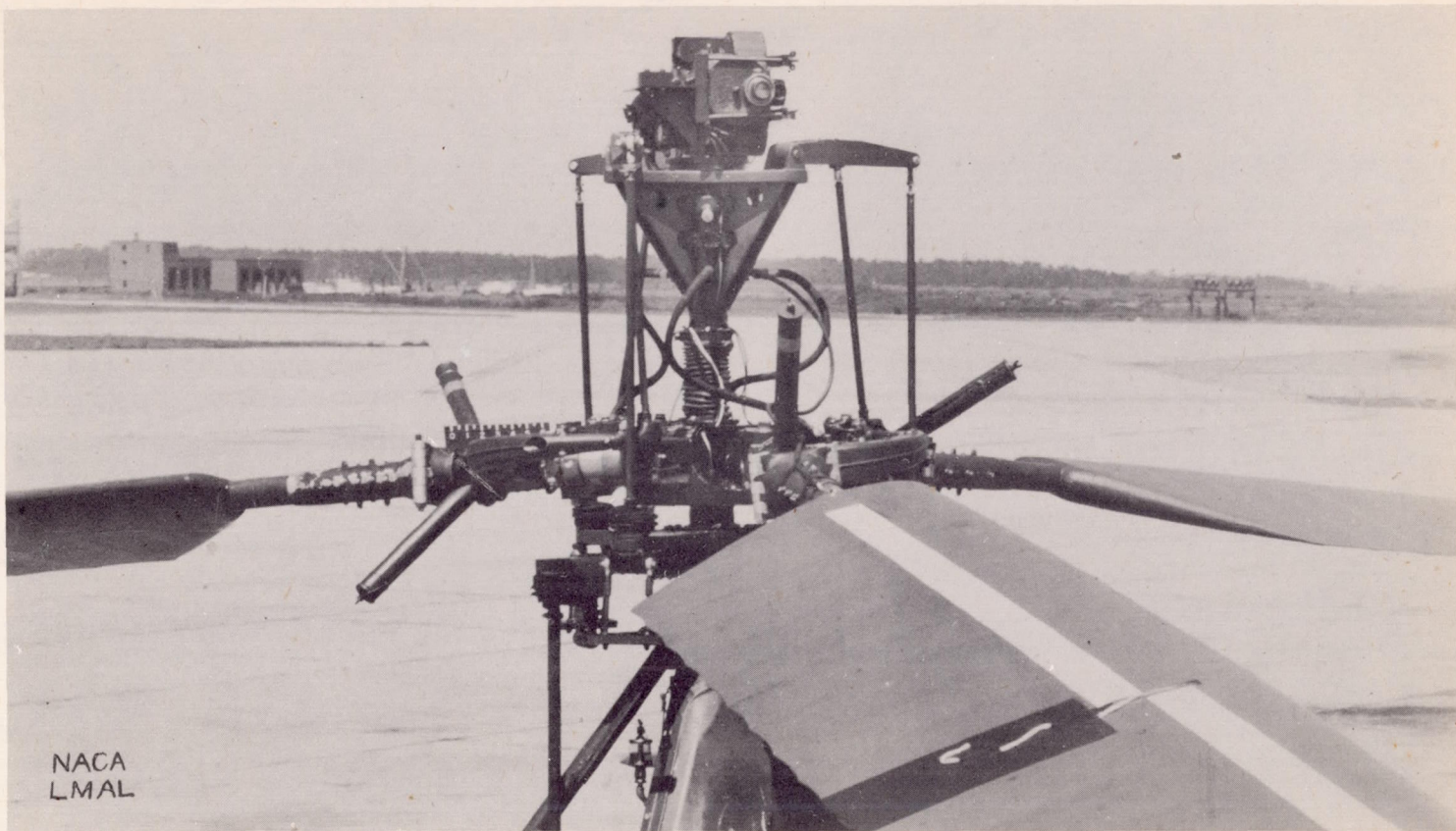
Figure 2.- Camera installation on helicopter rotor hub.
