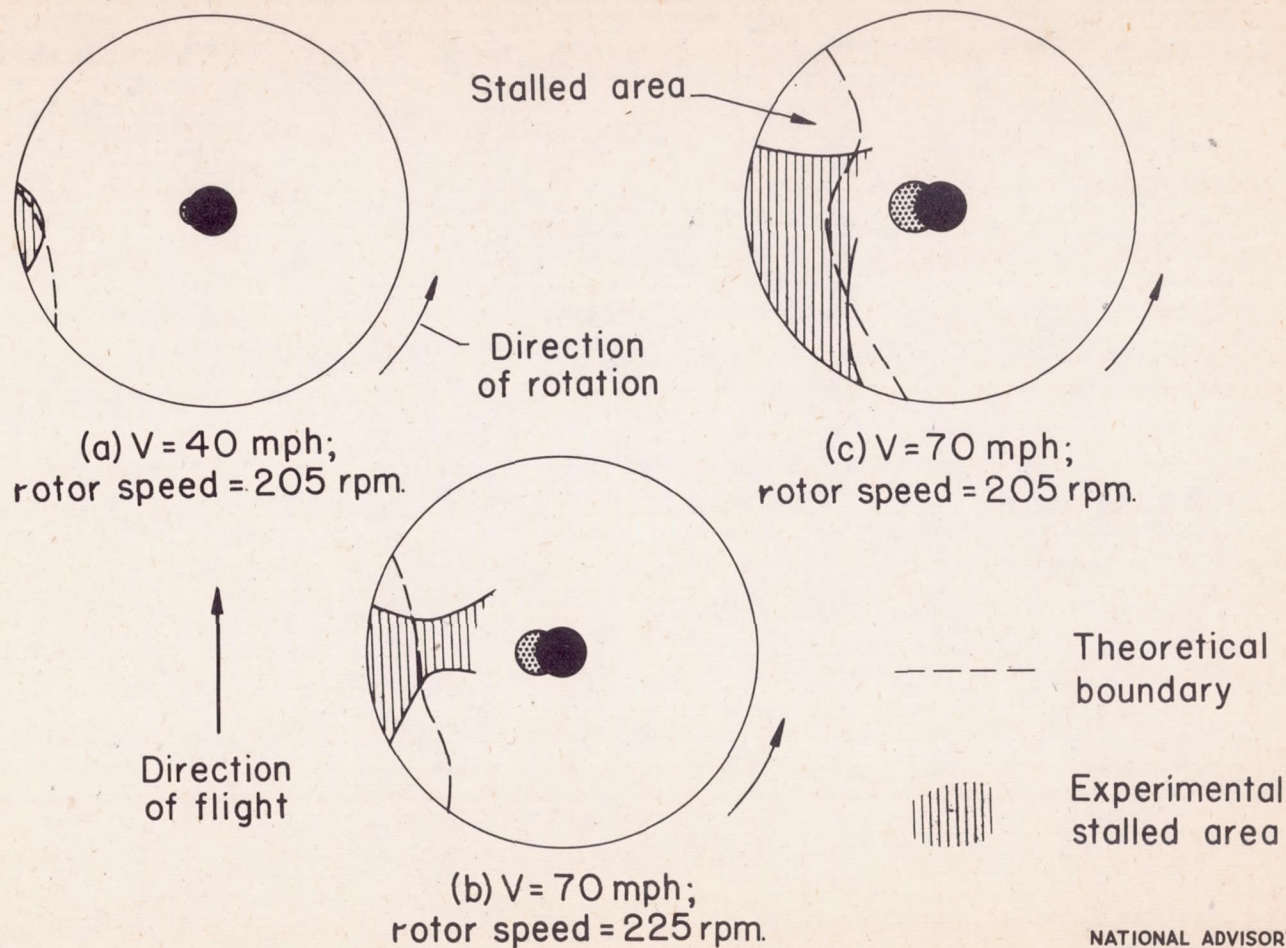
Figure 4.- Comparison between theoretical and experimental stalled areas.
