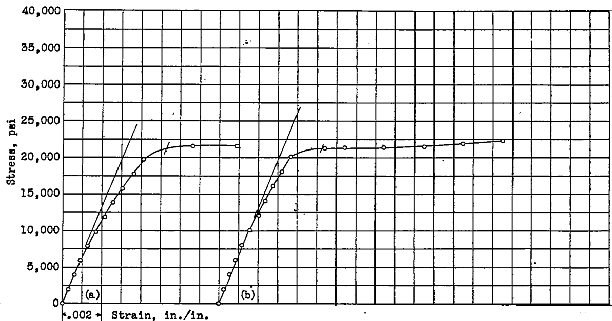
Figure 1.- Compressive stress-strain curves. (a) I-beam, die no. XM-844; web depth = 2.5 in.; flange width = 2 in.; thickness = 1/8 in.; (b) 2-1/2 × 2-1/2 × 7/16 in. angle. Metal, AM-C58S.
