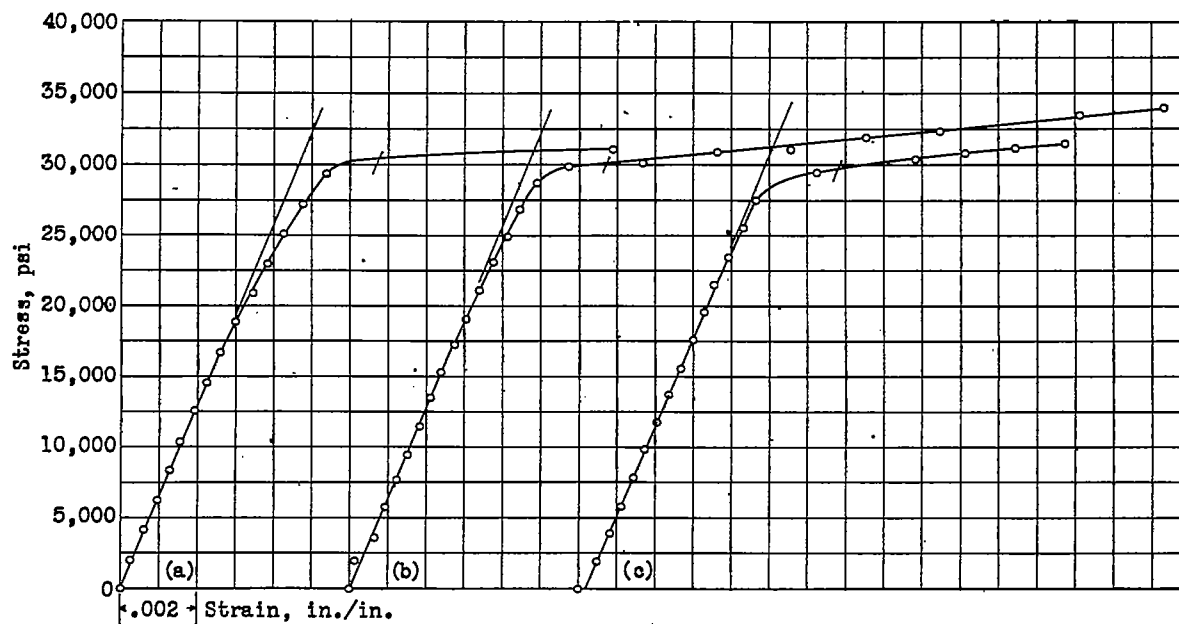
Figure 2.- Compressive stress-strain curves. (a) I-beam, die no. XM-844, web depth = 2.5 in., flange width = 2 in.; thickness = 1/8 in.; (b) 2-1/2 × 2-1/2 × 7/16 in. angle; (c) 4 × 4 × 1/2 in. angle. Metal, AM-C58S-T5.
