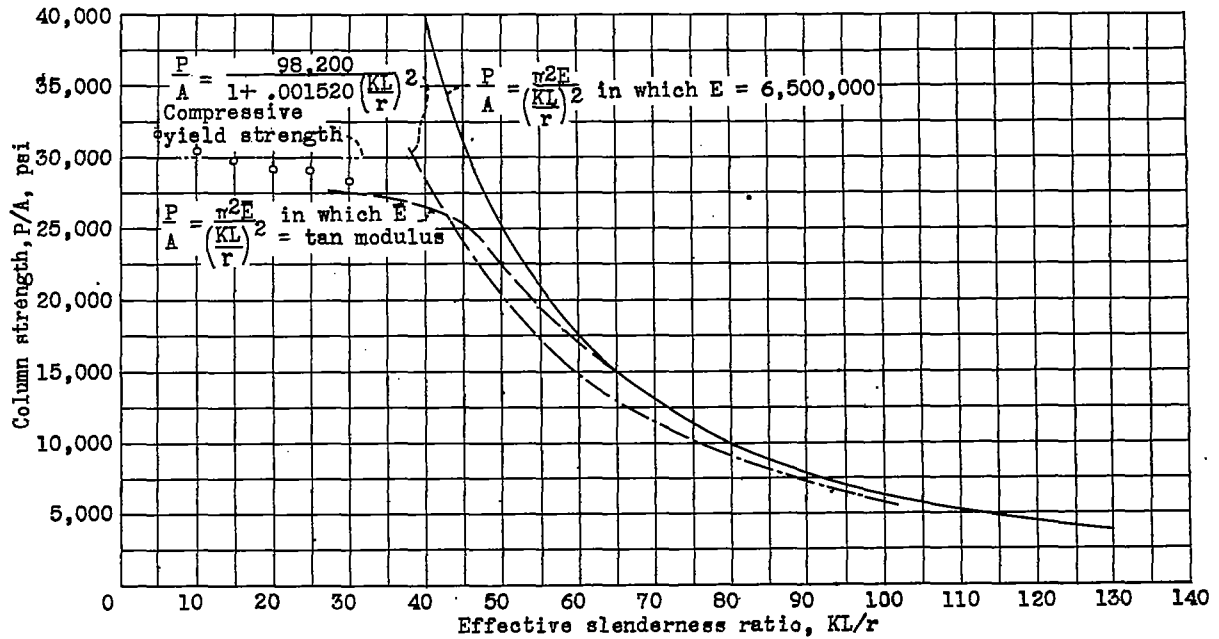
Figure 7.- Column strength of AM-C588-T5 4 x 4 x 1/2 in. angle. Specimens tested as columns with flat ends. K taken equal to .50.
