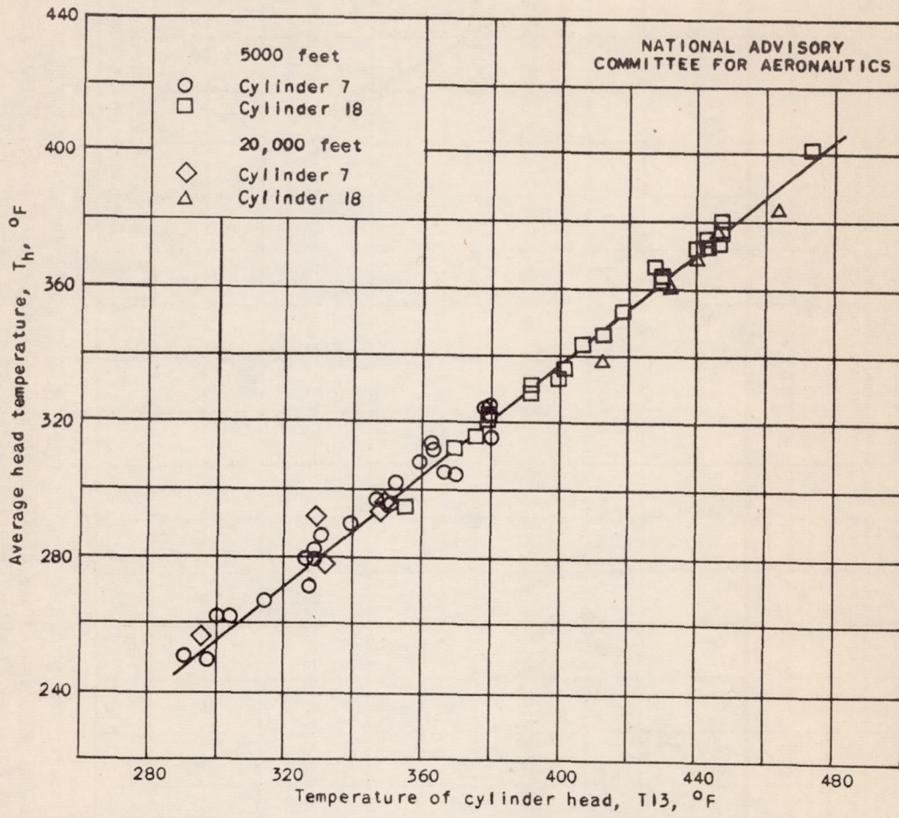
Figure 5. - Variation of average head temperature of cylinders 7 and 18 with cylinder head temperature as measured by thermocouple T13.
