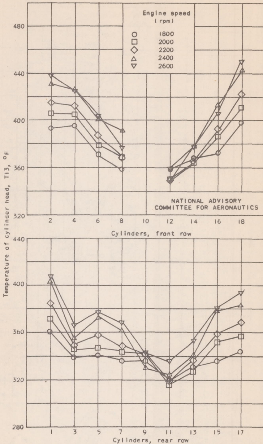
(a) Cylinder-head temperatures.
