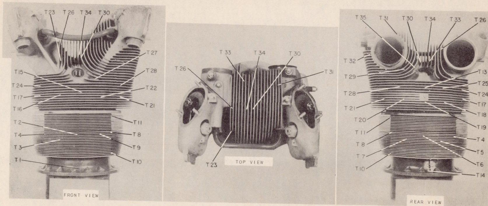
(a) Front-row cylinder 18.
