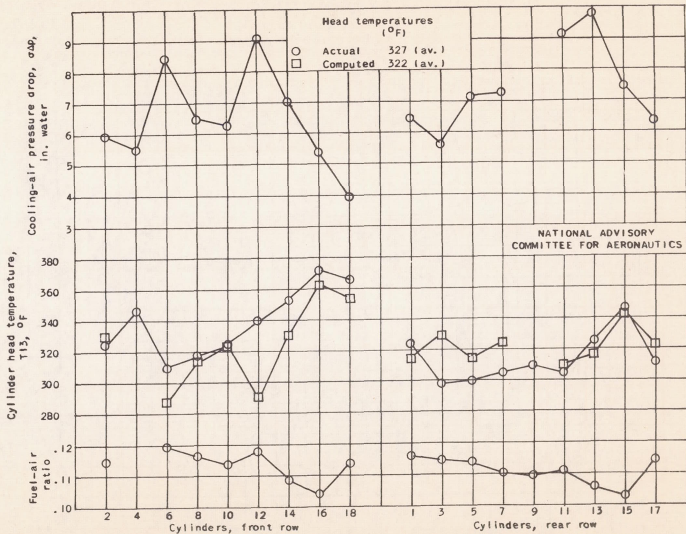
(c) Brake horsepower, 1500; cowl flaps closed; average engine fuel-air ratio, 0.112; impact pressure, 33.0 inches of water; angle of attack of thrust axis, 2^\circ .
