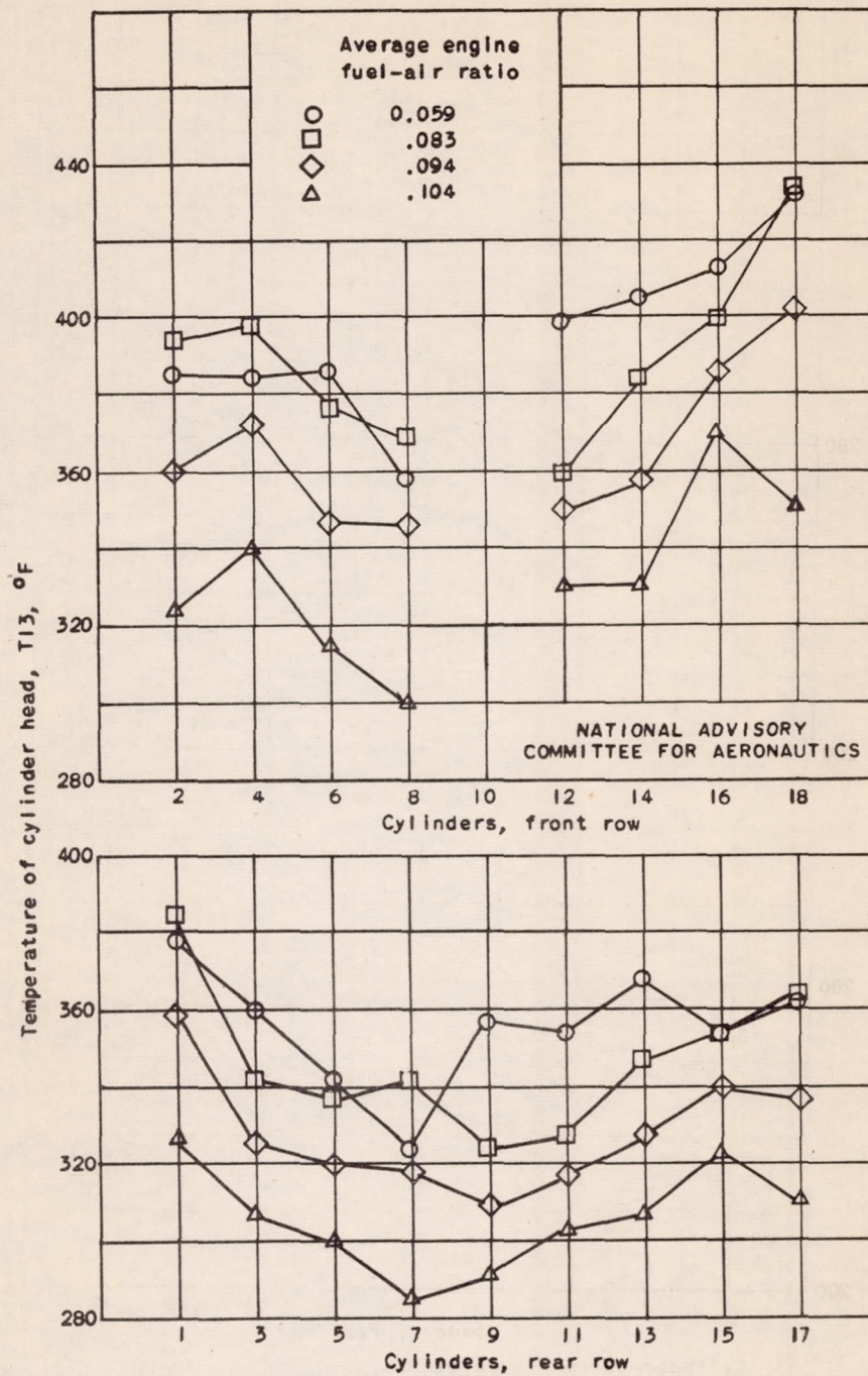
(a) Cylinder-head temperatures.
