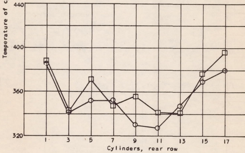
(a) Cylinder-head temperatures.
