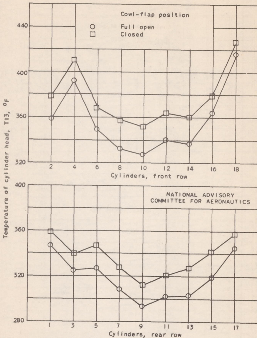
(a) Cylinder-head temperatures.
