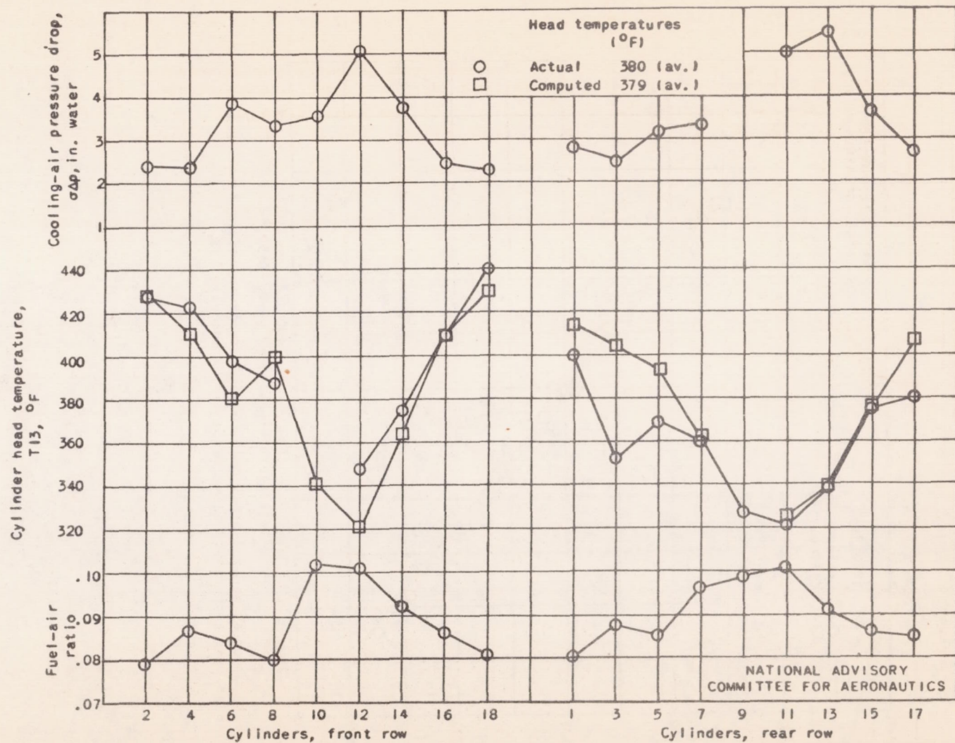
(a) Brake horsepower, 800; cowl flaps closed; average engine fuel-air ratio, 0.082; impact pressure, 16.6 inches of water; angle of attack of thrust axis, 5^\circ .
