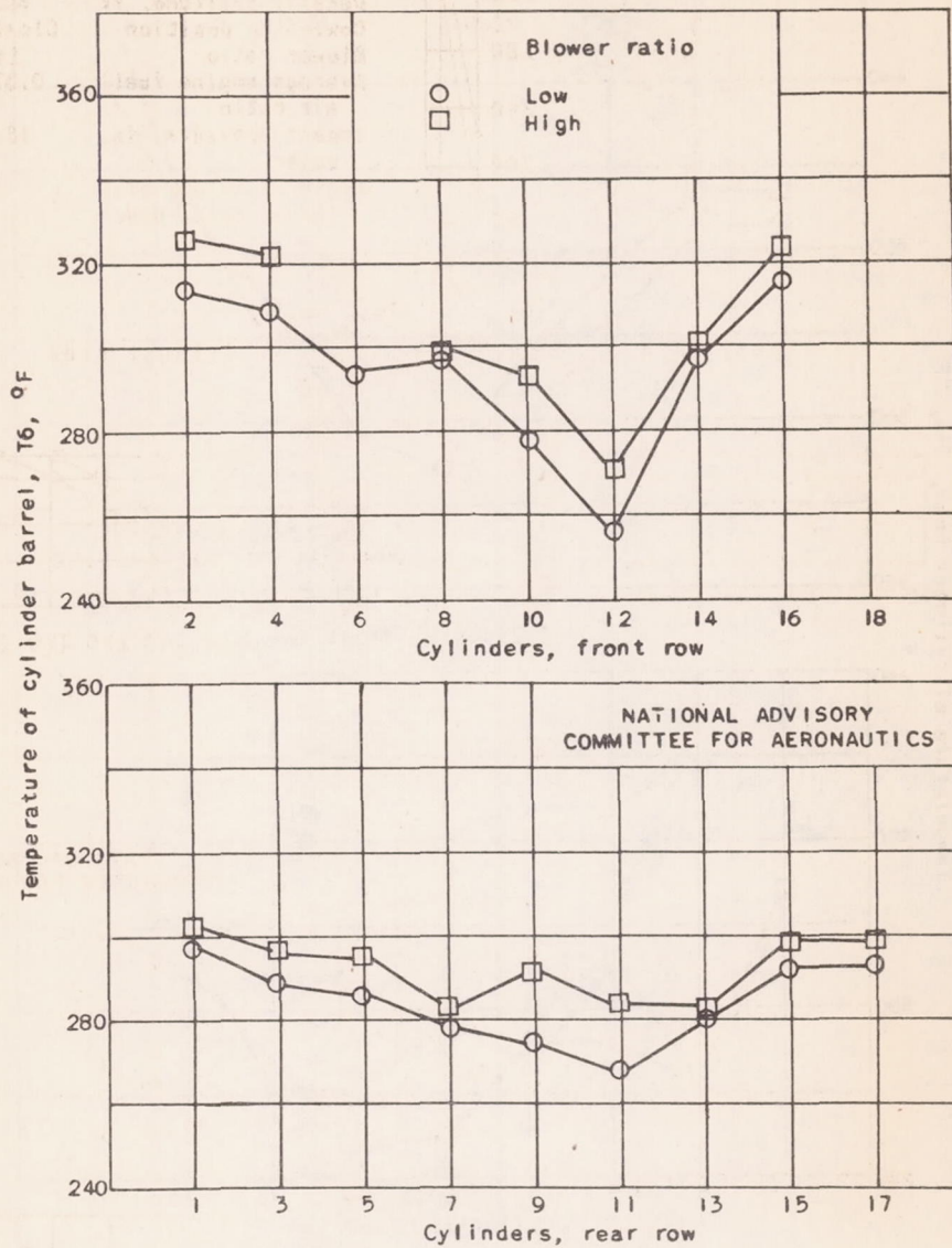
(b) Cylinder-barrel temperatures.
