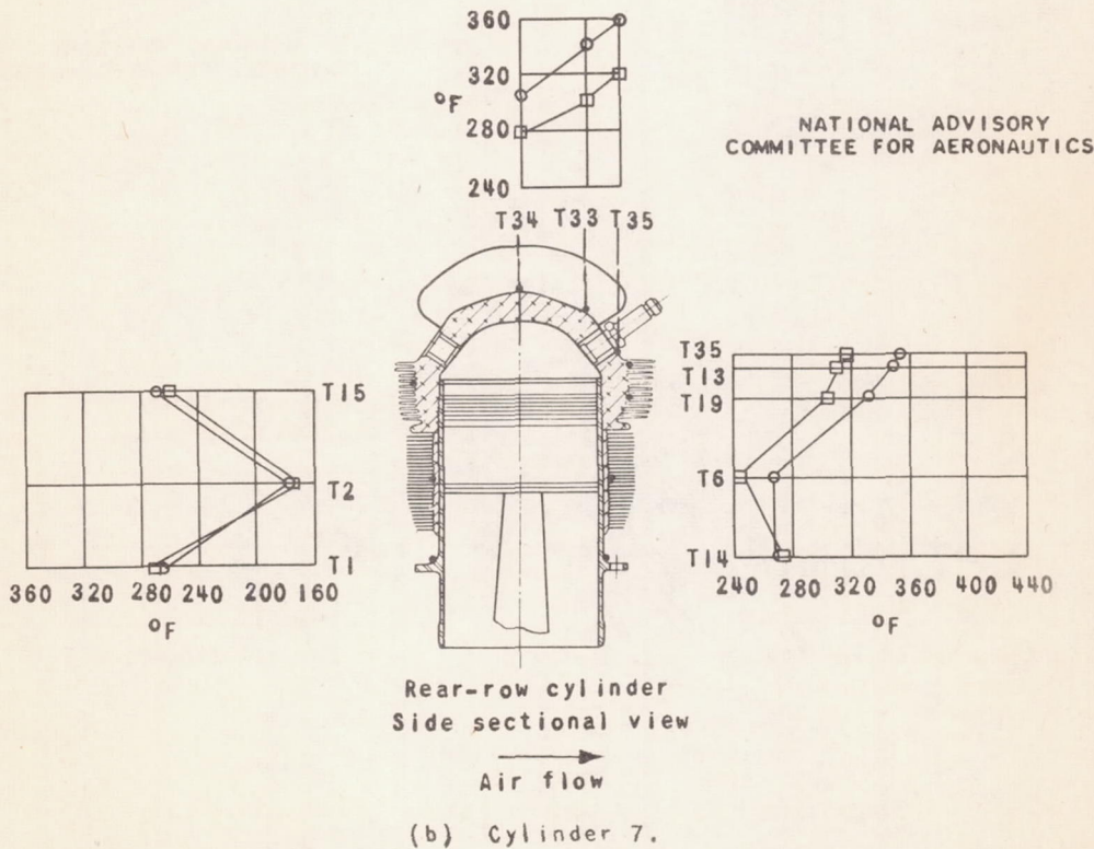
Figure 15. - Concluded. Longitudinal temperature distribution of cylinder.
