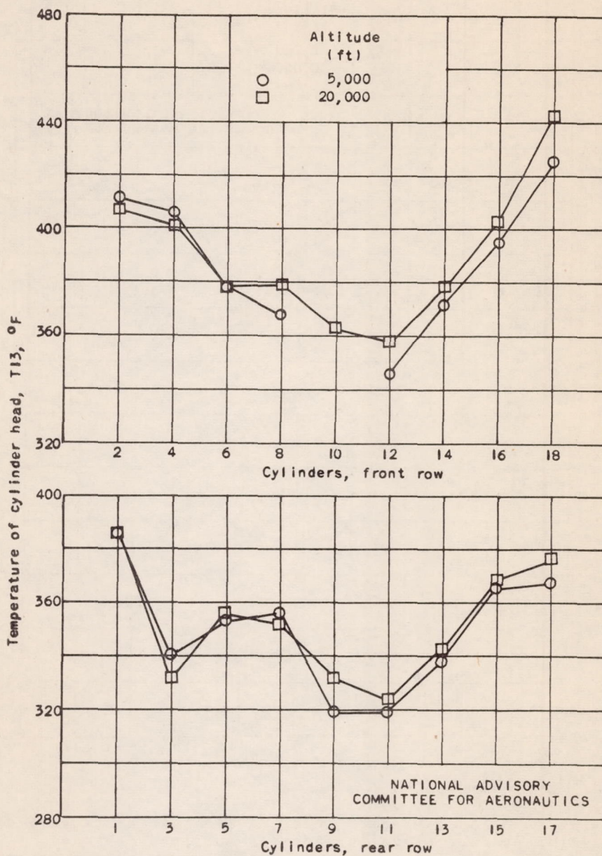
(a) Cylinder-head temperatures.
