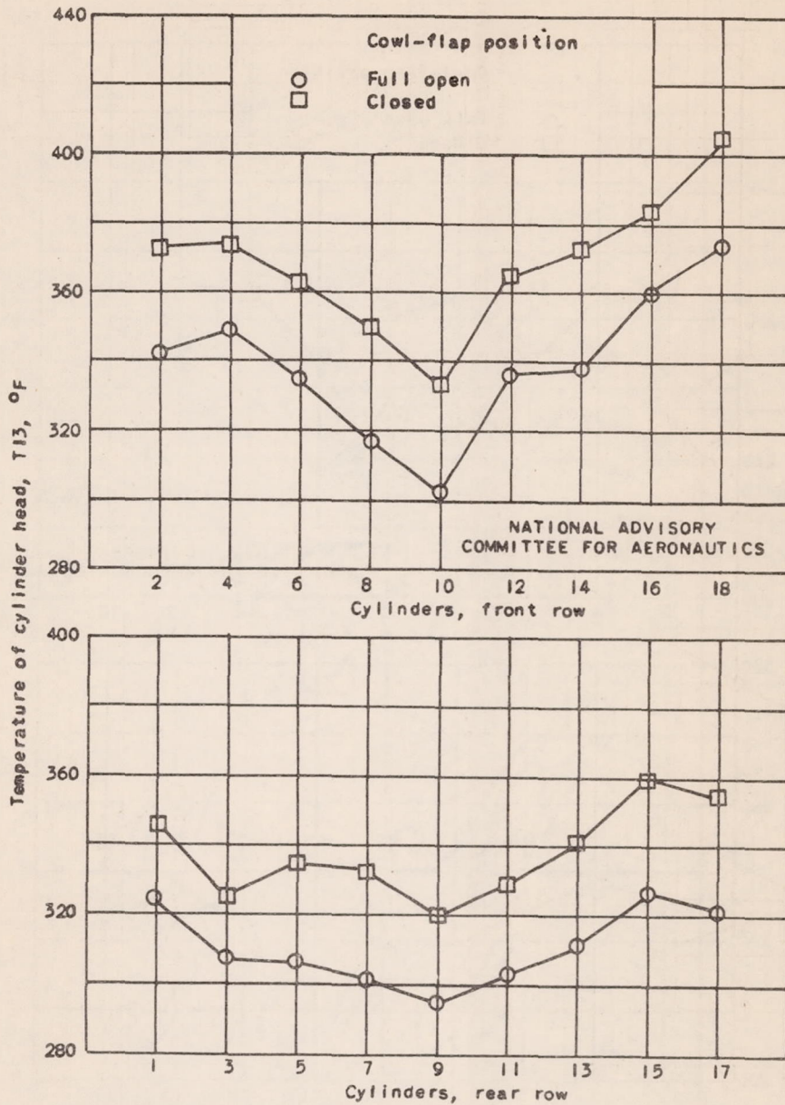
(a) Cylinder-head temperatures.
