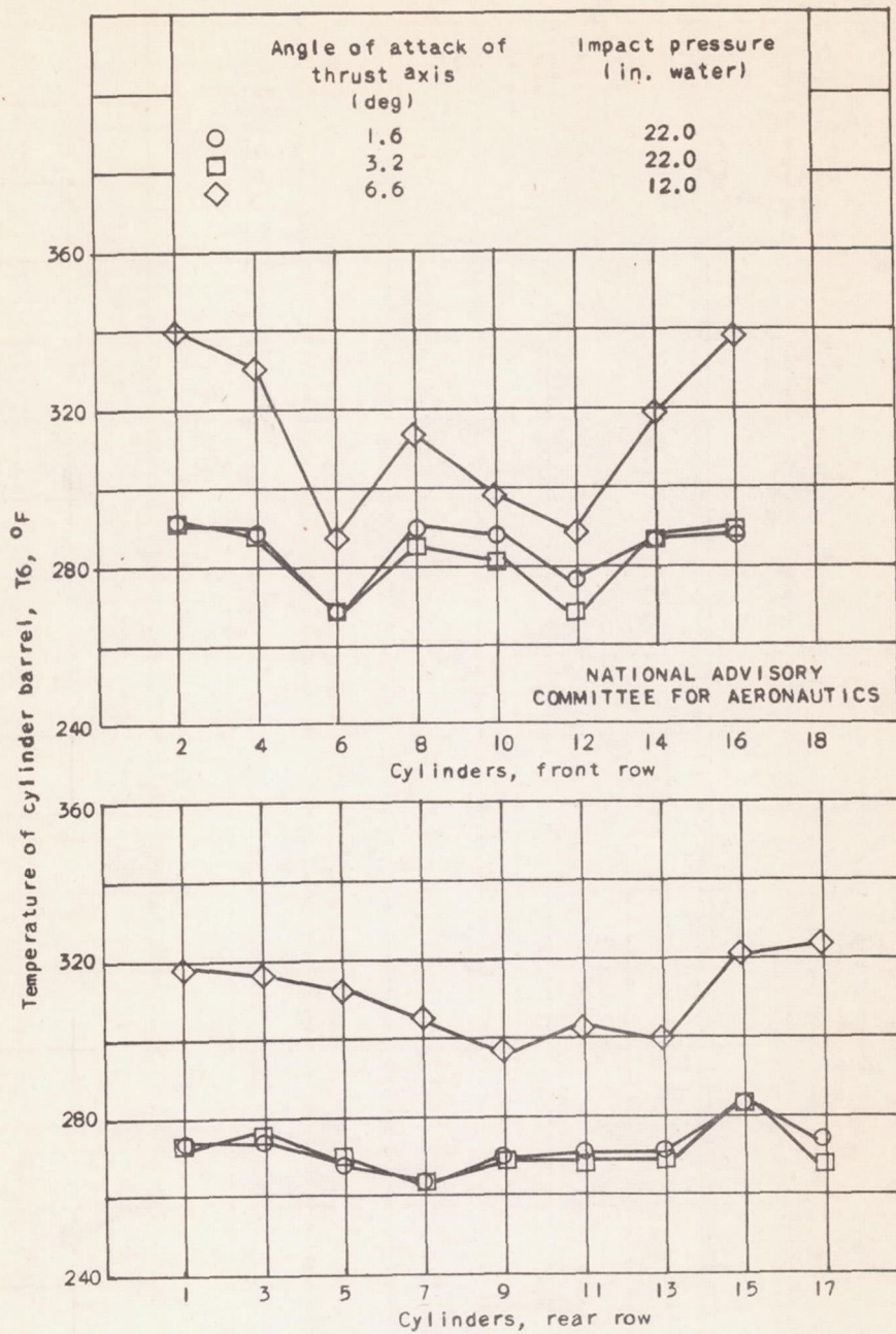
(b) Cylinder-barrel temperatures.
