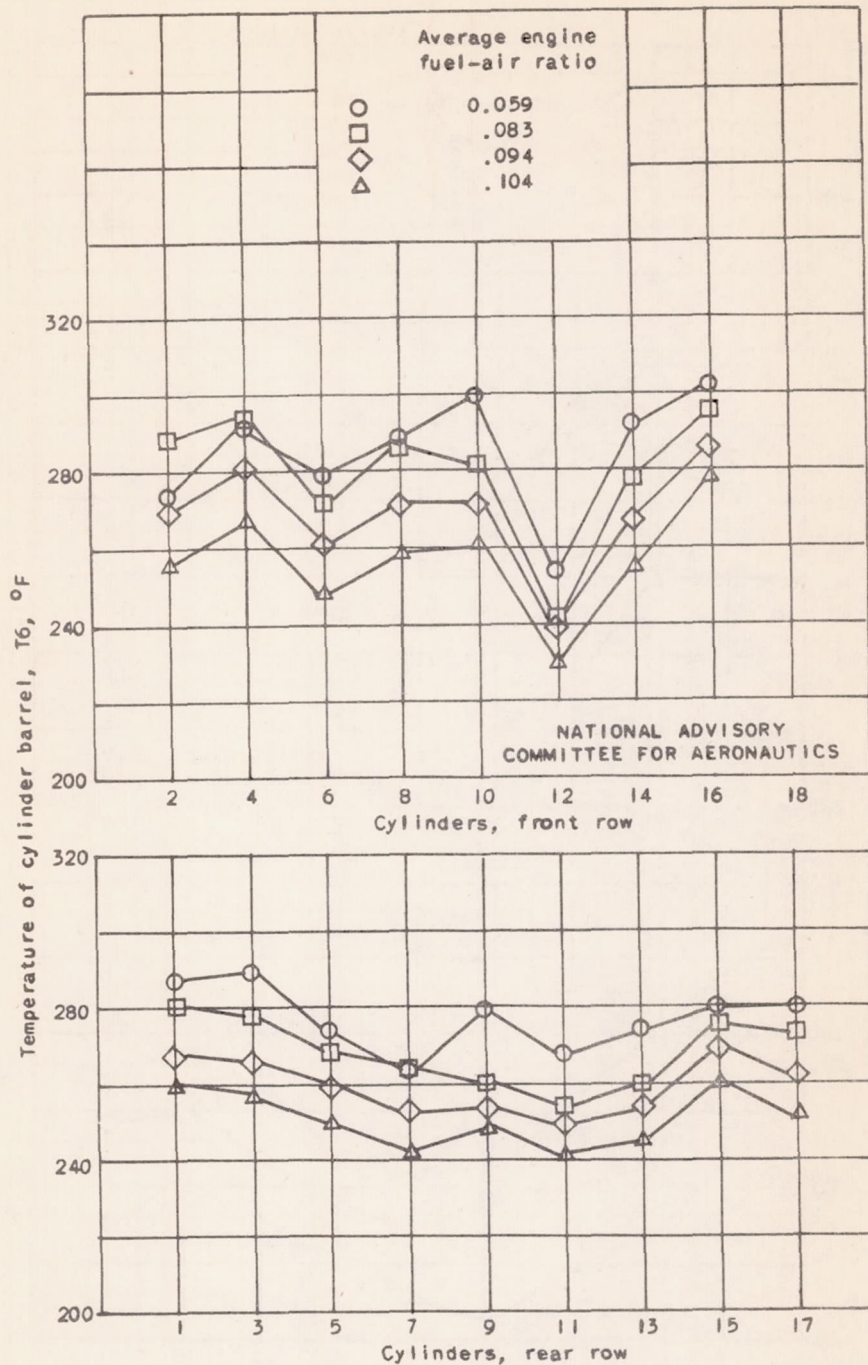
Figure 11. - Concluded. Effect of average engine fuel-air ratio on temperature distribution. Brake horsepower, 1000; engine speed, 2400 rpm; density altitude, 5000 feet; cowl flaps open; low blower ratio; impact pressure, 21 inches of water; angle of attack of thrust axis, 4°.
