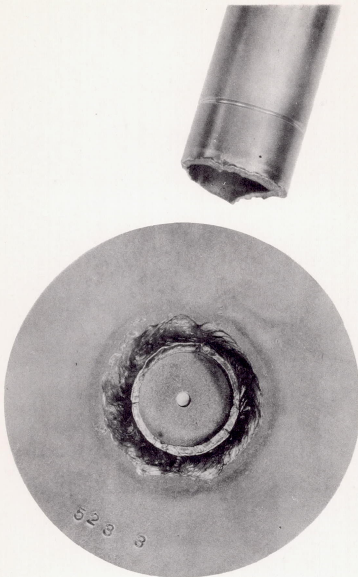
Figure 27.- Typical rotary-bending fatigue failure in arc-welded tube-plate specimen. Specimen shown was notched, but failed at toe of the weld with characteristic fracture.
