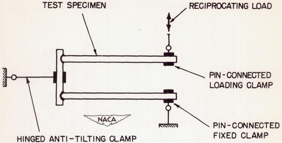
Figure 23.- Schematic diagram of method of loading tubular pi specimens, series H, to produce reversed bending stress (maximum at weld joints). (For specimen dimensions see fig. 20.)
