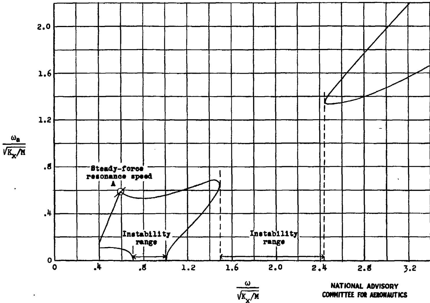
Figure 6.- Principal values of \omega_a plotted against rotor speed \omega for case of \Lambda_1 = 0.1 , \Lambda_2 = 0 , \Lambda_3 = 0.1 , and K_y = \infty .
