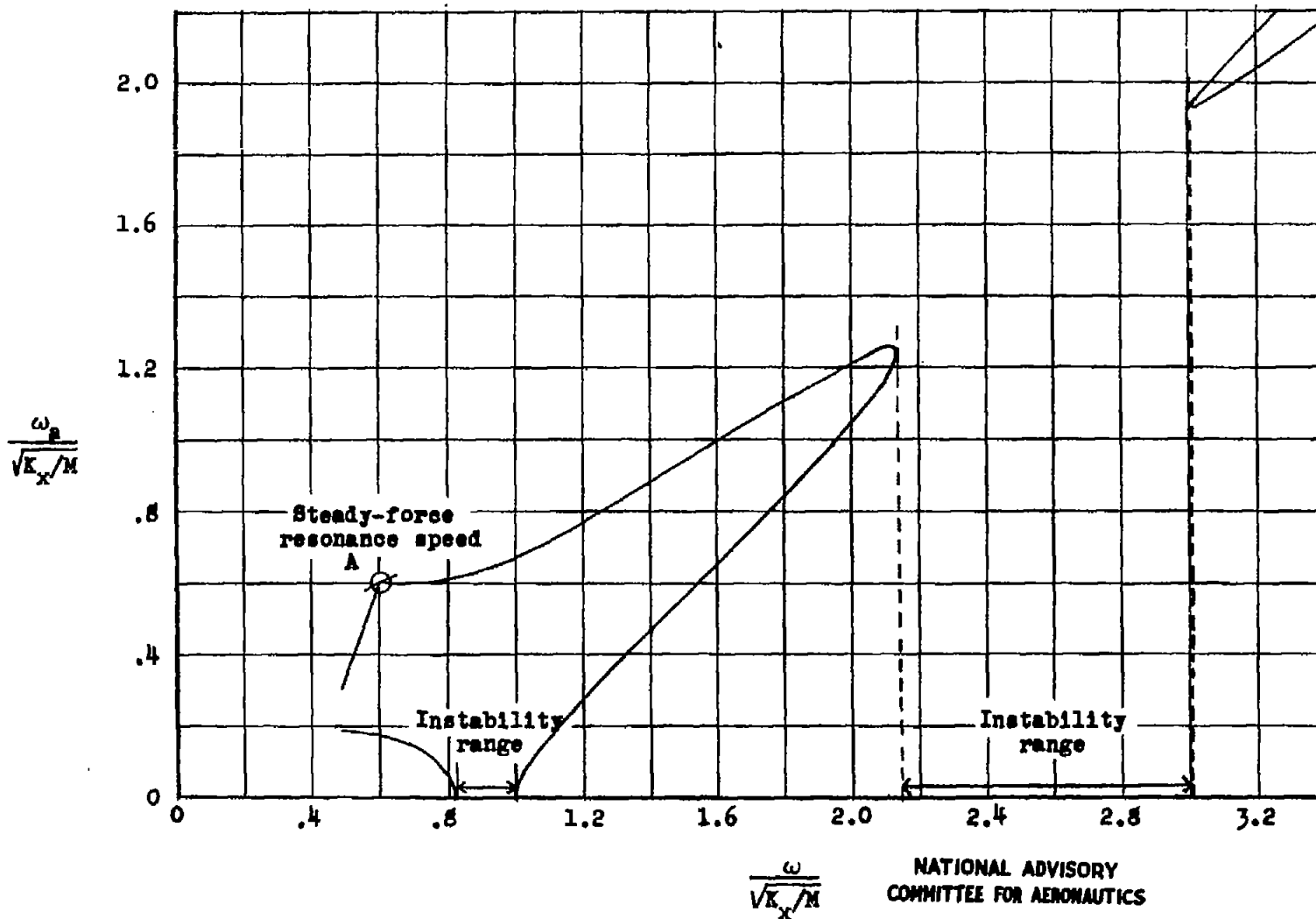
Figure 4.- Principal values of \omega_p plotted against rotor speed \omega for case of \Lambda_1 = 0.1 , \Lambda_2 = 0 , \Lambda_3 = 0.1 , and K_y = 0 .
