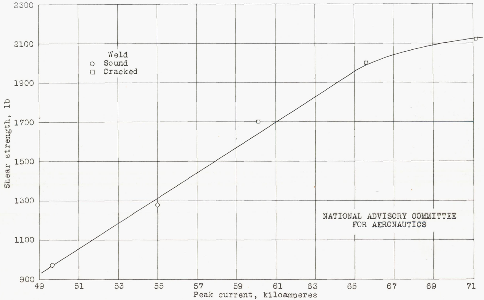
Figure 5.- Strength-current characteristic of Alclad 24S-T. Thickness, 0.081 inch; electrode dome-tip radius, 6 inches; electrode force, 1800 pounds (weld), 4700 pounds (forge); forge timing, 93 milliseconds; average rate of current rise, 1925 amperes per millisecond.
