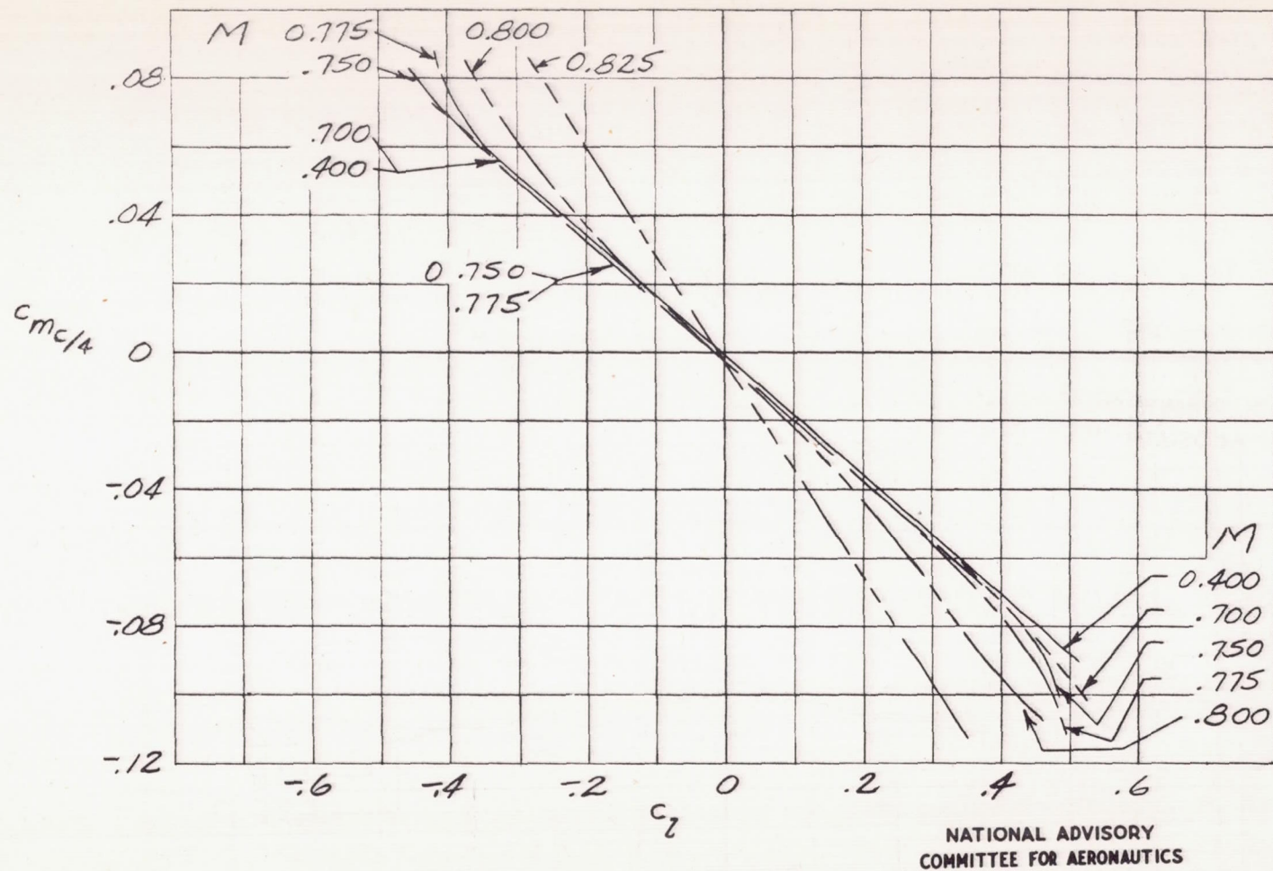
Figure 10.- Variation of section quarter-chord moment coefficient with section lift coefficient for a constant angle of attack. \alpha = 0^\circ .
