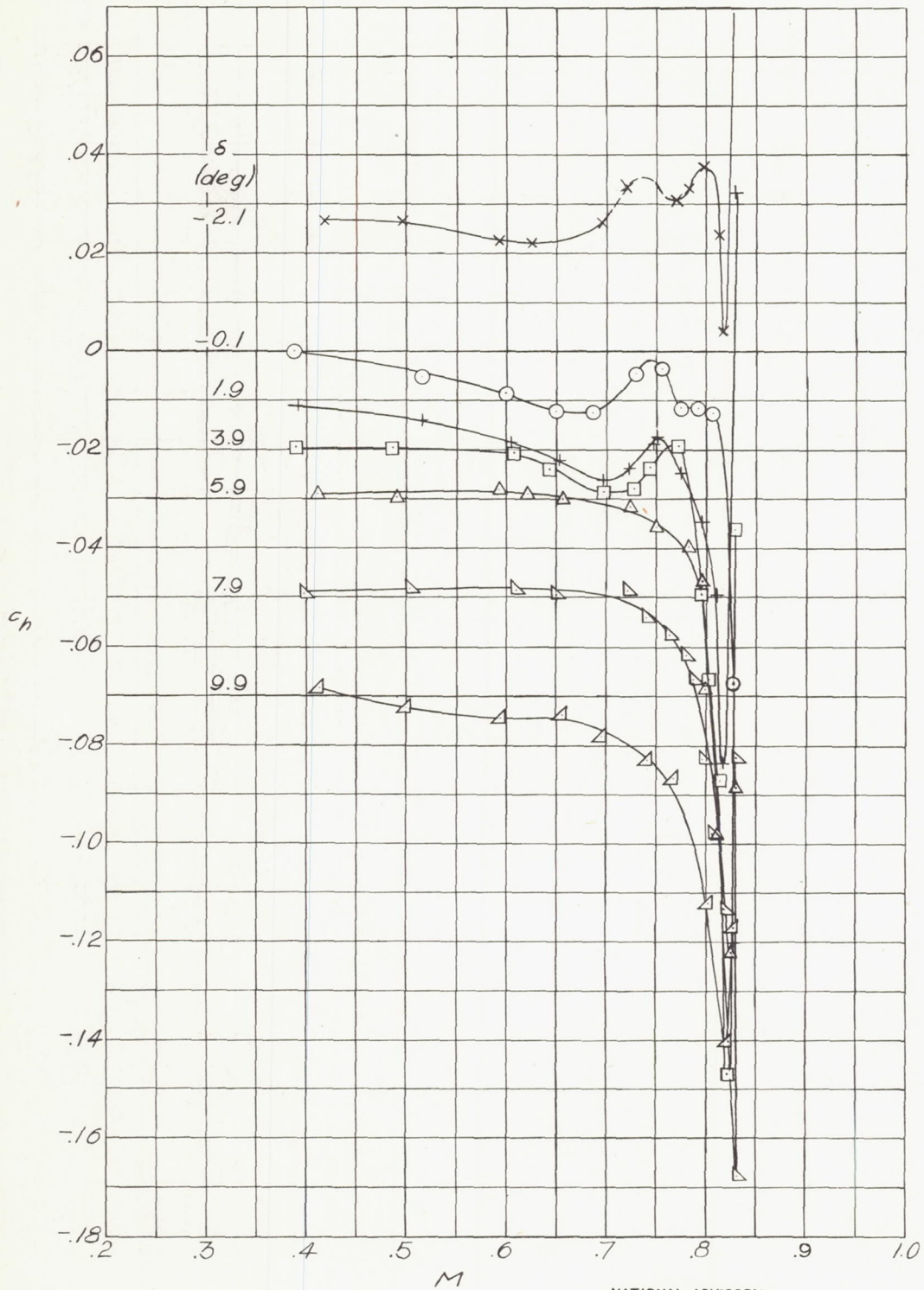
Figure 13. - Variation of flap section hinge-moment coefficient with Mach number.
