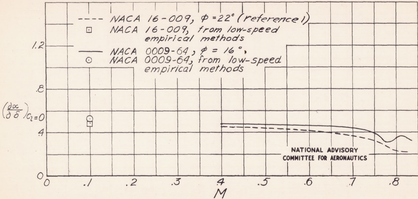
Figure 7. - Variation of flap effectiveness with Mach number.
