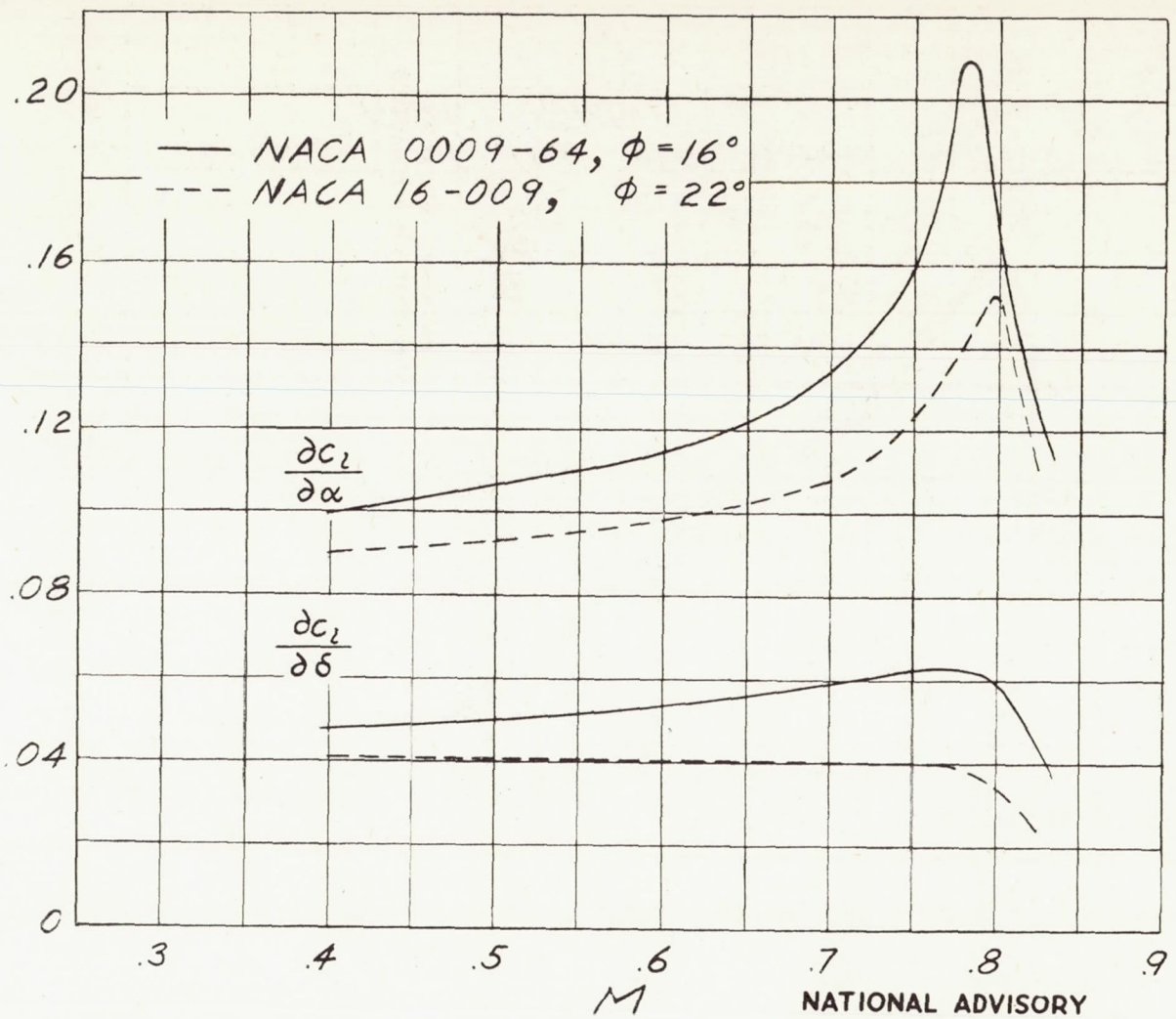
Figure 6. - Variation of lift curve slopes with Mach number.
