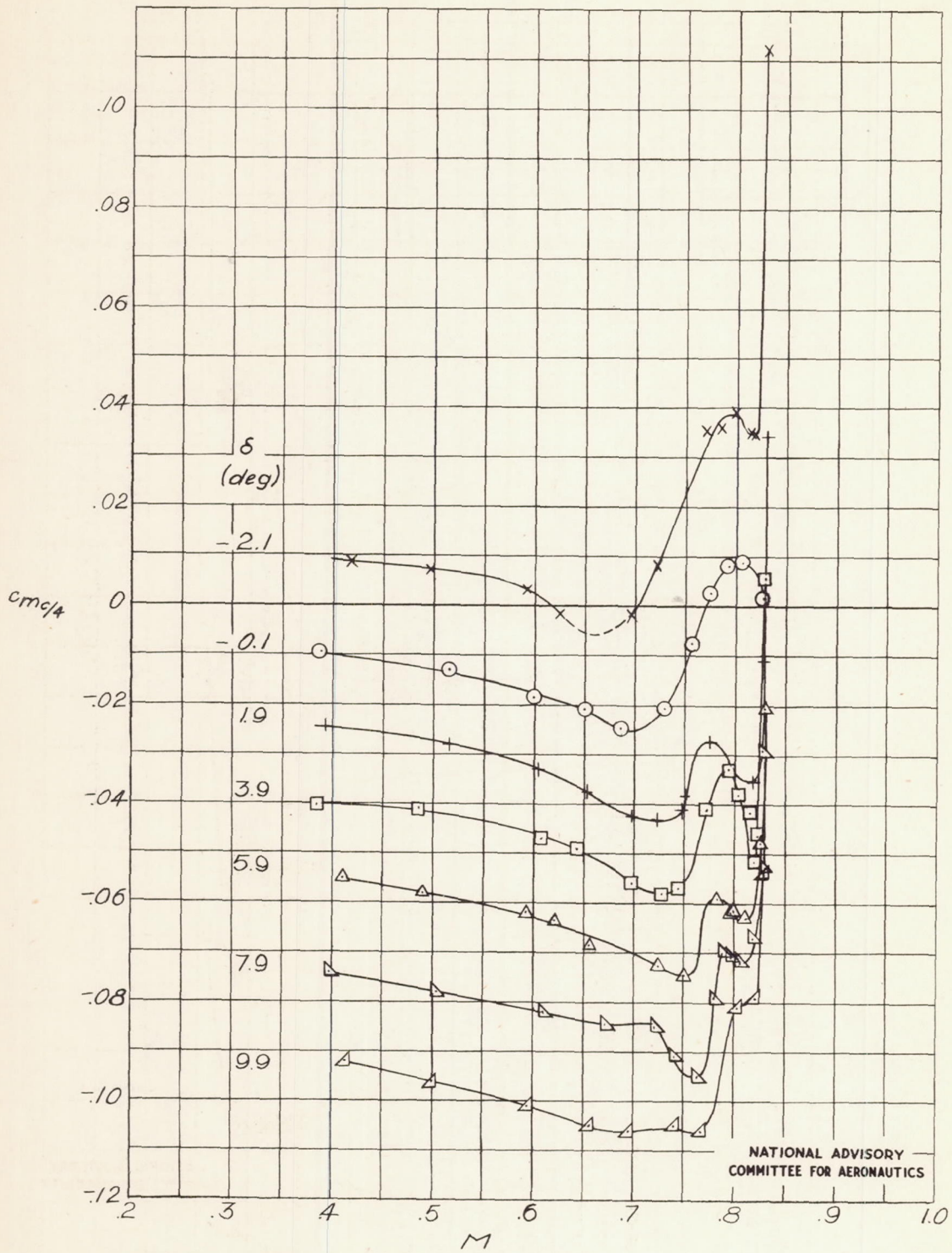
Figure 8. - Variation of section quarter-chord moment coefficient with Mach number.
