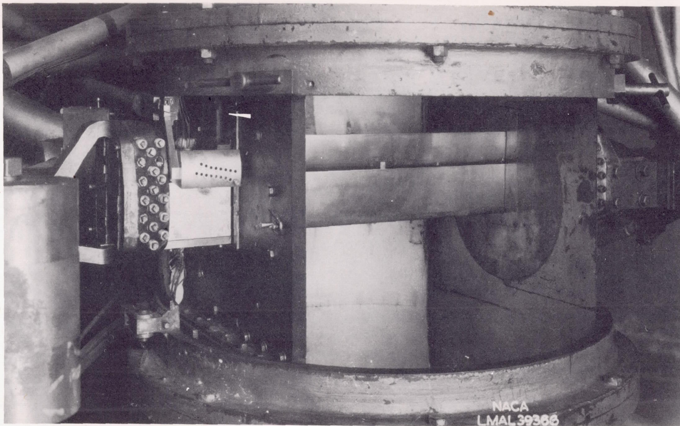
Figure 1.- Langley 24-inch high-speed tunnel test section with model mounted in balance.
