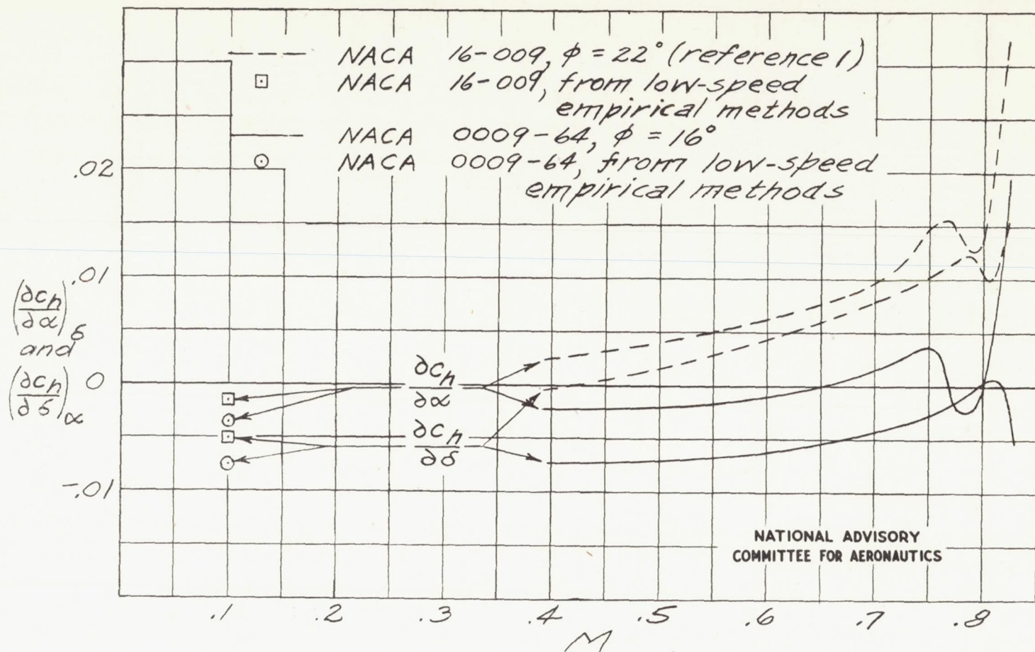
Figure 16. - Variation of hinge-moment parameters with Mach number. \alpha = 0^\circ ; \delta = -0.1^\circ
