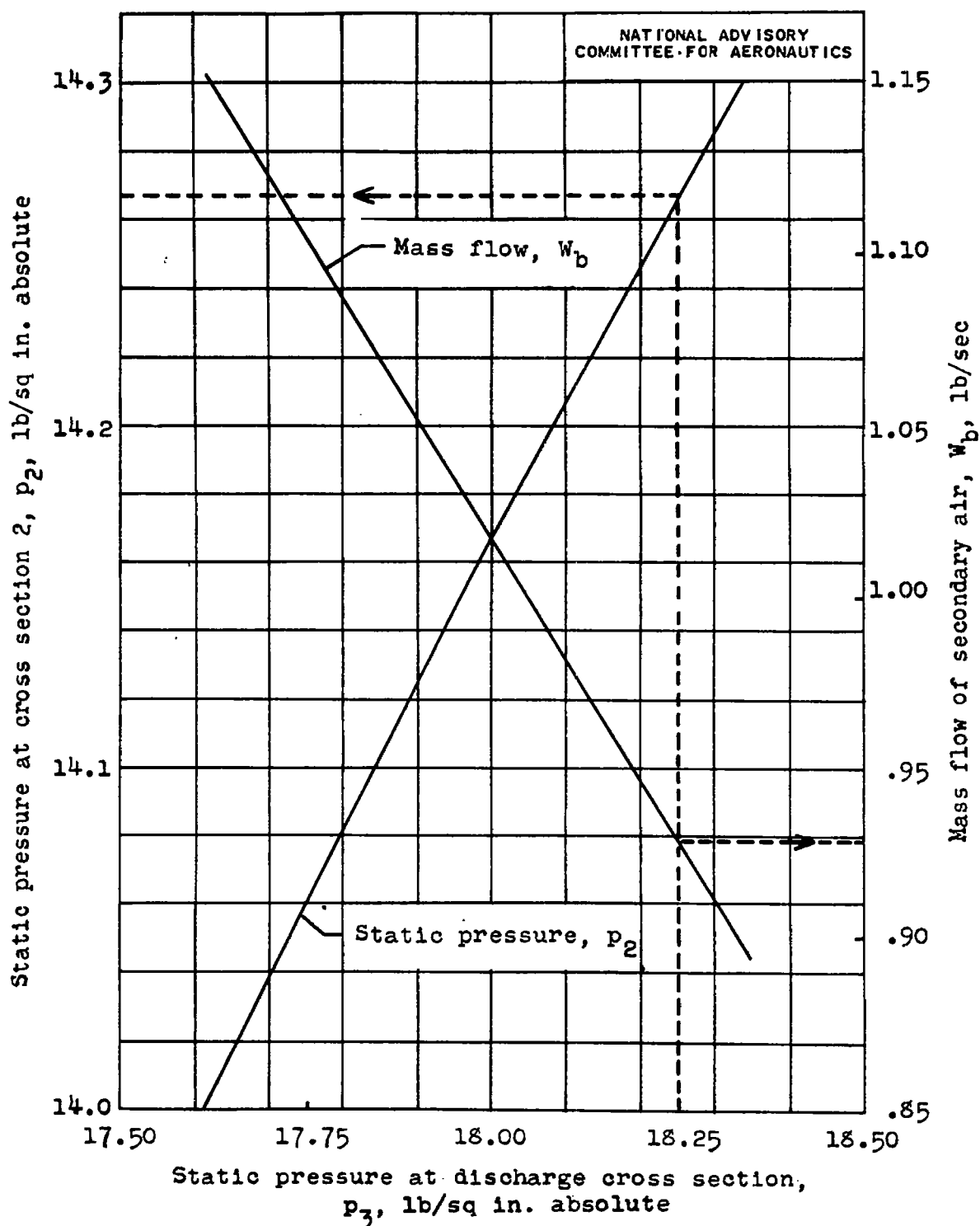
Figure 9. - Effect of static pressure at discharge cross section p_3 on static pressure p_2 at cross section 2 and mass flow of secondary air W_b for jet pump.
