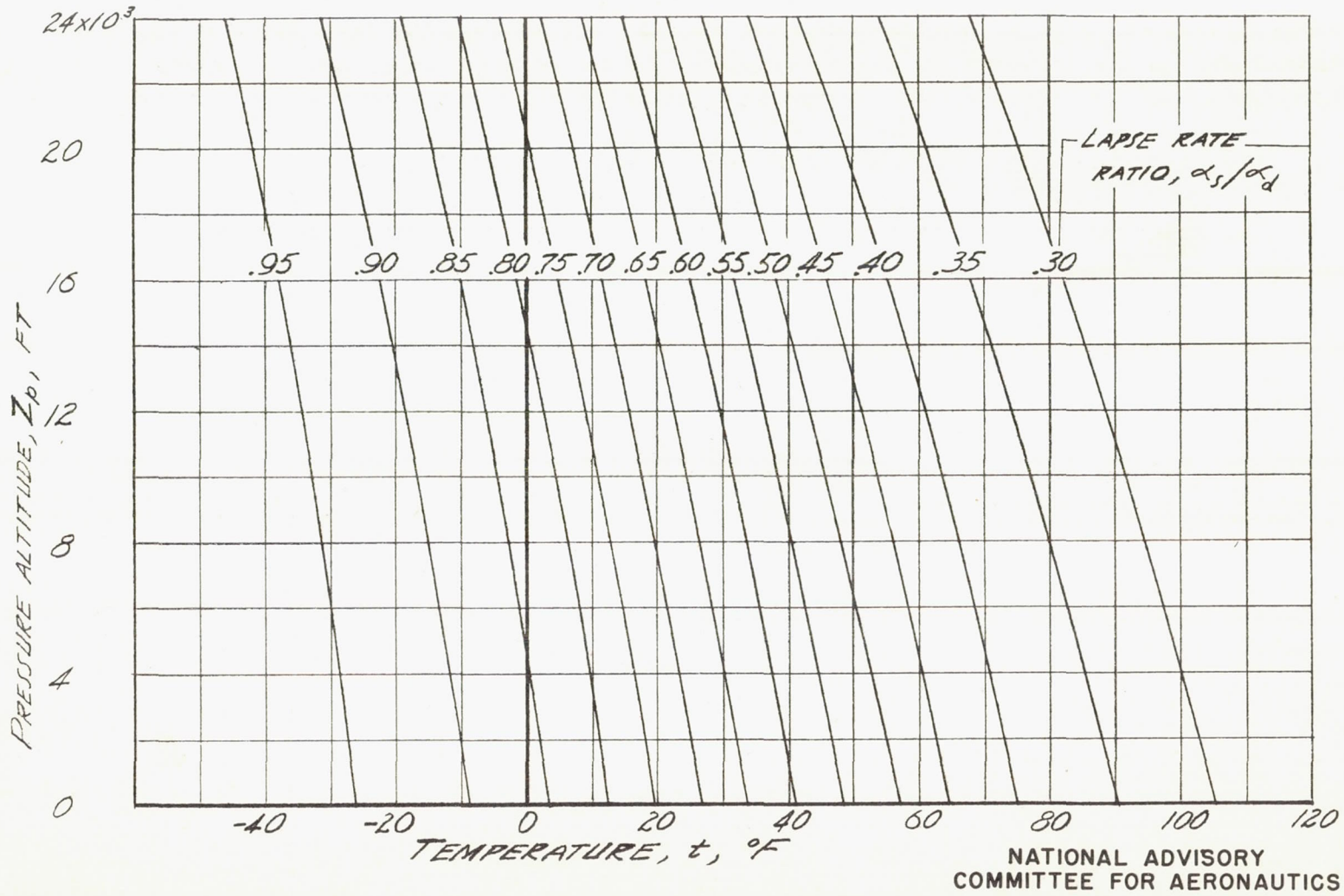
FIGURE 4.- RATIO OF SATURATED- TO DRY-ADIABATIC LAPSE RATES AS A FUNCTION OF TEMPERATURE AND PRESSURE ALTITUDE.
