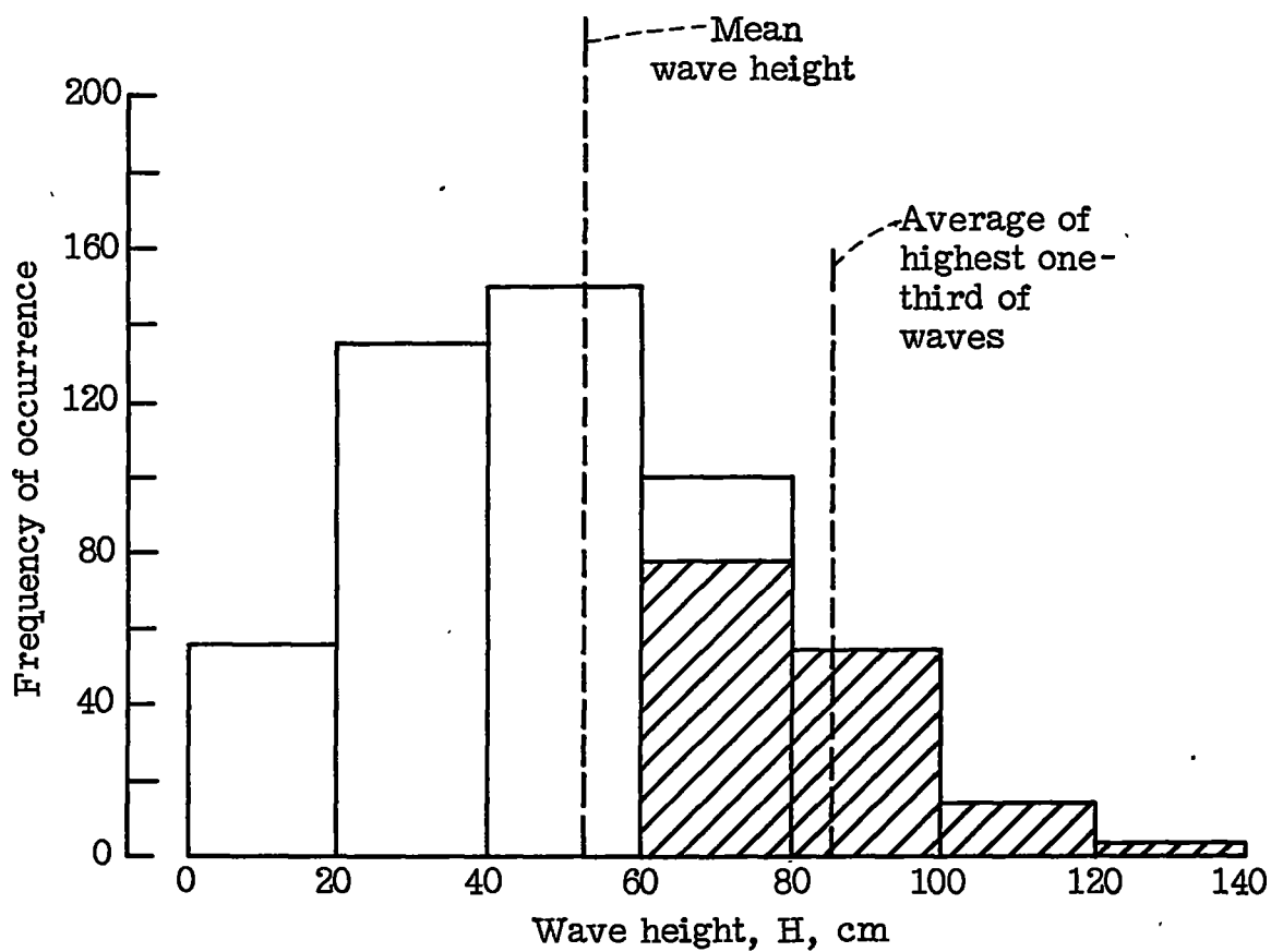
Figure 1.- Frequency distribution of wave heights of sea from German analysis of 517 waves (reference 1). Shaded area refers to highest one-third of waves.
