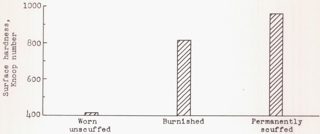
Figure 8. - Relation between hardness and surface condition of chrome-plated cast-iron rider specimen.
