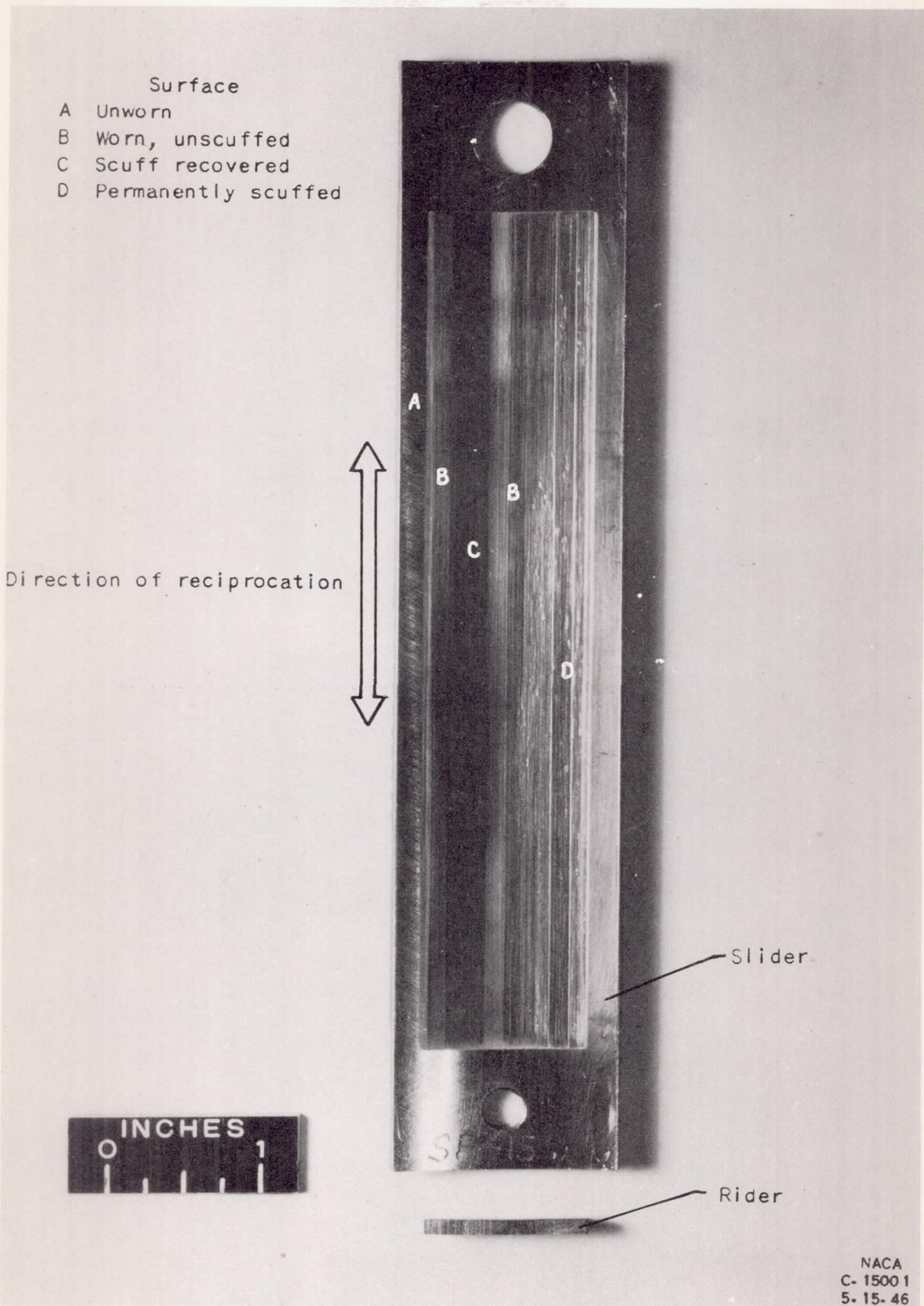
Figure 2. - Run-in and scuffed SAE 4140 steel slider and cast-iron rider showing types of surface on slider.
