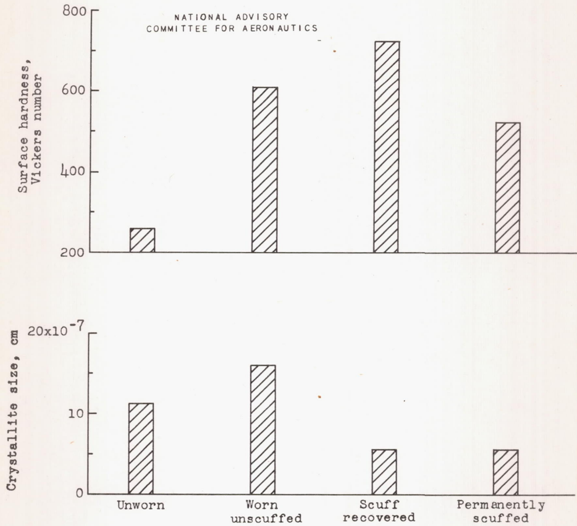
Figure 4. - Relation between surface changes and surface condition of SAE 4140 steel slider specimens.
