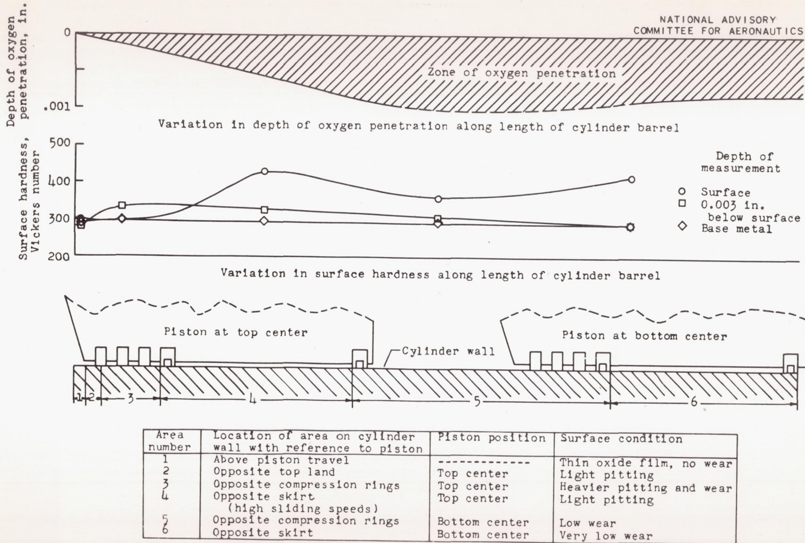
Figure 6. - Relations among surface condition, material hardness, and depth of oxygen penetration found on worn - unscuffed SAE 4140 steel aircraft-engine cylinder barrel.
