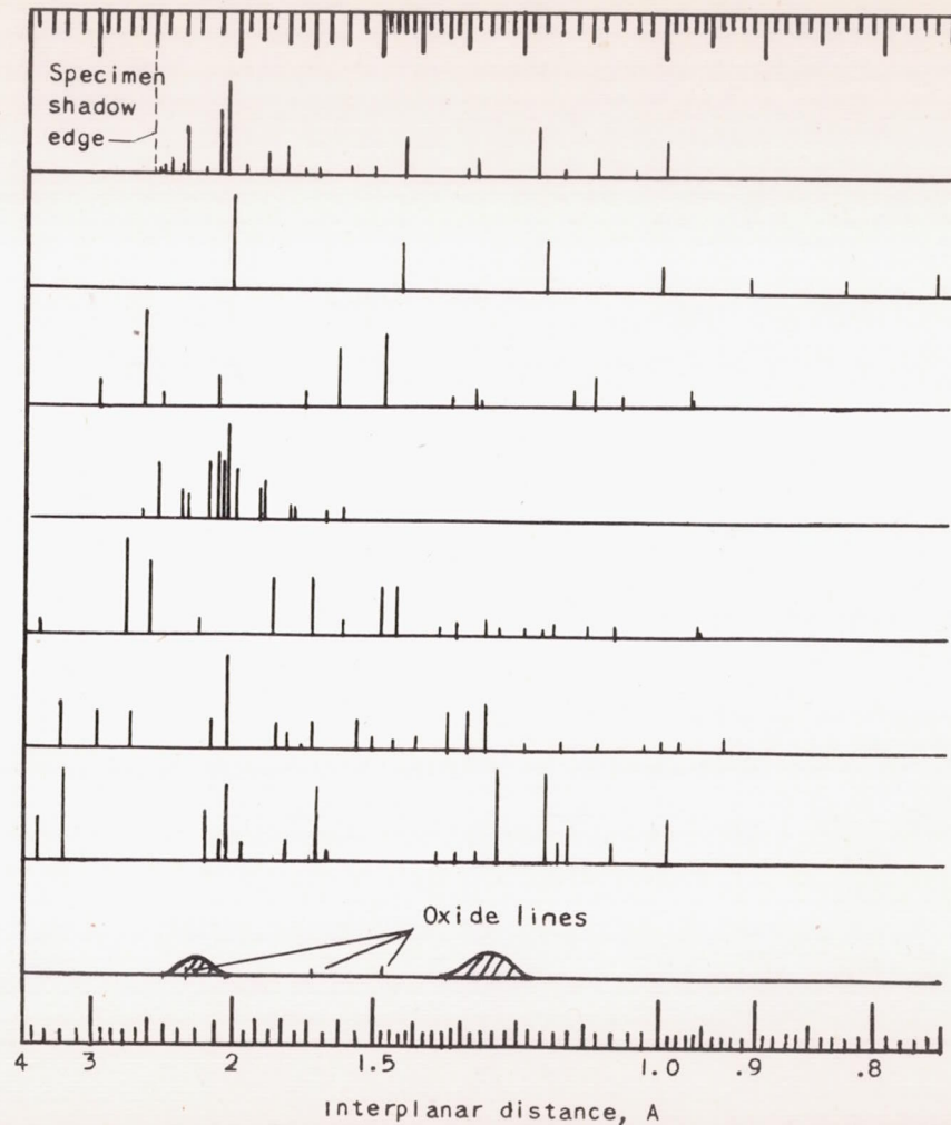
Figure 3. - Typical electron and X-ray diffraction patterns from surfaces of specimens of SAE 4140 steel slider and aircraft-engine cylinder barrel and standard X-ray diffraction patterns of materials identified.
