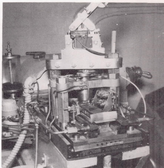
Detail of rider-loading mechanism
