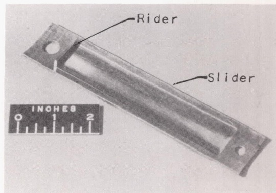
Typical specimens: rider and slider
