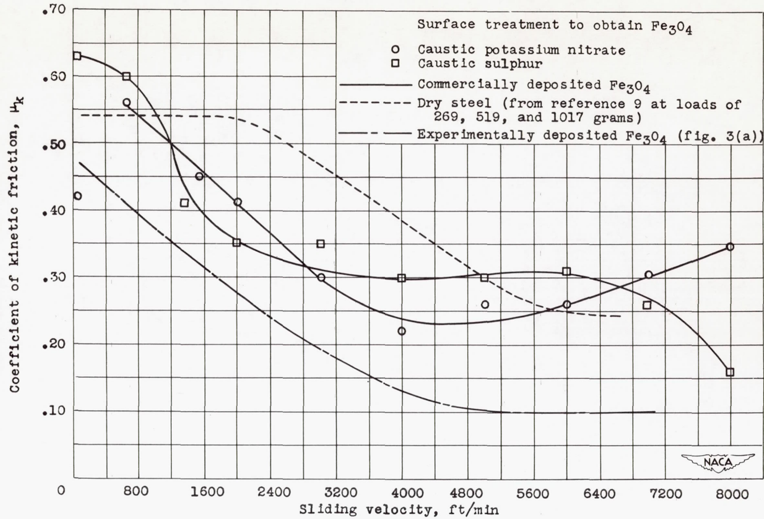
Figure 5. - Effect of sliding velocity on friction for surfaces with solid films of ferrous-ferrous oxide Fe 3 O 4 formed by commercial (caustic soda) treatments. Load, 269 grams. Friction essentially independent of load.
