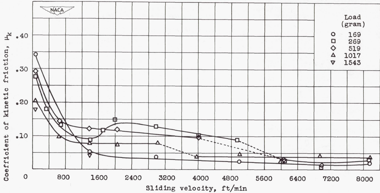
(a) Ferrous-chloride FeCl_2 film showing effect of various loads on friction.
