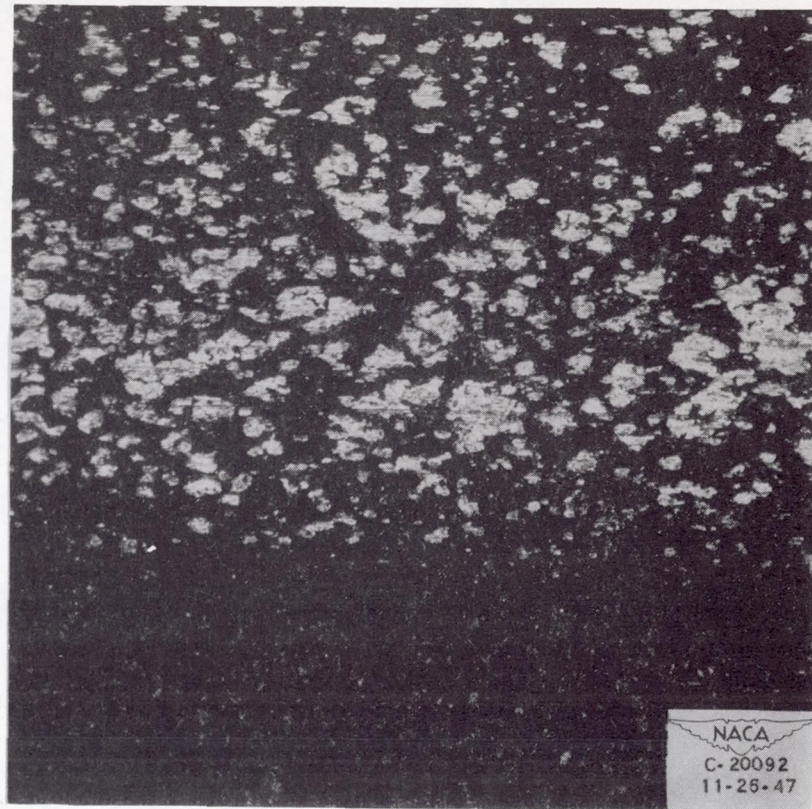
(b) Wear track on disk specimen treated in caustic-sulphur solution to form film of ferrous-ferric oxide \text{Fe}_3\text{O}_4 . (Mating surface shown in fig. 6(a).)
