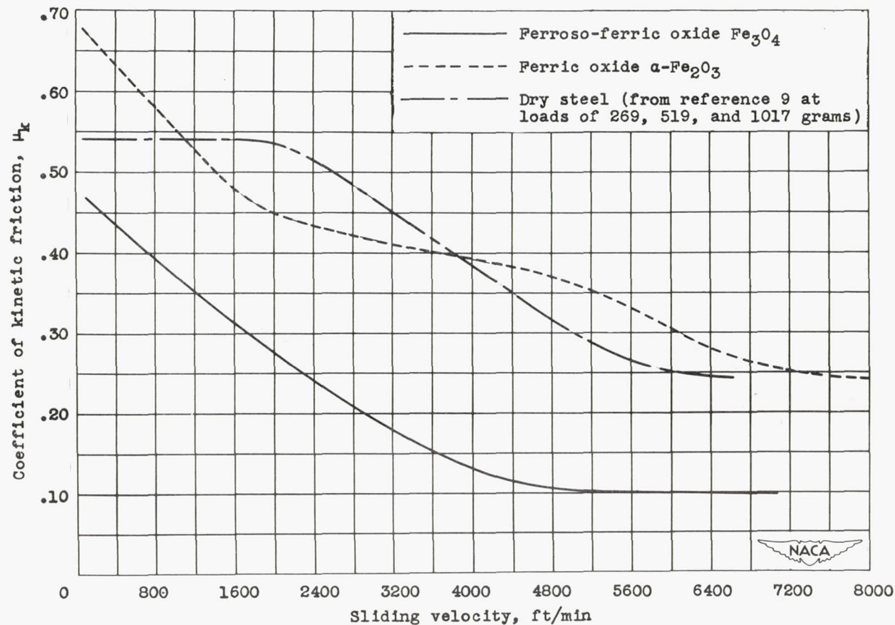
(d) Ferroso-ferric-oxide \text{Fe}_3\text{O}_4 and ferric-oxide \alpha\text{-Fe}_2\text{O}_3 films with loads of 269 grams.
