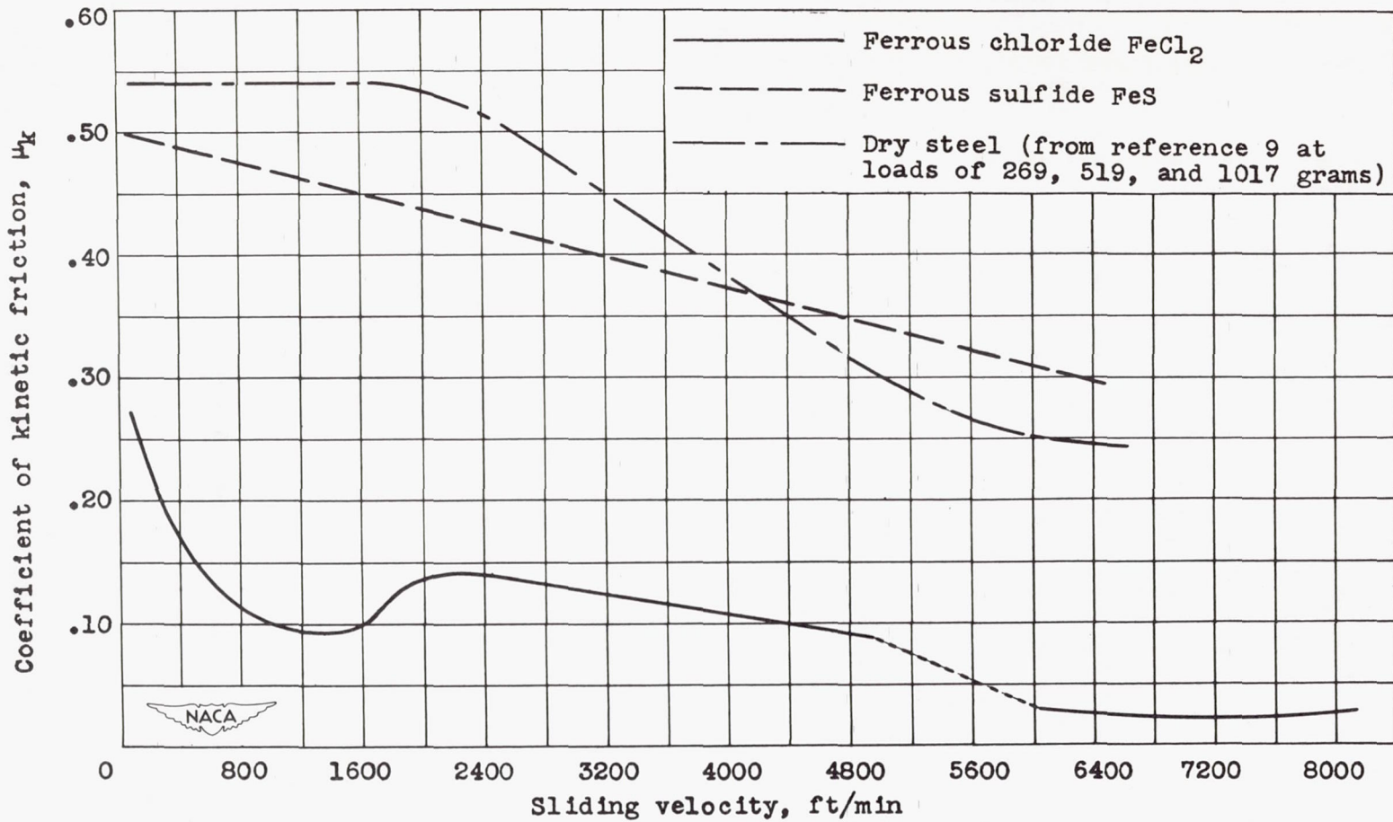
(c) Ferrous-chloride \text{FeCl}_2 and ferrous-sulfide \text{FeS} films with loads of 269 grams.
