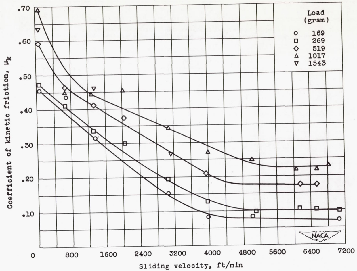
(a) Ferrous-ferric oxide Fe_3O_4 film showing that friction is not independent of load.
