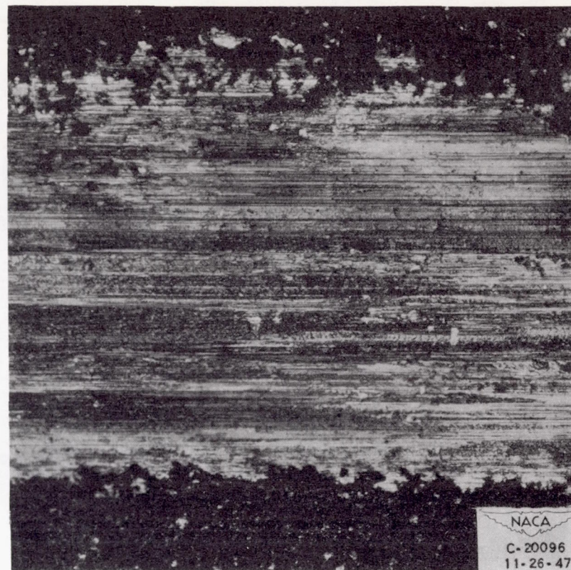
(b) Wear track on disk specimen with molybdenum-disulfide \text{MoS}_2 film. (Mating surface shown in fig. 10(a).)
