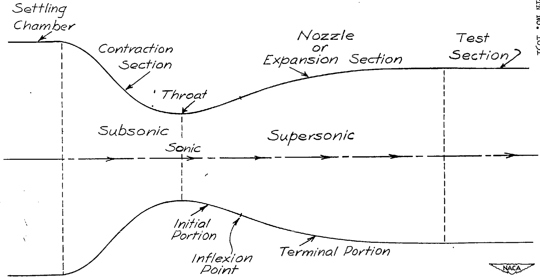
Figure 1.- Section of supersonic wind tunnel showing relative position of nozzle.
