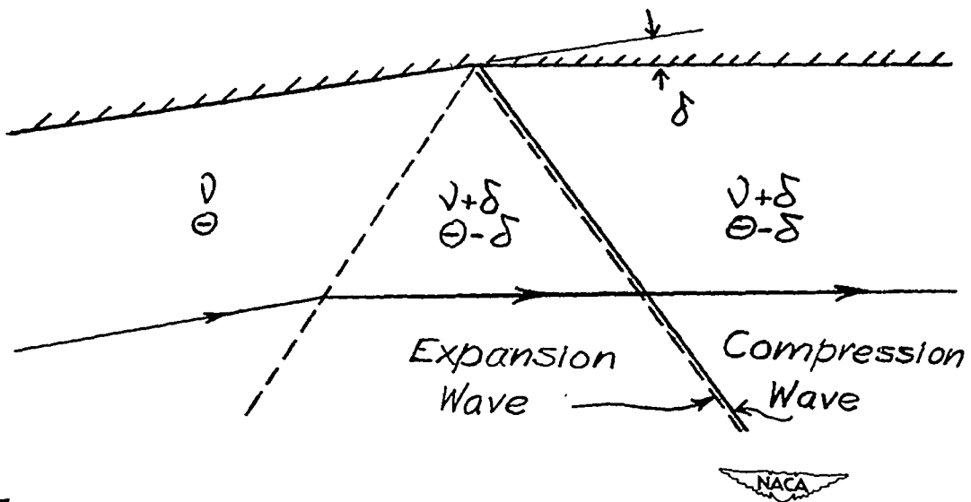
Figure 7.- Neutralization of an expansion wave of strength \delta .
