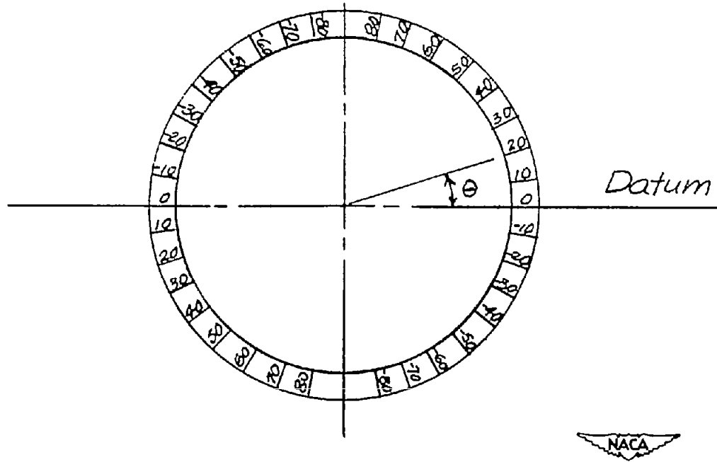
Figure 16.- Lower half of supersonic protractor.
