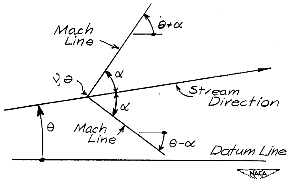
Figure 14.- Mach lines from a point disturbance.
