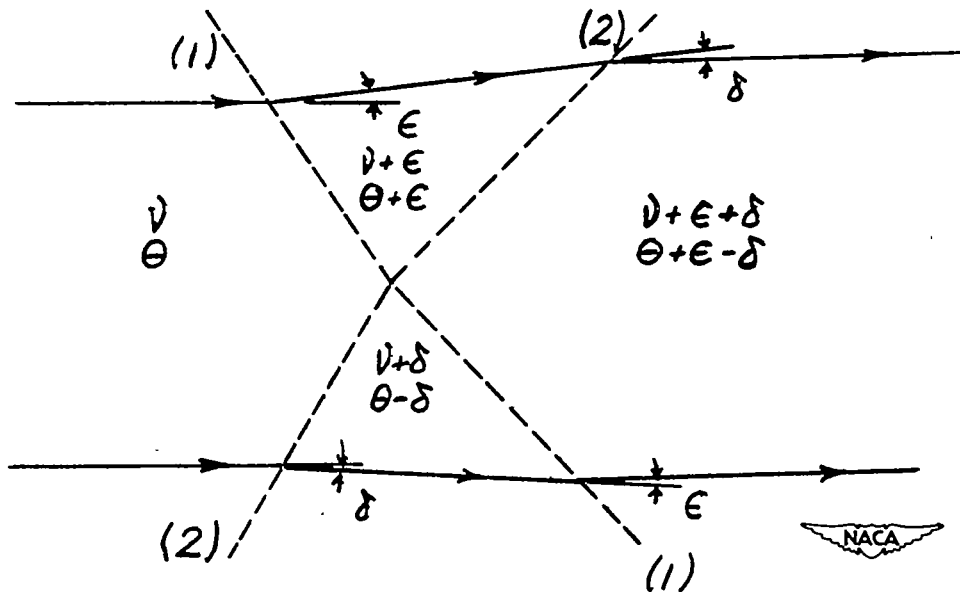
Figure 5.- Intersection of two expansion waves.
