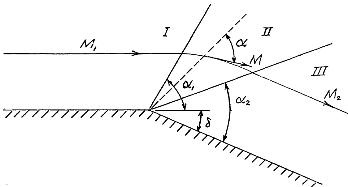
Figure 2.- Supersonic flow about a corner.
