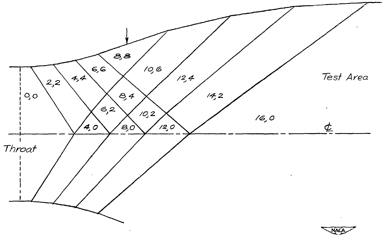
Figure 8.- Flow field in a nozzle with no waves reflected.
