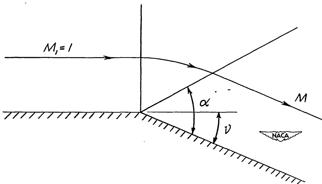
Figure 3.- Supersonic flow about a corner from an initial Mach number of unity.
