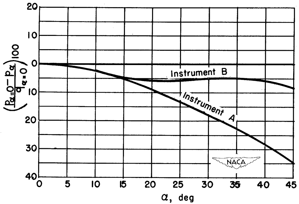
Figure 4.- Pitot-static-tube characteristics.
