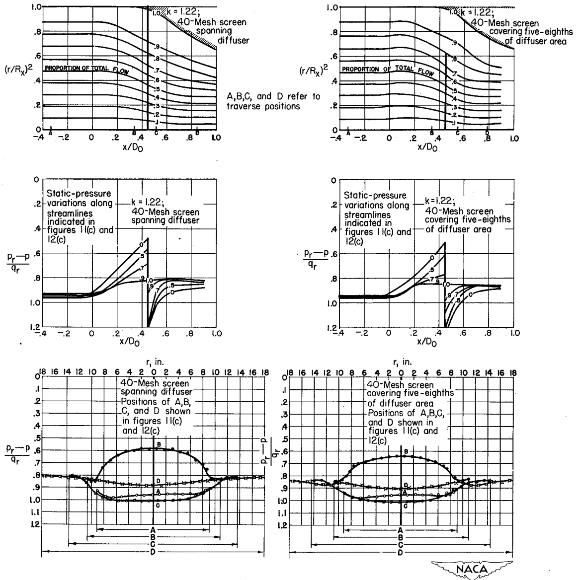
(c) Single 40-mesh screen placed 0.45 duct diameter from diffuser entrance. (See fig. 11(c).)
