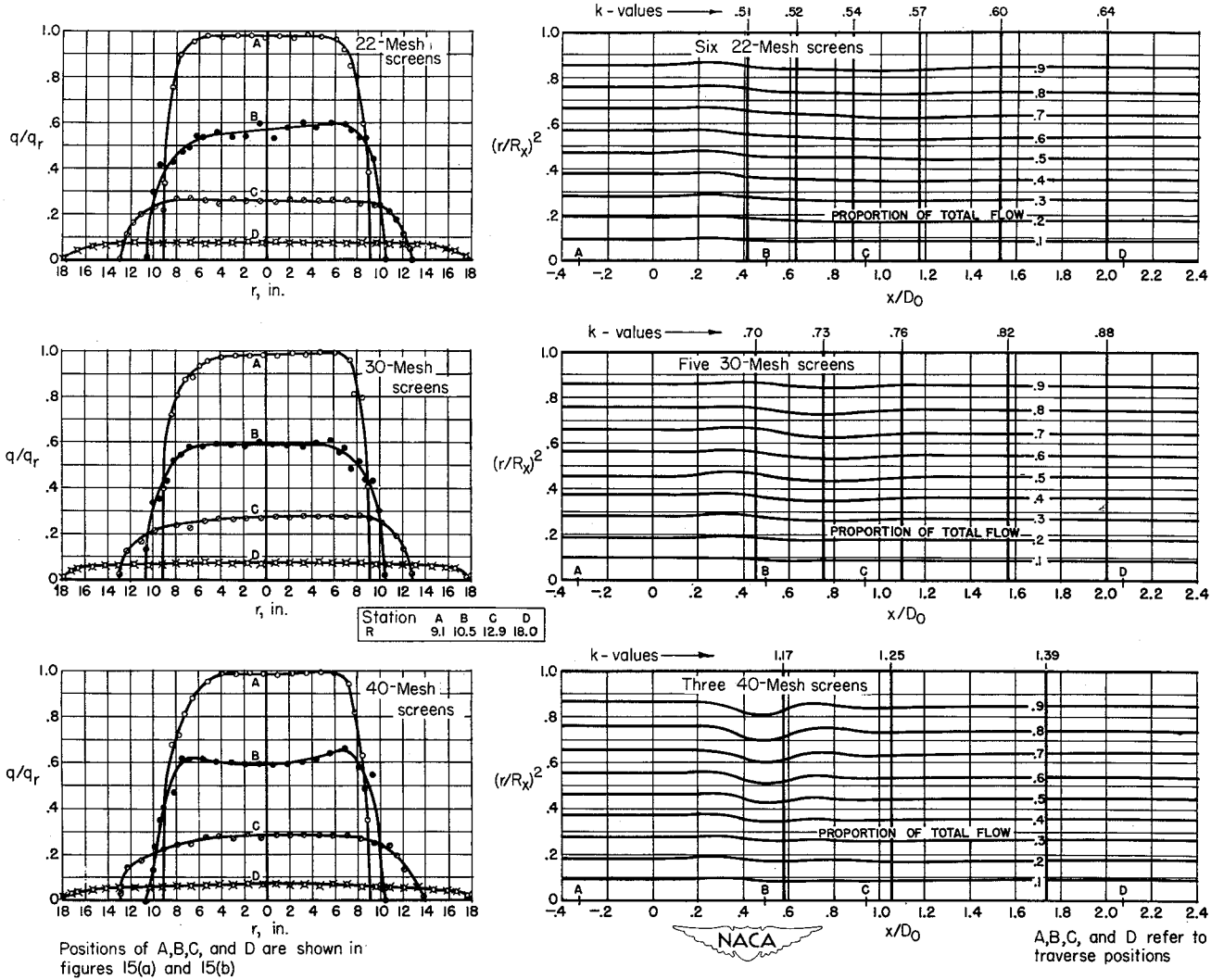
(b) Charts showing dynamic-pressure distributions at various diffuser sections and proportion of diffuser area filled by various proportions of total flow.
