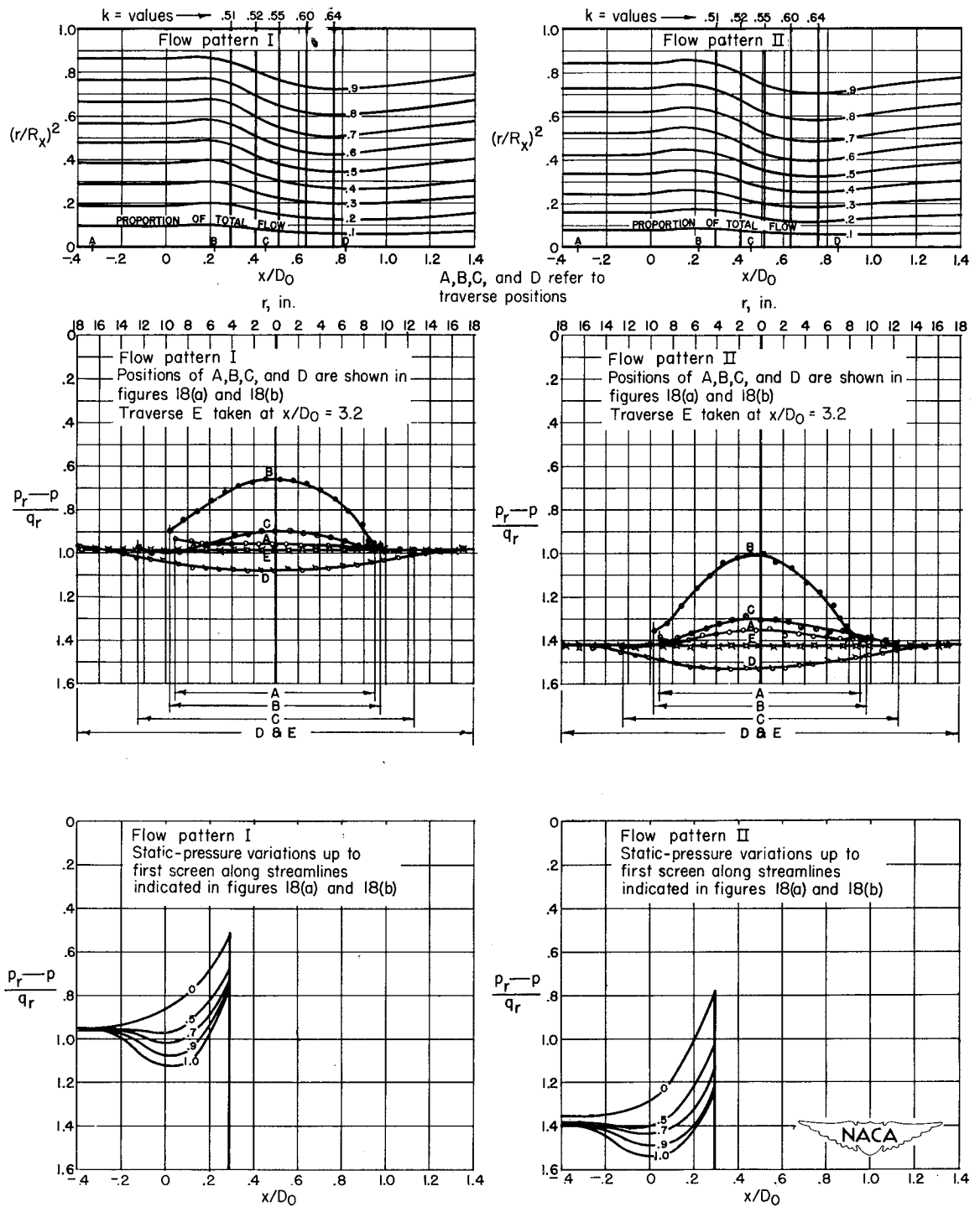
(b) Charts showing proportion of diffuser area filled by various proportions of total flow, static-pressure distributions at various diffuser sections, and static-pressure distributions along selected streamlines.
