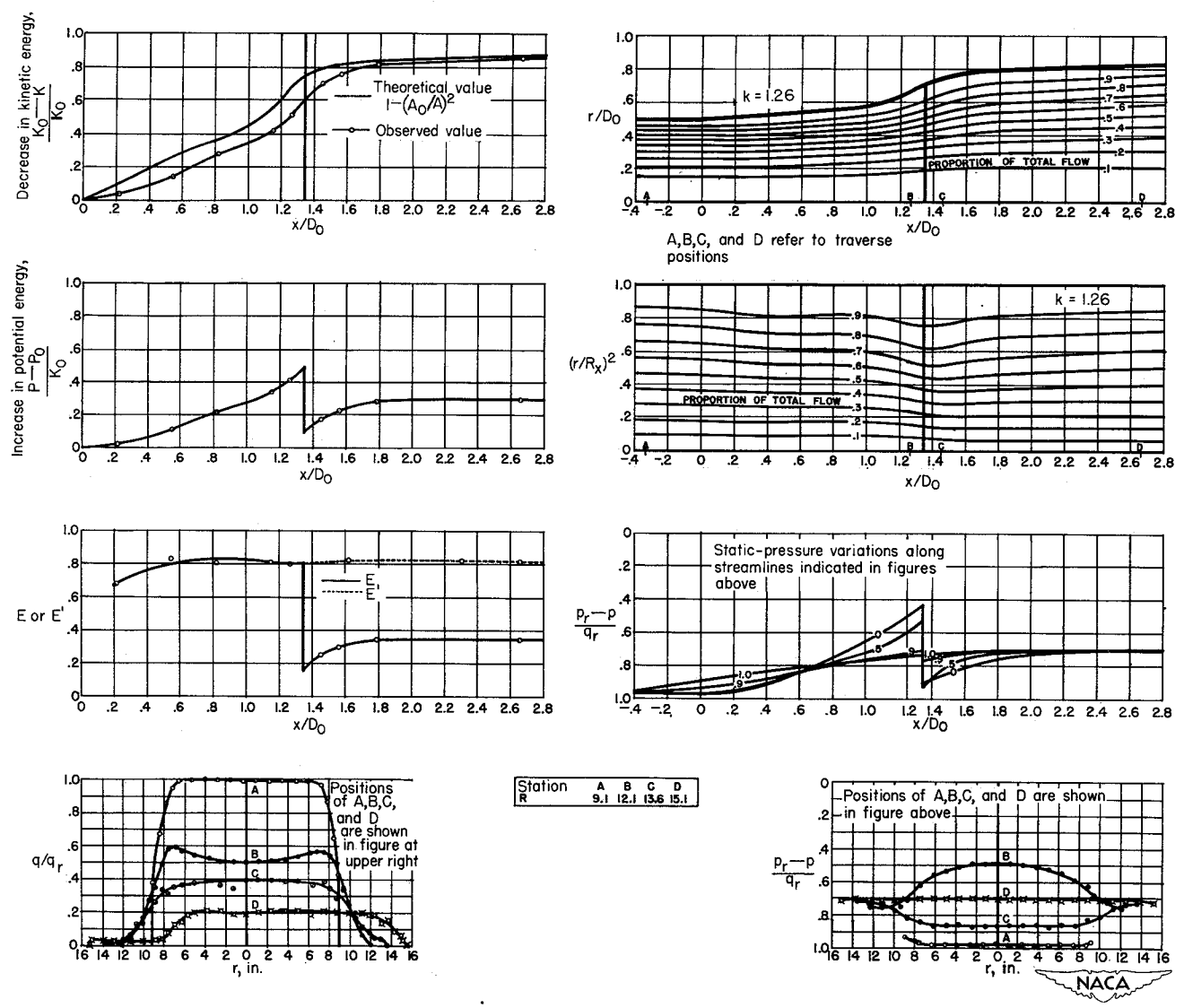
Figure 13.- Results of tests of diffuser C with 40-mesh screen.
