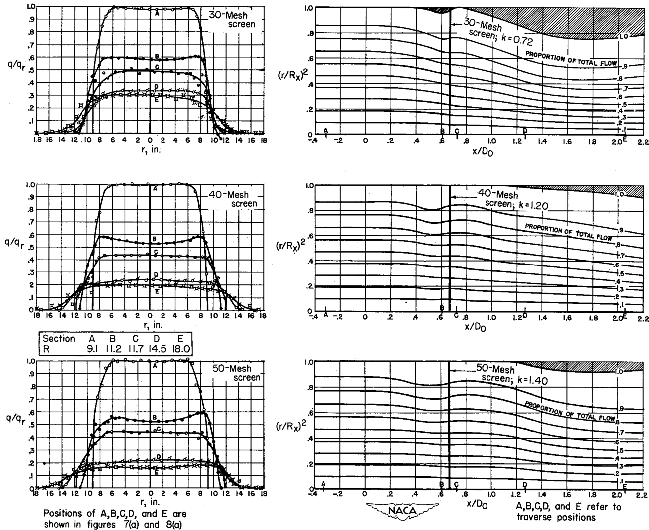
(a) Screens placed 2/3 duct diameter from diffuser entrance.
