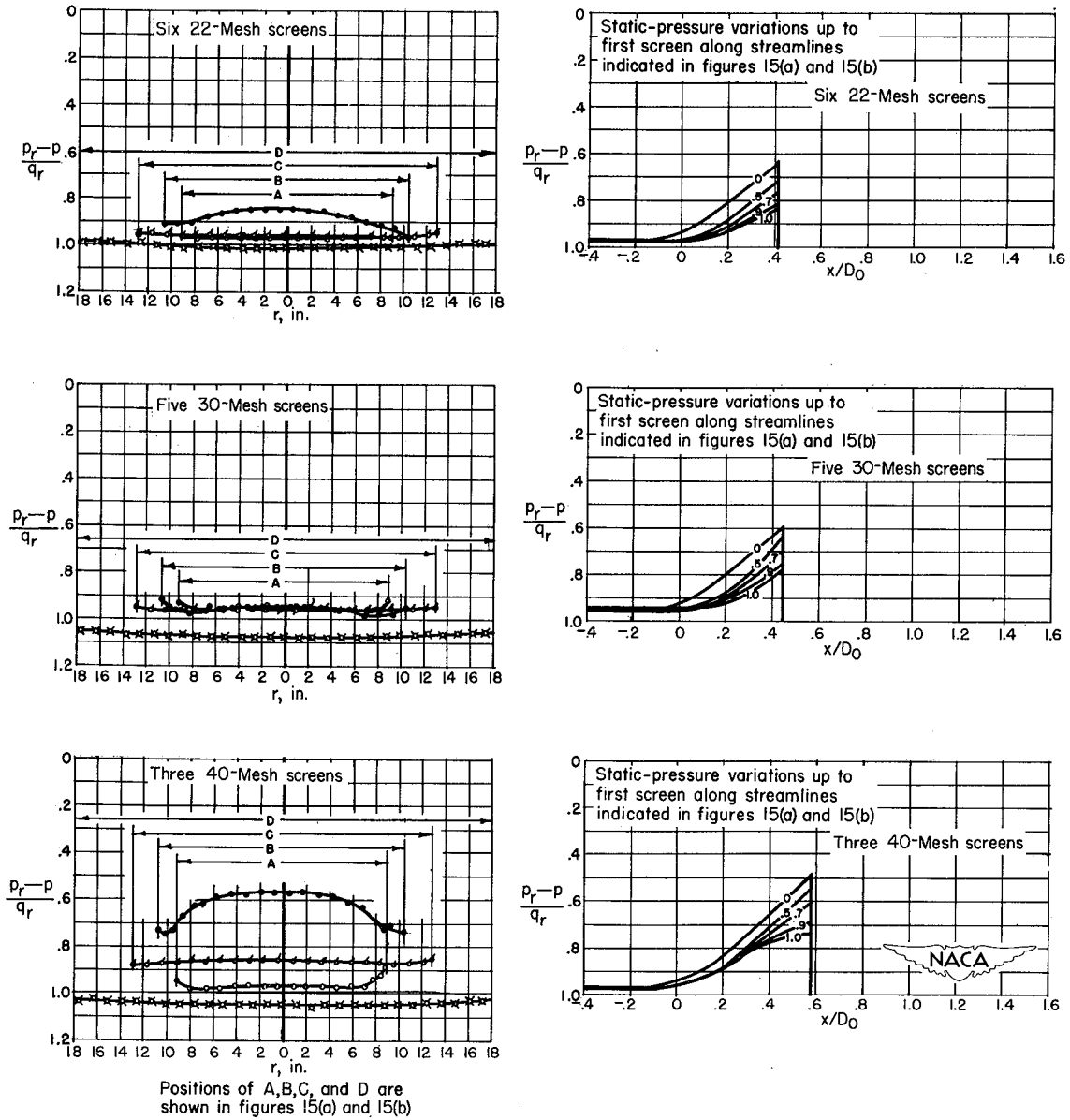
(c) Charts showing static-pressure distributions at various diffuser sections and along selected streamlines.
