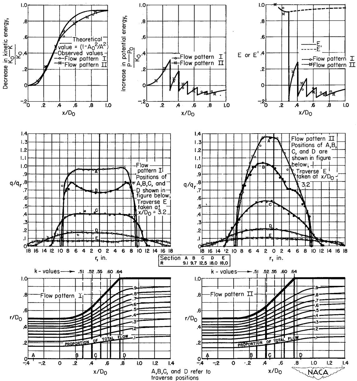
(a) Charts showing changes in kinetic and potential energies, efficiencies, dynamic-pressure distributions, and streamline patterns.
