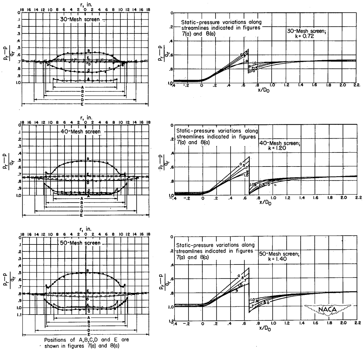
(a) Screens placed 2/3 duct diameter from diffuser entrance.
