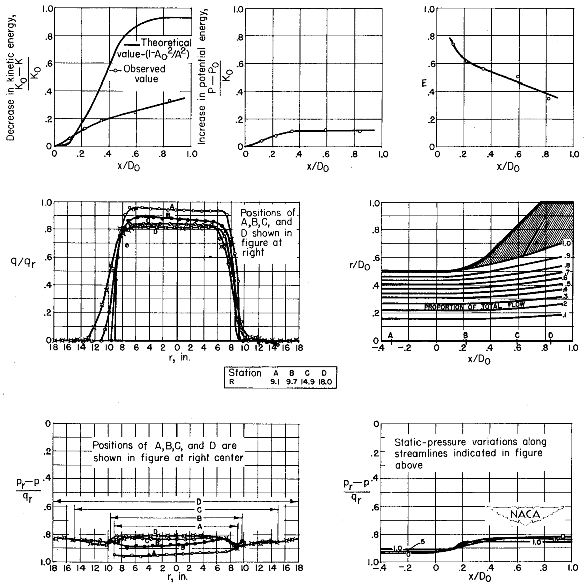
Figure 10.- Results of tests of diffuser B without screens. Charts showing changes in kinetic and potential energies, efficiency, dynamic- and static-pressure distributions at various diffuser sections, approximate streamline pattern, and static-pressure distributions along selected streamlines.
