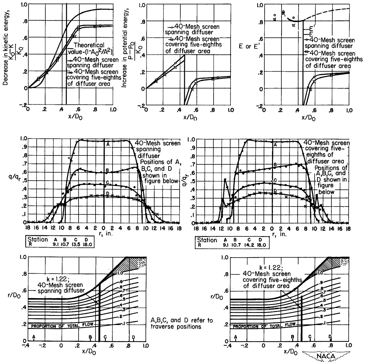
(c) Single 40-mesh screen placed 0.45 duct diameter from diffuser entrance. (See also fig. 12(c).)
