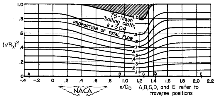
(c) Screens placed 1\frac{1}{3} duct diameters from diffuser entrance.
