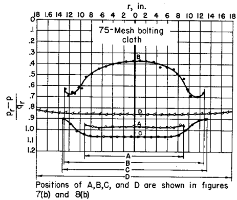
(b) Screens placed 1.0 duct diameter from diffuser entrance.
