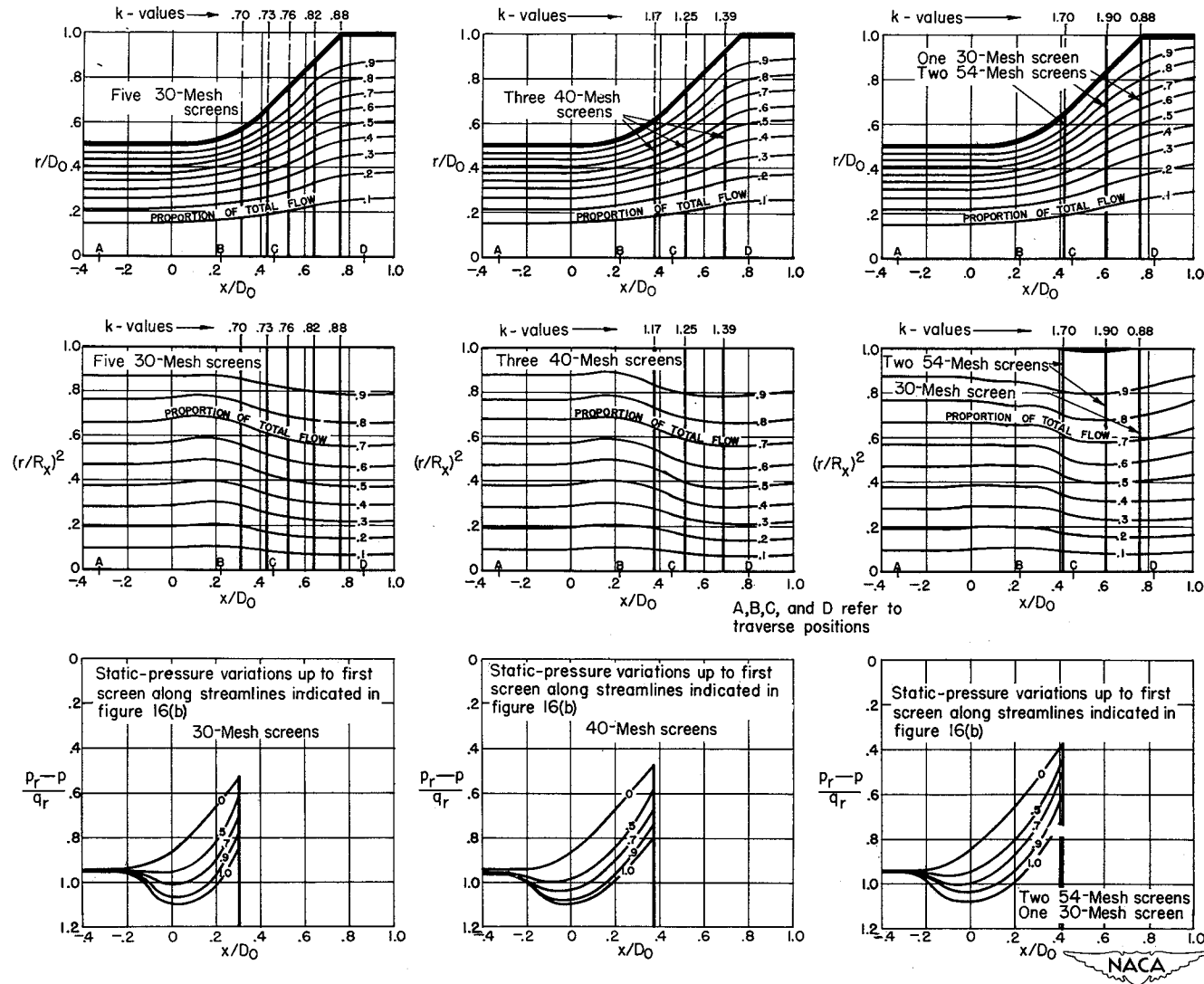
(a) Charts showing streamline patterns, proportion of diffuser area filled by various proportions of total flow, and static-pressure distributions along selected streamlines.
