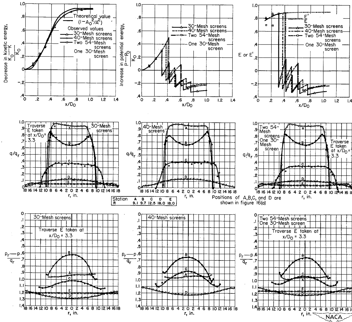
(b) Charts showing changes in kinetic and potential energies, efficiencies, and dynamic- and static-pressure distributions at various diffuser sections.
