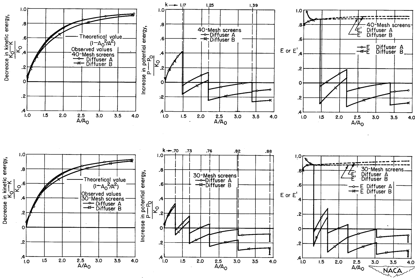
Figure 17.- Comparison of test results of diffusers A and B with the 30- and 40-mesh multiple screen combinations shown in figures 15 and 16. Charts showing changes in kinetic and potential energies and efficiencies.
