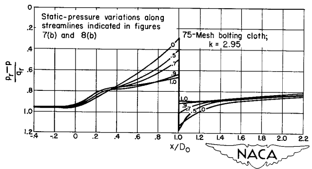
(b) Screens placed 1.0 duct diameter from diffuser entrance.
