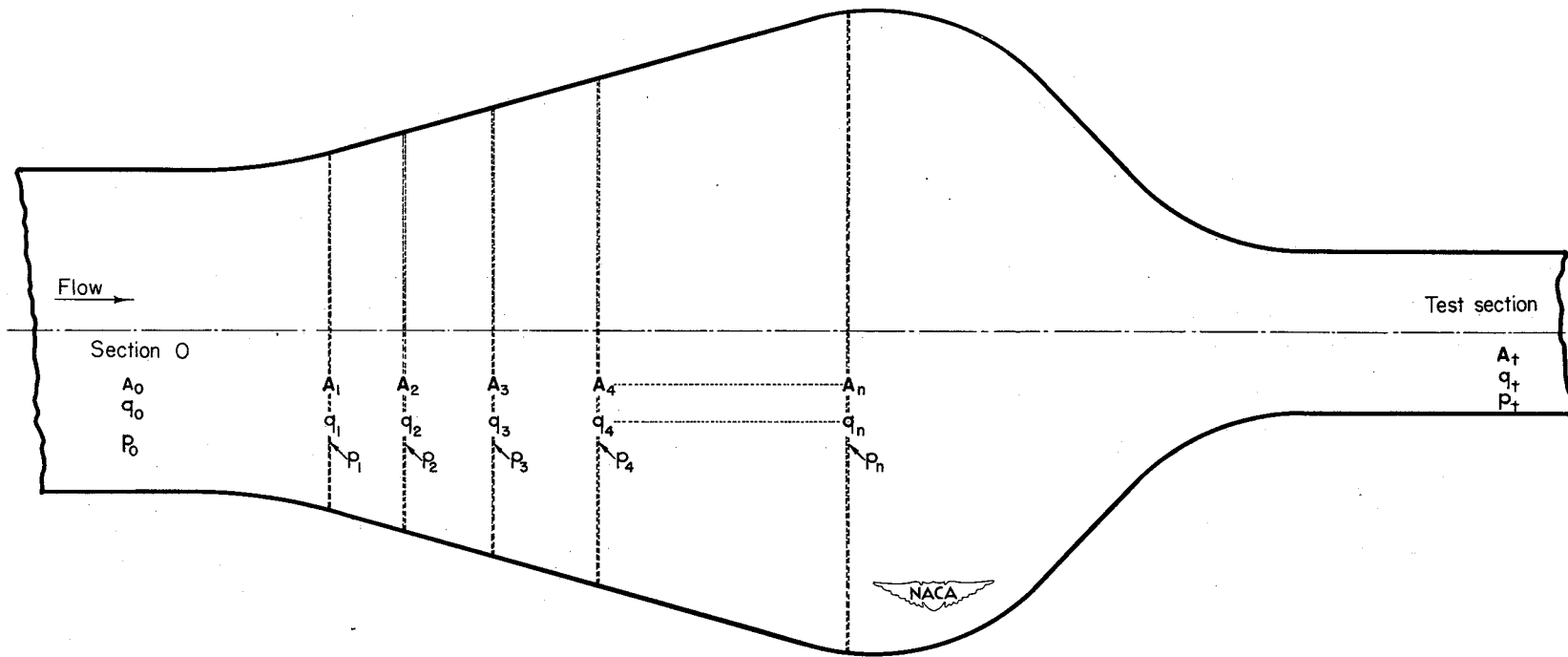
Figure 14.- Schematic diagram showing possible application of a diffuser screen combination to a wind tunnel.
