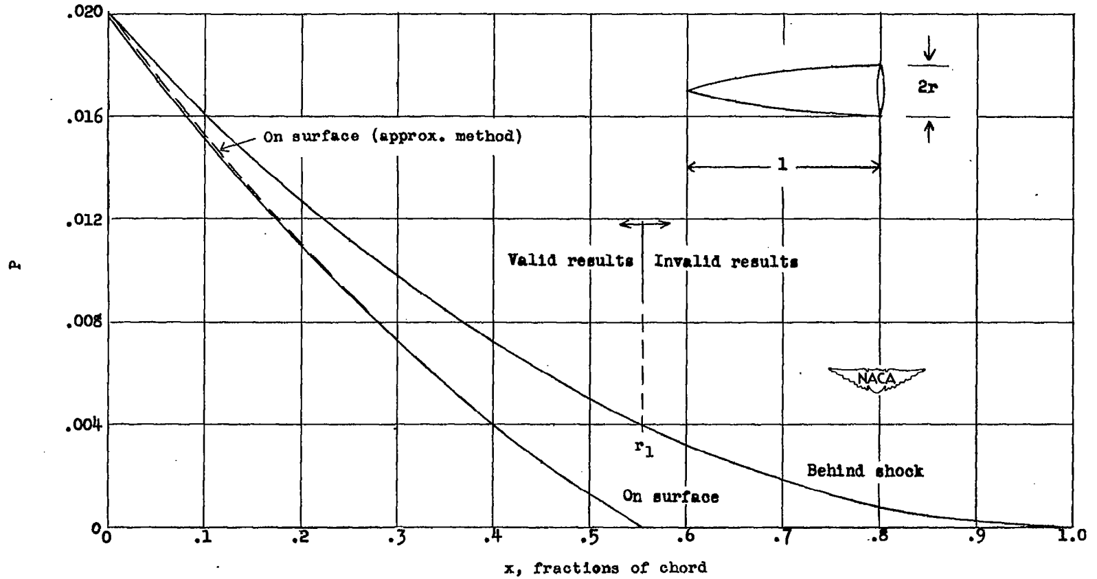
Figure 4.- Pressure distribution over parabolic body of revolution. Fineness ratio, 10; \alpha = 0 radian; C_D = 0.0042 .
