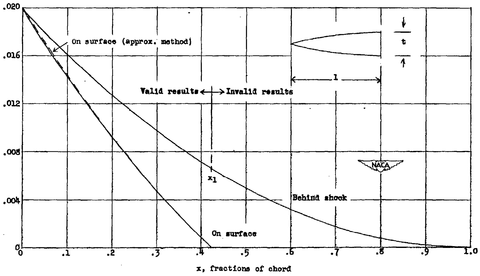
Figure 3.- Pressure distribution over parabolic airfoil. Thickness ratio, 0.10.
