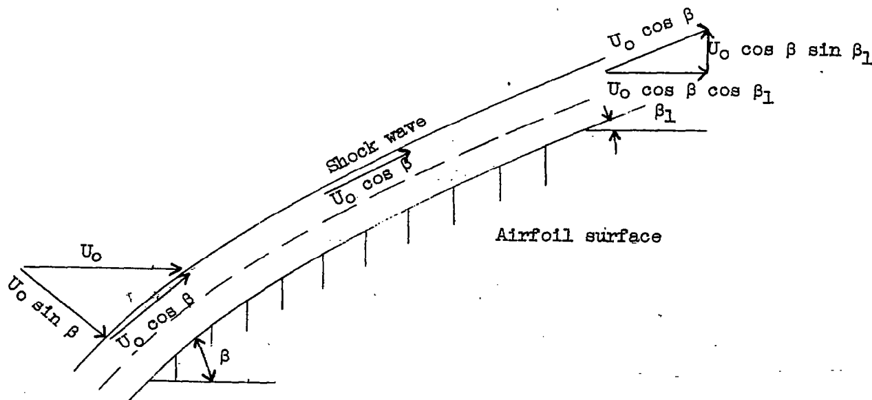
Figure 2.— Velocities over a surface.
