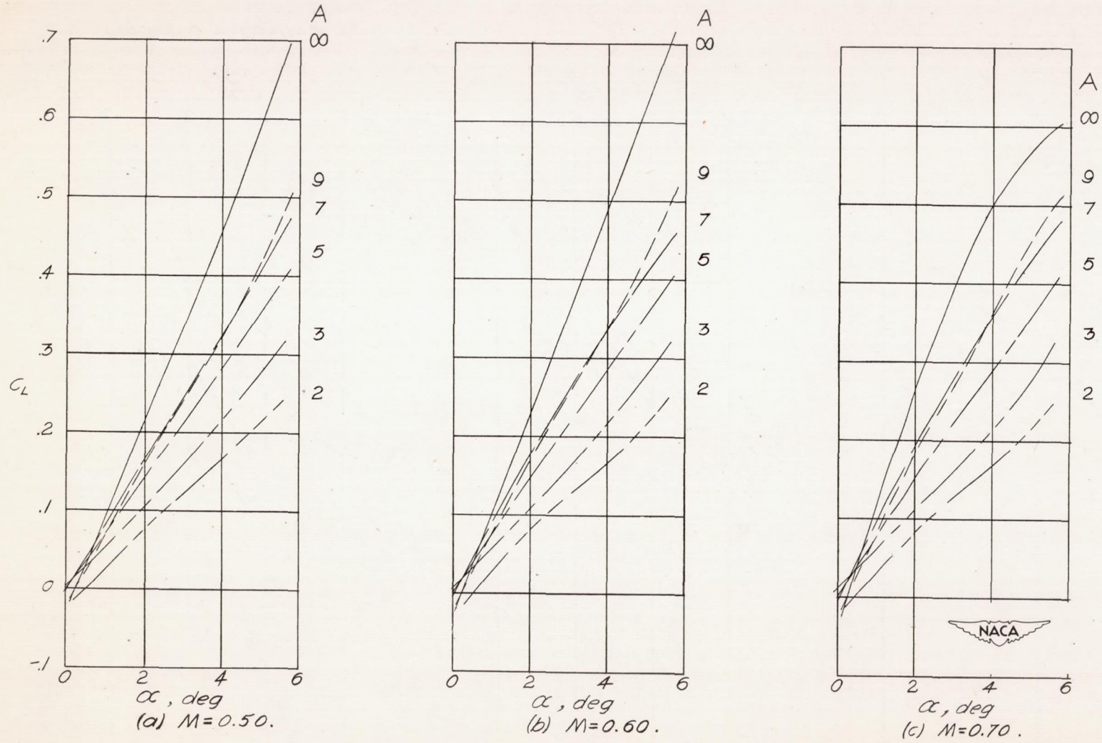
Figure 3.- Lift curves for various aspect ratios and Mach numbers. NACA 0012 section; rectangular plan form and tip.
