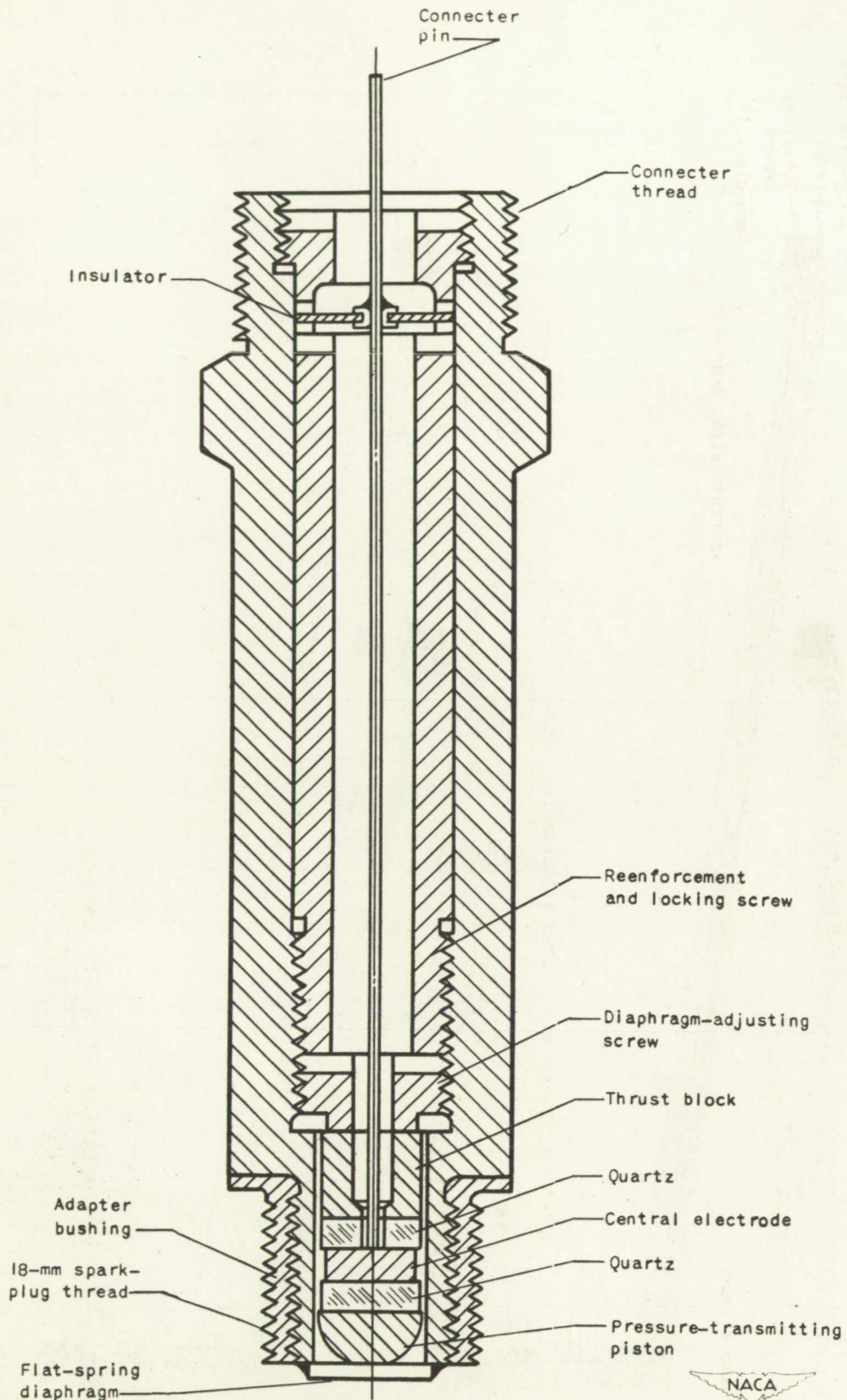
Figure 4. - Piezoelectric pressure pickup.
