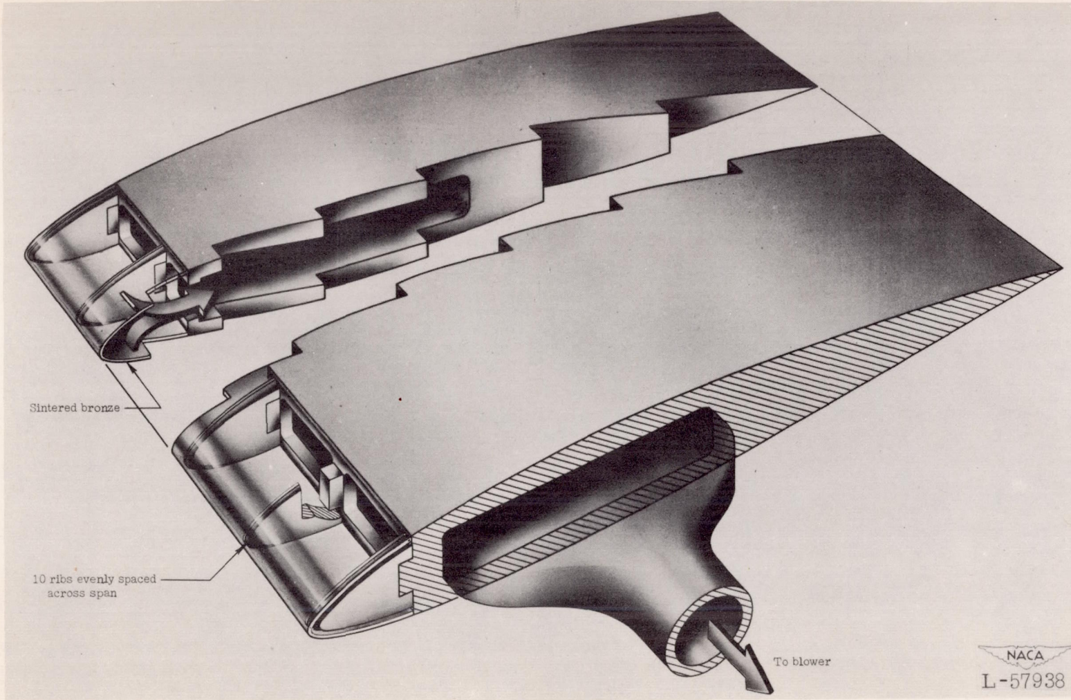
Figure 1.- Sketch of NACA 64 1 A212 airfoil showing construction of leading edge and ducting system.
