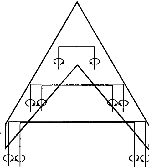
(a) Approximation by horseshoe vortices of 0° sweep.
