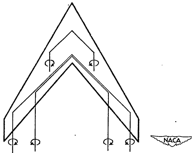
(b) Approximation by horseshoe vortices of 45° sweep.
