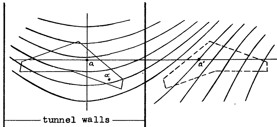
(a) Chart representing field of doubly infinite array of unit doublets with center doublet omitted; origin of chart is placed on point a .
