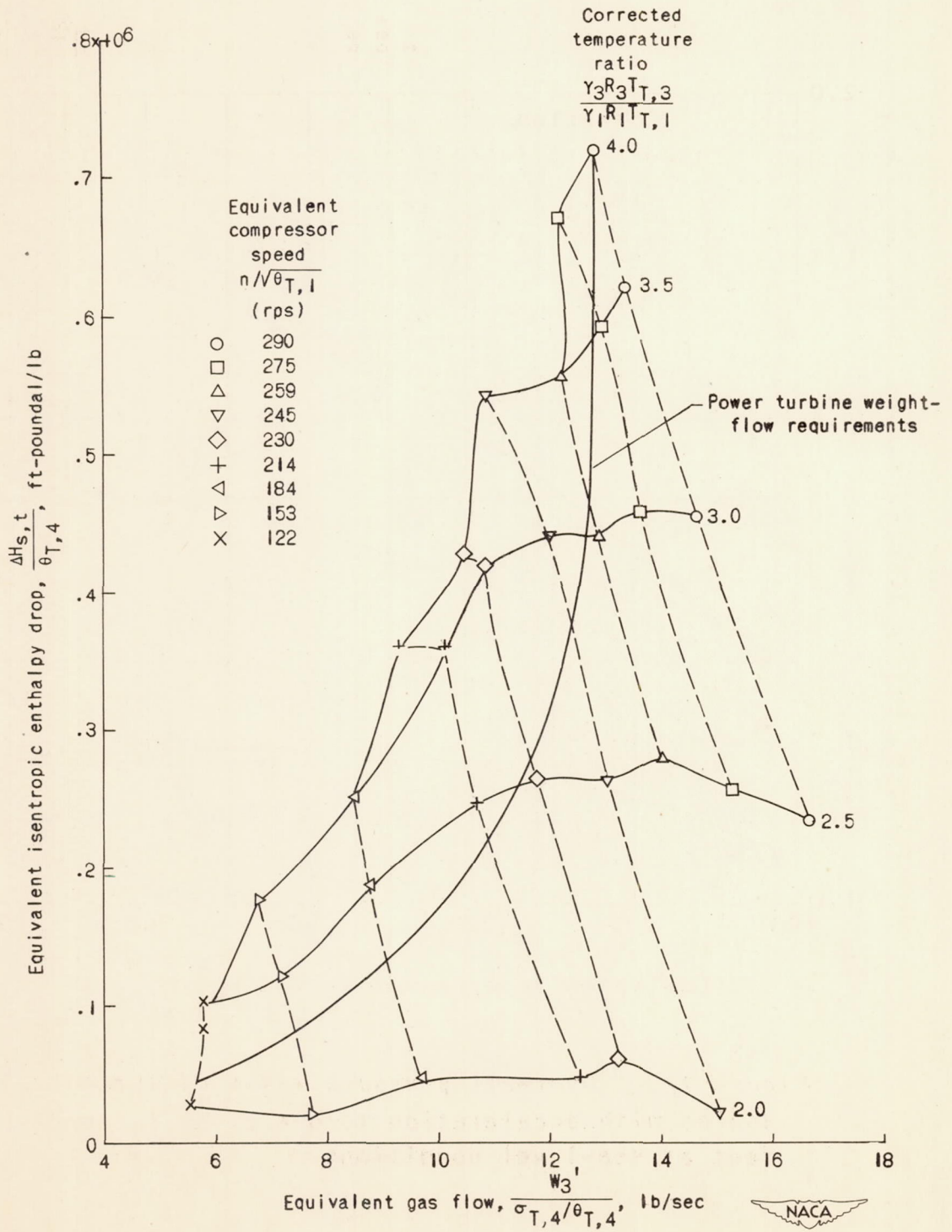
Figure 23. - Superposition of gas generator and power turbine characteristics.
