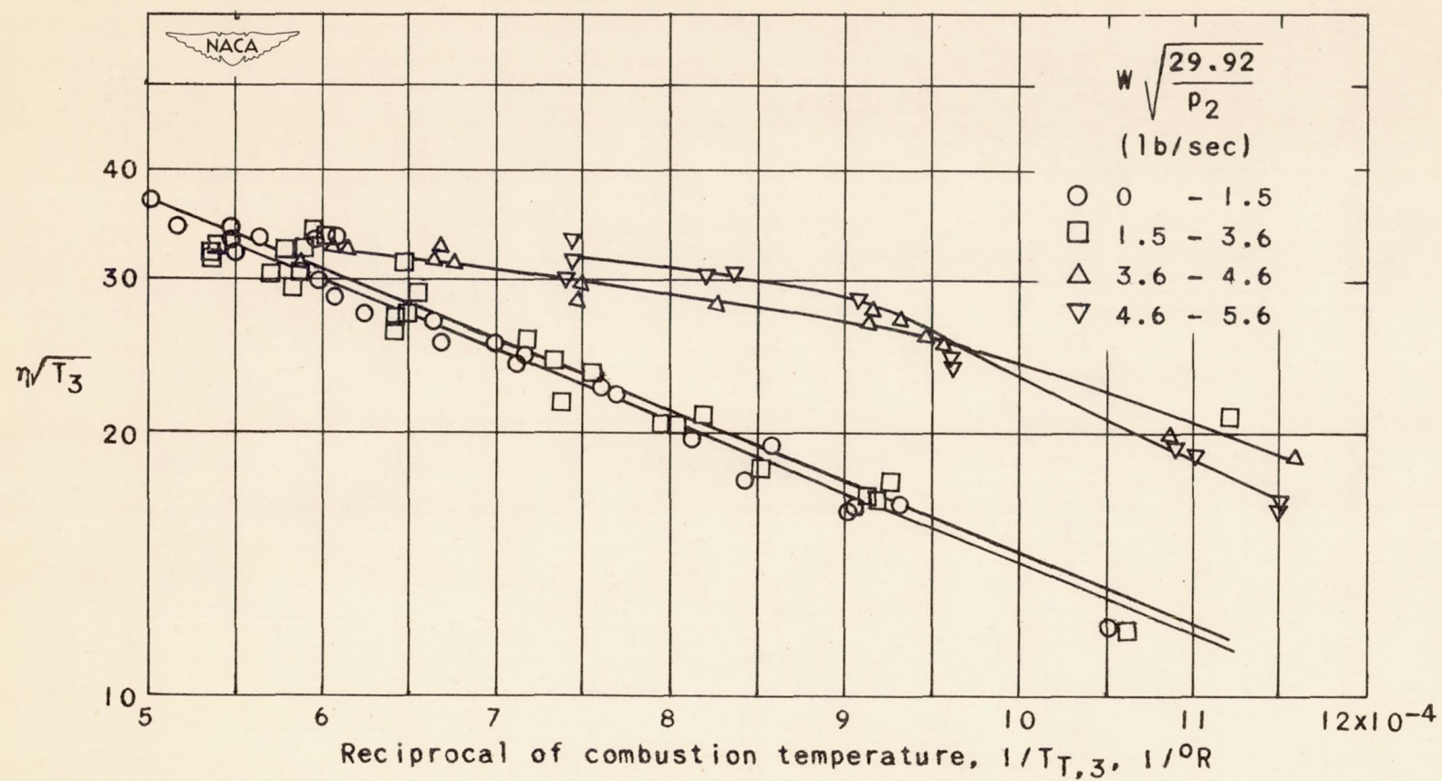
Figure 11. - Combustion performance of burner.
