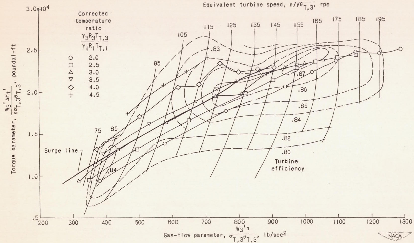
Figure 18. - Estimated turbine performance at various temperature ratios in engine with assumed modifications. Compressor-inlet stagnation temperature and pressure, 480° R and 1414 pounds per square foot, respectively.
