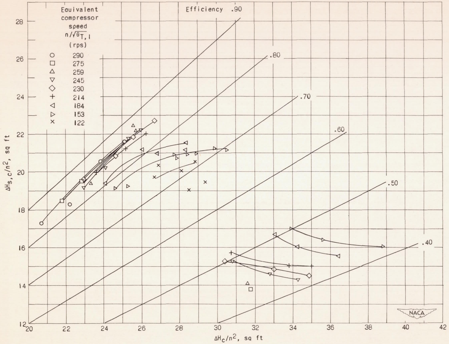
Figure 5. - Selected compressor data.
