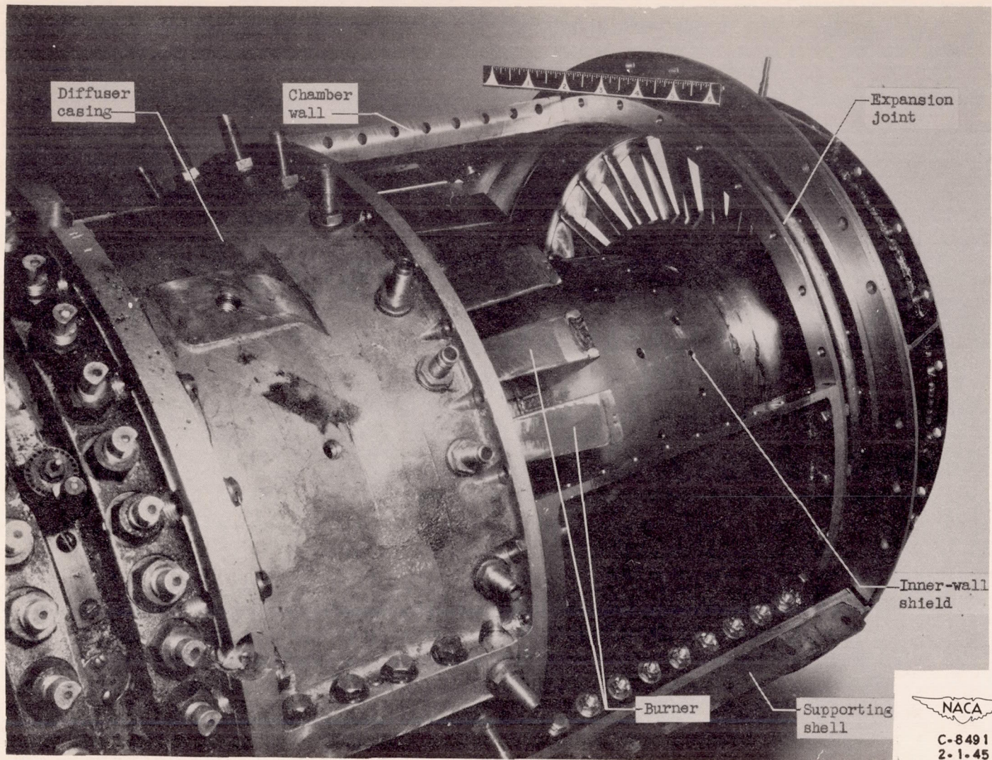
Figure 2. - View of burners and combustion-chamber structure.
