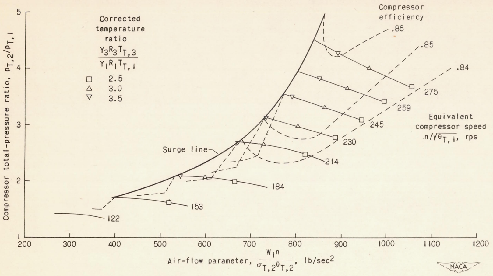
Figure 21. - Compressor operation with acceleration torque of 38.1 pound-feet at sea-level conditions.
