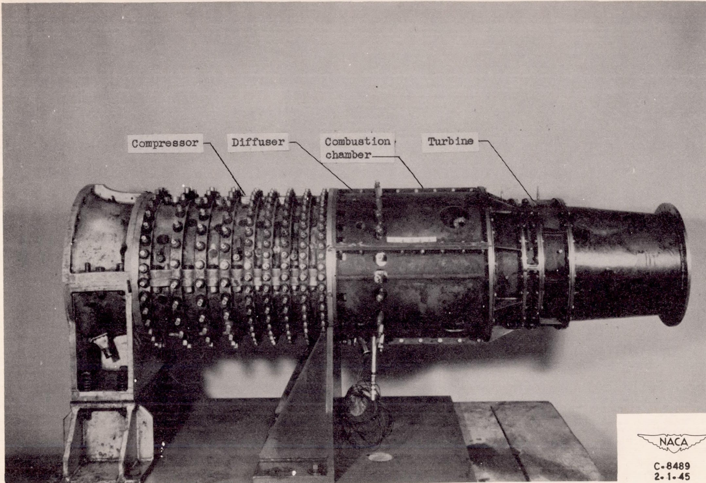
Figure 1. - NACA research jet engine.
