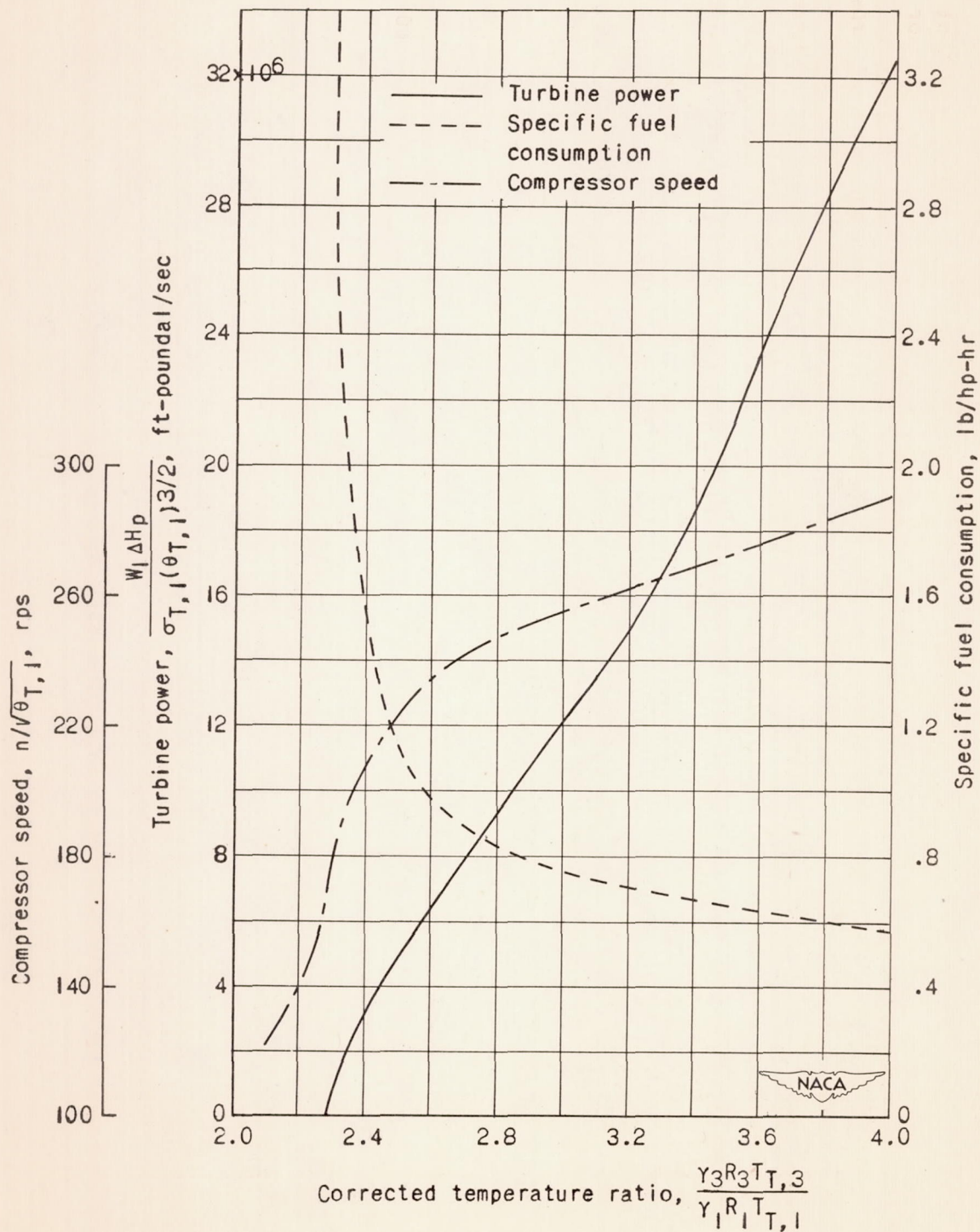
Figure 24. - Over-all performance characteristics of gas turbine.
