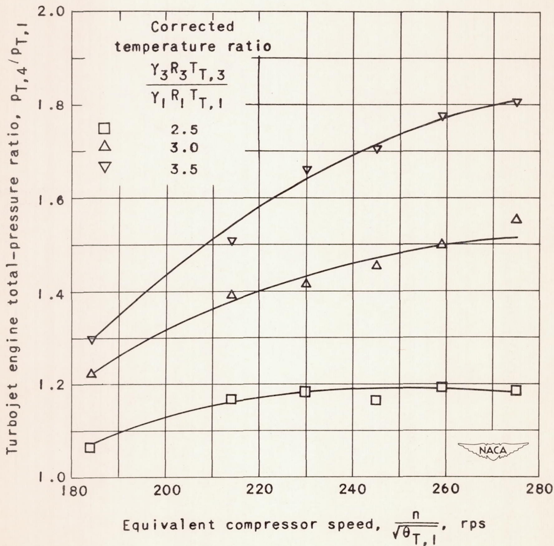
Figure 22. - Over-all pressure ratio of turbojet engine with acceleration torque of 38.1 pound-feet at sea-level conditions.
