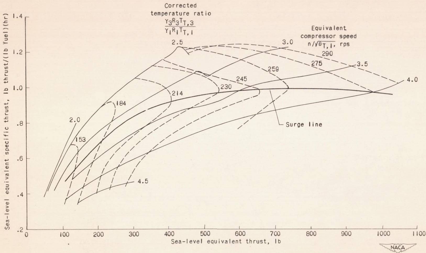
Figure 20. - Static performance of turbojet engine with assumed modifications. Compressor-inlet stagnation temperature and pressure, 480° R and 1414 pounds per square foot, respectively.
