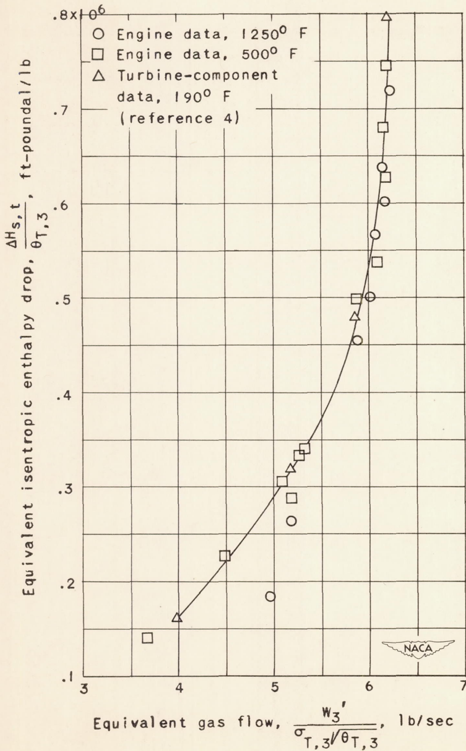
(a) Corrections applied to data of figure 7. Figure 8. - Equivalent isentropic enthalpy drop and gas flow through turbine corrected for clearance expansion.
