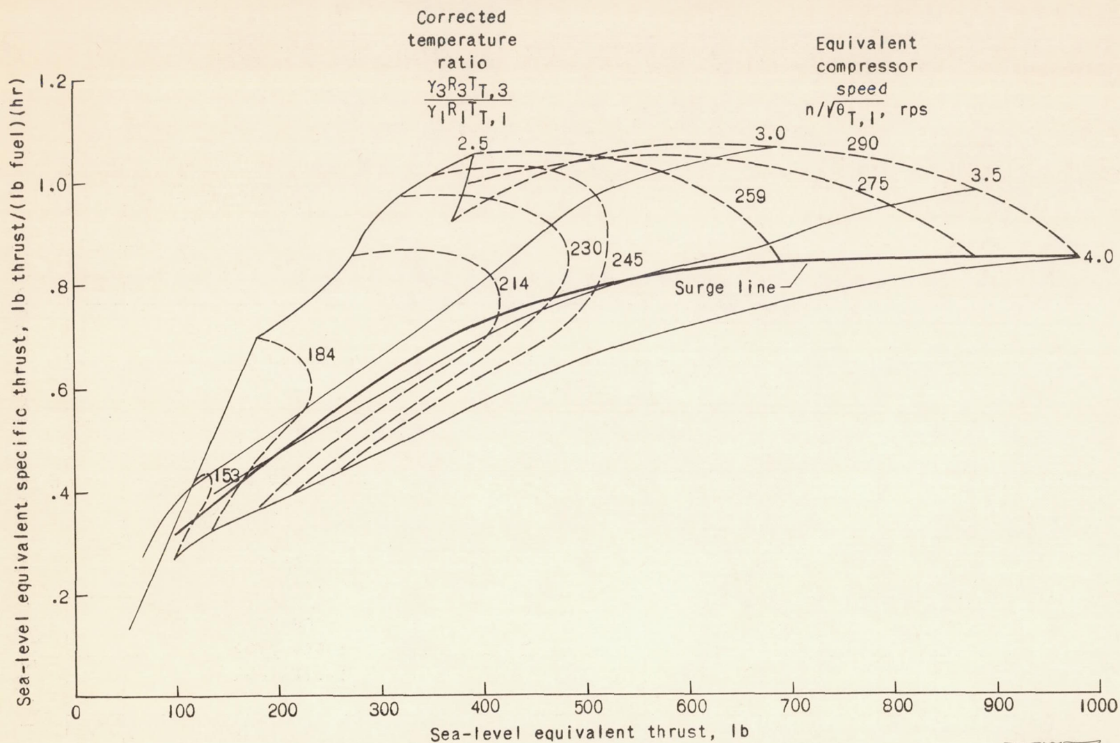
Figure 17. - Equivalent static performance of turbojet engine. Compressor-inlet stagnation temperature and pressure, 480° R and 1414 pounds per square foot, respectively.
