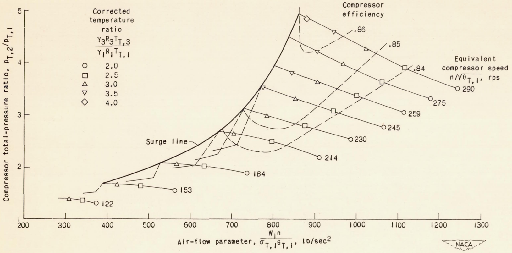
Figure 19. - Compressor performance at various temperature ratios in turbojet engine with assumed modifications. Compressor-inlet stagnation temperature and pressure, 480° R and 1414 pounds per square foot, respectively.
