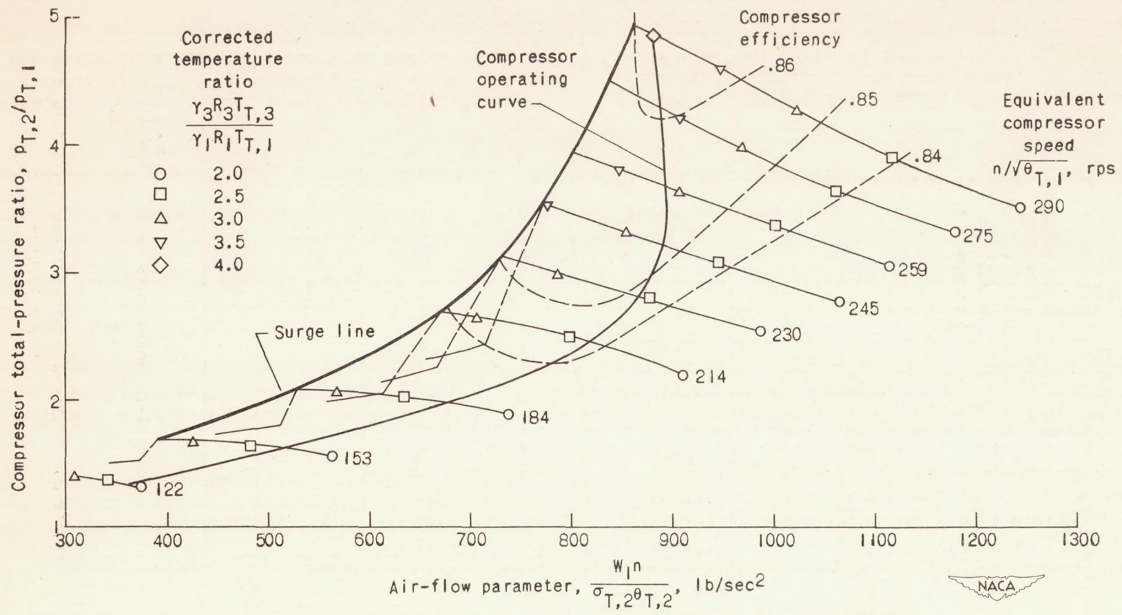
Figure 25. - Estimated compressor performance in gas-turbine engine.
