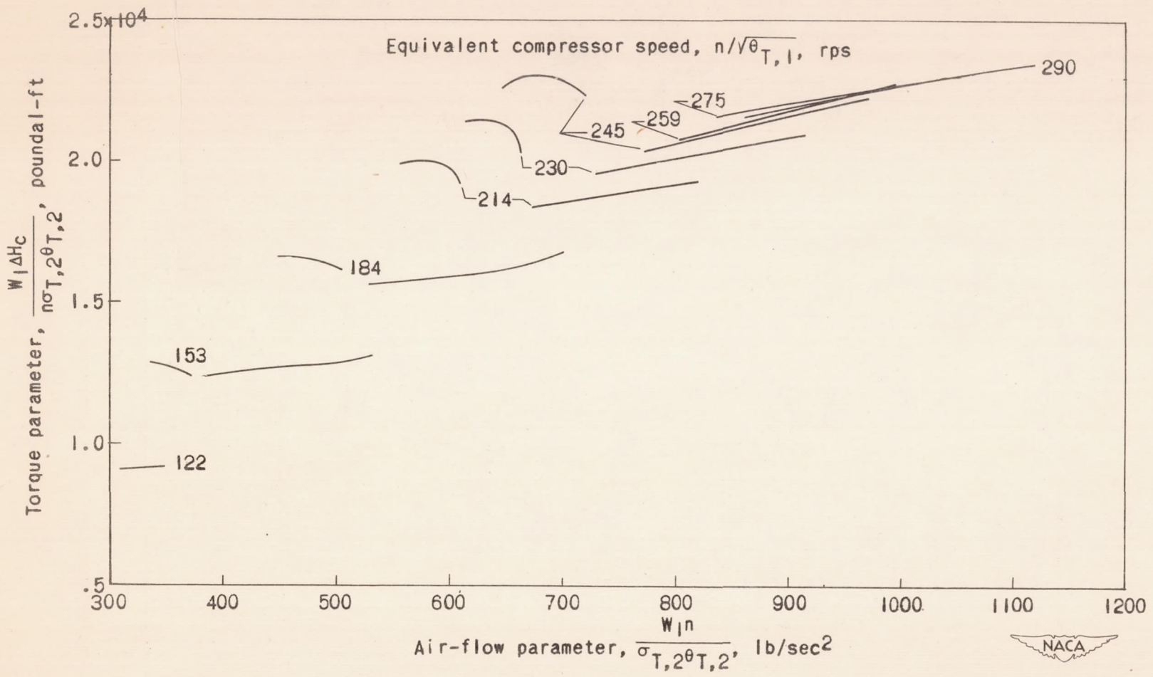
Figure 12. - Compressor performance in parameters for engine computations.
