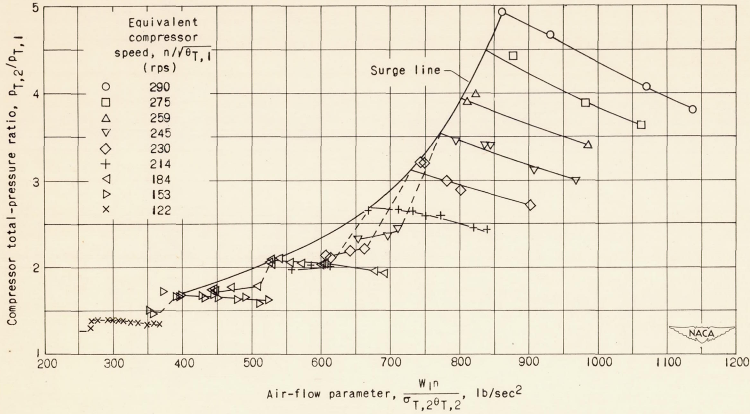
Figure 6. - Selected compressor-pressure-ratio and air-flow data.
