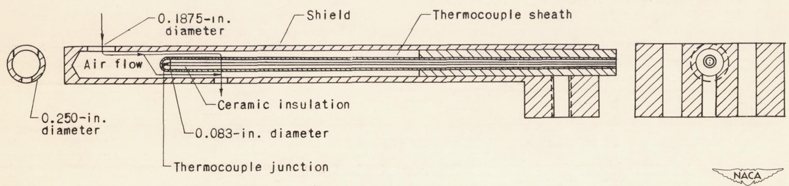
Figure 4. - Shielded-type thermocouple composed of chromel-alumel thermocouple wire and Inconel shield and sheath material.
