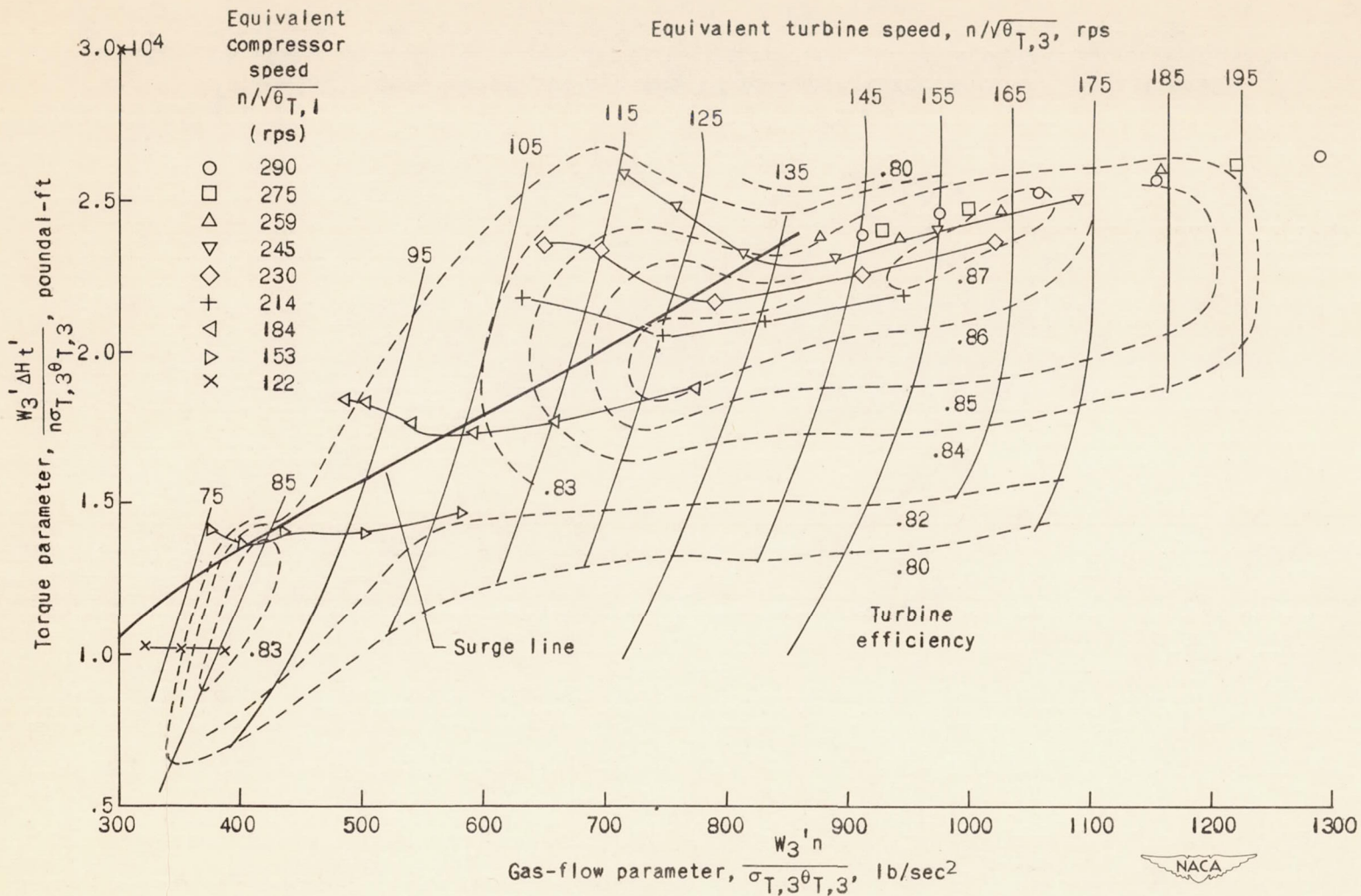
Figure 13. - Matching chart based on engine experiments. Component performance corrected for losses, clearance expansion, and change in gas properties. Compressor-inlet stagnation temperature and pressure, 480° R and 1414 pounds per square foot, respectively.
