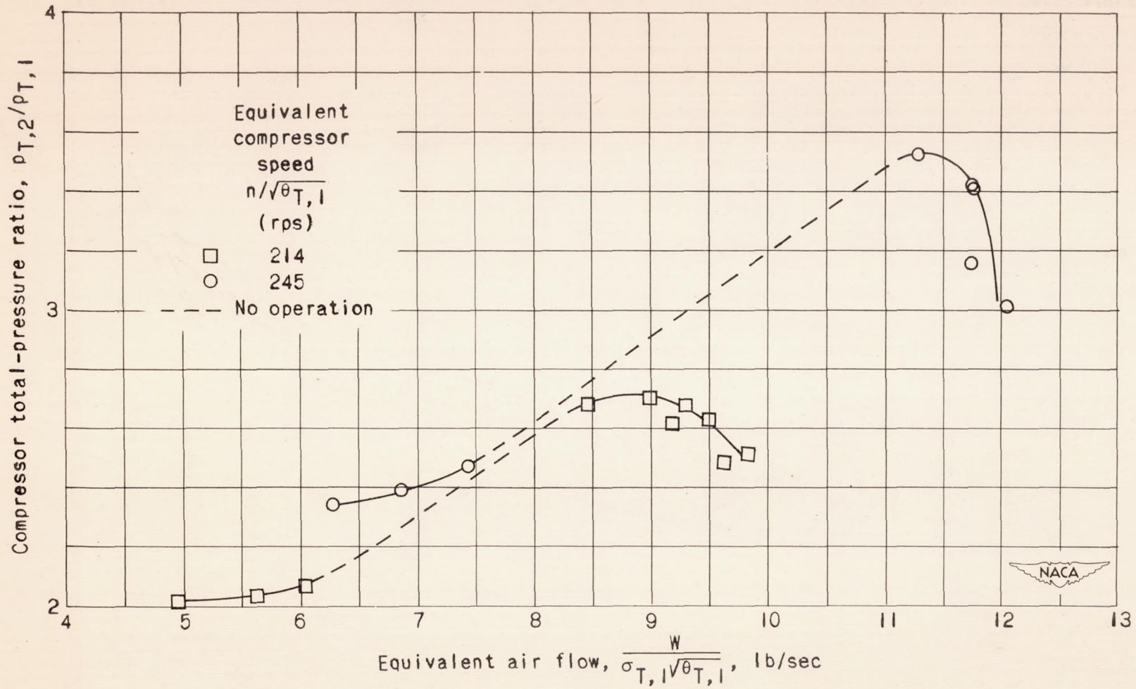
Figure 16. - Variation of compressor pressure ratio with inlet flow.
