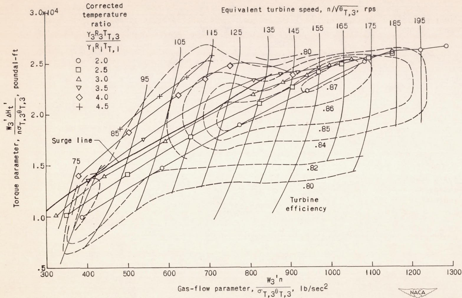
Figure 14. - Turbine operating conditions at various temperature ratios in engine. Compressor-inlet stagnation temperature and pressure, 480° R and 1414 pounds per square foot, respectively.
