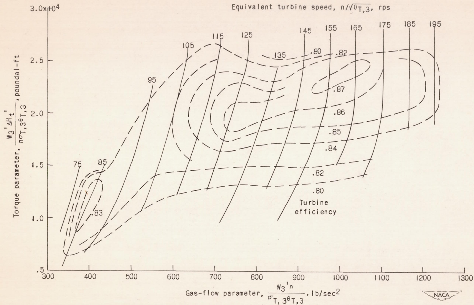
Figure 10. - Corrected performance of turbine in parameters for engine computations.
