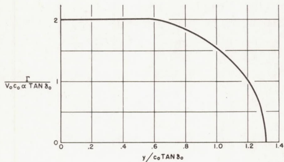
Figure 11.— Spanwise distribution of circulation for swept-back wing at M_0=1 , b=1.325 c_o \tan \delta_o and AR=4.57 \tan \delta_o .
