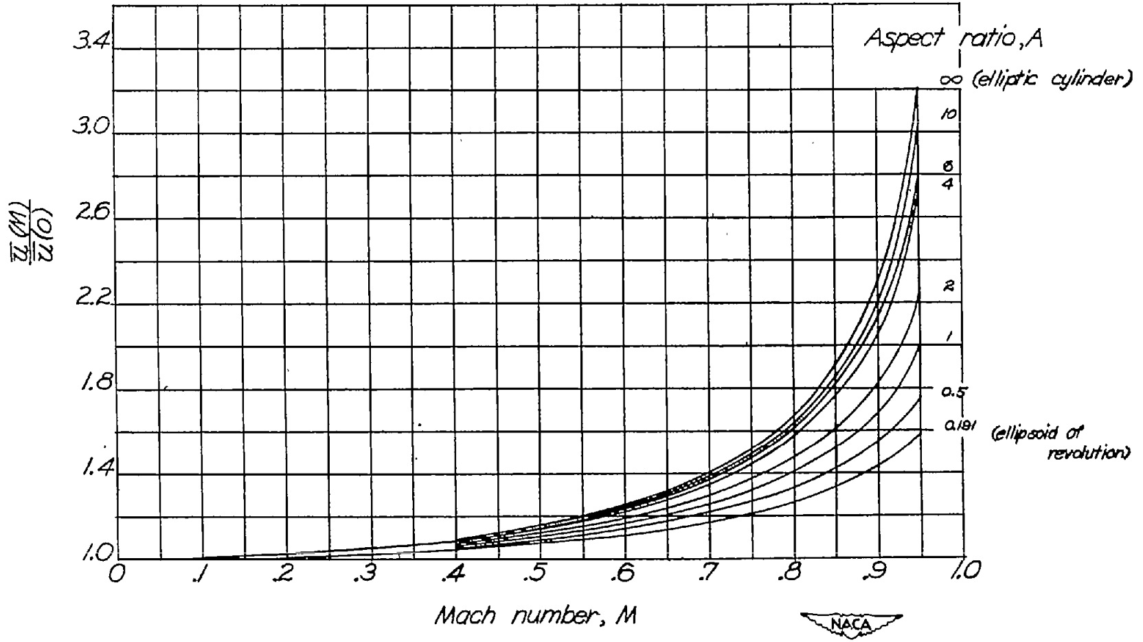
Figure 5.- Variation of compressibility effect with Mach number for ellipsoids having various aspect ratios, Thickness ratio, 0.15.
