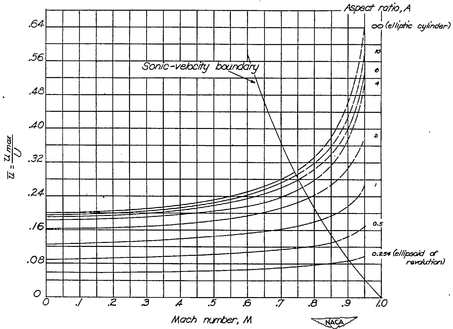
Figure 3.- Variation with Mach number of maximum incremental velocity for ellipsoids having various aspect ratios. Thickness ratio, 0.20.
